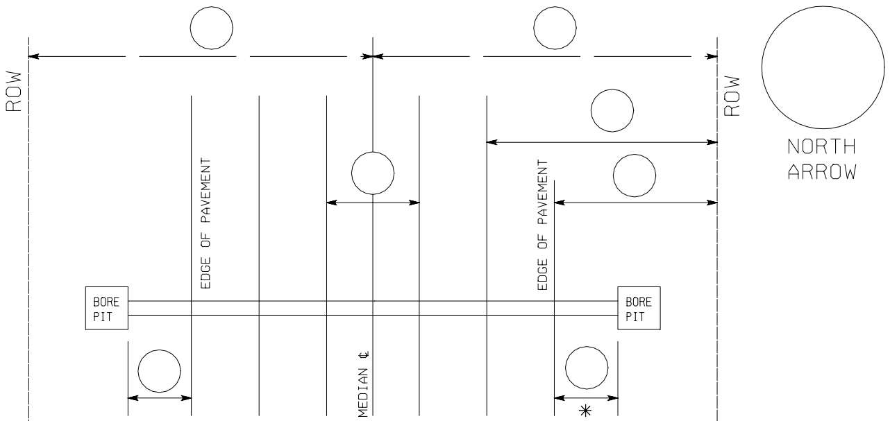
PLAN VIEW
