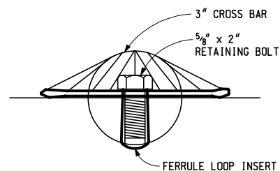
CROSS BAR ATTACHMENT DETAIL
