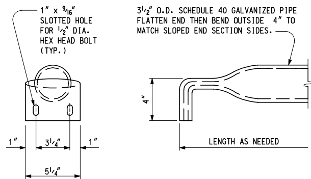
CROSS TUBE
