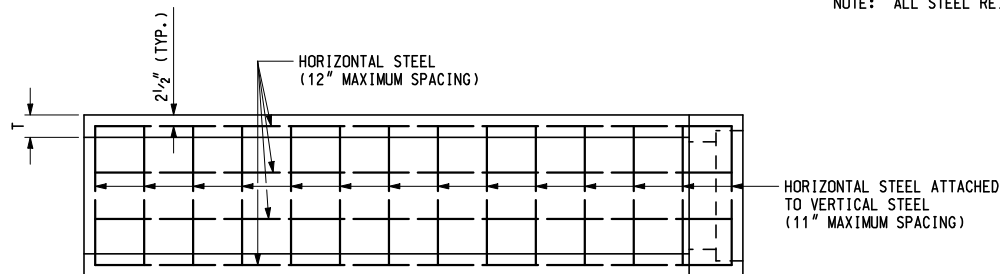
PLAN VIEW
