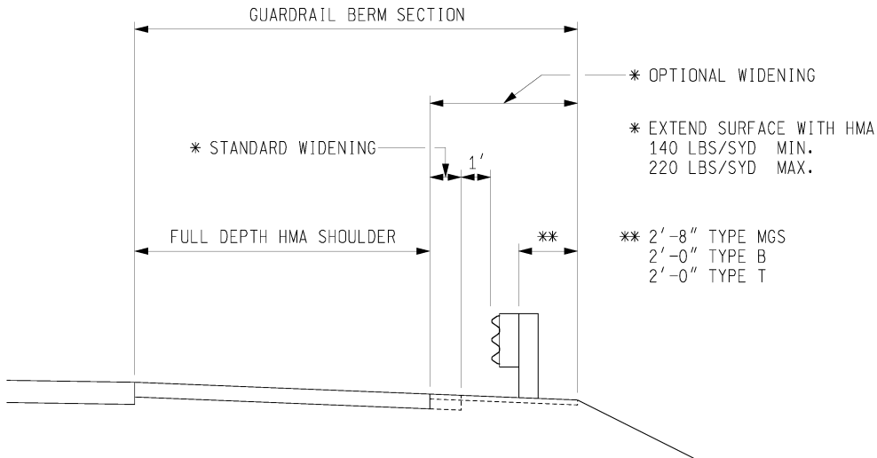
PAVED WIDENING FOR FULL DEPTH HMA SHOULDERS
