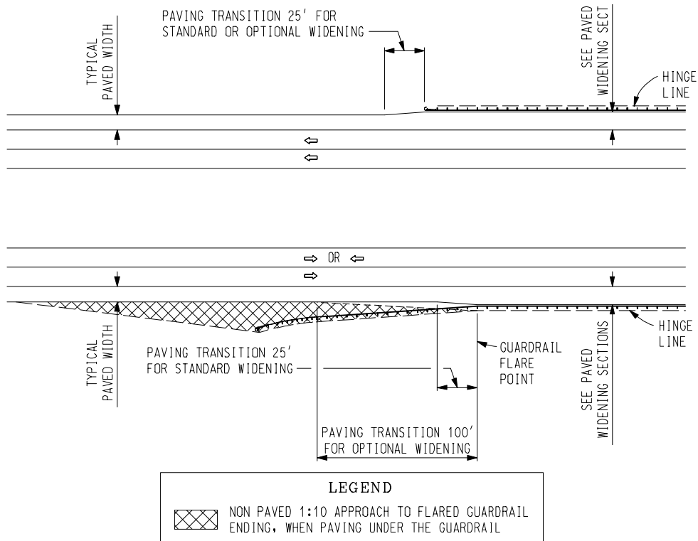
TRANSITIONS FOR ENDING WIDENED SHOULDER PAVING
