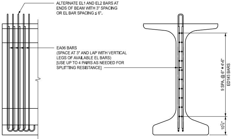
END OF BEAM ADDITIONAL REINFORCEMENT [[USE IF REQUIRED FOR SPLITTING RESISTANCE]]
