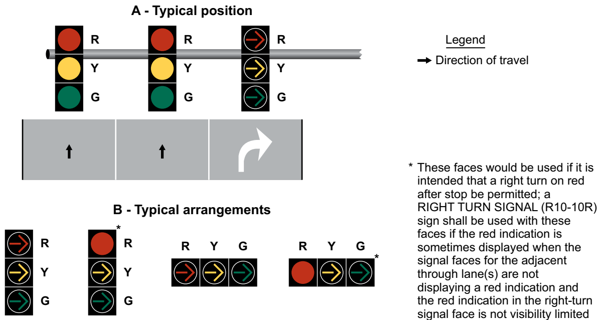
Figure 4D-17. Typical Position and Arrangements of Separate Signal Faces for Protected Only Mode Right Turns
