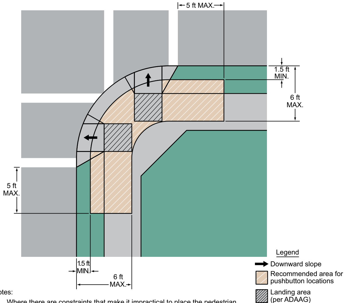
Figure 4E-3. Pushbutton Location Area
