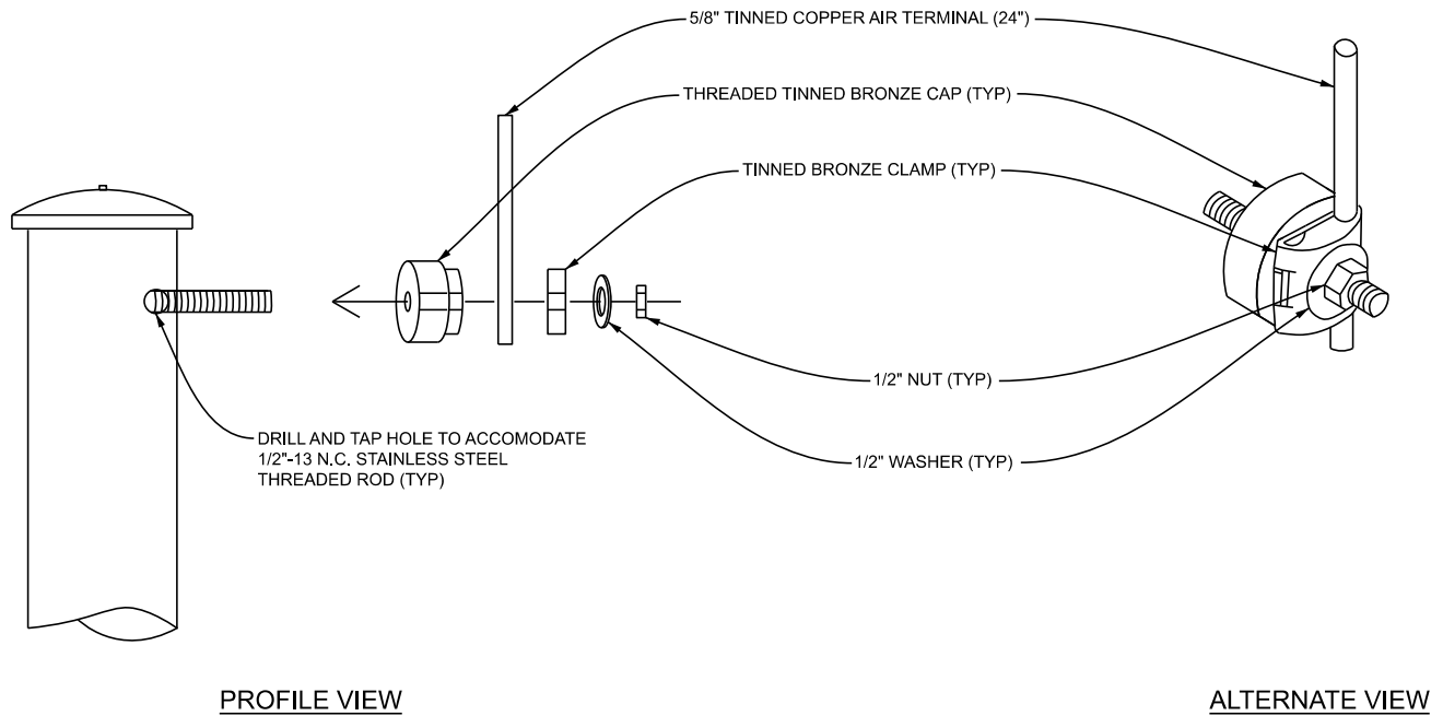
I DETAIL - LIGHTNING PROTECTION CLAMP ON MAST ARM POLE N.T.S.
