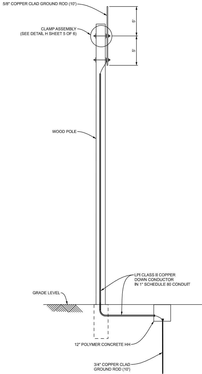
B DETAIL - LIGHTNING PROTECTION ON WOOD POLE N.T.S.
