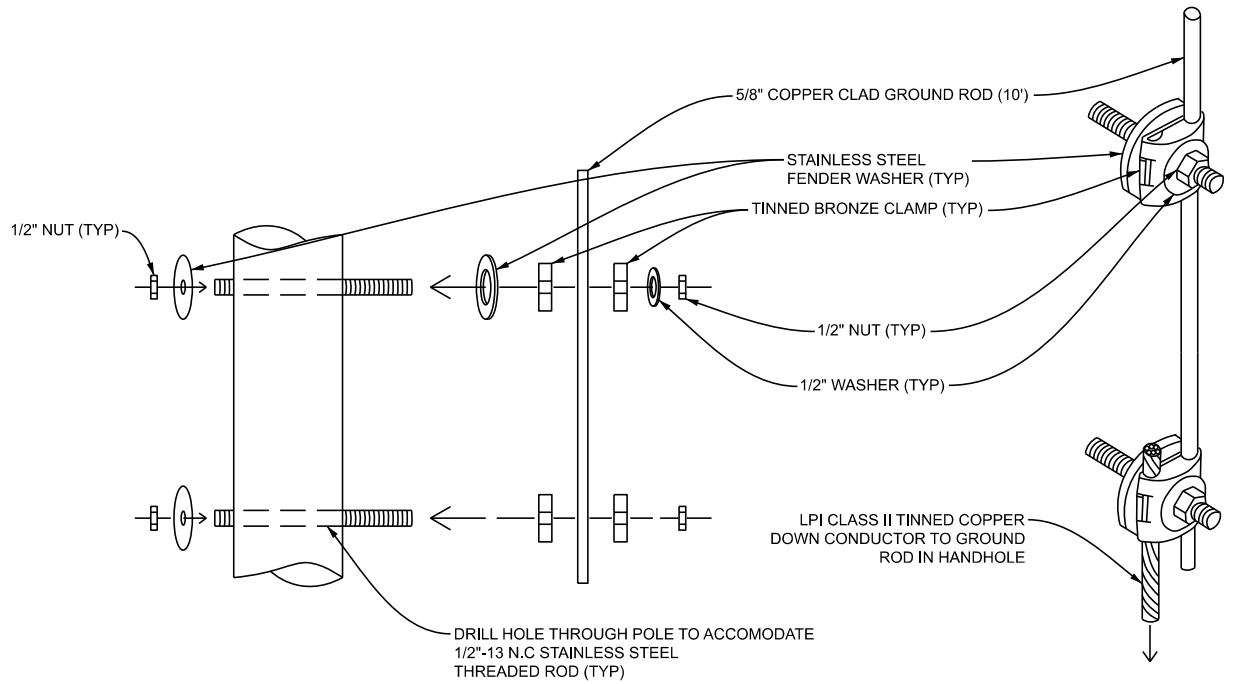
PROFILE VIEW
