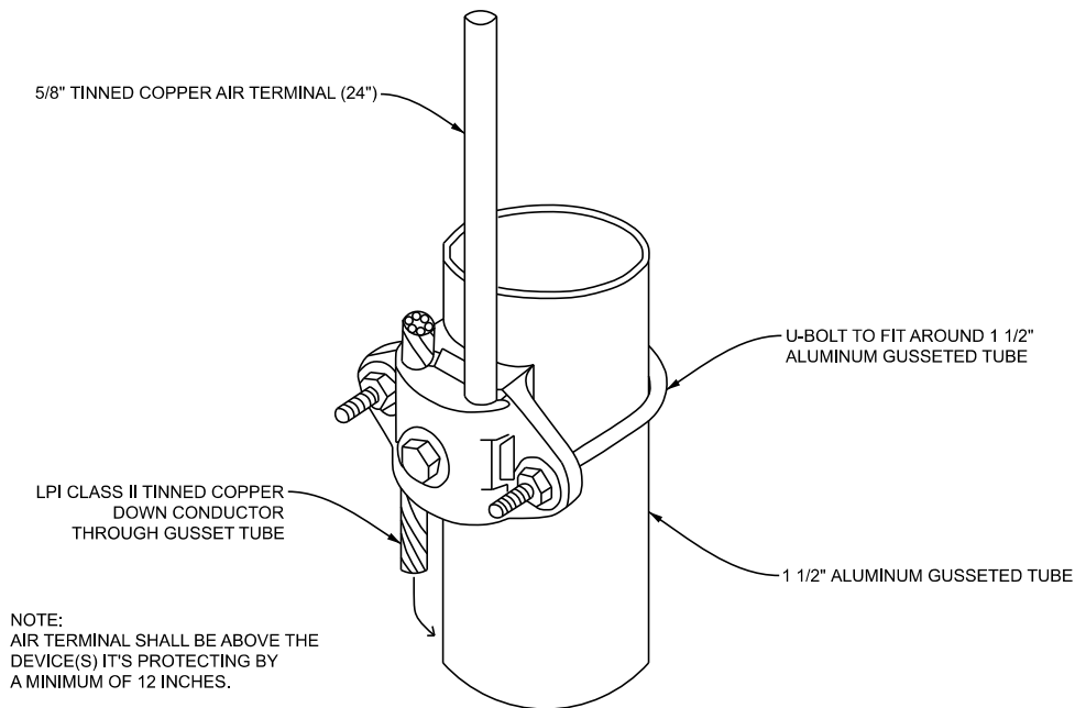
J DETAIL - LIGHTNING PROTECTION CLAMP ON ALUMINUM STEEL GUSSETED POLE N.T.S.
