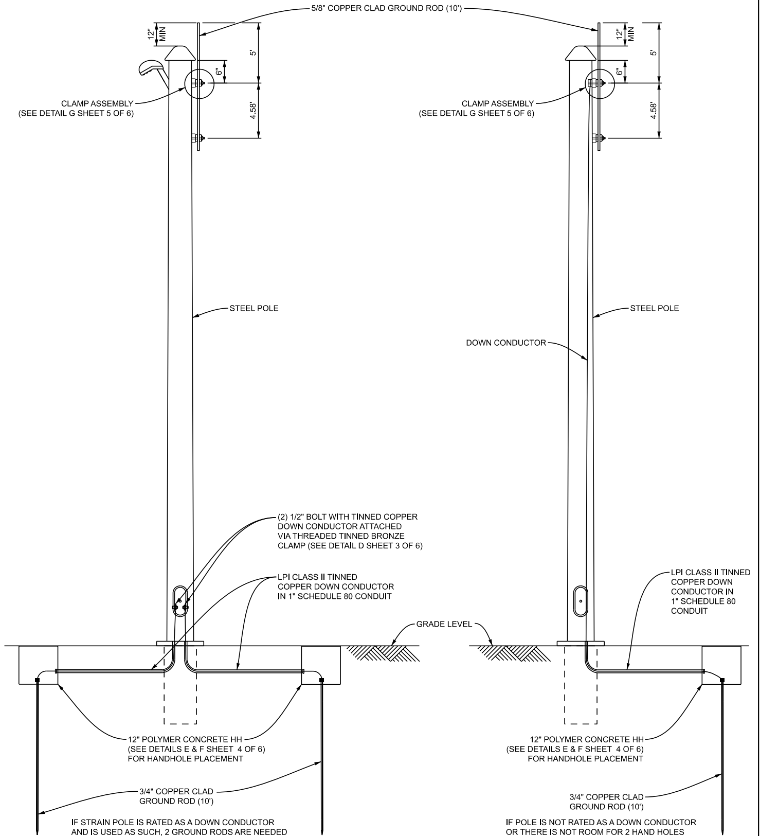
A DETAIL - LIGHTNING PROTECTION ON STEEL POLE N.T.S.
