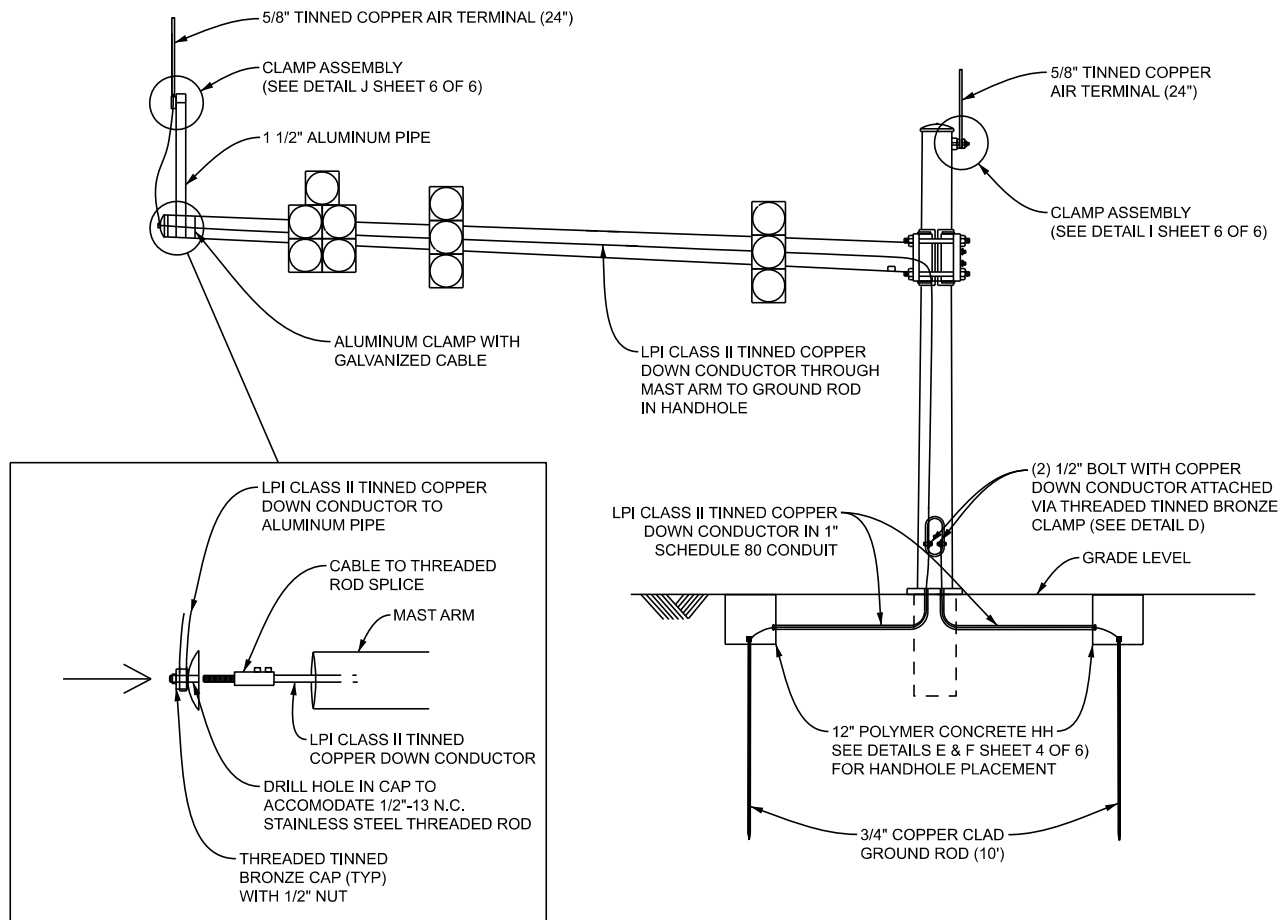
C DETAIL - LIGHTNING PROTECTION ON MAST ARM N.T.S.
