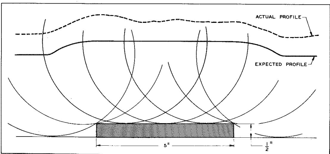
Figure 5. Profiling known waveforms.
