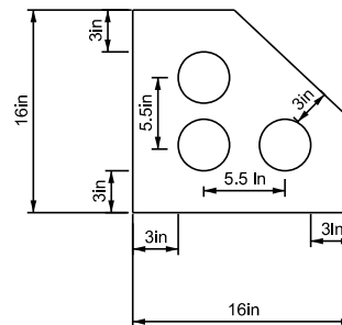
THREE 4" CONDUIT
