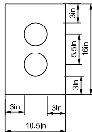
TWO 4" CONDUIT
