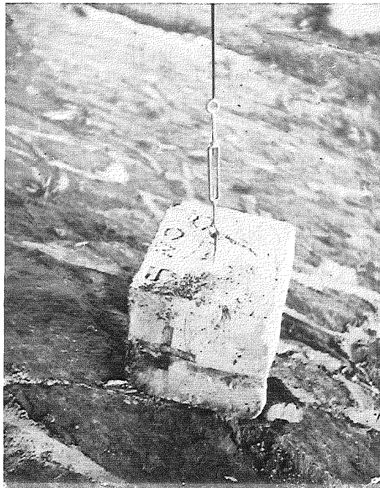
▲ FIGURE 2-DEFLECTOMETER USED TO MEASURE THE VIBRATION AND DEFLECTION AT THE CENTER OF THE SPAN
