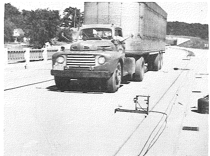
▲ FIGURE 5- A COMMERCIAL TEST TRUCK PASSING OVER THE BRIDGE
