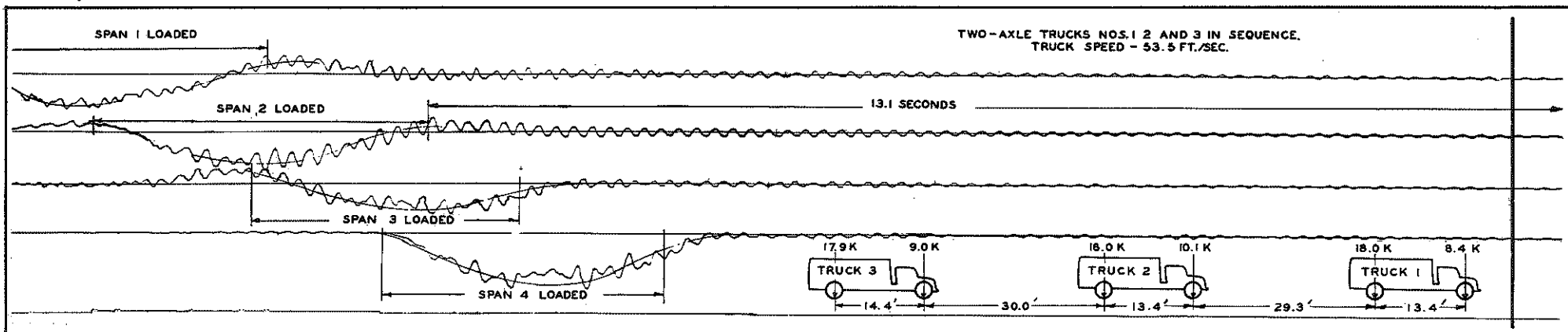
FIGURE 18- OSCILLOGRAPH TRACE SHOWING VIBRATION AND DEFLECTION OF SPANS 1 THROUGH 4 AS A RESULT OF THREE 2-AXLE TRUCKS PASSING OVER THE BRIDGE IN SEQUENCE.
