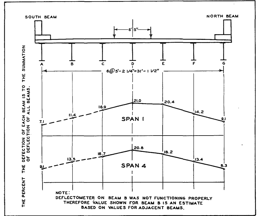
FIGURE 24- LATERAL DISTRIBUTION OF DEFLECTION (THREE-AXLE TEST TRUCK)
