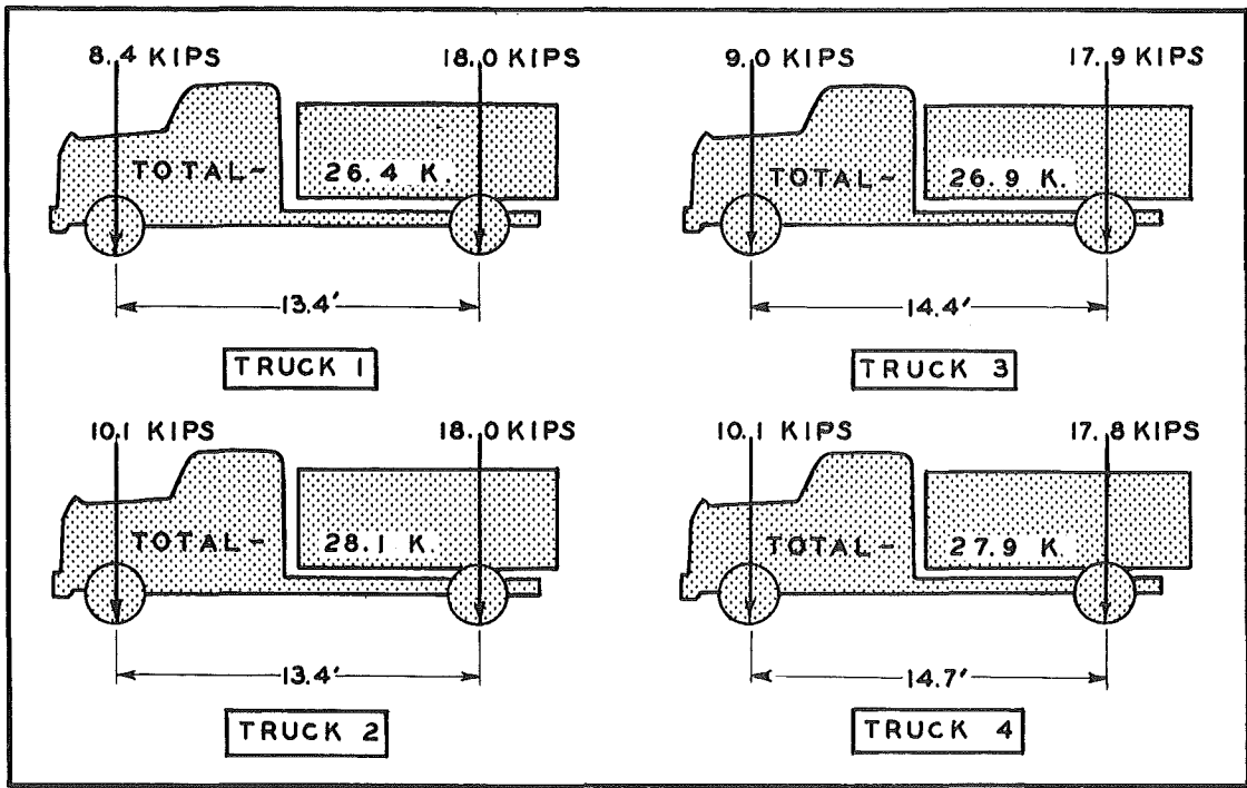
FIGURE 6- LOADING DIAGRAM OF FOUR COUNTY MAINTENANCE TRUCKS USED FOR CON- TROLLED LOADING TESTS ON FENVILLE BRIDGE.
