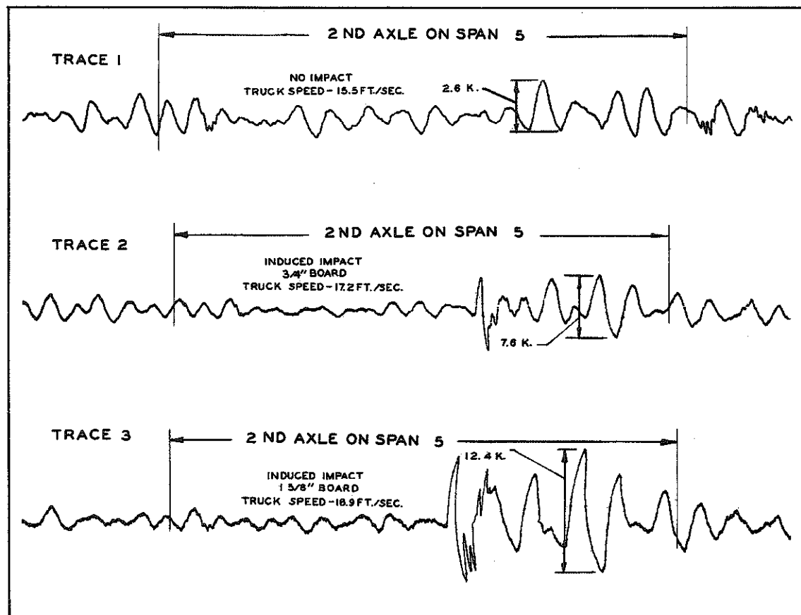
▲ NOTE: ALL THREE TRACES ARE NOT TO THE SAME SCALE FIGURE 17-BRUSH OSCILLOGRAPH TRACES SHOWING THE VARIATION IN EFFECTIVE AXLE LOAD WITH AND WITHOUT IMPACT (THREE-AXLE TRUCK)
