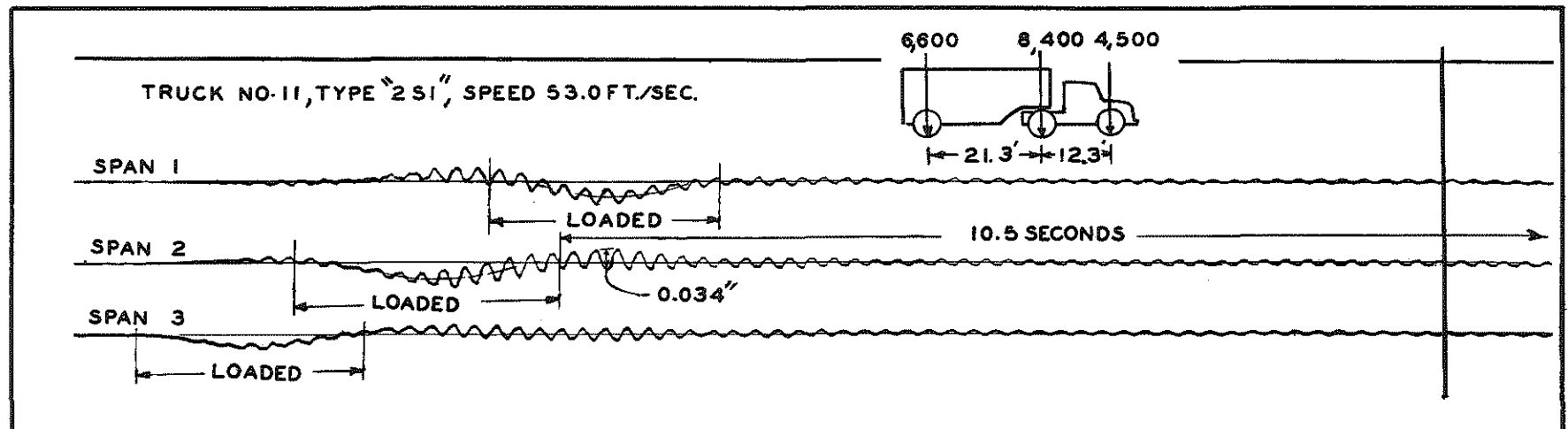
▲ FIGURE 11 - OSCILLOGRAPH TRACE SHOWING MAXIMUM AMPLITUDE OF VIBRATION - SPAN UNLOADED
