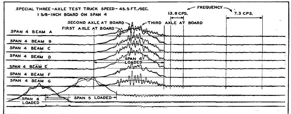
FIGURE 26- OSCILLOGRAPH TRACE ILLUSTRATING THE VIBRATION OF SPAN 4 AT TWO FREQUENCIES.
