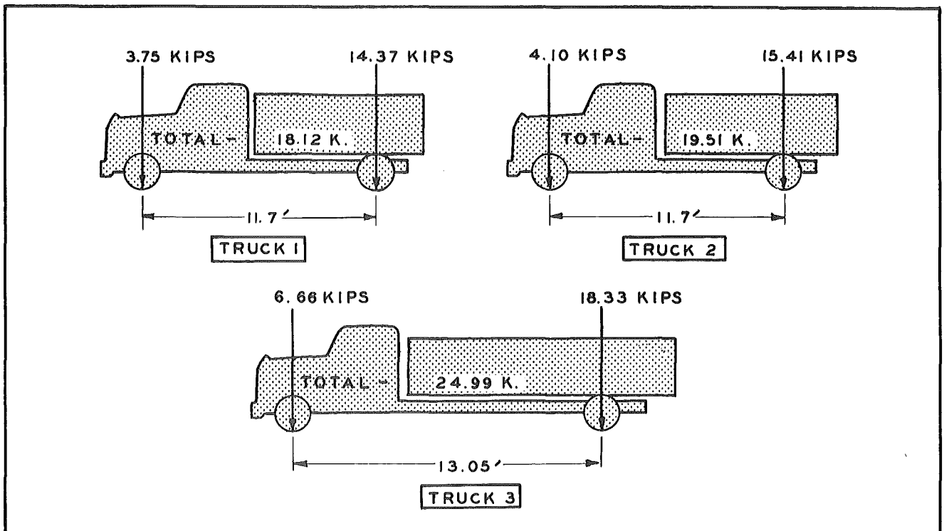
▲ FIGURE 22- LOADING DIAGRAM OF THREE COUNTY MAINTENANCE TRUCKS USED FOR CONTROLLED LOADING TESTS ON FENNVILLE BRIDGE.
