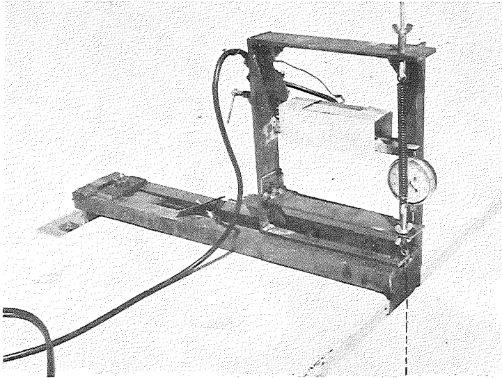
▲ FIGURE 2-DEFLECTOMETER USED TO MEASURE THE VIBRATION AND DEFLECTION AT THE CENTER OF THE SPAN
