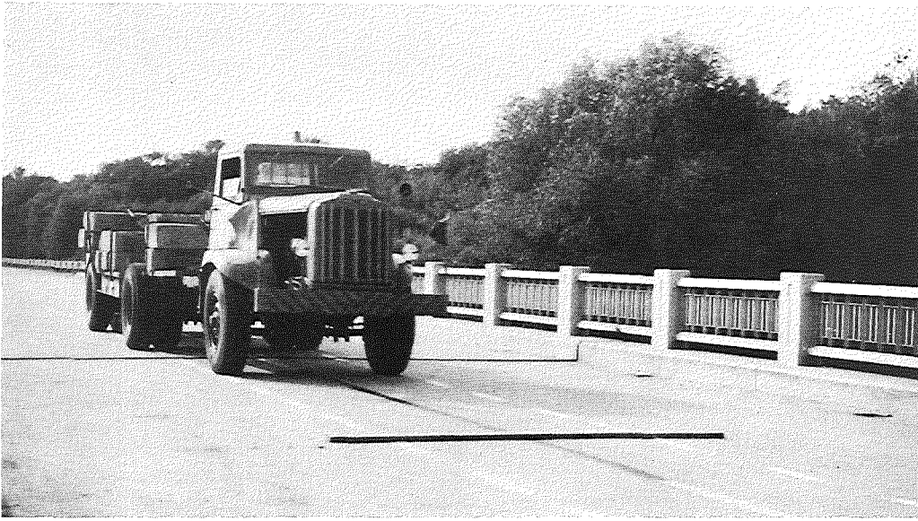
FIGURE 23- THREE-AXLE TEST TRUCK APPROACHING A 1 5/8-INCH BOARD PLACED ON THE SPAN TO CAUSE IMPACT.
