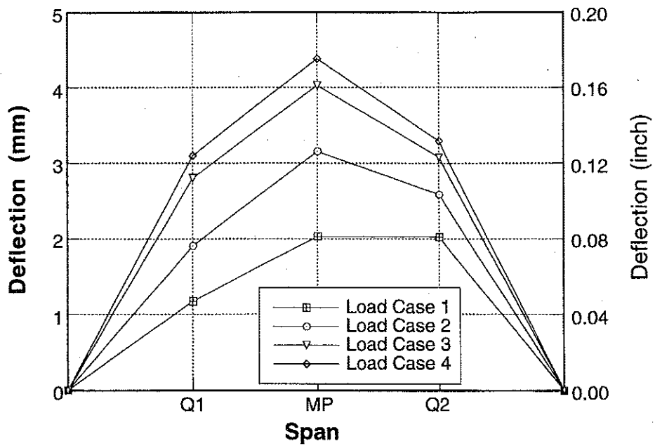
Figure A-37 Longitudinal Distribution of Deflections for Bridge No. 2, Girder 5 due to Upstream Loading.
