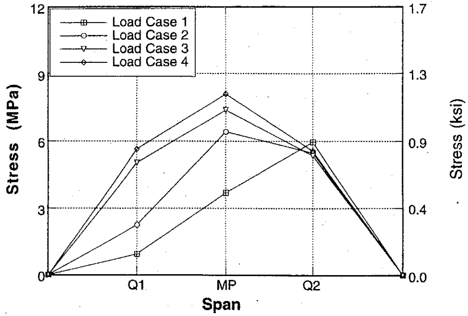
Figure A-55 : Longitudinal Distribution of Stresses for Bridge No. 2, Girder 2 due to Upstream Loading.
