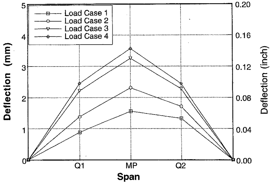
Figure A-35 : Longitudinal Distribution of Deflections for Bridge No. 2, Girder 5 due to Downstream Loading.
