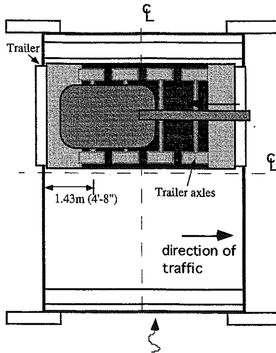
(b) Load Position 2 - Downstream.
