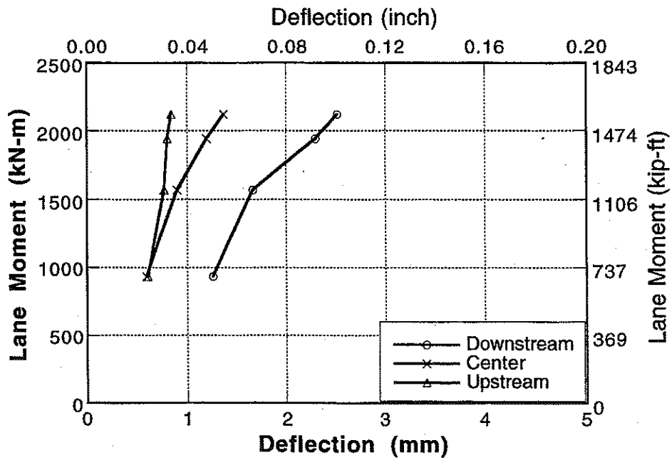
Figure A-19: Deflection vs Lane Moment for Bridge No. 2, Girder 8 and 9.
