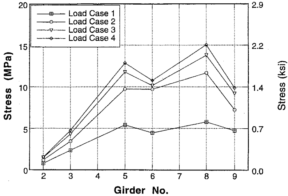
Figure A-50 : Girder Distribution of Stresses at Mid Point for Bridge No. 2 due to Downstream Loading.
