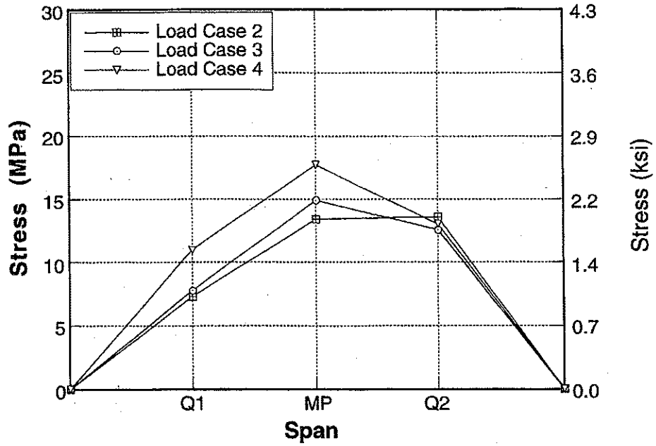
Figure A-80 : Longitudinal Distribution of Stresses for North Span of Bridge No. 3, Girder 5 due to Upstream Loading.
