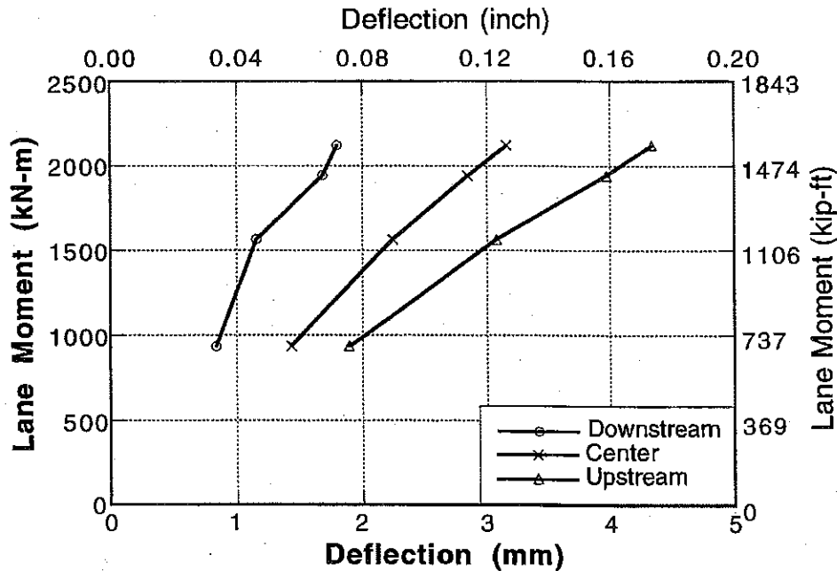
Figure 7-7 : Deflections at Mid-Span of Girder 3 of Bridge No. 2.
