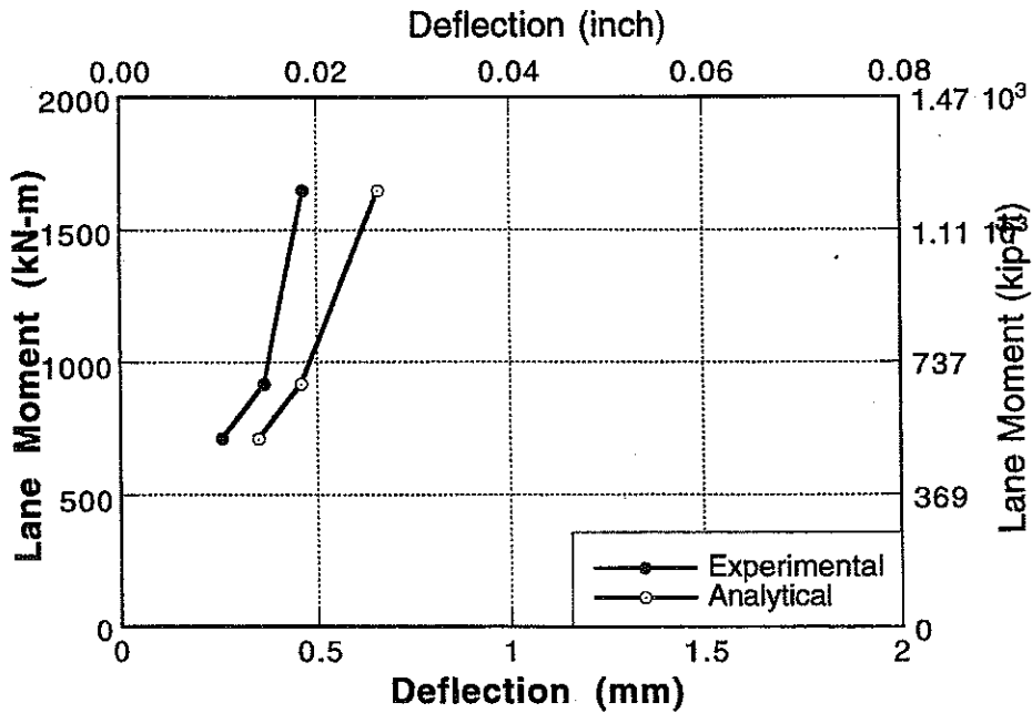
Figure A-183 : Experimental and Analytical Deflections for Bridge No. 5, Girder 5 and 6 for Lane 4 and 5 Loading.
