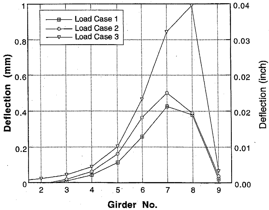
Figure 10-10 : Girder Distribution of Deflections for Loading in Lane 4 and 5.
