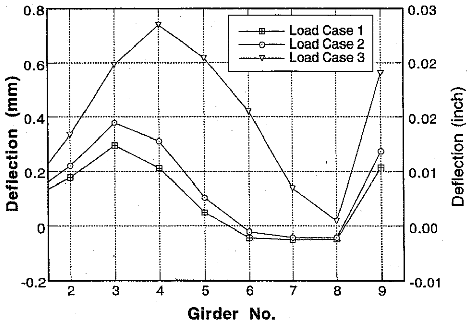
Figure A-187 : Girder Distribution of Deflections for Bridge No. 5 due to Loading in Lane 2 and 3.
