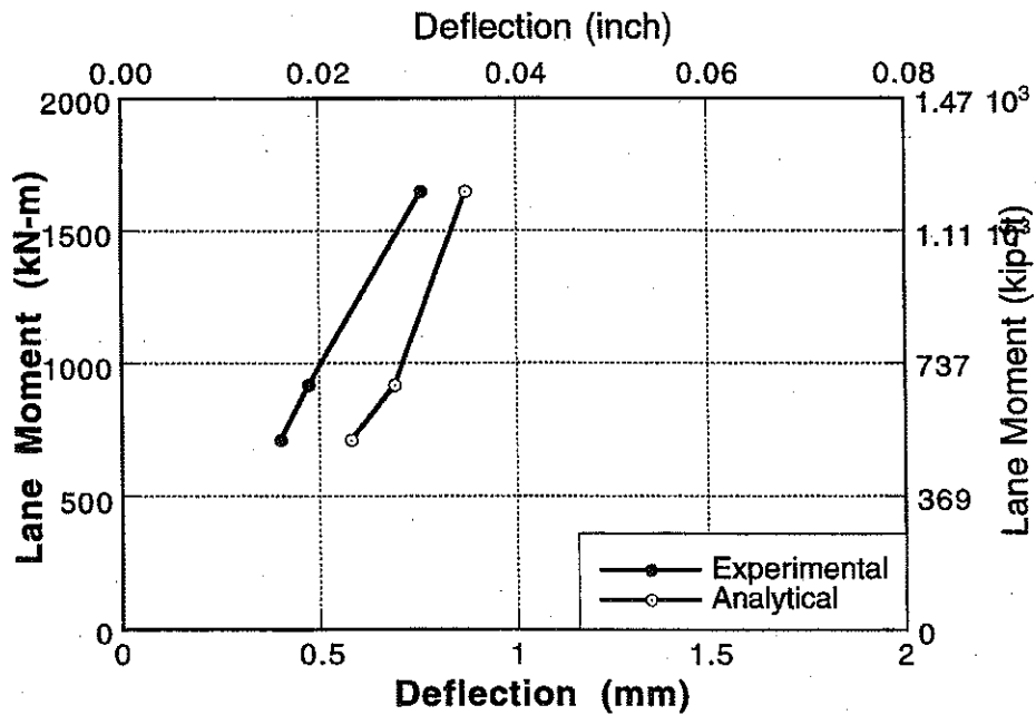
Figure A-166 : Experimental and Analytical Deflections for Bridge No. 5, Girder 1 and 2 for Lane 1 and 2 Loading.
