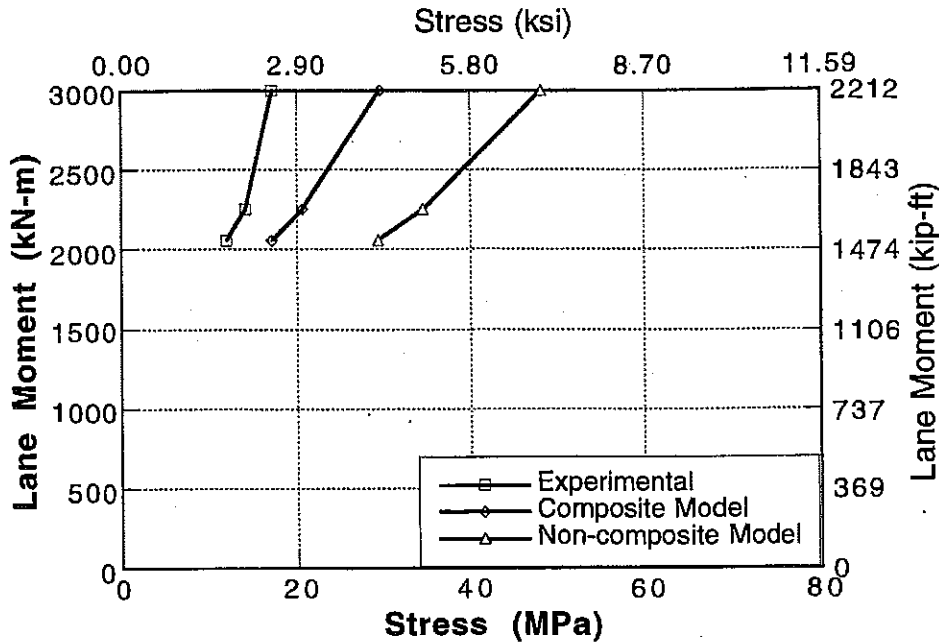
Figure 8-16 : Stress in Girder 6 for Downstream Loading on Bridge No. 3 - South Span.
