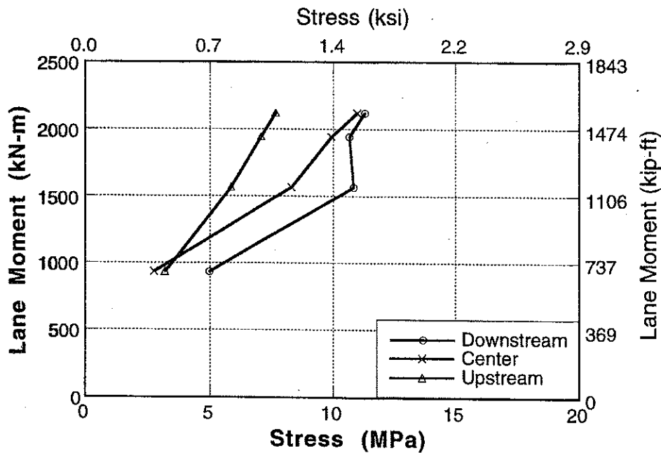
Figure A-39 : Stress vs Lane Moment for Bridge No. 2, Girder 5 and 6 at Mid Point.
