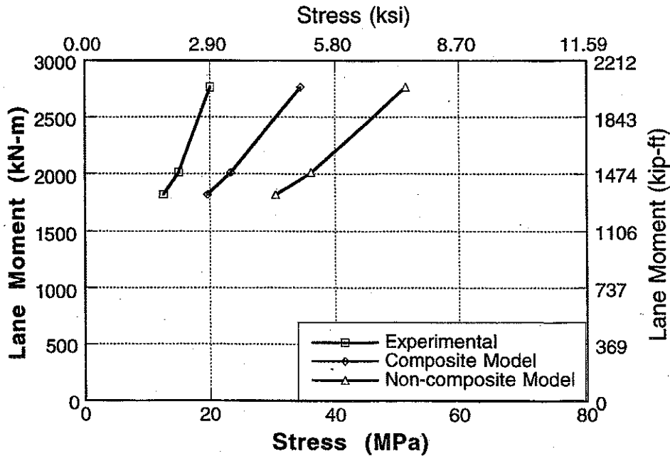
Figure A-68 : Experimental and Analytical Stresses for North Span of Bridge No. 3, Girder 4 and 5 for Center Loading.
