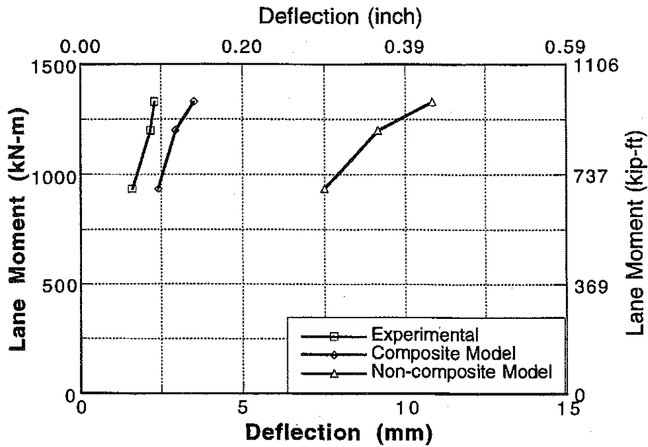
Figure 9-8 : Deflections at Mid-Span of Girder 5 for Center Loading on Bridge No. 4.
