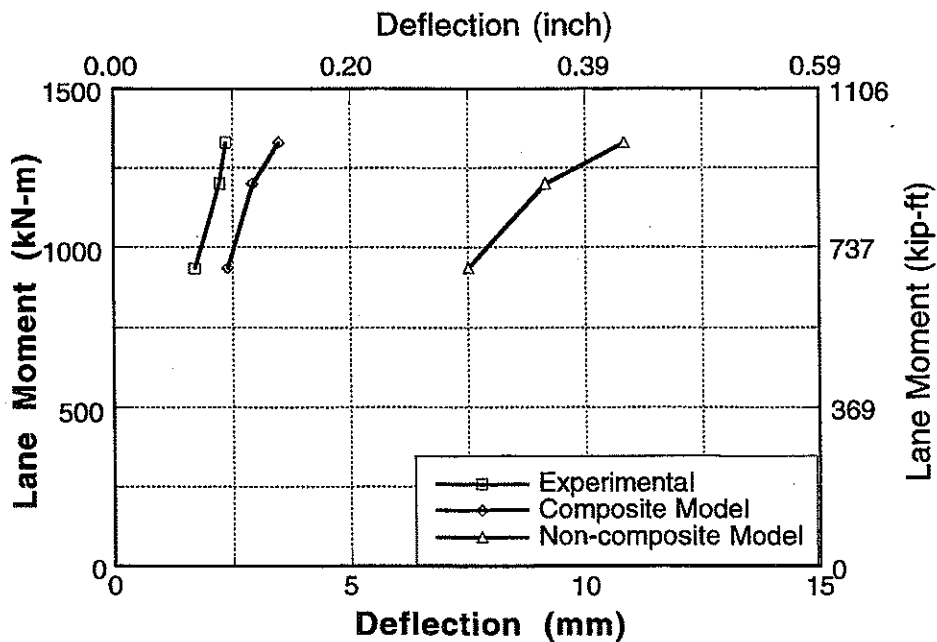
Figure A-118 : Experimental and Analytical Deflections for Bridge No. 4, Girder 5 and 6 for Center Loading.
