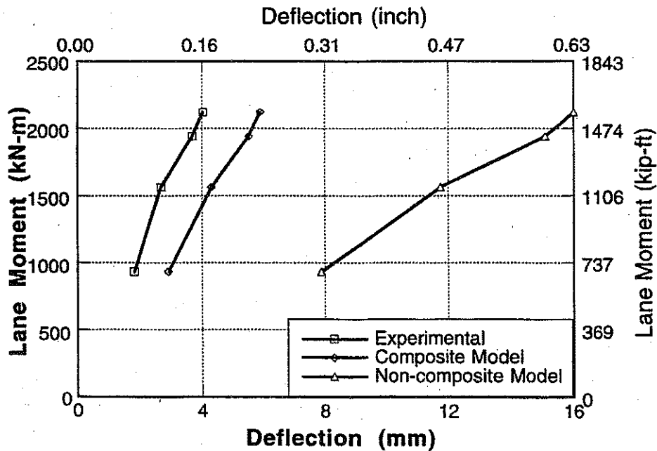
Figure A-22 : Experimental and Analytical Deflections for Bridge No. 2, Girder 6 and 7 for Downstream Loading.
