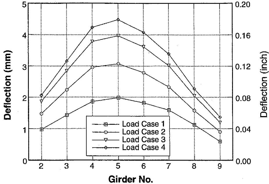
Figure 7-9 : Girder Distribution of Deflections due to Center Loading on Bridge No. 2.
