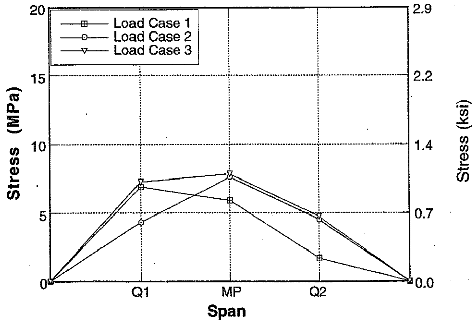
Figure A-155 : Longitudinal Distribution of Stresses for Bridge No. 4, Girder 6 due to Downstream Loading.
