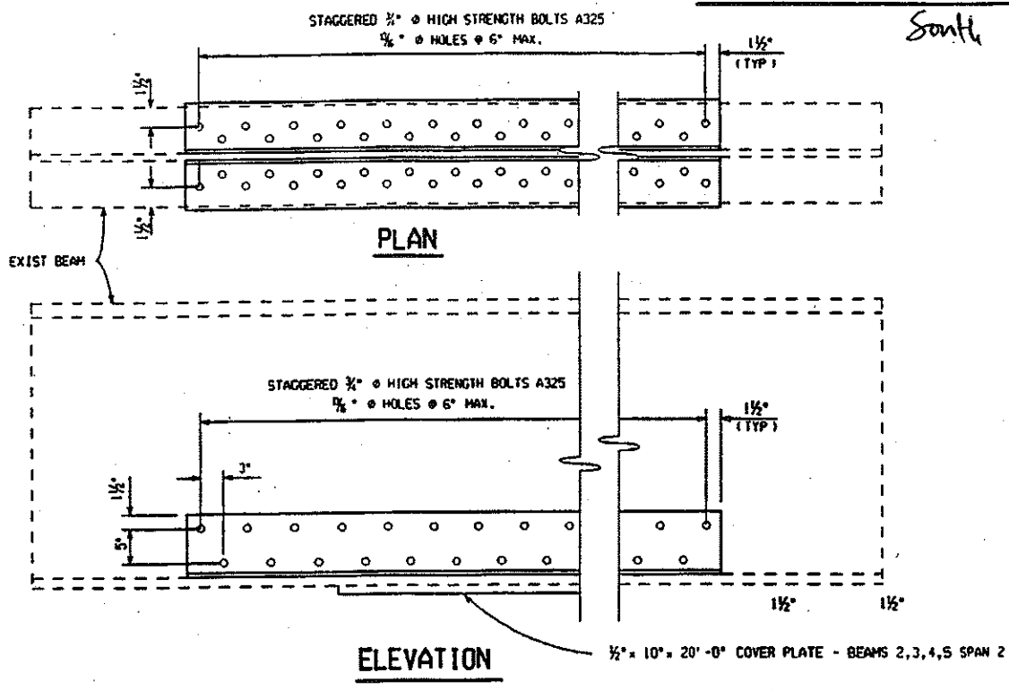
BEAM REPAIR LOCATION DIAGRAM
