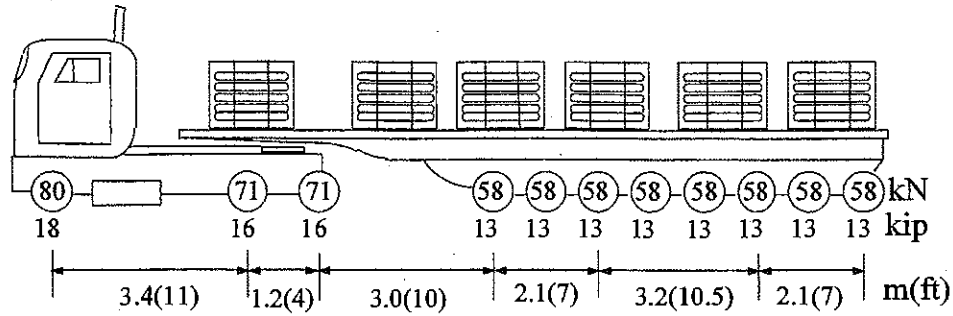
Figure 3-1 : 11-Axle Two-Unit Truck.
