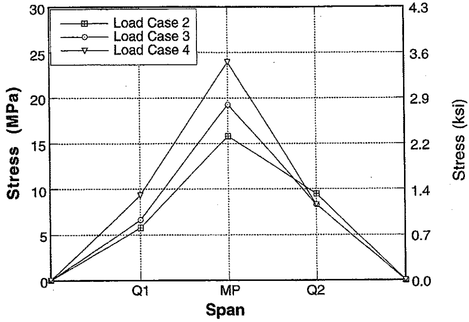
Figure A-105 : Longitudinal Distribution of Stresses for South Span of Bridge No. 3, Girder 5 due to Upstream Loading.
