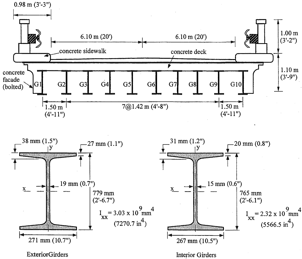
Figure 8-2 : Cross-Section of Bridge No. 3.
