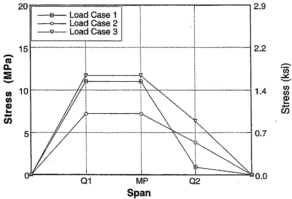
Figure A-153 : Longitudinal Distribution of Stresses for Bridge No. 4, Girder 5 due to Center Loading.
