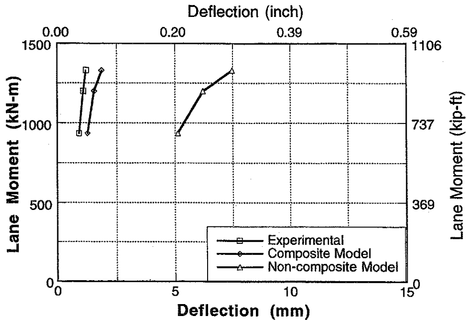
Figure A-119 : Experimental and Analytical Deflections for Bridge No. 4, Girder 7 and 8 for Center Loading.
