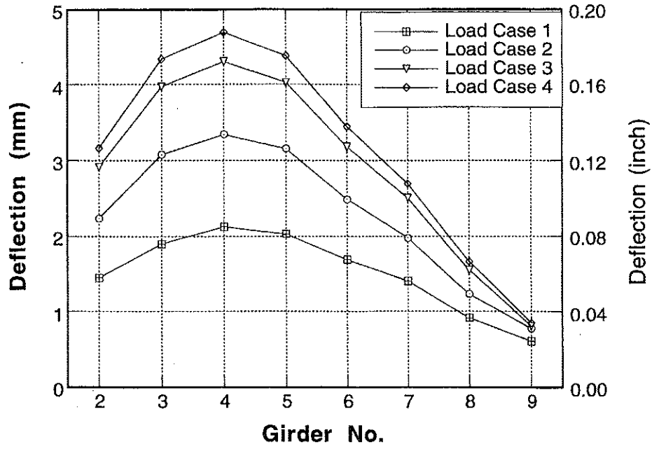
Figure A-34 : Girder Distribution of Deflections for Bridge No. 2 due to Upstream Loading.
