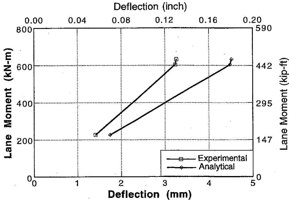
Figure 6-8 : Deflections at Mid-Span of Girder 4 for center loading on Bridge No. 1.
