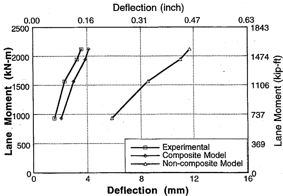
Figure A-21 : Experimental and Analytical Deflections for Bridge No. 2, Girder 4 and 5 for Downstream Loading.
