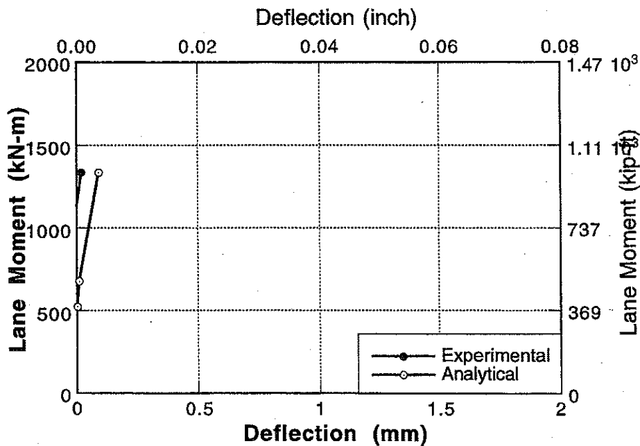
Figure A-174 : Experimental and Analytical Deflections for Bridge No. 5, Girder 7 and 8 for Lane 2 and 3 Loading.
