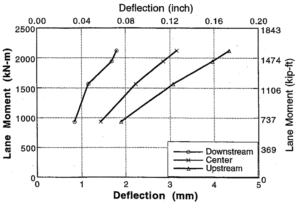
Figure A-16: Deflection vs Lane Moment for Bridge No. 2, Girder 2 and 3.
