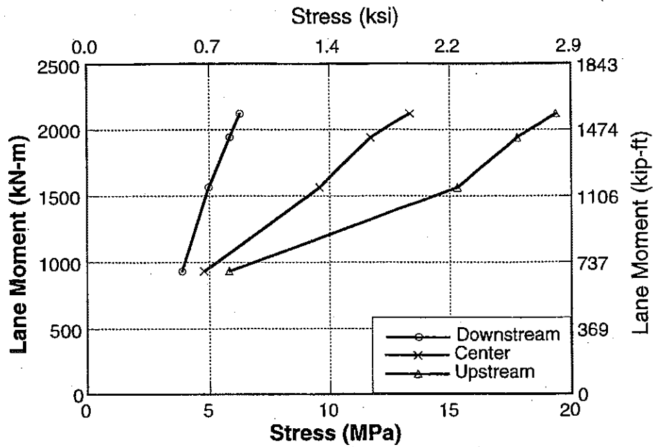
Figure 7-10 : Stresses at Mid-Span of Girder 3 of Bridge No. 2.
