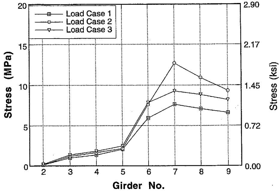
Figure A-146 : Girder Distribution of Stresses at Mid Point for Bridge No. 4 due to Downstream Loading.
