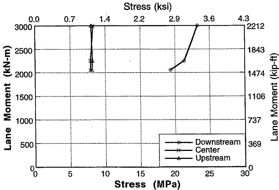
Figure A-87 : Stress vs Lane Moment for South Span of Bridge No. 3, Girder 8 and 9 at Mid Point.
