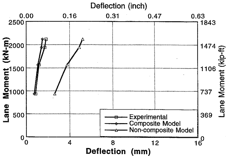
Figure A-20 : Experimental and Analytical Deflections for Bridge No. 2, Girder 2 and 3 for Downstream Loading.
