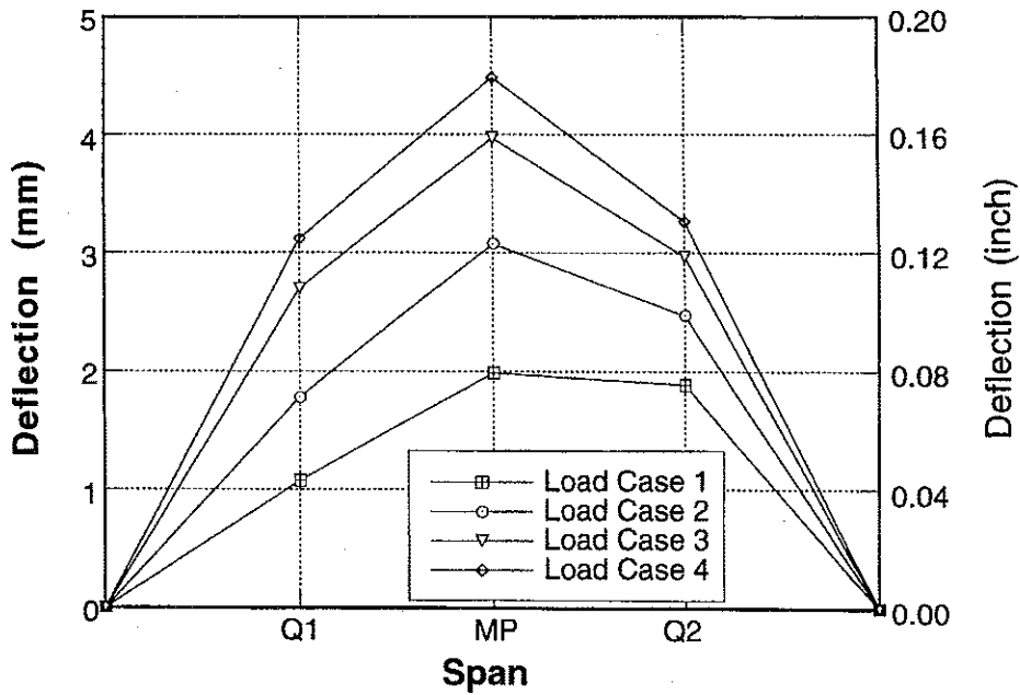
Figure A-36 : Longitudinal Distribution of Deflections for Bridge No. 2, Girder 5 due to Center Loading.
