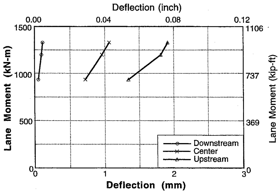
Figure A-109: Deflection vs Lane Moment for Bridge No. 4, Girder 2 and 3.
