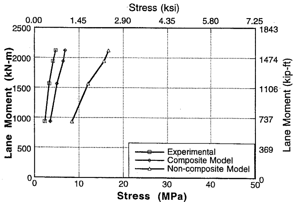
Figure A-46 : Experimental and Analytical Stresses for Bridge No. 2, Girder 8 and 9 for Center Loading.
