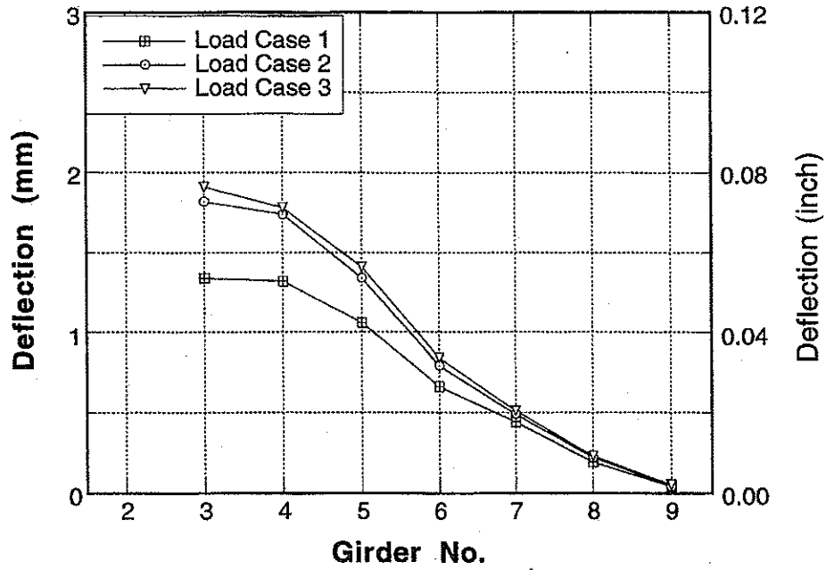
Figure A-127 : Girder Distribution of Deflections for Bridge No. 4 due to Upstream Loading.
