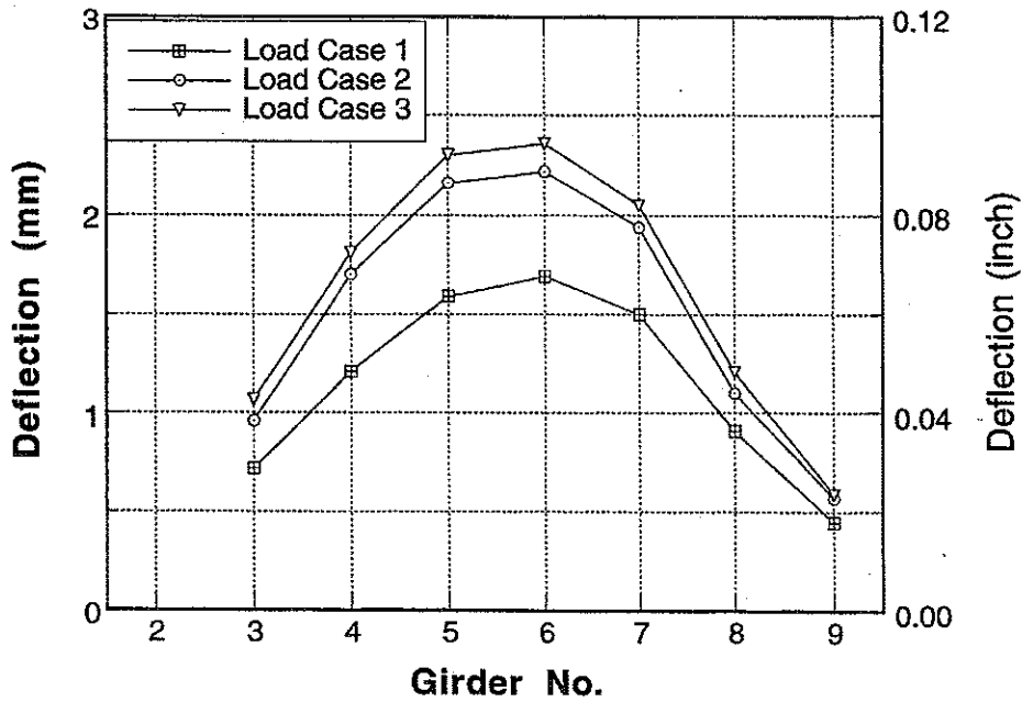
Figure A-126 : Girder Distribution of Deflections for Bridge No. 4 due to Center Loading.
