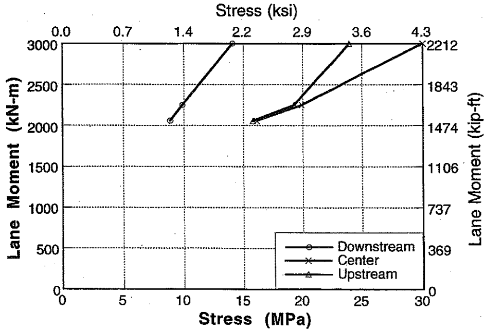
Figure A-85 : Stress vs Lane Moment for South Span of Bridge No. 3, Girder 4 and 5 at Mid Point..
