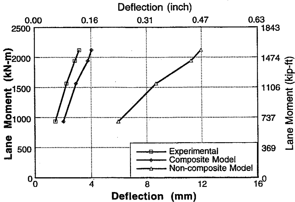
Figure A-24 : Experimental and Analytical Deflections for Bridge No. 2, Girder 2 and 3 for Center Loading.
