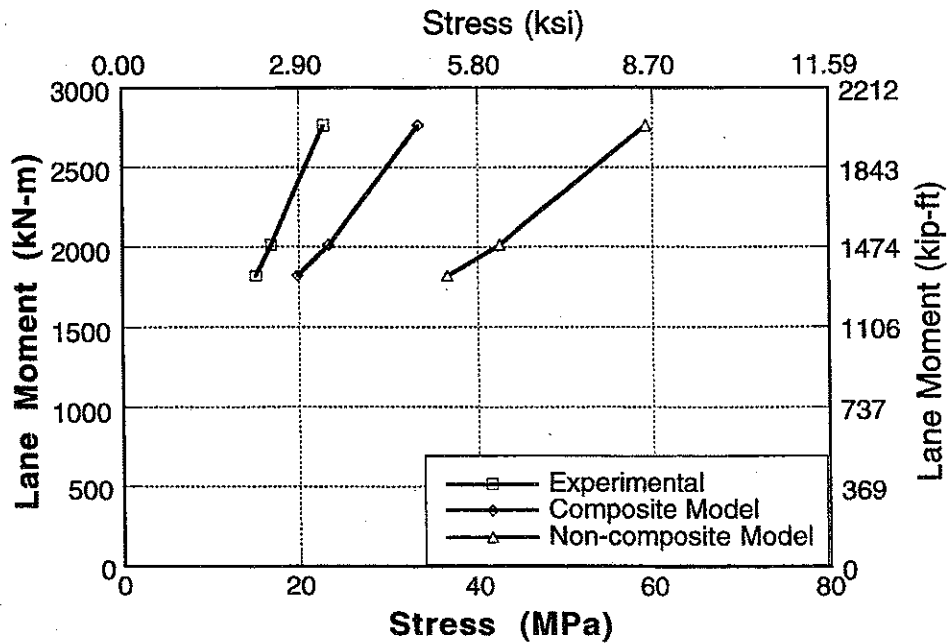
Figure A-71 : Experimental and Analytical Stresses for North Span of Bridge No. 3, Girder 2 and 3 for Upstream Loading.
