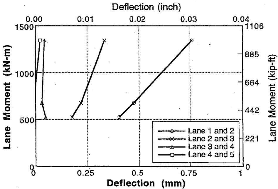
Figure A-161 : Deflection vs Lane Moment for Bridge No. 5, Girder 1 and 2.
