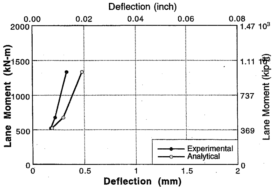
Figure A-171 : Experimental and Analytical Deflections for Bridge No. 5, Girder 1 and 2 for Lane 2 and 3 Loading.
