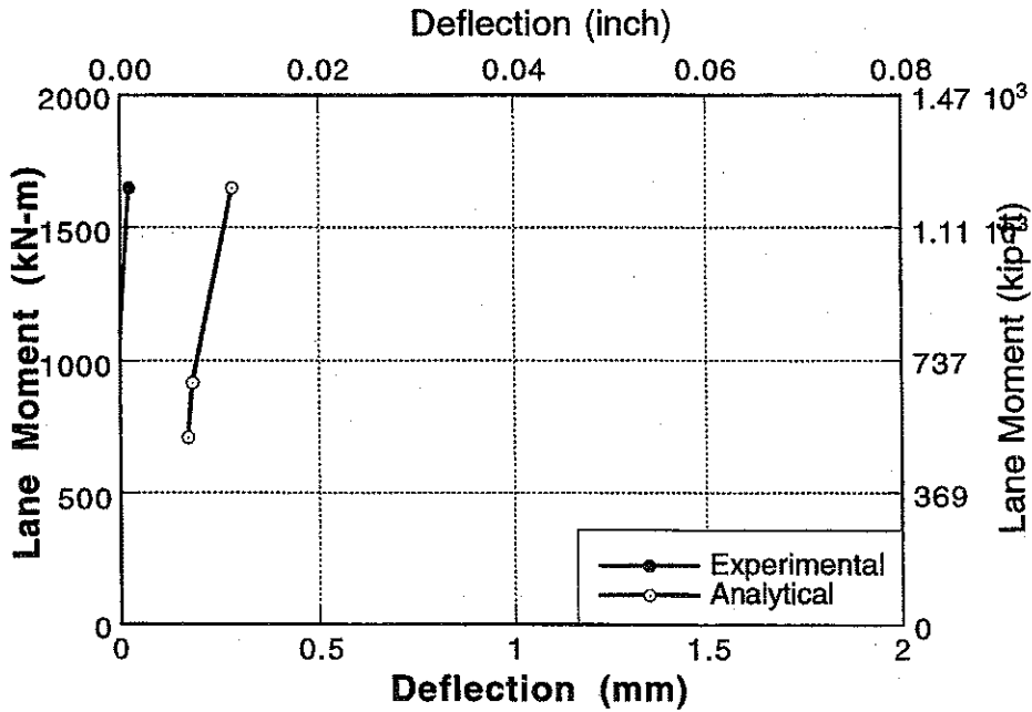
Figure A-181 : Experimental and Analytical Deflections for Bridge No. 5, Girder 1 and 2 for Lane 4 and 5 Loading.
