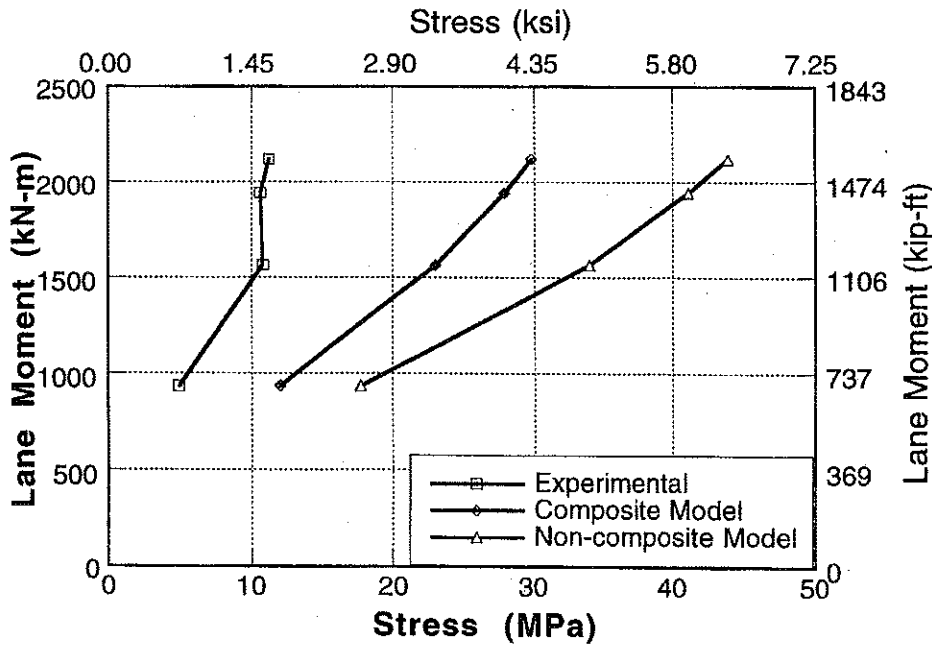
Figure A-42 : Experimental and Analytical Stresses for Bridge No. 2, Girder 5 and 6 for Downstream Loading.
