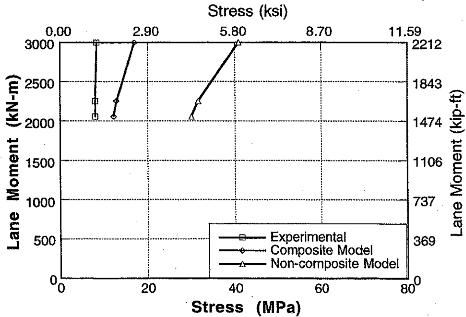
Figure A-95 : Experimental and Analytical Stresses for South Span of Bridge No. 3, Girder 8 and 9 for Center Loading.
