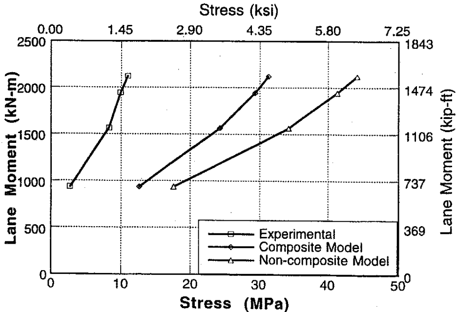
Figure A-45 : Experimental and Analytical Stresses for Bridge No. 2, Girder 5 and 6 for Center Loading.
