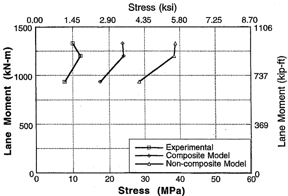
Figure A-140 : Experimental and Analytical Stresses for Bridge No. 4, Girder 6 and 7 for Center Loading.
