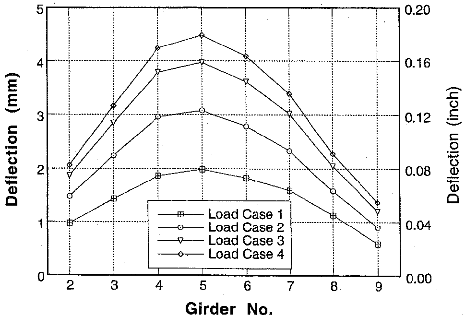
Figure A-33 : Girder Distribution of Deflections for Bridge No. 2 due to Center Loading.
