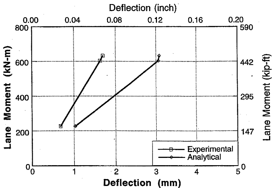
Figure A-10 : Experimental and Analytical Deflections for Bridge No. 1, Girder 1 and 2 for Upstream Loading.
