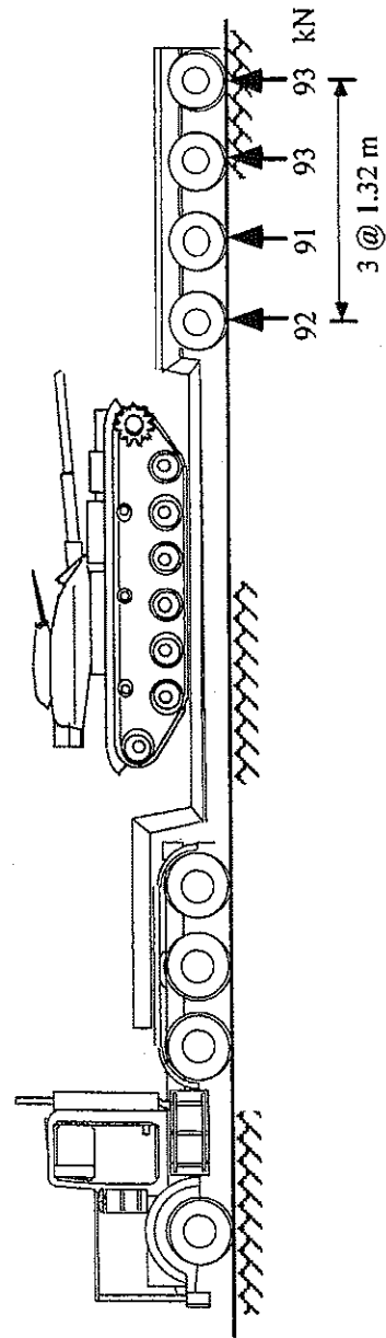
Figure 3-6 : Tank on Commercial Trailer.
