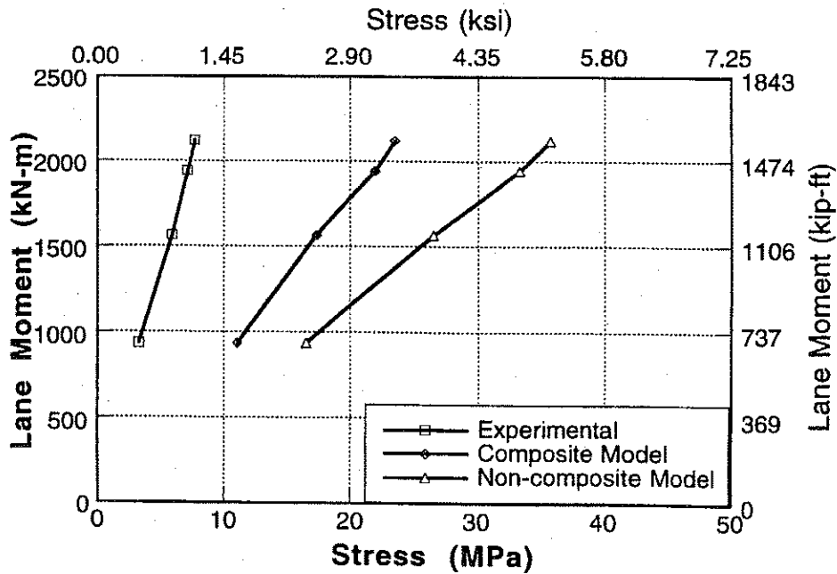
Figure A-48 : Experimental and Analytical Stresses for Bridge No. 2, Girder 5 and 6 for Upstream Loading.
