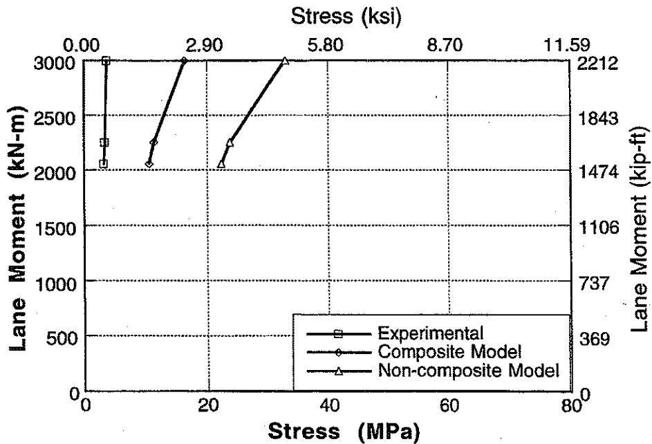
Figure A-98 : Experimental and Analytical Stresses for South Span of Bridge No. 3, Girder 6 and 7 for Upstream Loading.
