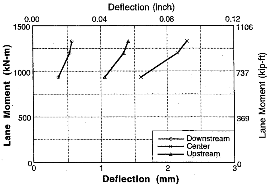
Figure A-110: Deflection vs Lane Moment for Bridge No. 4, Girder 4 and 5.
