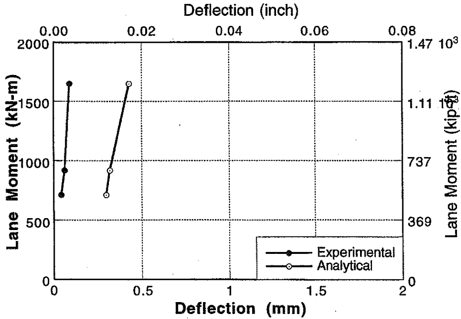
Figure A-182 : Experimental and Analytical Deflections for Bridge No. 5, Girder 3 and 4 for Lane 4 and 5 Loading.
