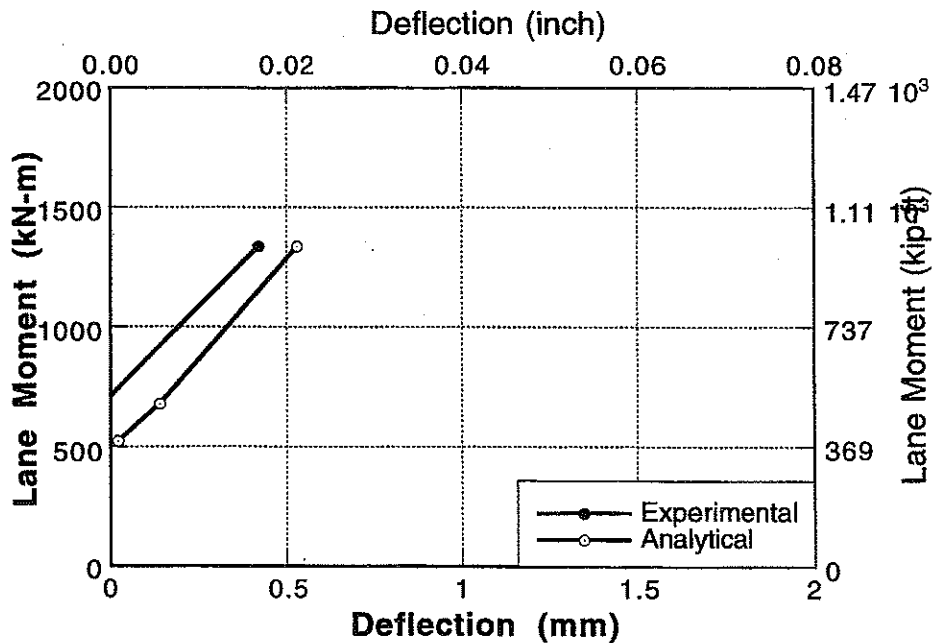
Figure A-173 : Experimental and Analytical Deflections for Bridge No. 5, Girder 5 and 6 for Lane 2 and 3 Loading.
