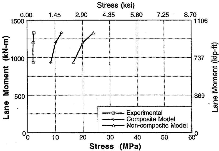
Figure A-135 : Experimental and Analytical Stresses for Bridge No. 4, Girder 4 and 5 for Downstream Loading.
