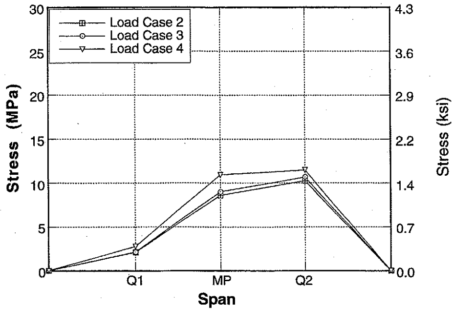
Figure A-108 : Longitudinal Distribution of Stresses for South Span of Bridge No. 3, Girder 6 due to Upstream Loading.
