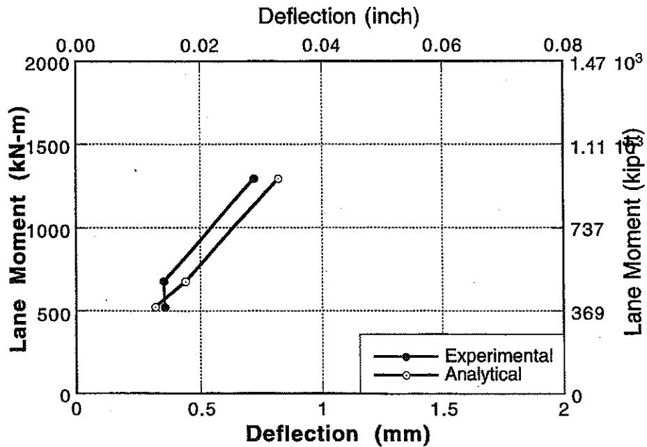
Figure A-178 : Experimental and Analytical Deflections for Bridge No. 5, Girder 5 and 6 for Lane 3 and 4 Loading.
