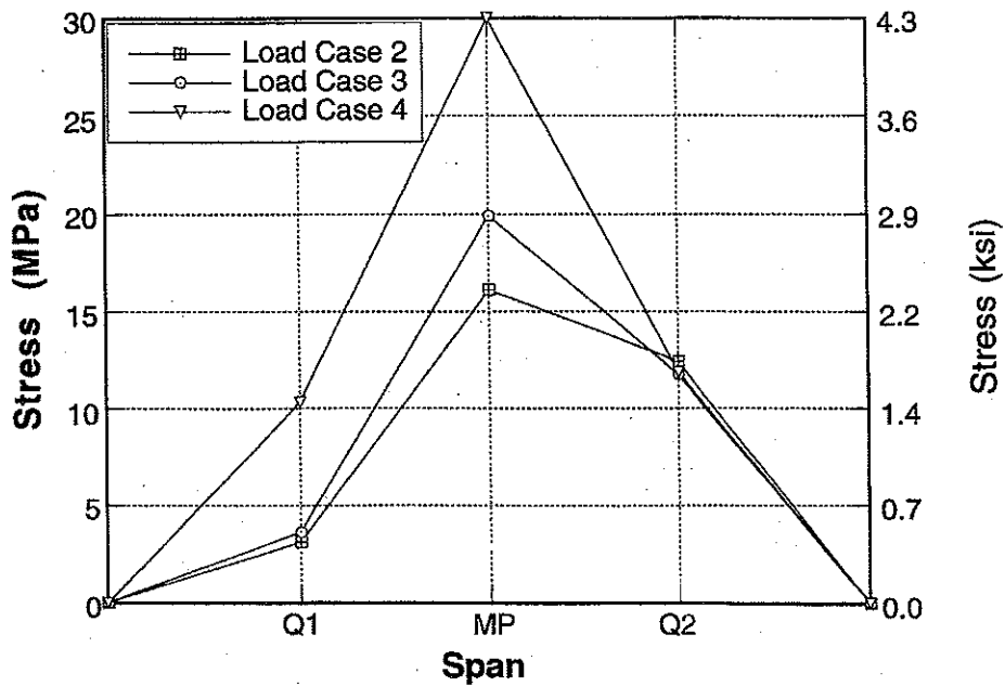
Figure A-104 : Longitudinal Distribution of Stresses for South Span of Bridge No. 3, Girder 5 due to Center Loading.
