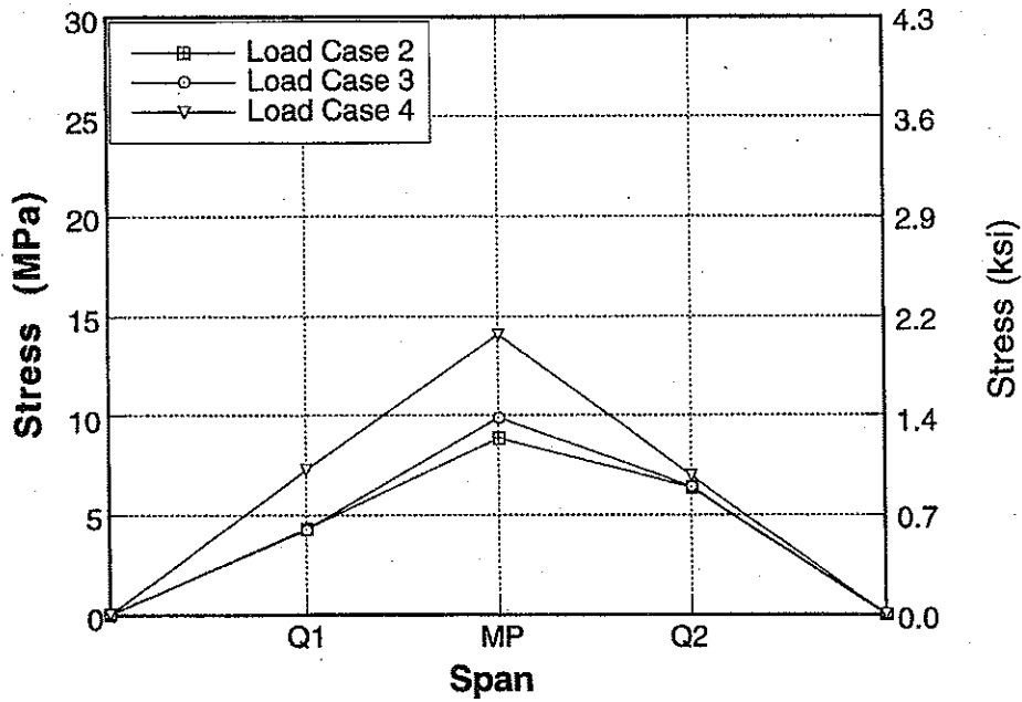
Figure A-103 : Longitudinal Distribution of Stresses for South Span of Bridge No. 3, Girder 5 due to Downstream Loading.
