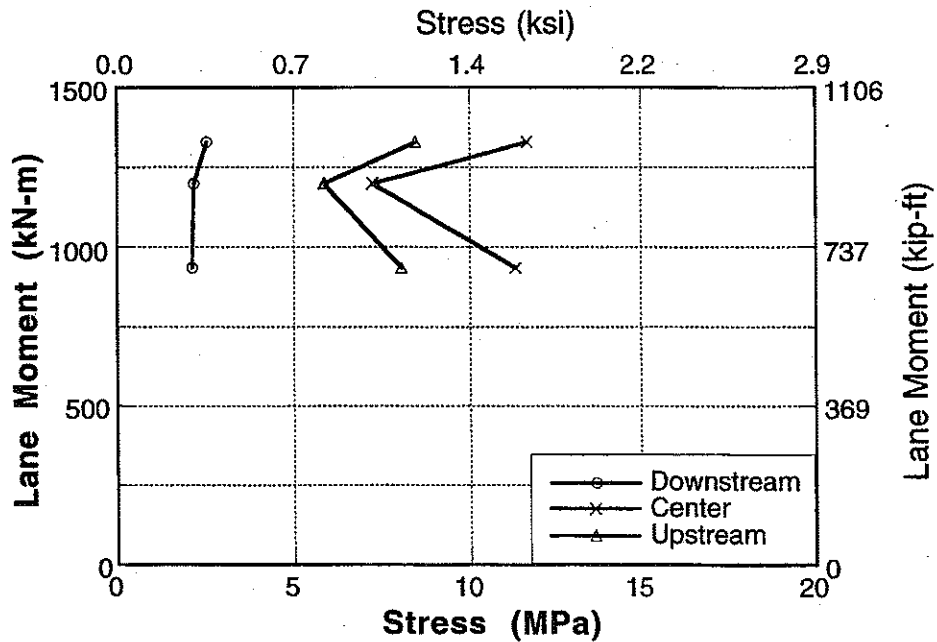
Figure A-132 : Stress vs Lane Moment for Bridge No. 4, Girder 4 and 5 at Mid Point.
