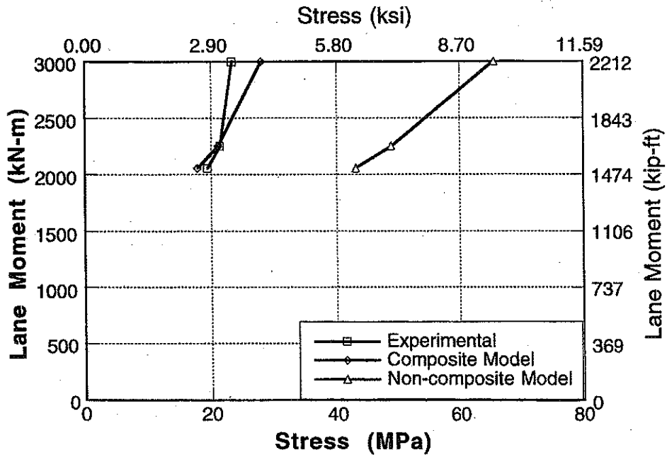
Figure A-91 : Experimental and Analytical Stresses for South Span of Bridge No. 3, Girder 8 and 9 for Downstream Loading.
