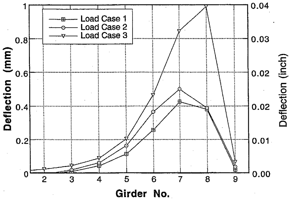
Figure A-189 : Girder Distribution of Deflections for Bridge No. 5 due to Loading in Lane 4 and 5.
