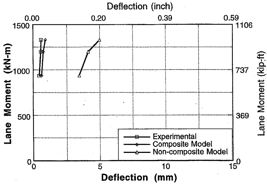
Figure A-120 : Experimental and Analytical Deflections for Bridge No. 4, 9 for Center Loading.
