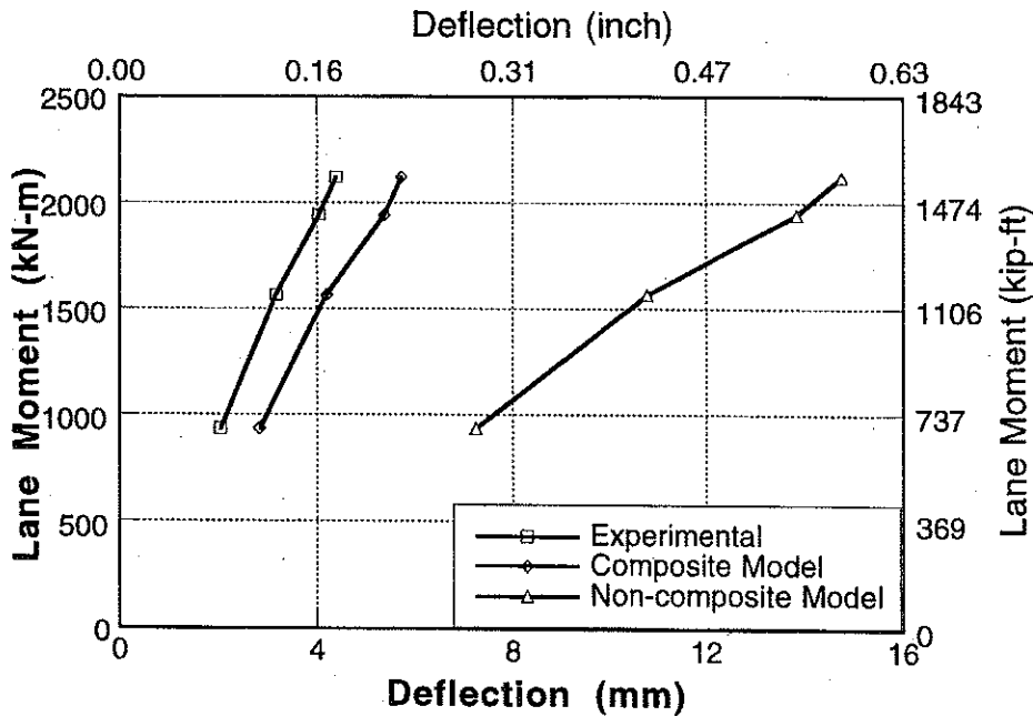
Figure A-29 : Experimental and Analytical Deflections for Bridge No. 2, Girder 4 and 5 for Upstream Loading.
