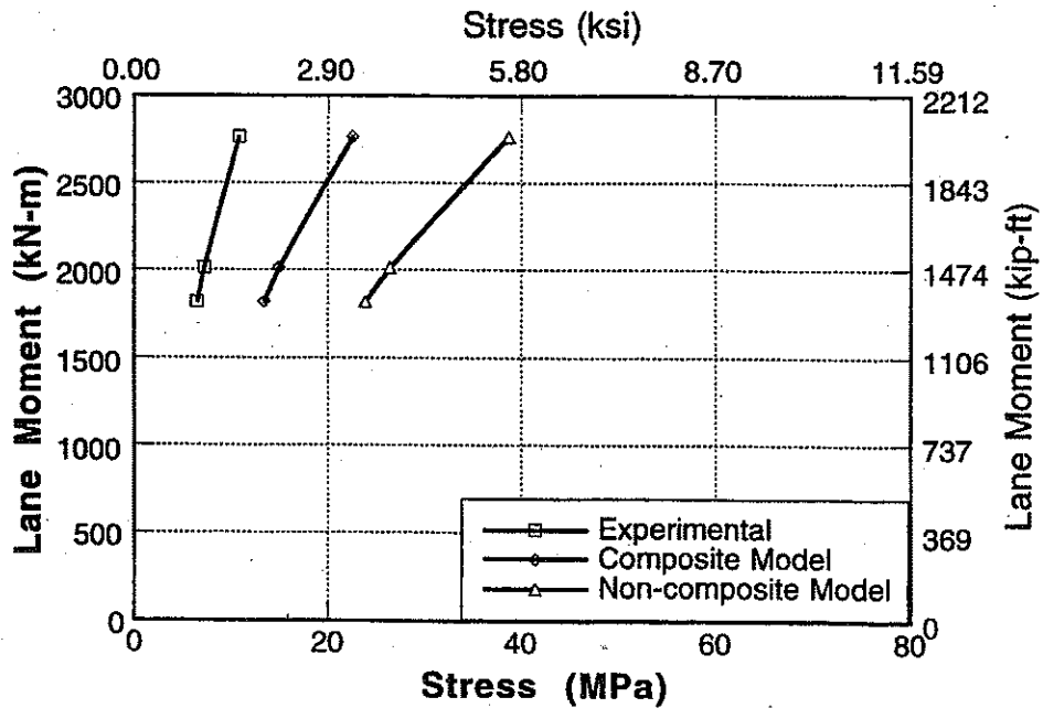
Figure A-64 : Experimental and Analytical Stresses for North Span of Bridge No. 3, Girder 4 and 5 for Downstream Loading.
