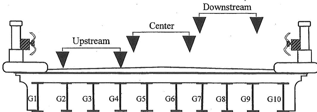
Figure 3-8 : Transverse Load Positions for Bridge No. 2 (others were similar).
