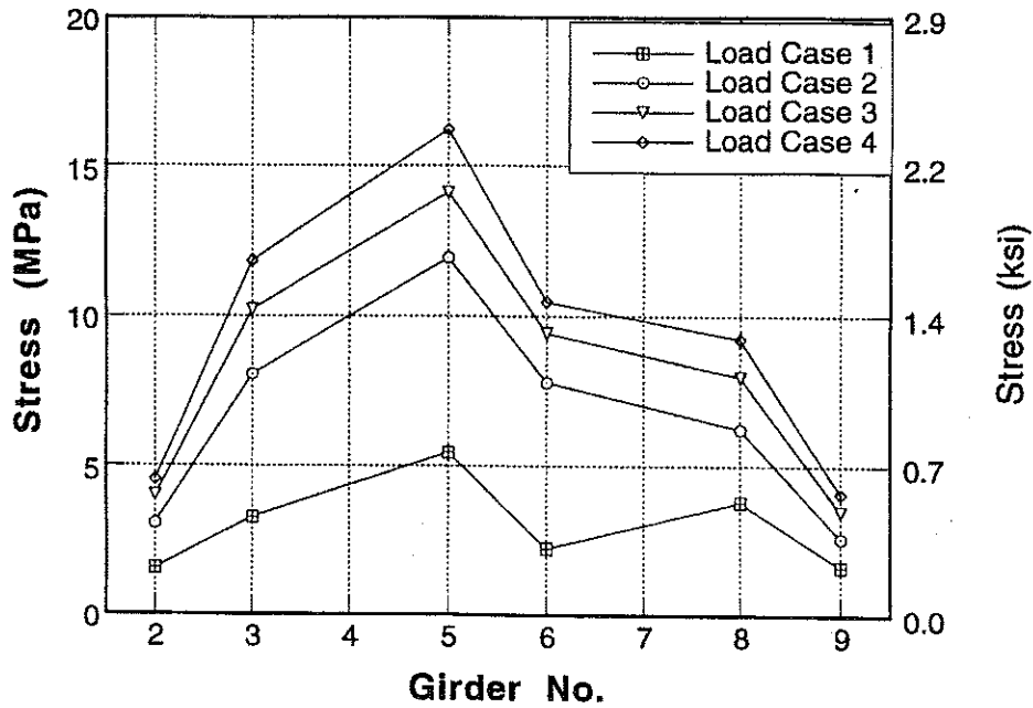
Figure A-51 : Girder Distribution of Stresses at Mid Point for Bridge No. 2 due to Center Loading.
