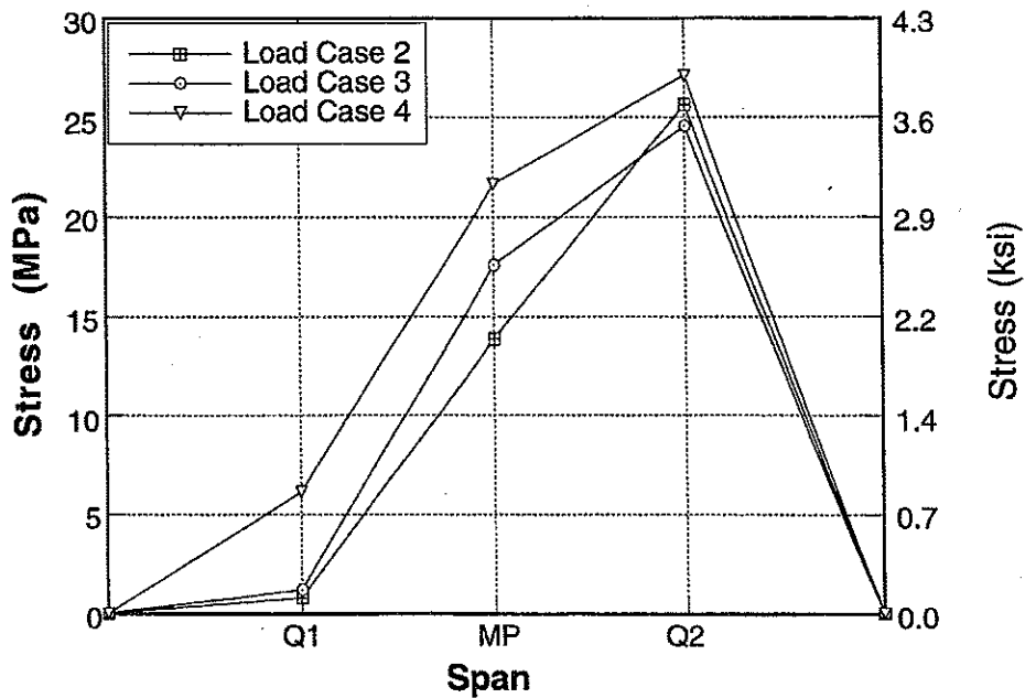
Figure A-107 : Longitudinal Distribution of Stresses for South Span of Bridge No. 3, Girder 6 due to Center Loading.
