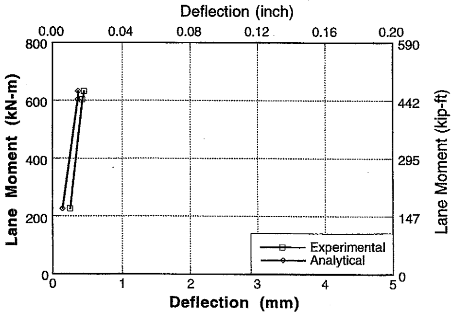
Figure A-4 : Experimental and Analytical Deflections for Bridge No. 1, Girder 1 and 2 for Downstream Loading.
