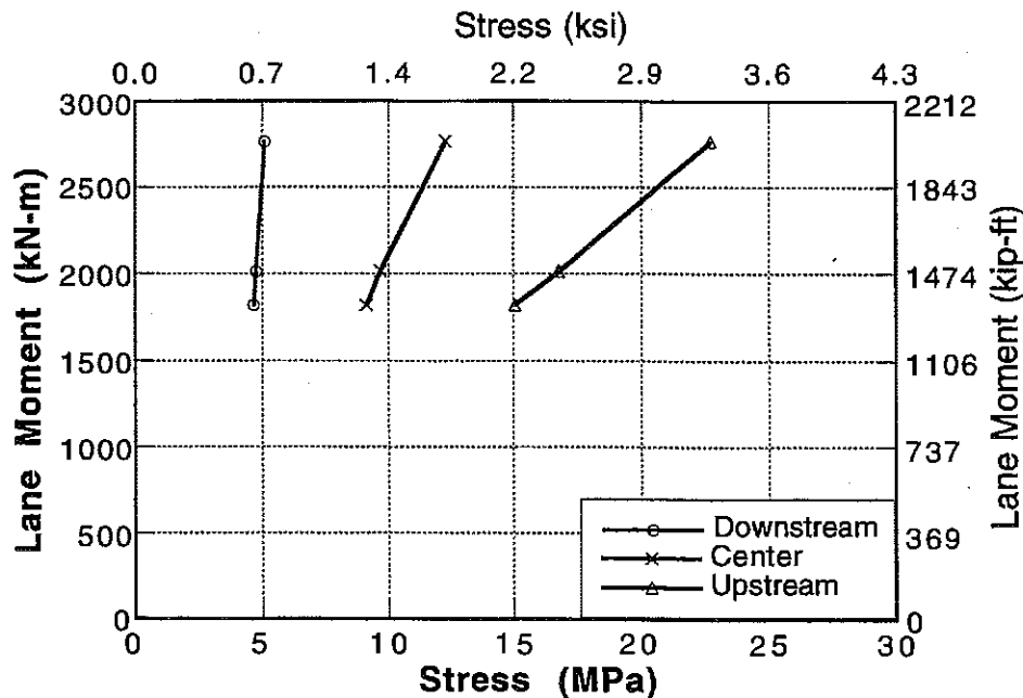
Figure 8-11 : Stress at Mid-Span of Girder 3 of Bridge No. 3 - North Span.
