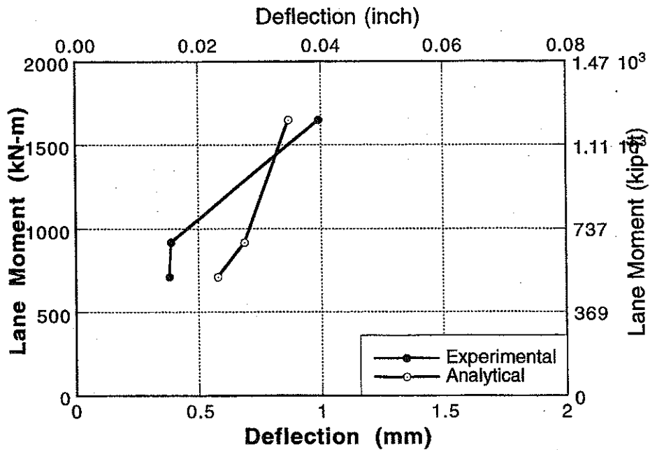
Figure A-184 : Experimental and Analytical Deflections for Bridge No. 5, Girder 7 and 8 for Lane 4 and 5 Loading.
