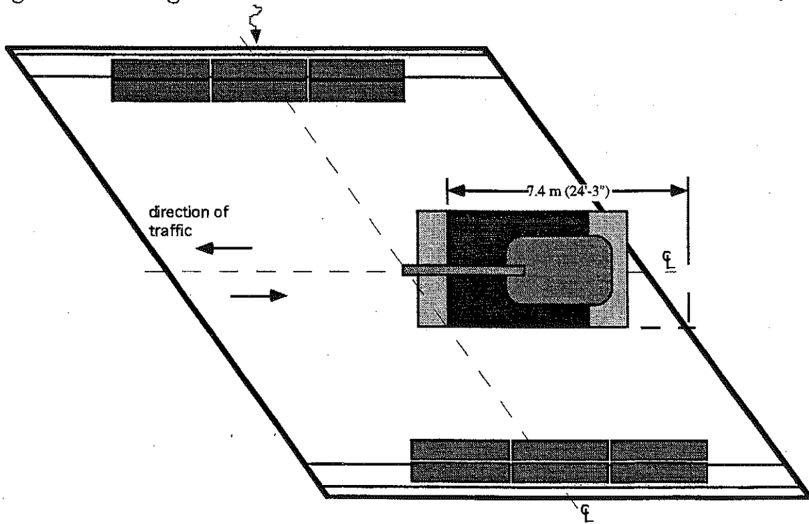
(a) Load Position 2 - Center Case.
