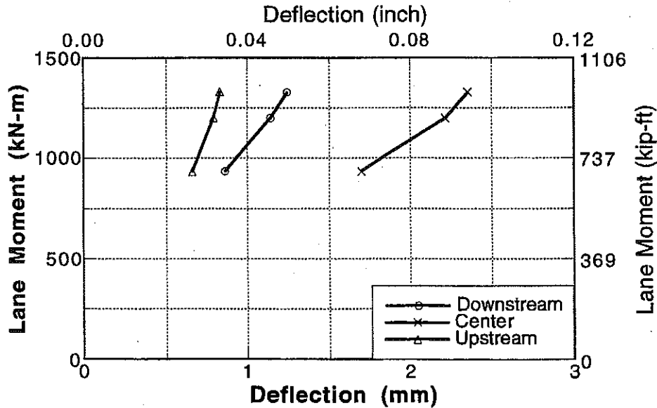
Figure 9-7 : Deflections at Mid-Span of Girder 6 of Bridge No. 4.
