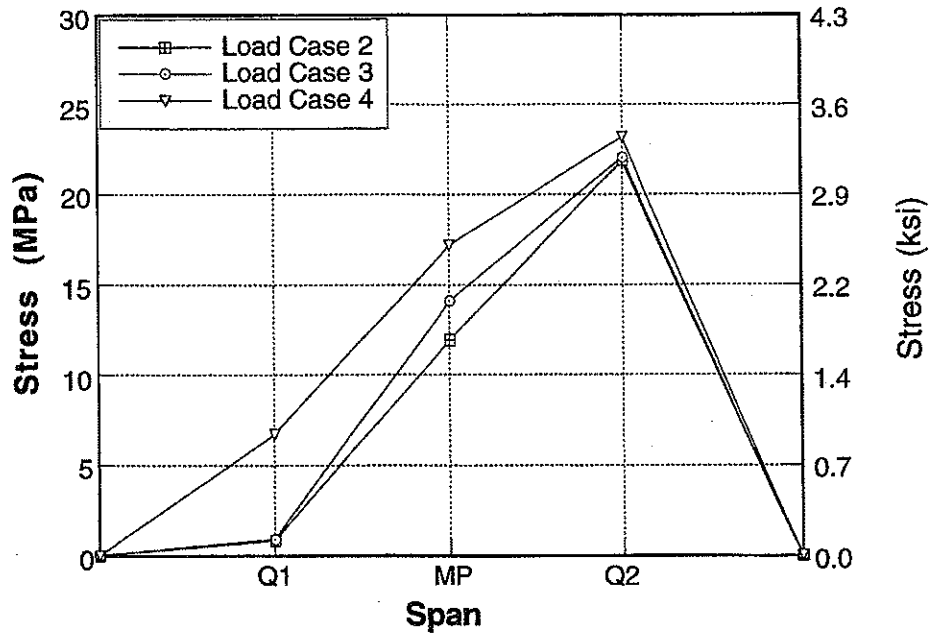
Figure A-106 : Longitudinal Distribution of Stresses for South Span of Bridge No. 3, Girder 6 due to Downstream Loading.
