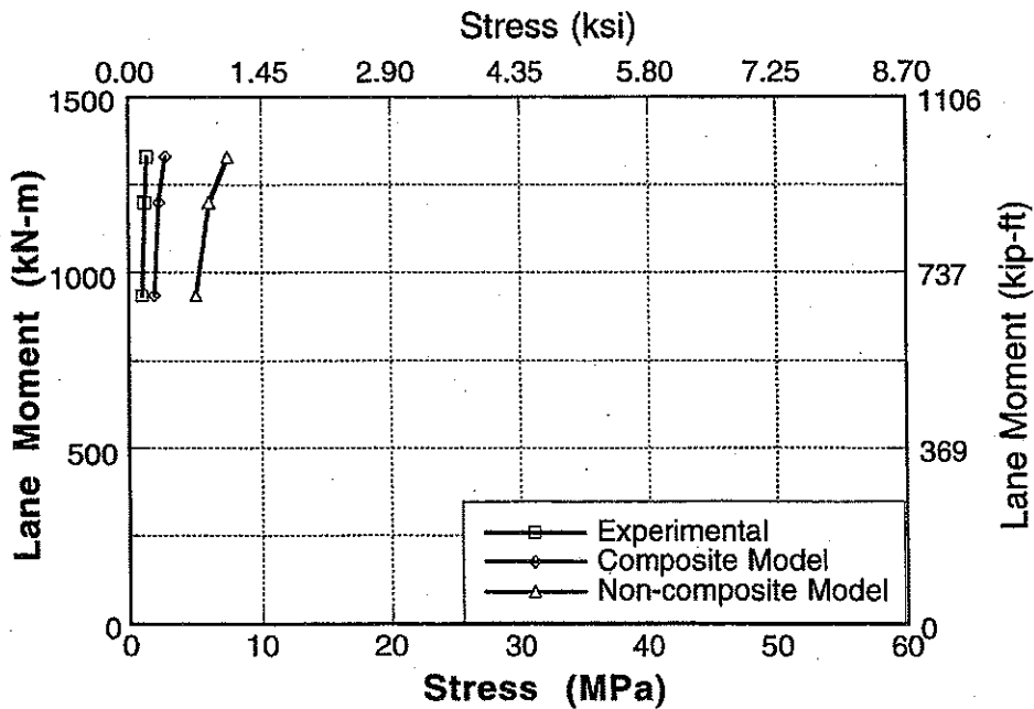
Figure A-41 : Experimental and Analytical Stresses for Bridge No. 4, Girder 2 and 3 for Downstream Loading.
