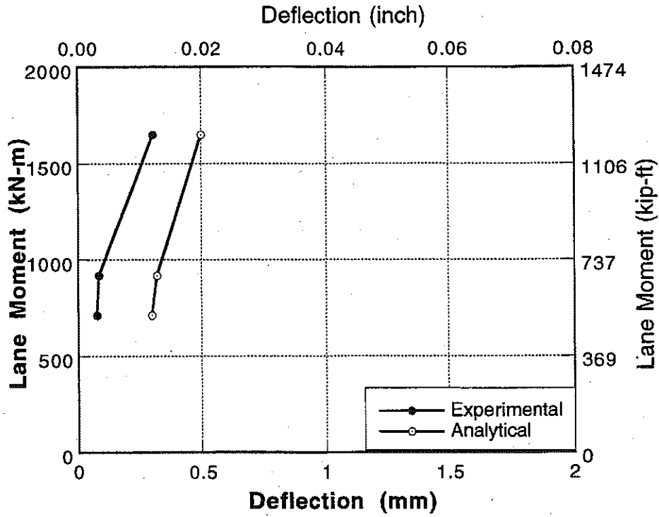
Figure 10-9 : Comparison of Measured and Analytical Deflections at Mid-span of Girder 5 due to Loading in Lane 1 and Lane 2.
