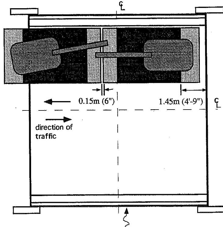
(c) Load Position 3 - Downstream Case.
