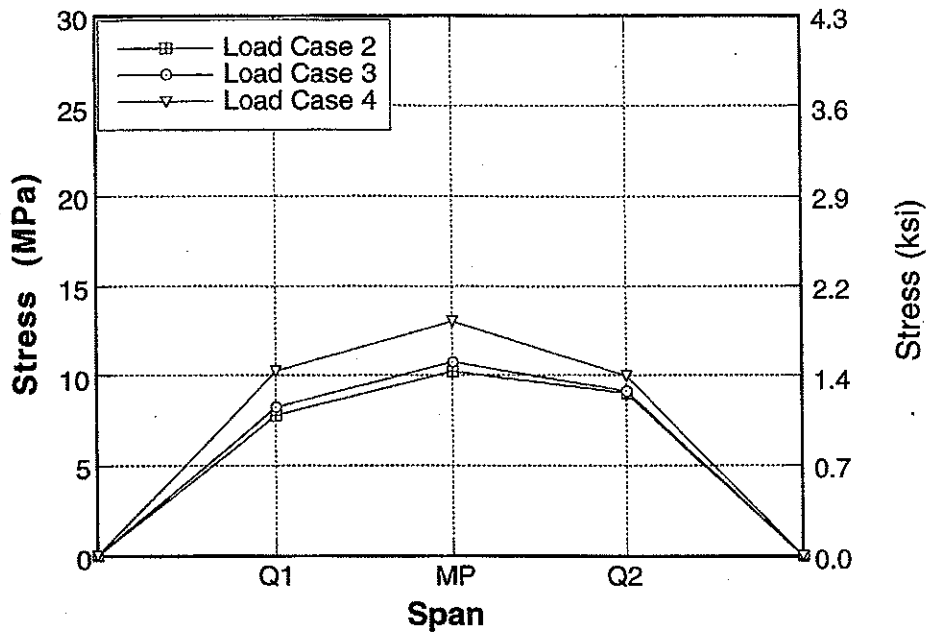
Figure A-83 : Longitudinal Distribution of Stresses for North Span of Bridge No. 3, Girder 6 due to Upstream Loading.
