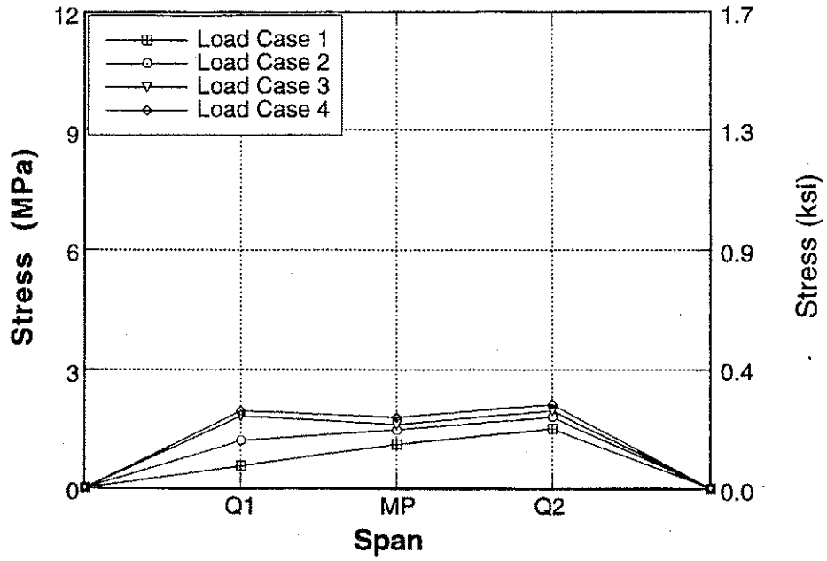
Figure A-58 : Longitudinal Distribution of Stresses for Bridge No. 2, Girder 9 due to Upstream Loading.
