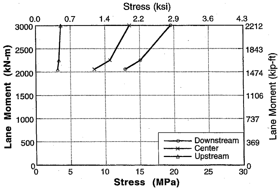
Figure A-86 : Stress vs Lane Moment for South Span of Bridge No. 3, Girder 6 and 7 at Mid Point.
