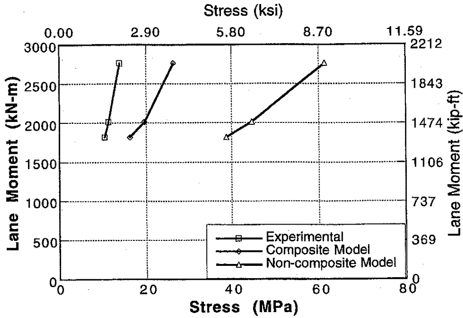
Figure 8-12 : Stress in Girder 3 for Upstream Loading on Bridge No. 3 - North Span.
