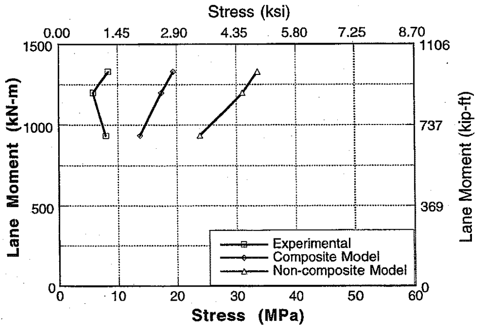
Figure A-143 : Experimental and Analytical Stresses for Bridge No. 4, Girder 4 and 5 for Upstream Loading.
