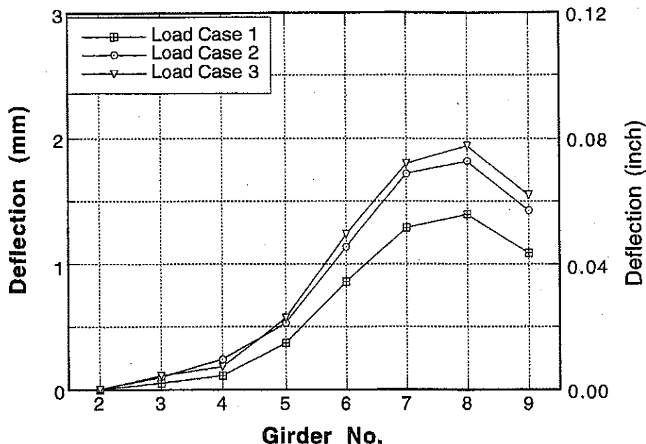
Figure 9-9 : Girder Distribution of Deflections due to Downstream Loading on Bridge No. 4.
