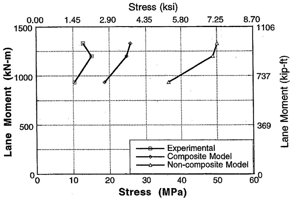
Figure A-142 : Experimental and Analytical Stresses for Bridge No. 4, Girder 2 and 3 for Upstream Loading.
