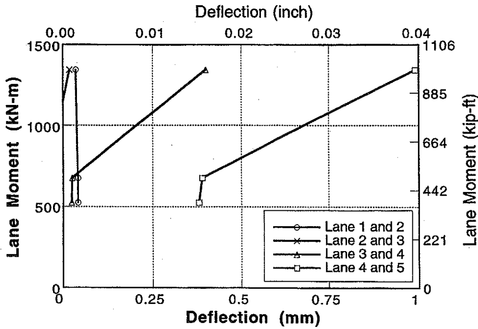
Figure A-164 : Deflection vs Lane Moment for Bridge No. 5, Girder 7 and 8.
