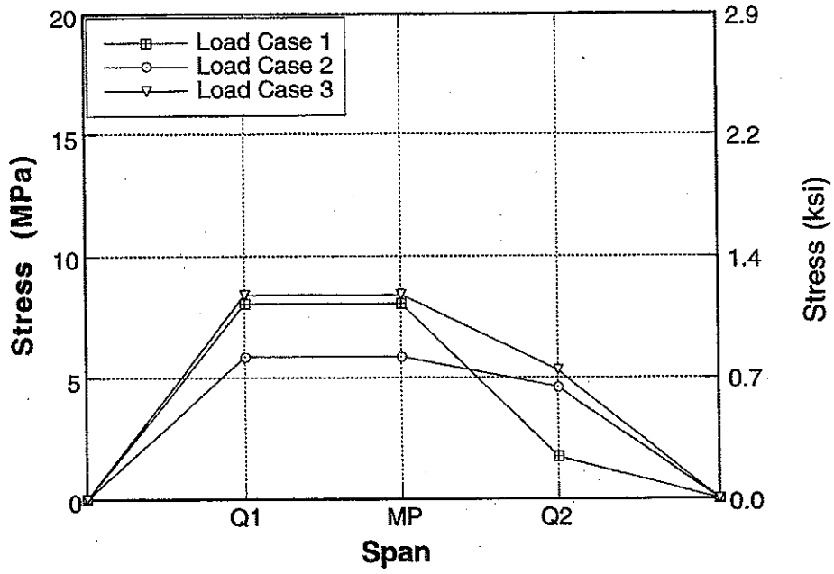
Figure A-154 : Longitudinal Distribution of Stresses for Bridge No. 4, Girder 5 due to Upstream Loading.
