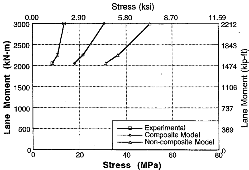
Figure A-94 : Experimental and Analytical Stresses for South Span of Bridge No. 3, Girder 6 and 7 for Center Loading.
