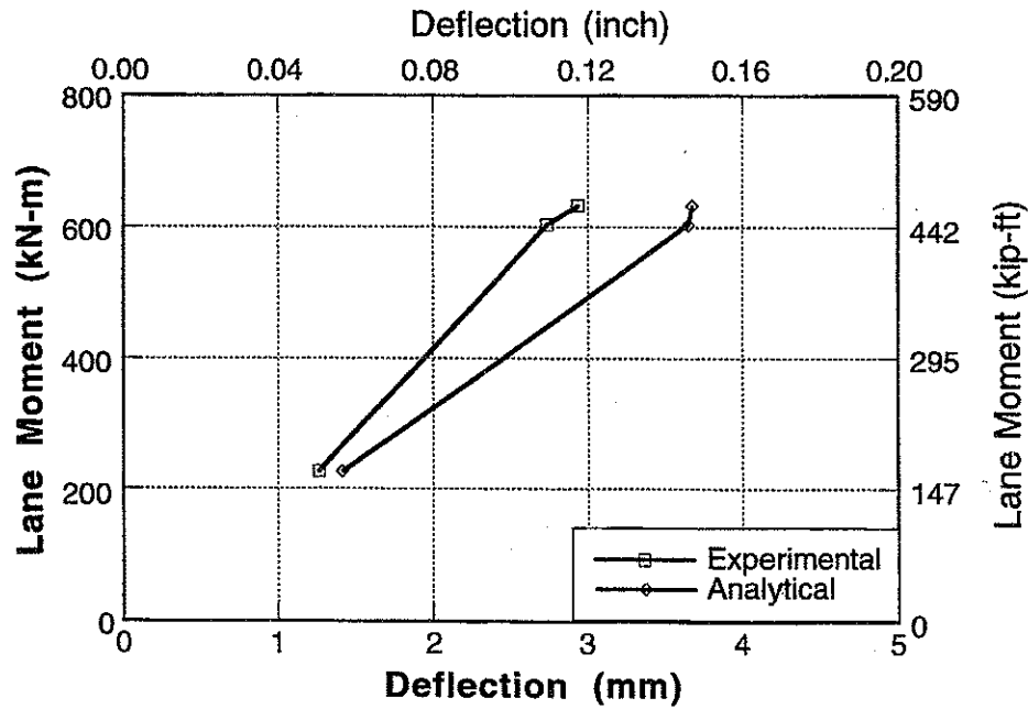
Figure A-5 : Experimental and Analytical Deflections for Bridge No. 1, Girder 3 and 4 for Downstream Loading.
