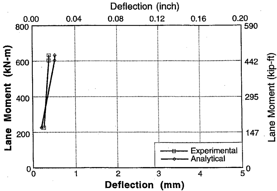
Figure A-6 : Experimental and Analytical Deflections for Bridge No. 1, Girder 5 and 6 for Downstream Loading.
