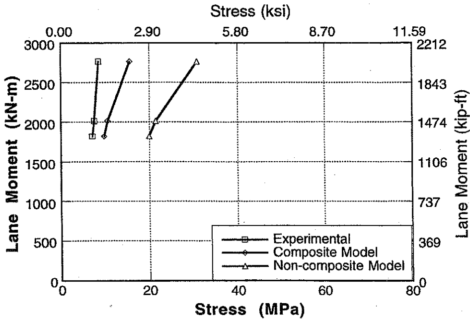
Figure A-73 : Experimental and Analytical Stresses for North Span of Bridge No. 3, Girder 6 and 7 for Upstream Loading.
