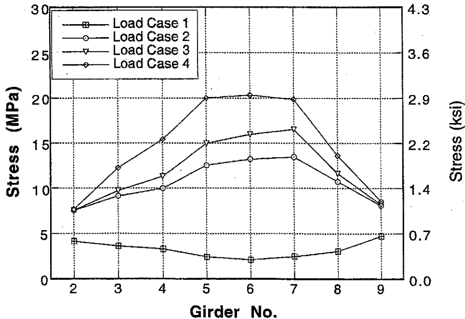
Figure 8-14 : Girder Distribution in terms of Stress due to Center Loading on Bridge No. 3 - North Span.
