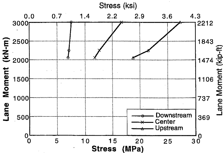
Figure 8-15 : Stress in Girder 3 on Bridge No. 3 - South Span.
