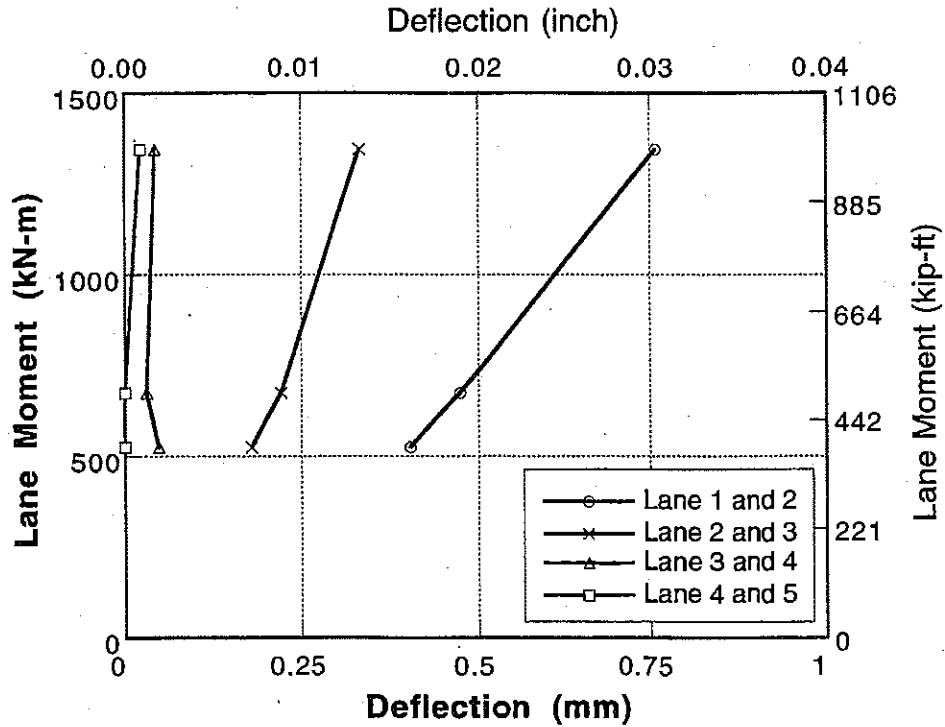
Figure 10-8 : Measured Deflections at Mid-span of Girder 2.
