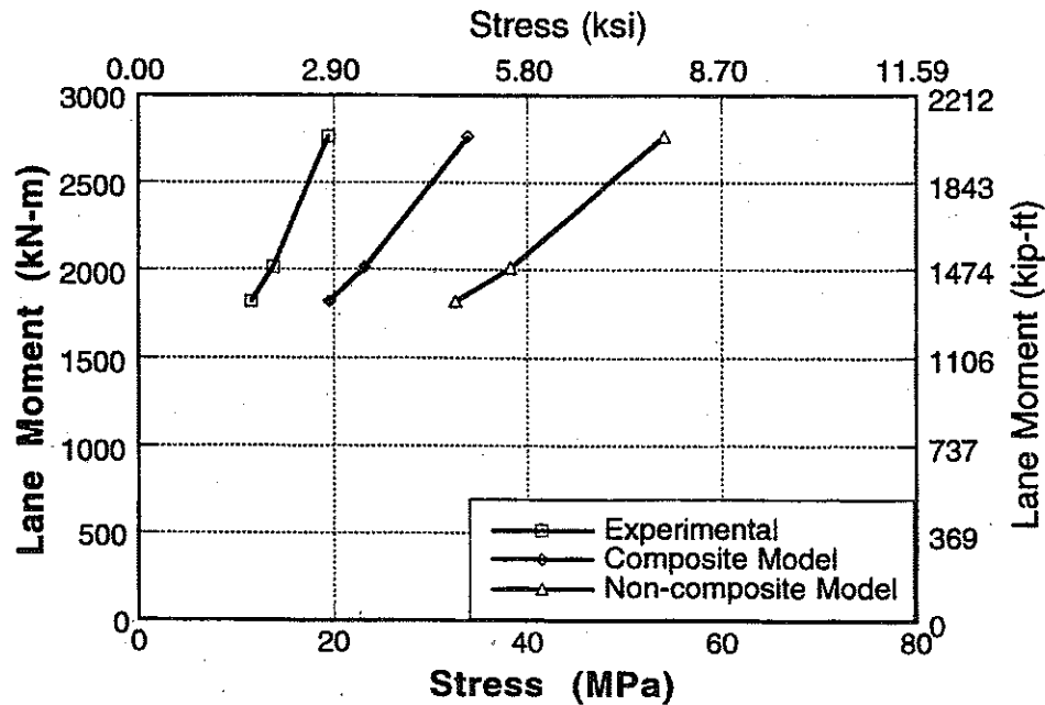
Figure A-65 : Experimental and Analytical Stresses for North Span of Bridge No. 3, Girder 6 and 7 for Downstream Loading.
