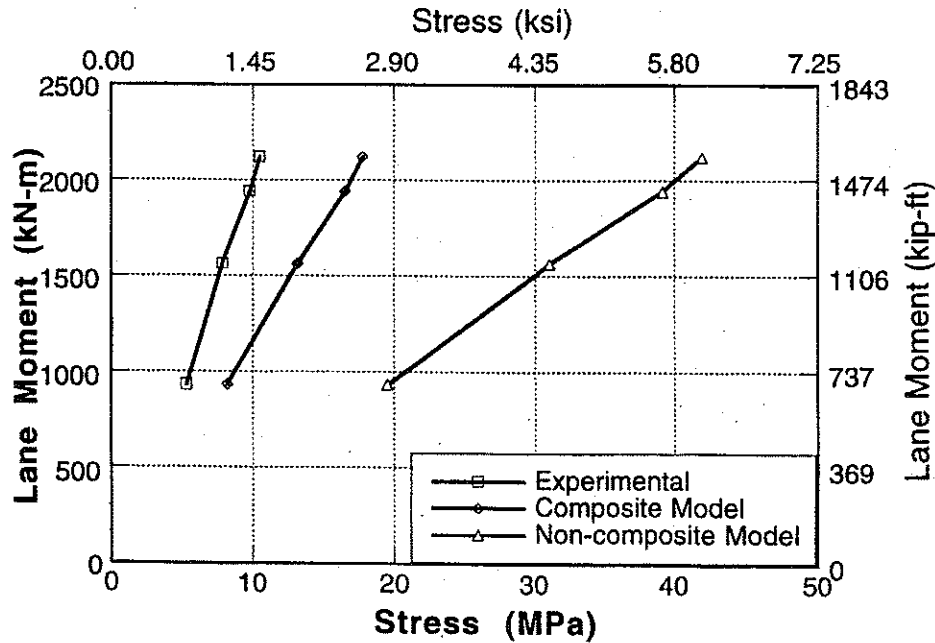
Figure A-43 : Experimental and Analytical Stresses for Bridge No. 2, Girder 8 and 9 for Downstream Loading.
