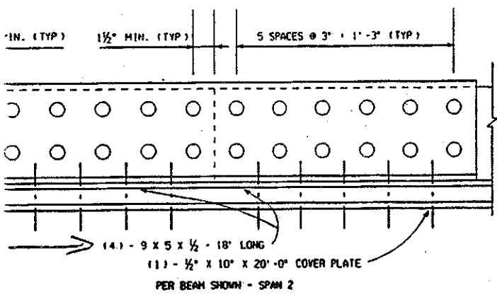
SPLICE DETAIL ELEVATION
