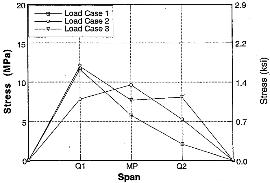
Figure A-150 : Longitudinal Distribution of Stresses for Bridge No. 4, Girder 4 due to Center Loading.
