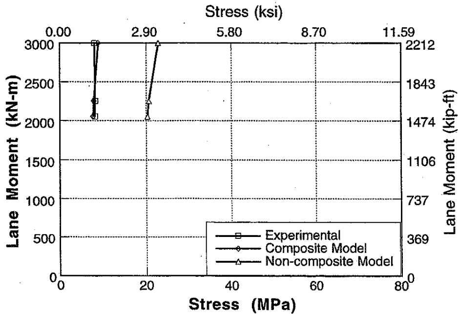
Figure A-99 : Experimental and Analytical Stresses for South Span of Bridge No. 3, Girder 8 and 9 for Upstream Loading.
