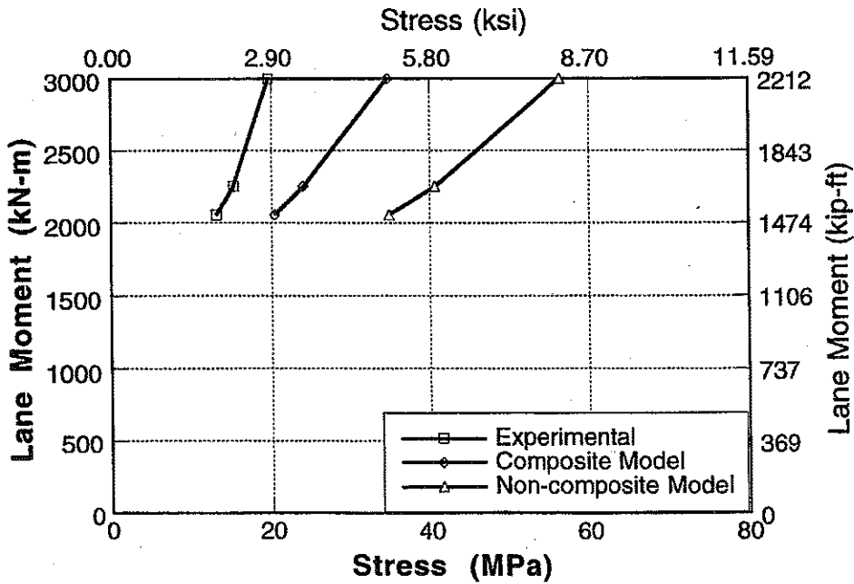
Figure A-90 : Experimental and Analytical Stresses for South Span of Bridge No. 3, Girder 6 and 7 for Downstream Loading.
