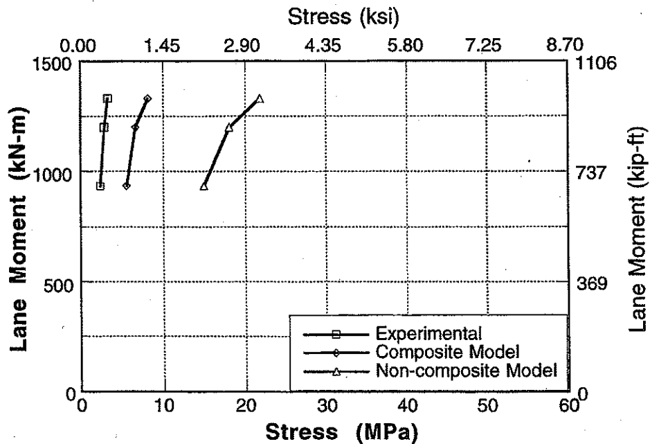
Figure A-141 : Experimental and Analytical Stresses for Bridge No. 4, Girder 8 and 9 for Center Loading.
