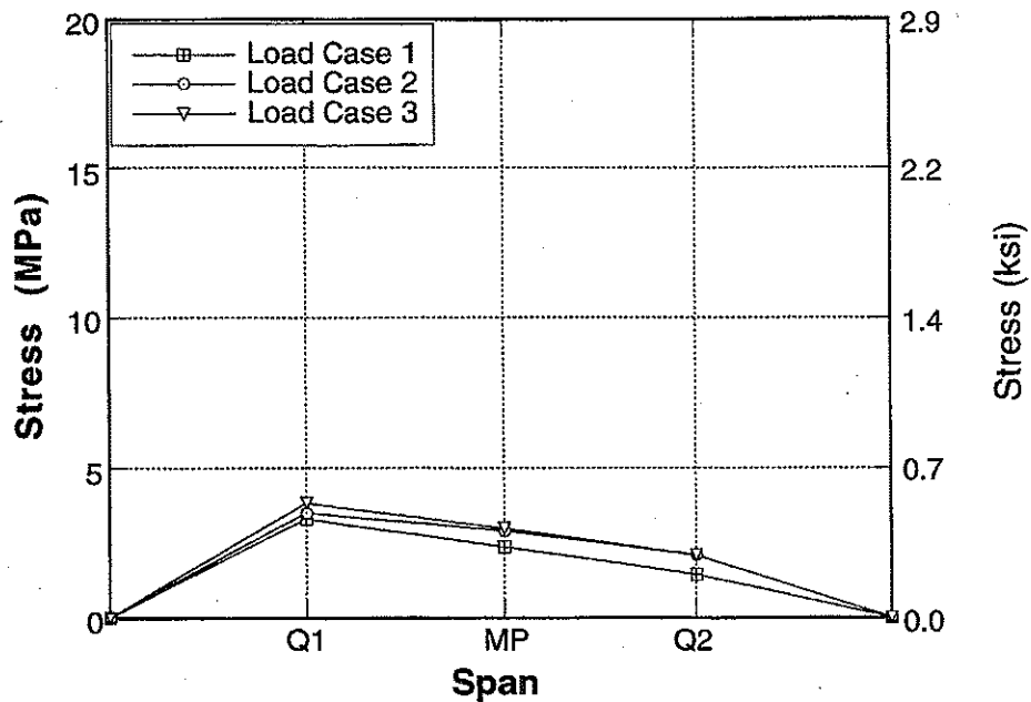
Figure A-160 : Longitudinal Distribution of Stresses for Bridge No. 4, Girder 7 due to Upstream Loading.
