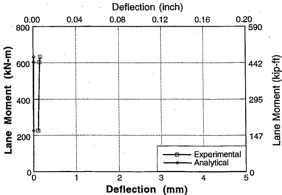
Figure A-12 : Experimental and Analytical Deflections for Bridge No. 1, Girder 5 and 6 for Upstream Loading.
