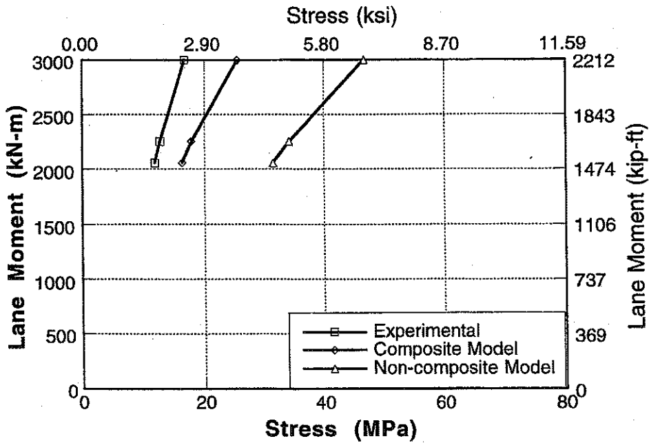
Figure A-92 : Experimental and Analytical Stresses for South Span of Bridge No. 3, Girder 2 and 3 for Center Loading.
