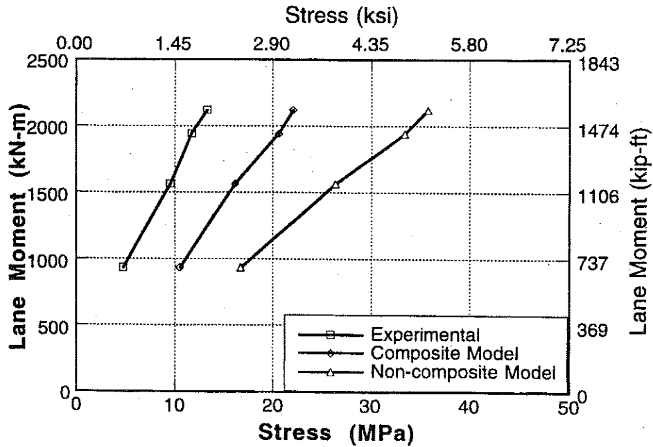
Figure A-44 : Experimental and Analytical Stresses for Bridge No. 2, Girder 2 and 3 for Center Loading.
