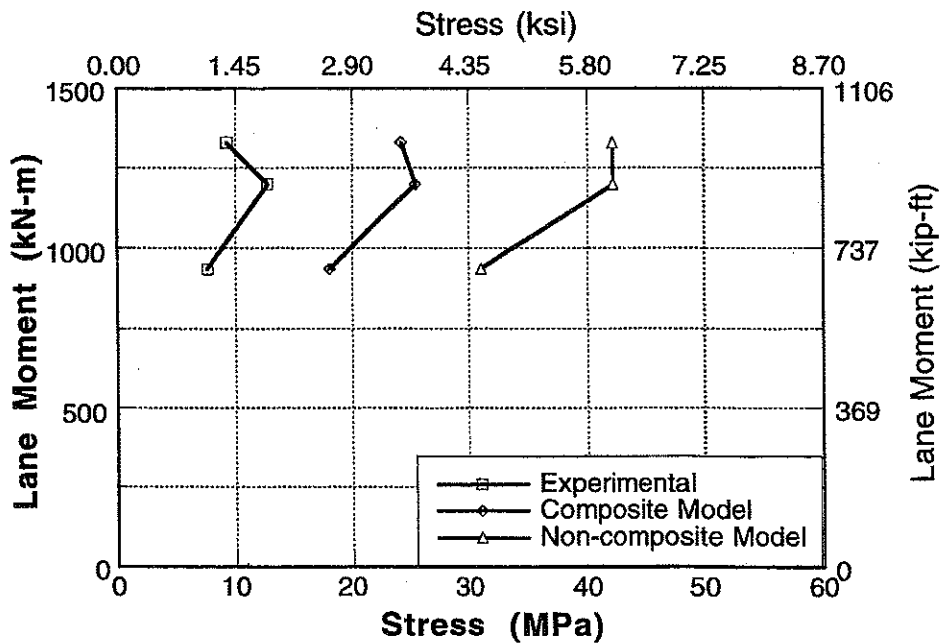
Figure A-136 : Experimental and Analytical Stresses for Bridge No. 4, Girder 6 and 7 for Downstream Loading.
