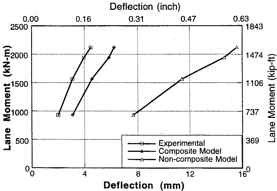
Figure A-25 : Experimental and Analytical Deflections for Bridge No. 2, Girder 4 and 5 for Center Loading.
