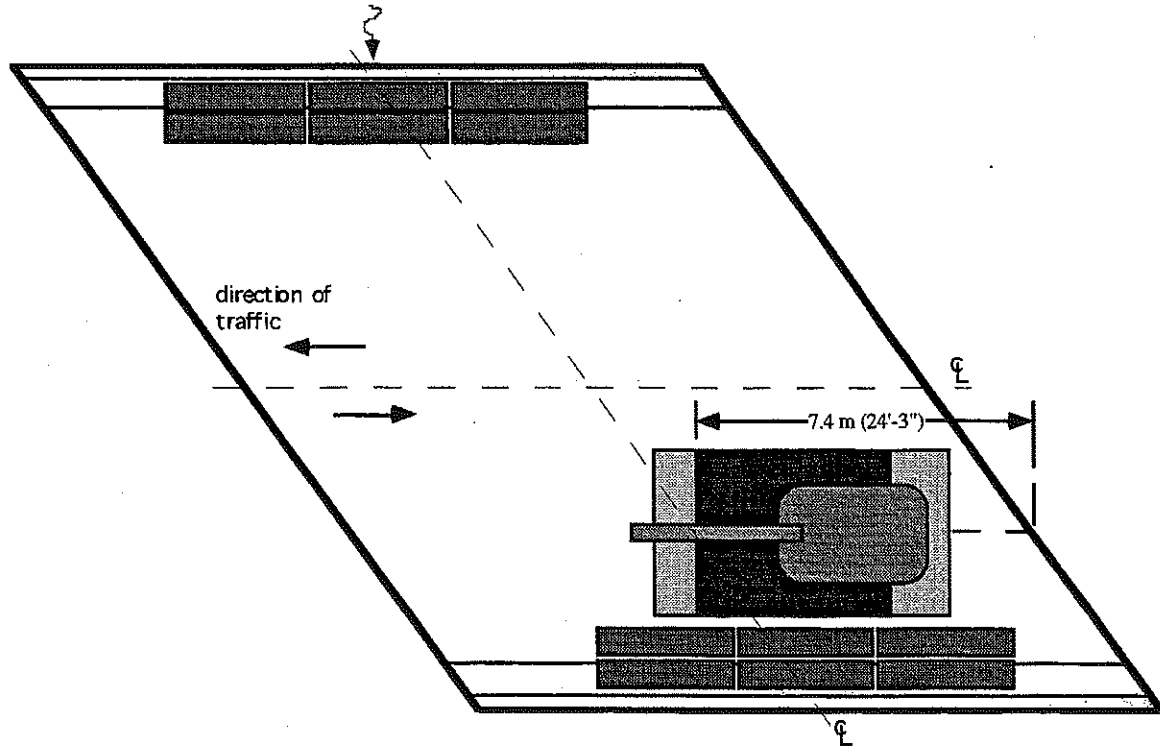
(c) Load Position 3 - Downstream Case.
