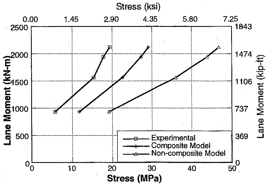
Figure 7-11 : Stresses at Mid-Span of Girder 3 for Upstream Loading on Bridge No. 2.
