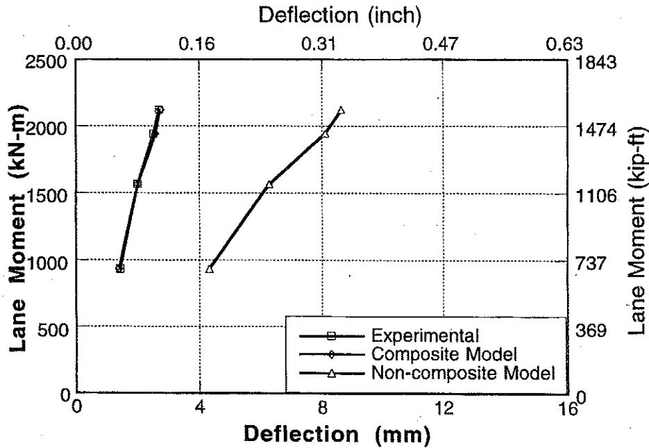
Figure A-30 : Experimental and Analytical Deflections for Bridge No. 2, Girder 6 and 7 for Upstream Loading.
