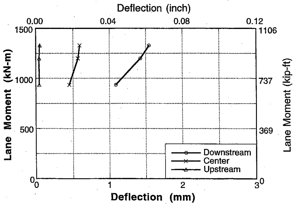
Figure A-112: Deflection vs Lane Moment for Bridge No. 4, Girder 8 and 9.
