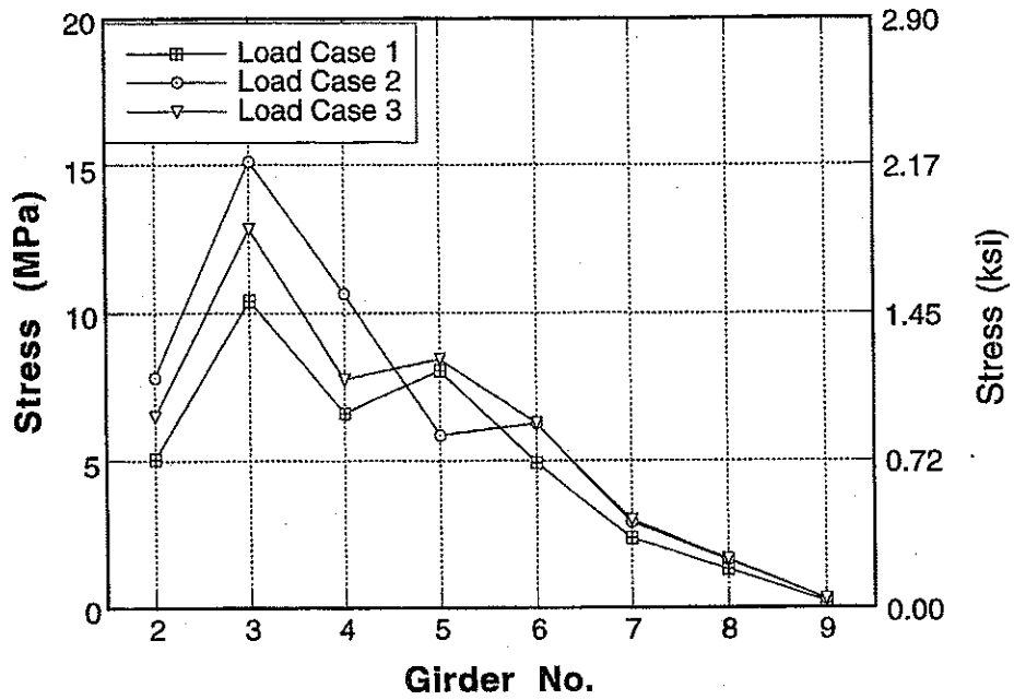
Figure A-148 : Girder Distribution of Stresses at Mid Point for Bridge No. 4 due to Upstream Loading.
