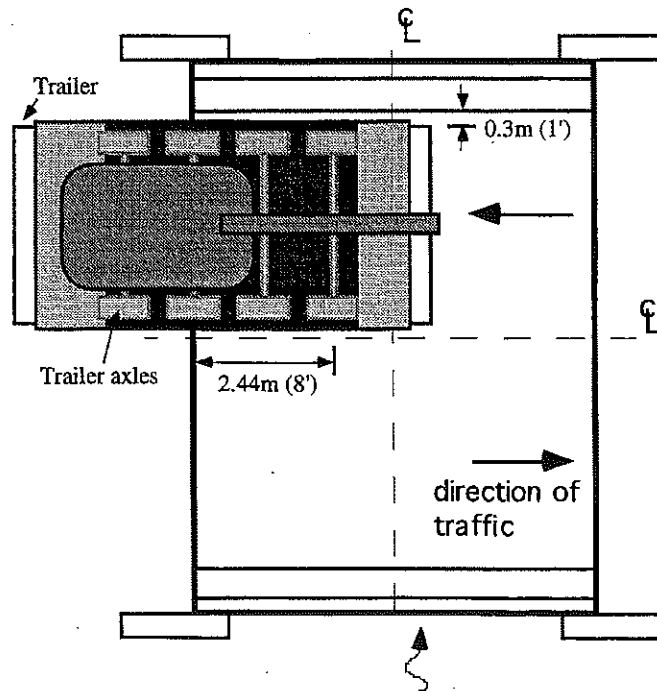
(a) Load Position 1 - Downstream.
