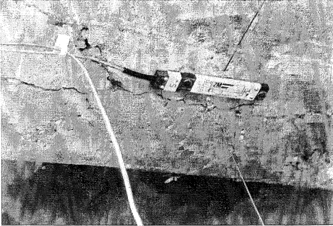
Figure 4-2 : Typical Strain Transducer Setup for Bridge No. 1.
