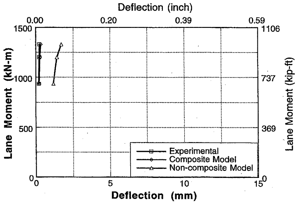
Figure A-123 : Experimental and Analytical Deflections for Bridge No. 4, Girder 7 and 8 for Upstream Loading.
