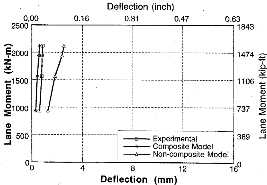
Figure A-31 : Experimental and Analytical Deflections for Bridge No. 2, Girder 8 and 9 for Upstream Loading.
