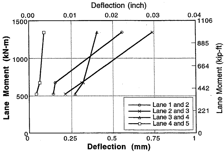
Figure A-162 : Deflection vs Lane Moment for Bridge No. 5, Girder 3 and 4.
