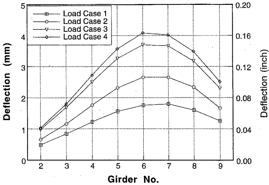
Figure A-32 : Girder Distribution of Deflections for Bridge No. 2 due to Downstream Loading.
