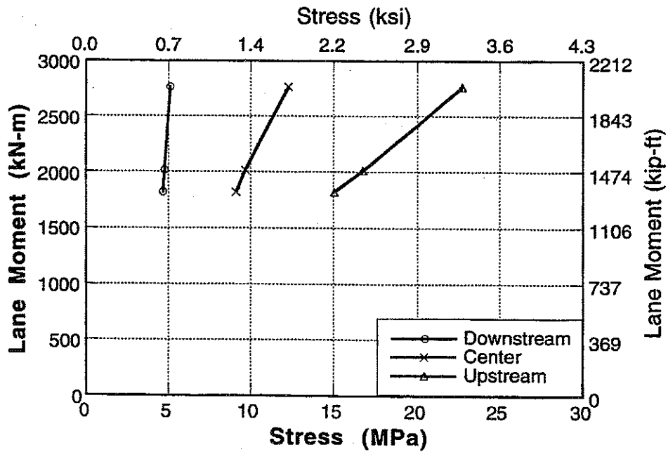
Figure A-59: Stress vs Lane Moment for North Span of Bridge No. 3, Girder 2 and 3 at Mid Point.
