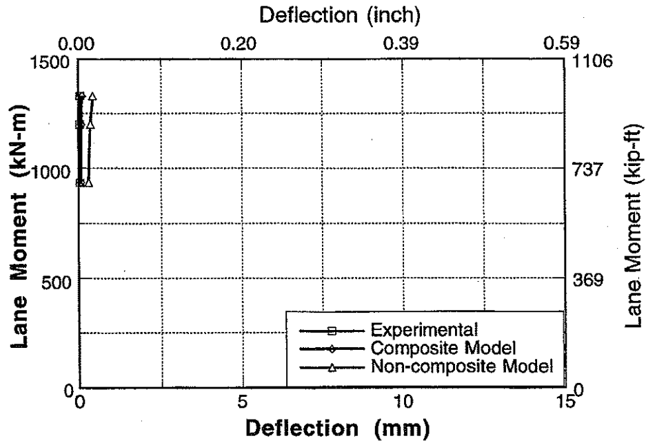
Figure A-124 : Experimental and Analytical Deflections for Bridge No. 4, Girder 8 and 9 for Upstream Loading.
