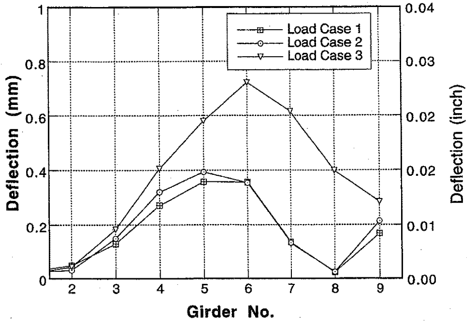
Figure A-188 : Girder Distribution of Deflections for Bridge No. 5 due to Loading in Lane 3 and 4.
