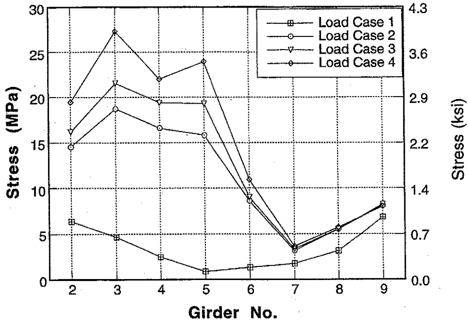
Figure A-102 : Girder Distribution of Stresses at Mid Point for South Span of Bridge No. 3 due to Upstream Loading.
