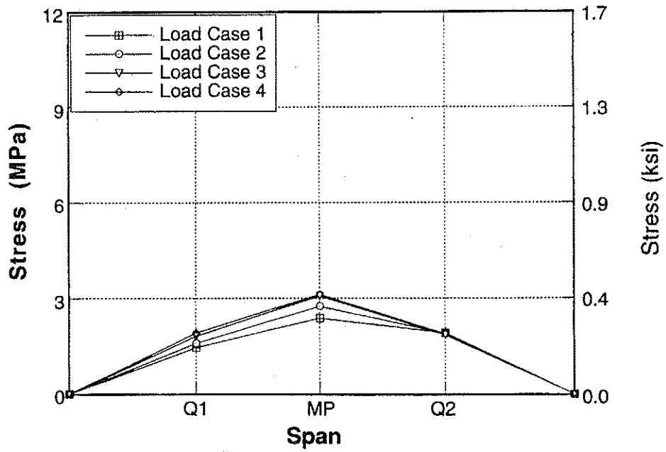
Figure A-53 : Longitudinal Distribution of Stresses for Bridge No. 2, Girder 2 due to Downstream Loading.
