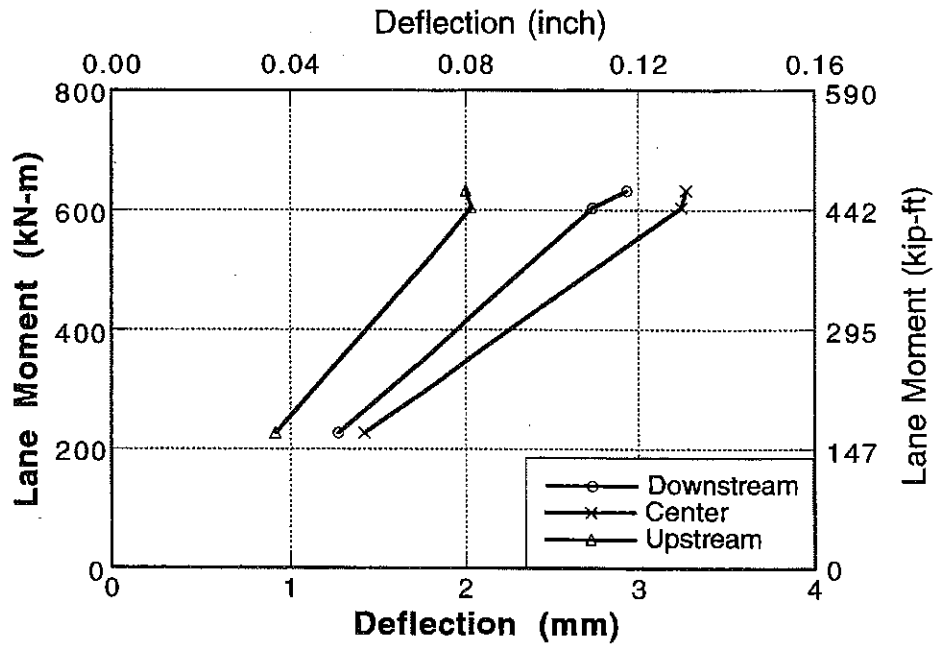
Figure 6-7 : Deflection at Mid-Span of Girder 4 of Bridge No. 1.
