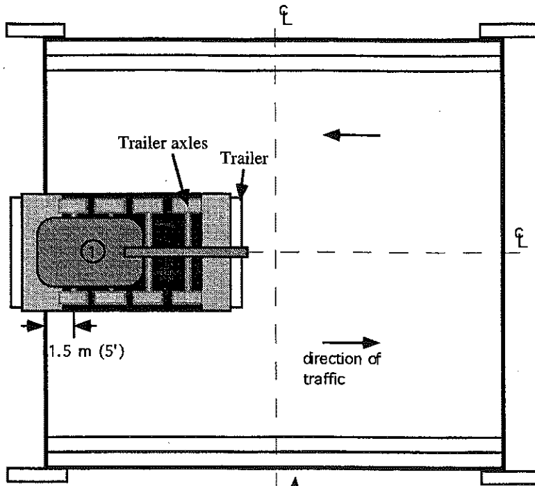
(a) Load Case 1 - Center Case.
