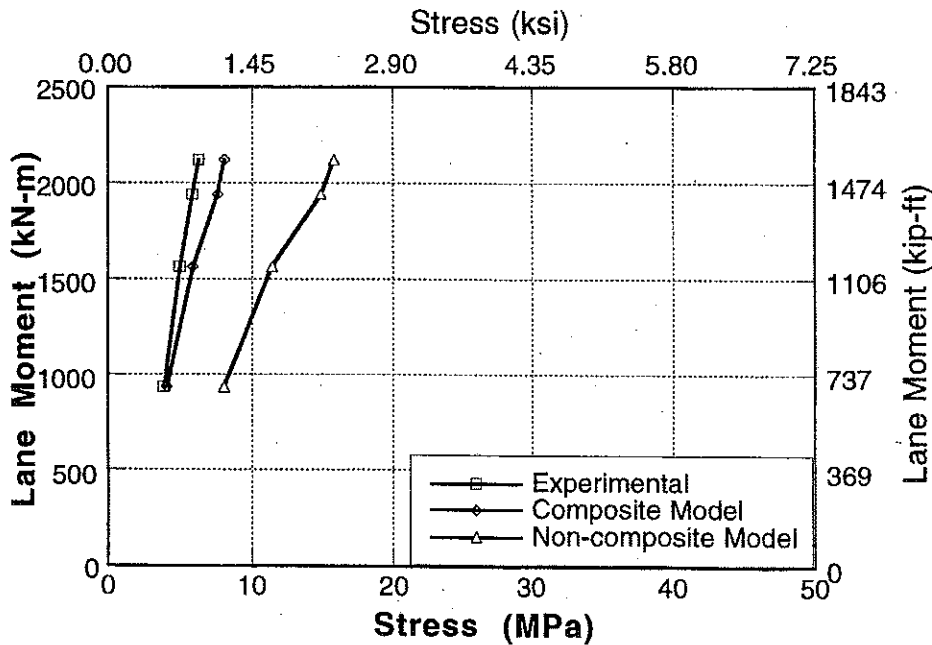
Figure A-41 : Experimental and Analytical Stresses for Bridge No. 2, Girder 2 and 3 for Downstream Loading.
