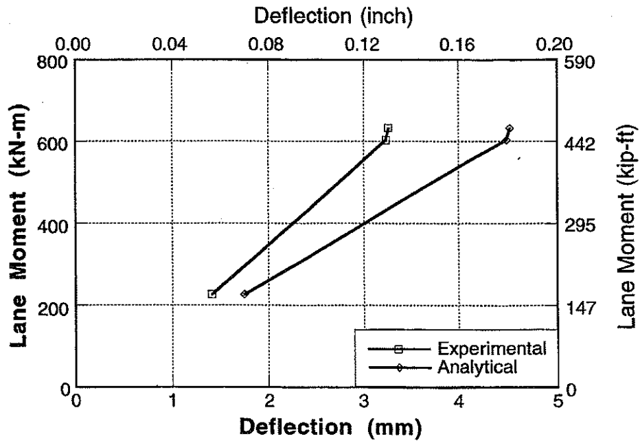
Figure A-8 : Experimental and Analytical Deflections for Bridge No. 1, Girder 3 and 4 for Center Loading.
