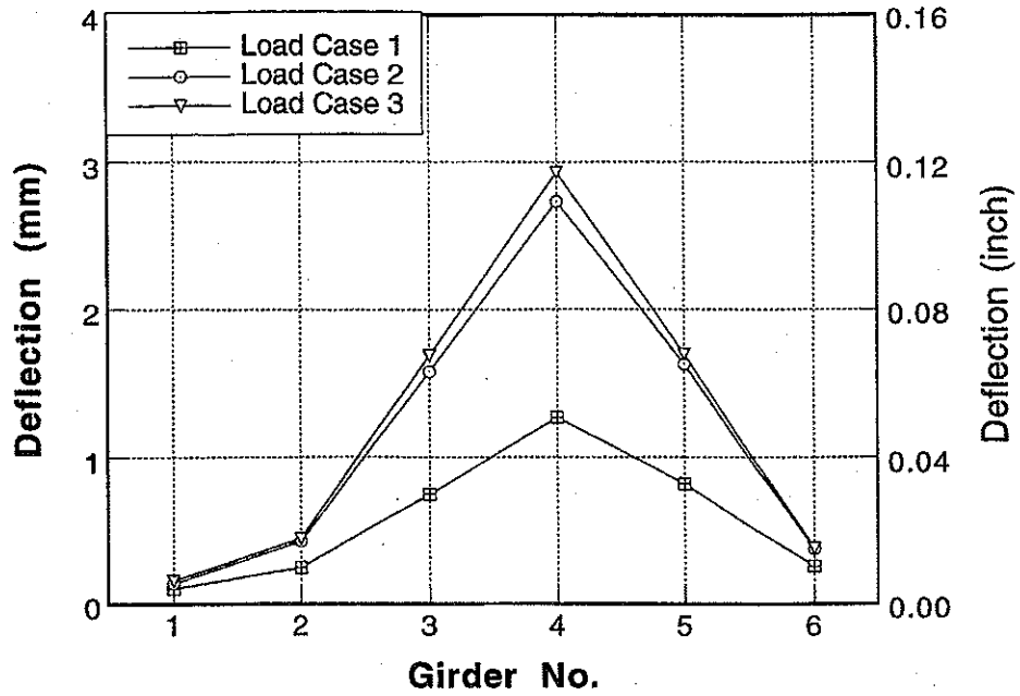
Figure A-13 Girder Distribution of Deflections for Bridge No. 1 due to Downstream Loading.
