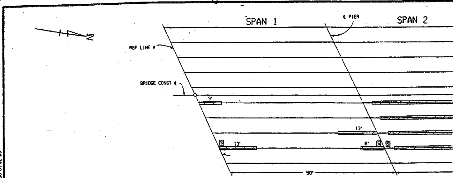
BEAM REPAIR LOCATION DIAGRAM
