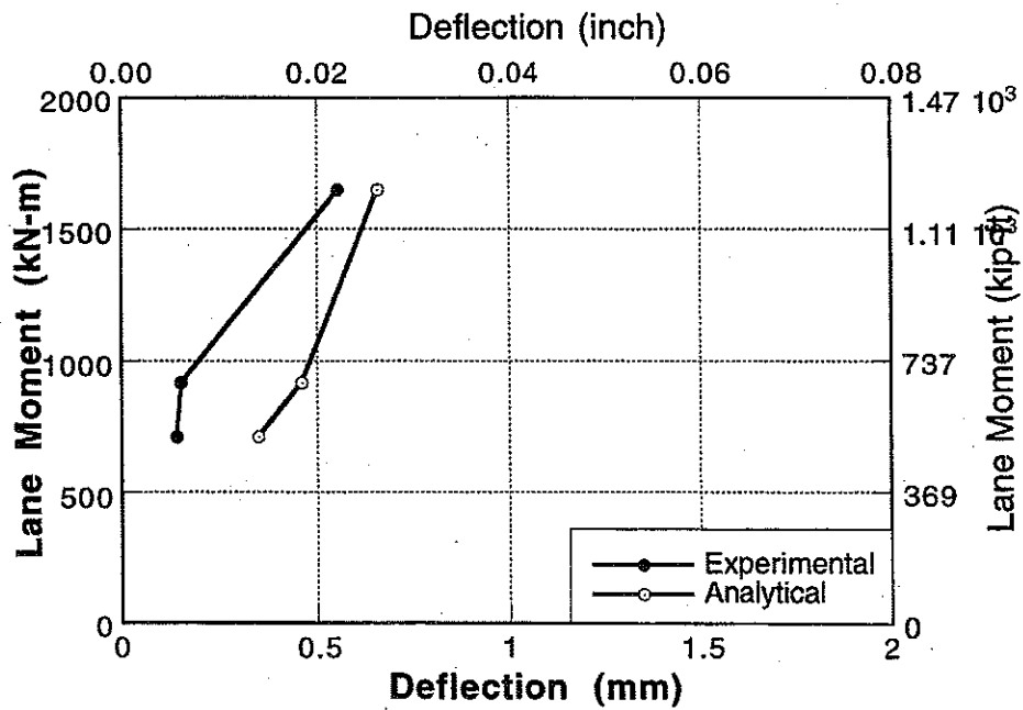
Figure A-167 : Experimental and Analytical Deflections for Bridge No. 5, Girder 3 and 4 for Lane 1 and 2 Loading.
