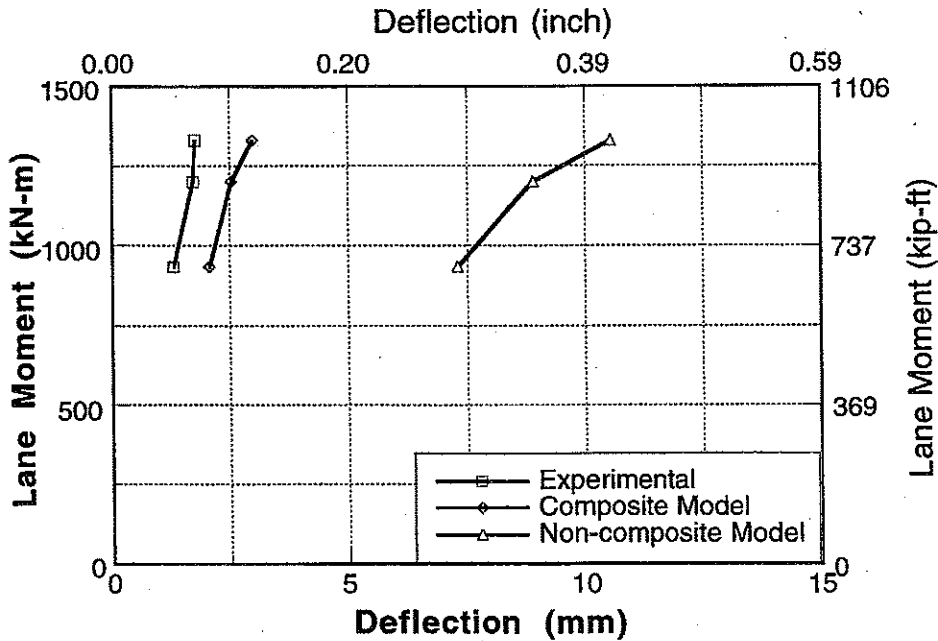
Figure A-121 : Experimental and Analytical Deflections for Bridge No. 4, Girder 3 and 4 for Upstream Loading.
