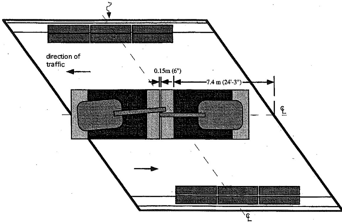
(c) Load Position 4 - Center Case.
