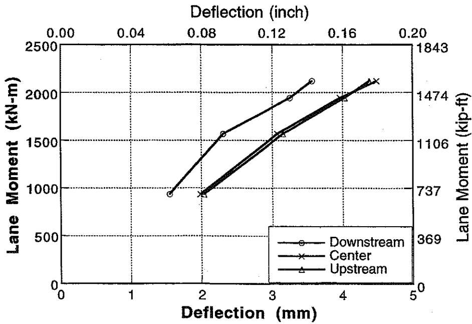
Figure A-17: Deflection vs Lane Moment for Bridge No. 2, Girder 4 and 5.
