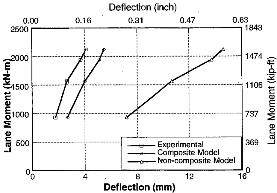
Figure 7-8 : Deflections at Mid-Span of Girder 6 for Downstream Loading on Bridge No. 2.
