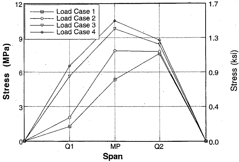
Figure A-56 : Longitudinal Distribution of Stresses for Bridge No. 2, Girder 9 due to Downstream Loading.
