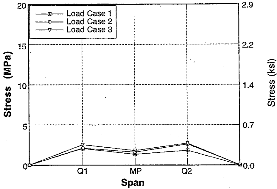
Figure A-149 : Longitudinal Distribution of Stresses for Bridge No. 4, Girder 4 due to Downstream Loading.
