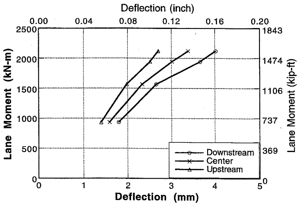
Figure A-18: Deflection vs Lane Moment for Bridge No. 2, Girder 6 and 7.
