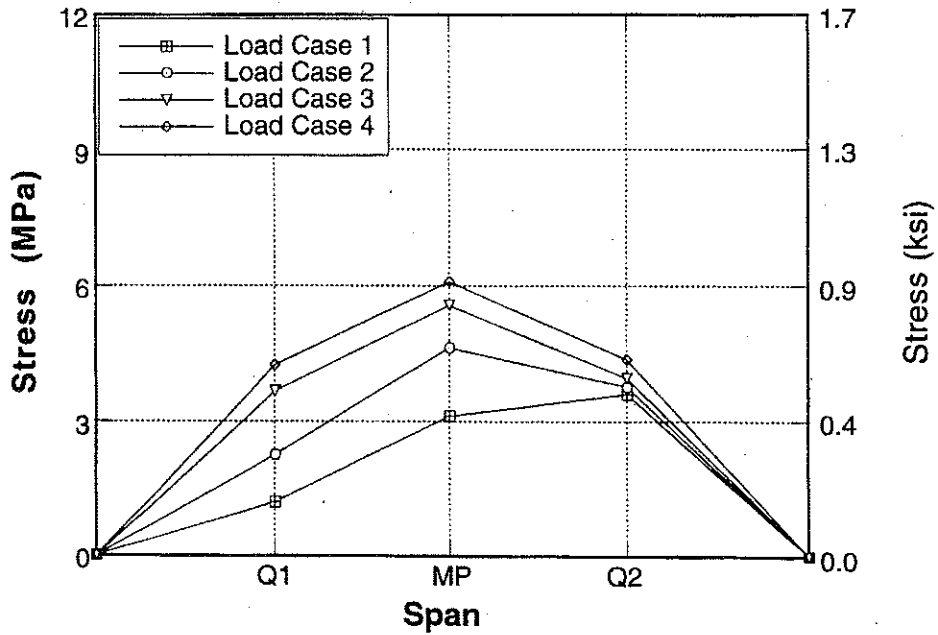
Figure A-54 : Longitudinal Distribution of Stresses for Bridge No. 2, Girder 2 due to Center Loading.
