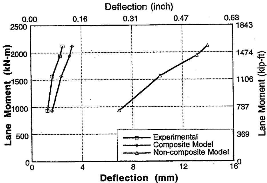
Figure A-23 : Experimental and Analytical Deflections for Bridge No. 2, Girder 8 and 9 for Downstream Loading.
