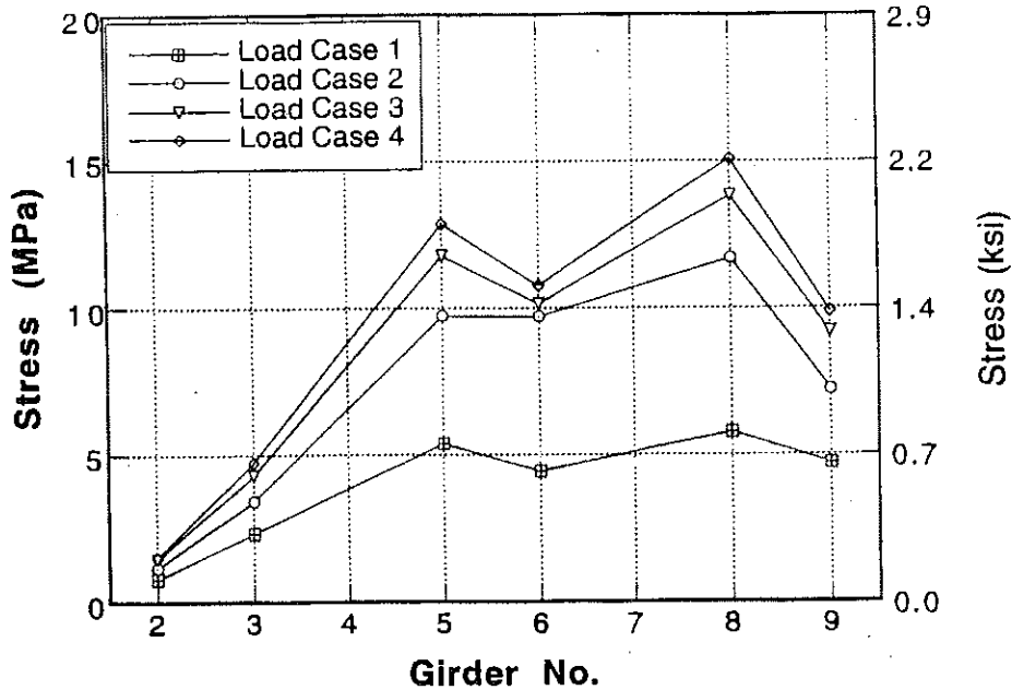
Figure 7-13 : Girder Distribution of Stresses due to Downstream Loading on Bridge No. 2.
