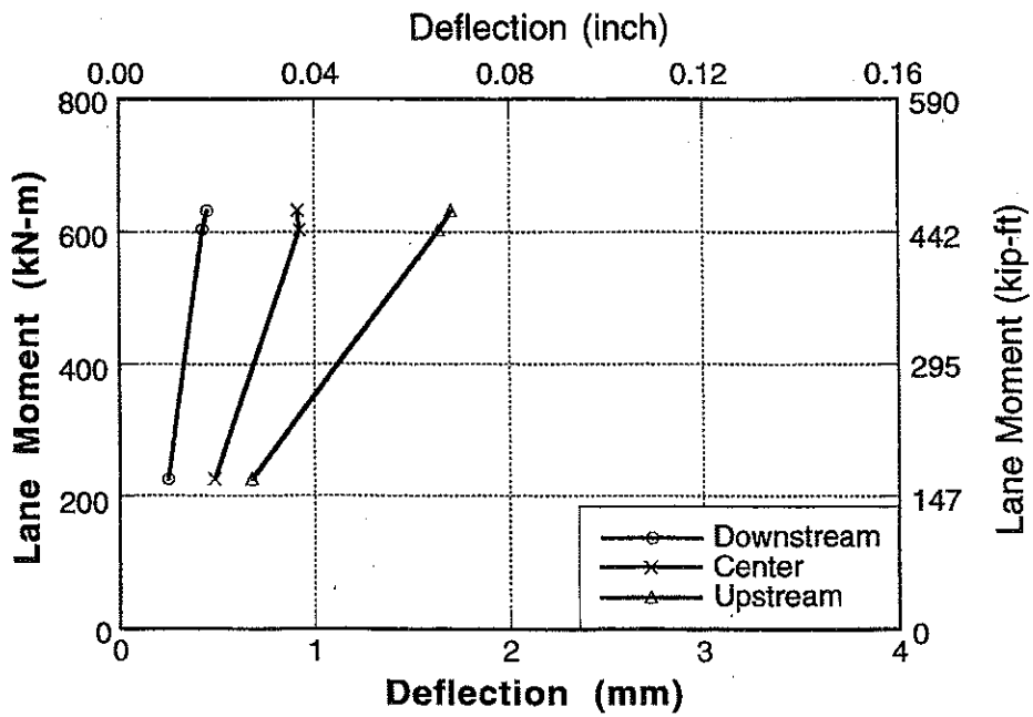
Figure A-1 : Deflection vs Lane Moment for Bridge No. 1, Girder 1 and 2.
