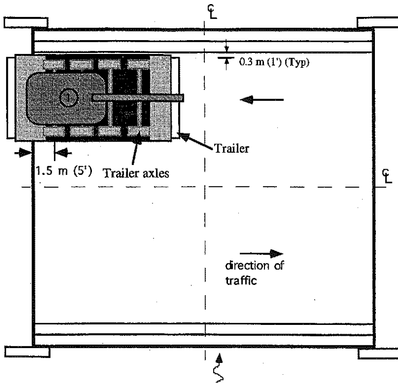
(a) Load Position 1 - Downstream Case.
