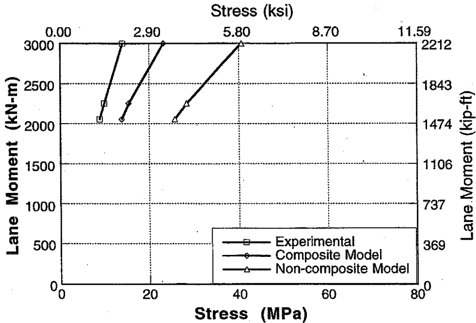
Figure A-89 : Experimental and Analytical Stresses for South Span of Bridge No. 3, Girder 4 and 5 for Downstream Loading.
