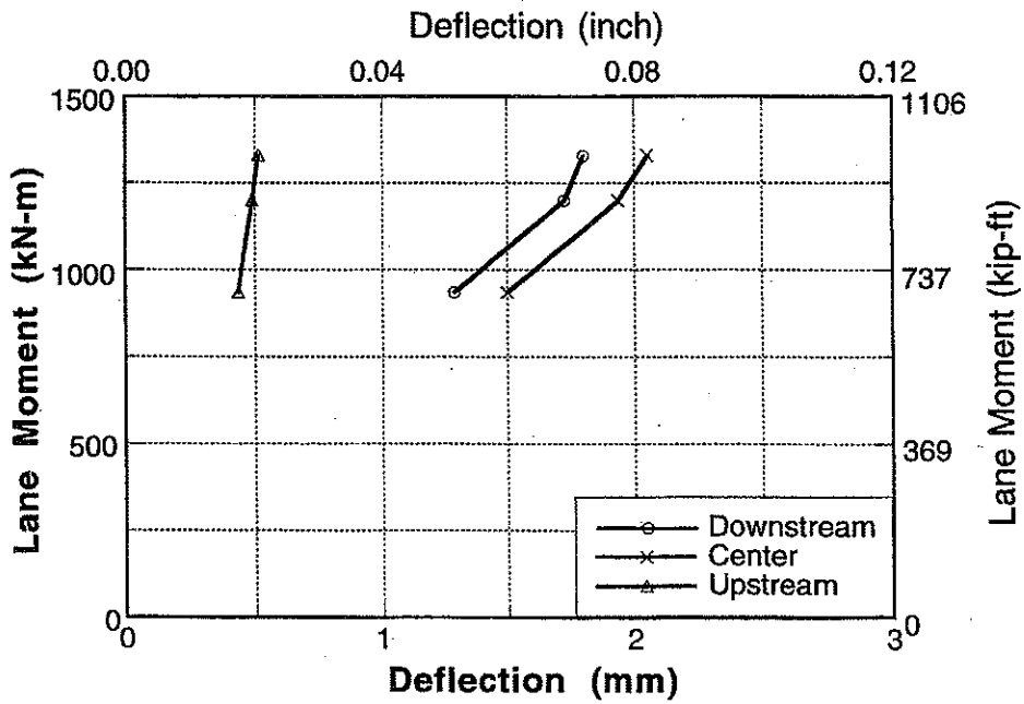
Figure A-111: Deflection vs Lane Moment for Bridge No. 4, Girder 6 and 7.
