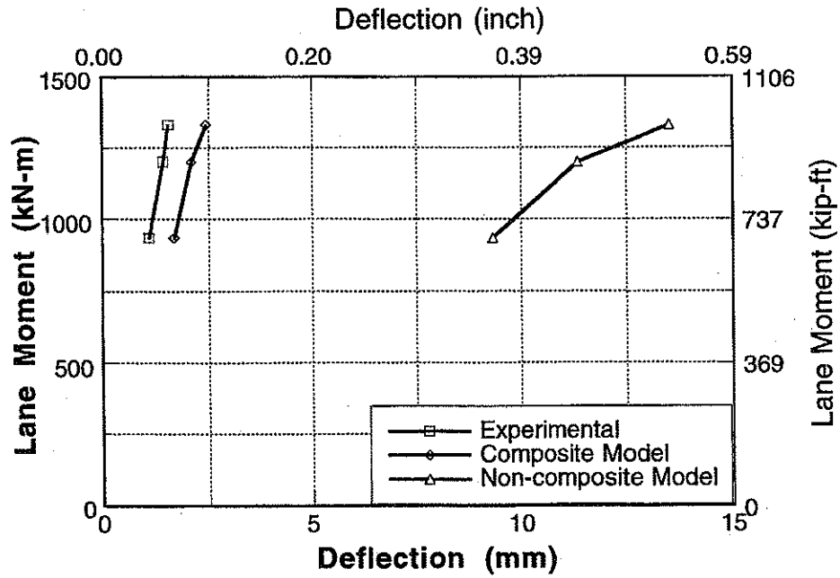
Figure A-116 : Experimental and Analytical Deflections for Bridge No. 4, Girder 9 for Downstream Loading.
