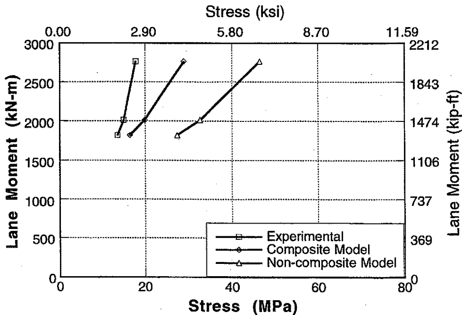
Figure A-72 : Experimental and Analytical Stresses for North Span of Bridge No. 3, Girder 4 and 5 for Upstream Loading.
