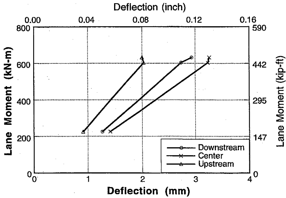
Figure A-2 : Deflection vs Lane Moment for Bridge No. 1, Girder 3 and 4.
