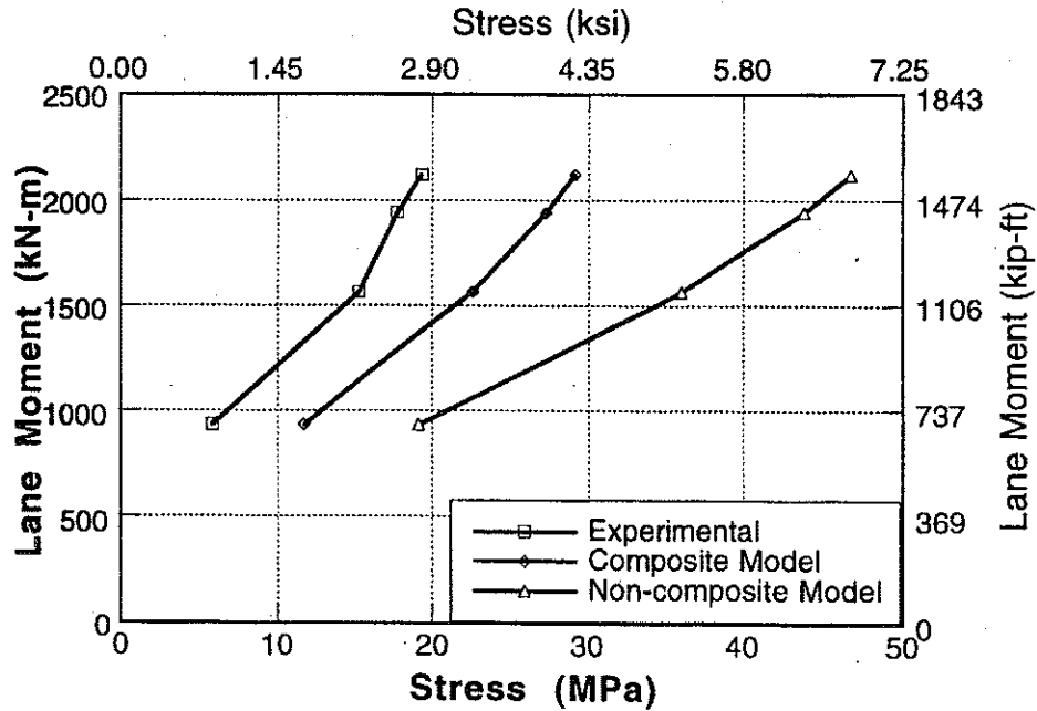
Figure A-47 : Experimental and Analytical Stresses for Bridge No. 2, Girder 2 and 3 for Upstream Loading.
