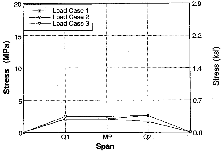
Figure A-152 : Longitudinal Distribution of Stresses for Bridge No. 4, Girder 5 due to Downstream Loading.
