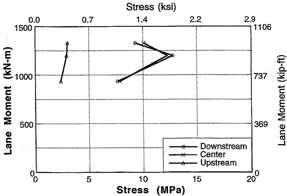
Figure A-133 : Stress vs Lane Moment for Bridge No. 4, Girder 6 and 7 at Mid Point.
