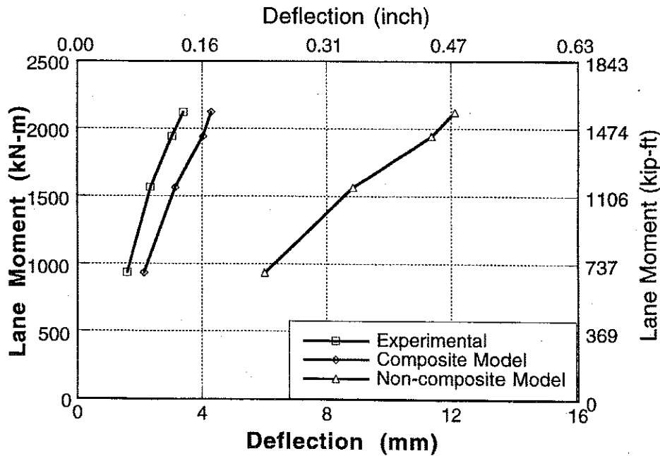
Figure A-26 : Experimental and Analytical Deflections for Bridge No. 2, Girder 6 and 7 for Center Loading.
