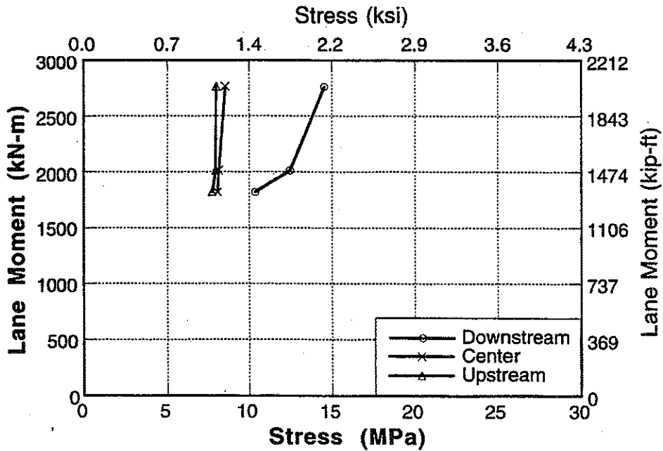
Figure A-62 : Stress vs Lane Moment for North Span of Bridge No. 3, Girder 8 and 9 at Mid Point.
