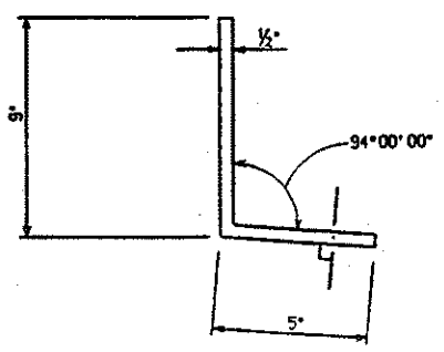
BENT PLATE DETAIL
