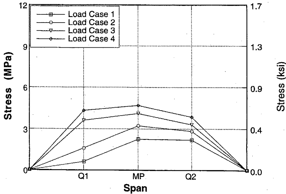
Figure A-57 : Longitudinal Distribution of Stresses for Bridge No. 2, Girder 9 due to Center Loading.
