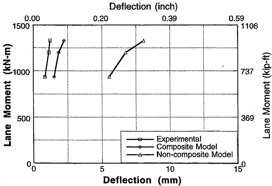
Figure A-114 : Experimental and Analytical Deflections for Bridge No. 4, Girder 5 and 6 for Downstream Loading.
