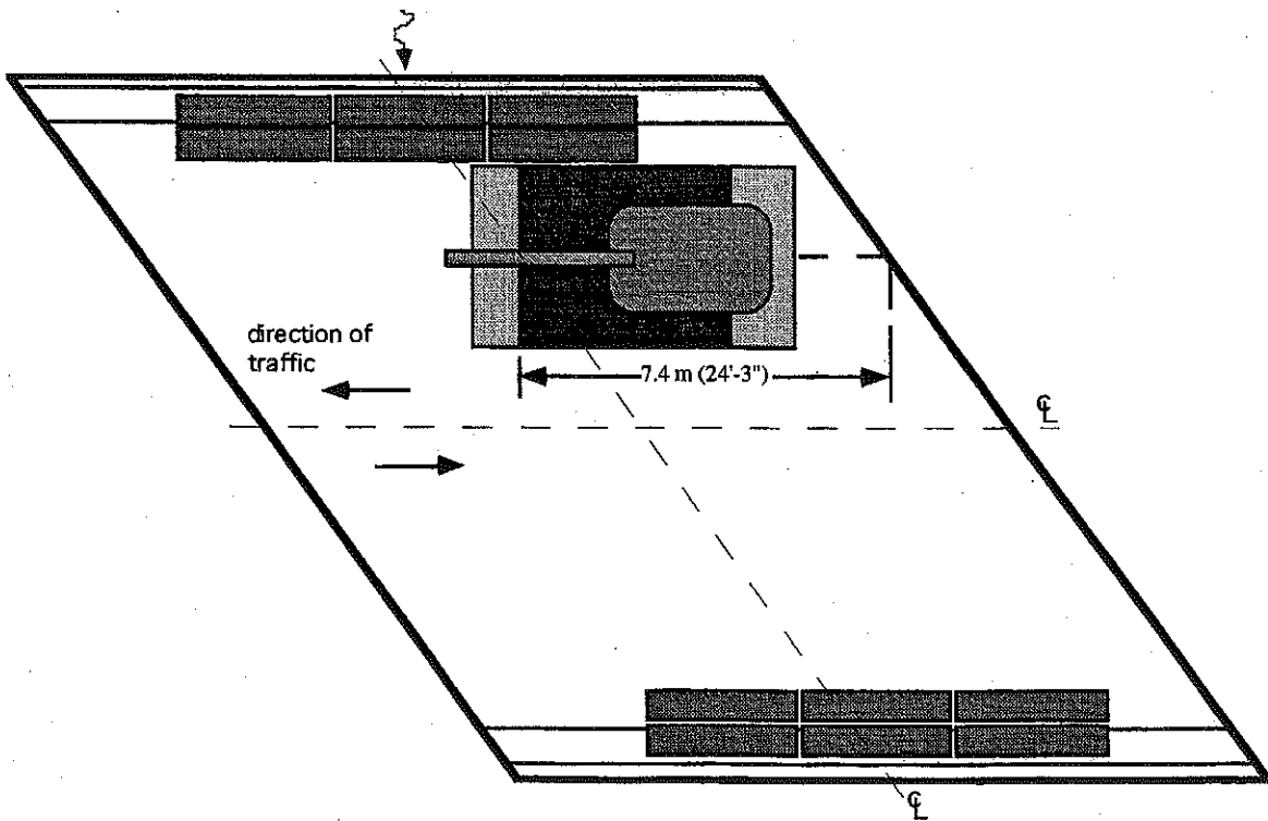
(b) Load Position 3 - Upstream Case.
