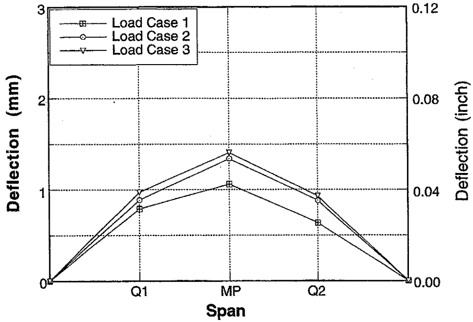
Figure A-130 Longitudinal Distribution of Deflections for Bridge No. 4, Girder 5 due to Upstream Loading.
