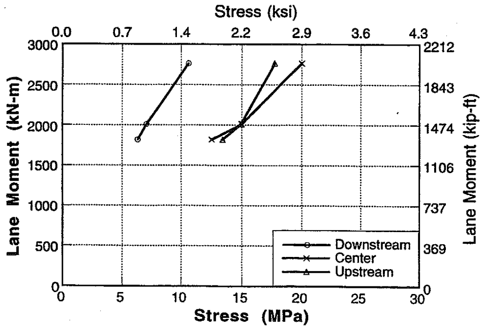
Figure A-60 : Stress vs Lane Moment for North Span of Bridge No. 3, Girder 4 and 5 at Mid Point.
