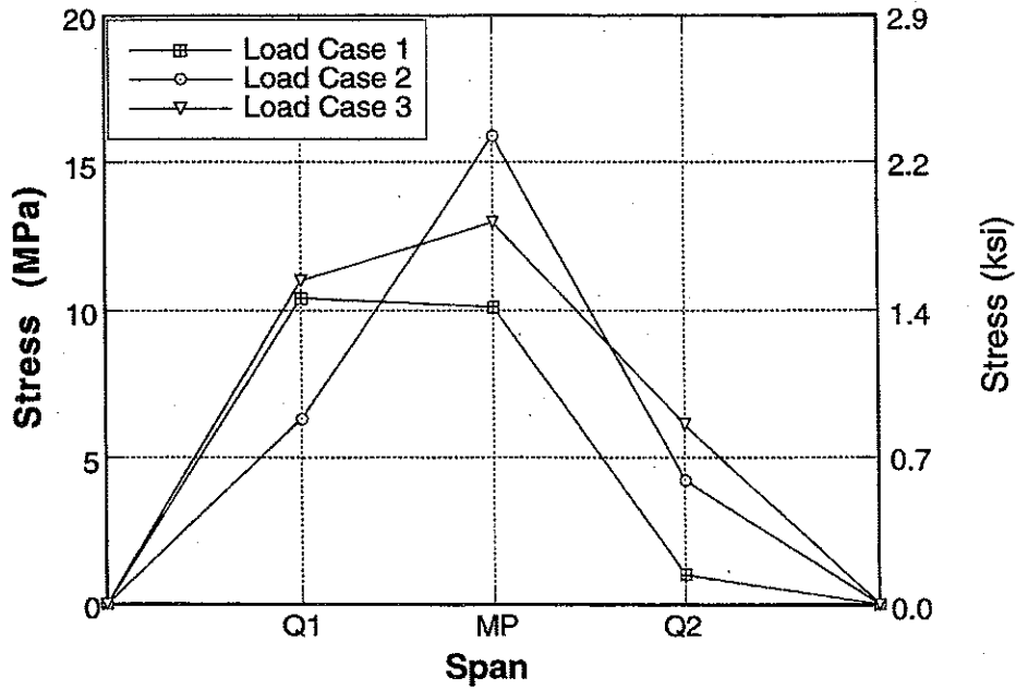
Figure A-156 : Longitudinal Distribution of Stresses for Bridge No. 4, Girder 6 due to Center Loading.
