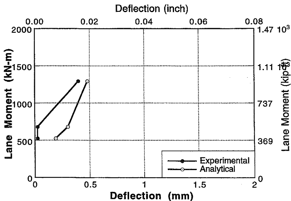
Figure A-179 : Experimental and Analytical Deflections for Bridge No. 5, Girder 7 and 8 for Lane 3 and 4 Loading.
