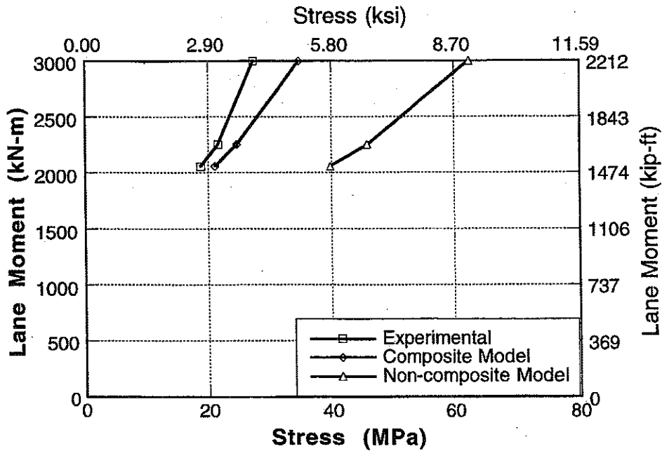
Figure A-96 : Experimental and Analytical Stresses for South Span of Bridge No. 3, Girder 2 and 3 for Upstream Loading.
