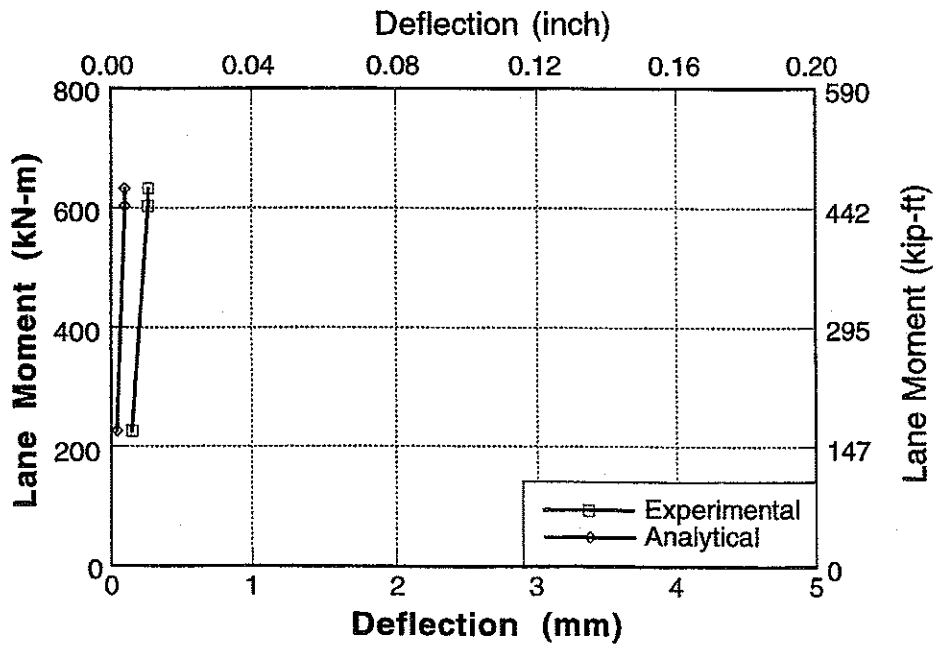
Figure A-9 : Experimental and Analytical Deflections for Bridge No. 1, Girder 5 and 6 for Center Loading.
