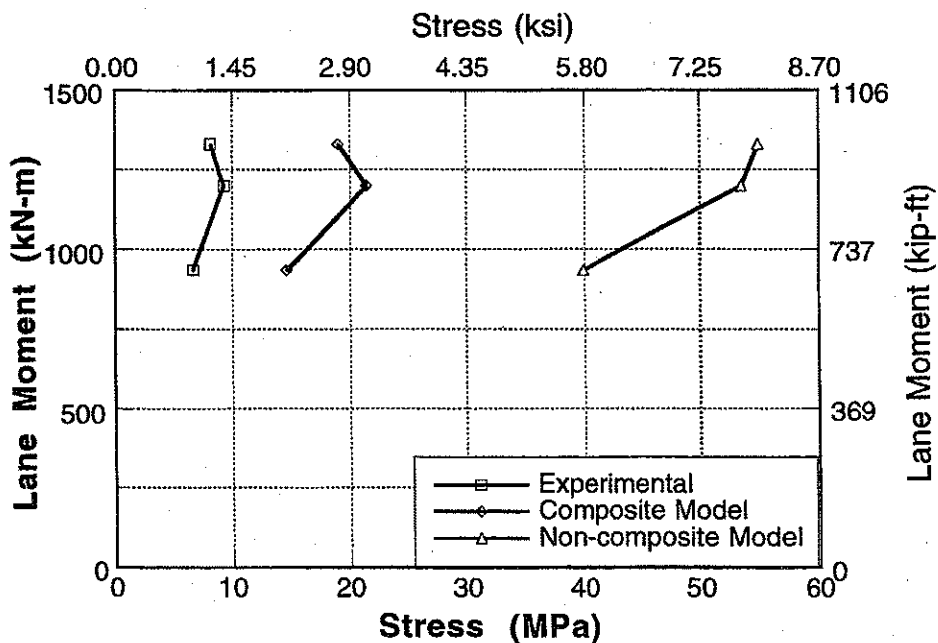
Figure A-137 : Experimental and Analytical Stresses for Bridge No. 4, Girder 8 and 9 for Downstream Loading.
