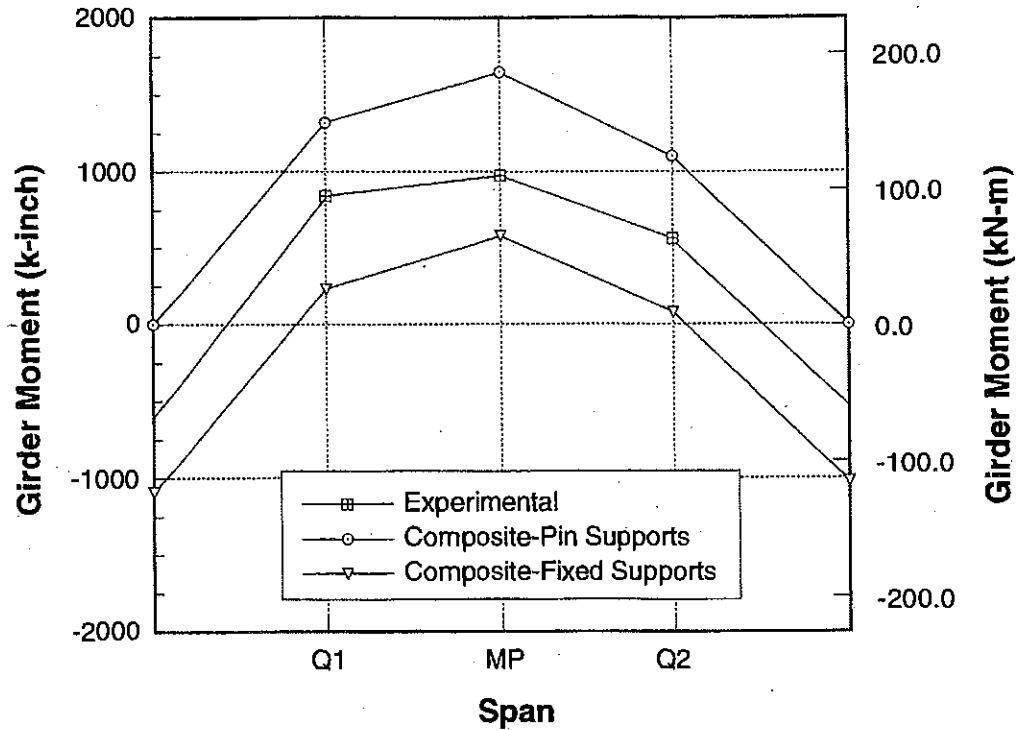
Figure 7-12 : Longitudinal Distribution of Stresses in Girder No. 9 due to the Downstream Loading on Bridge No. 2.
