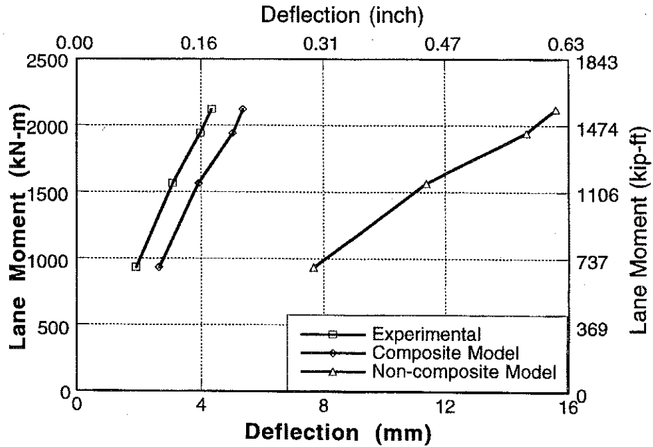
Figure A-28 : Experimental and Analytical Deflections for Bridge No. 2, Girder 2 and 3 for Upstream Loading.
