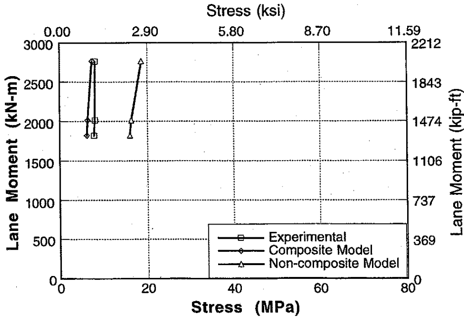
Figure A-74 : Experimental and Analytical Stresses for North Span of Bridge No. 3, Girder 8 and 9 for Upstream Loading.
