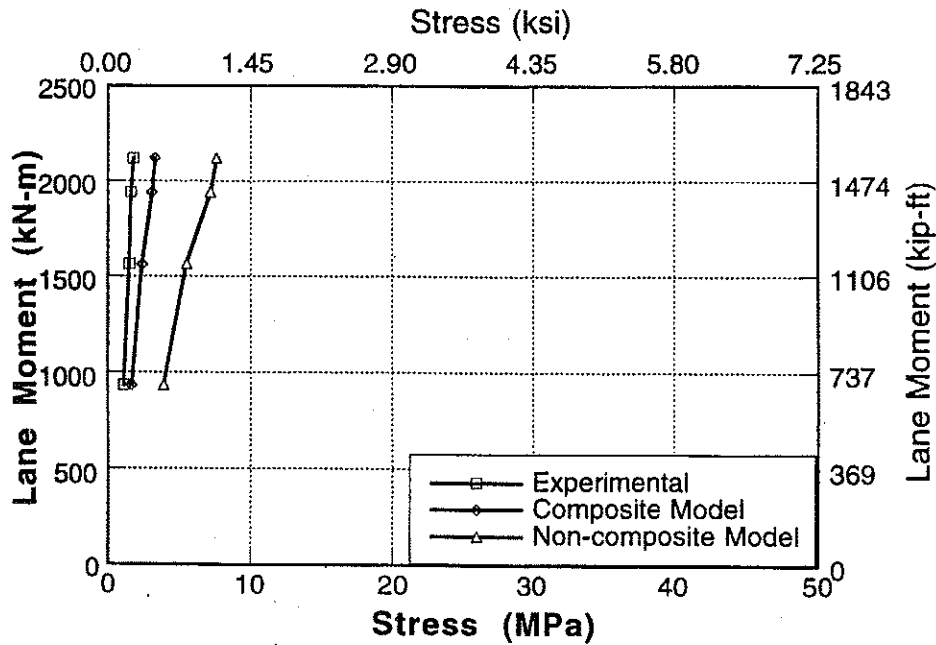
Figure A-49 : Experimental and Analytical Stresses for Bridge No. 2, Girder 8 and 9 for Upstream Loading.
