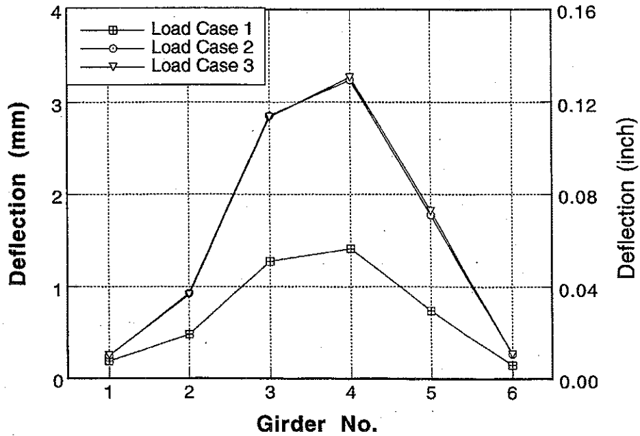
Figure A-14 Girder Distribution of Deflections for Bridge No. 1 due to Center Loading.
