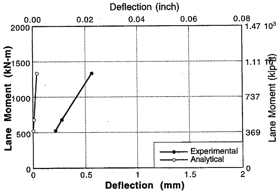
Figure A-175 : Experimental and Analytical Deflections for Bridge No. 5, Girder 9 for Lane 2 and 3 Loading.
