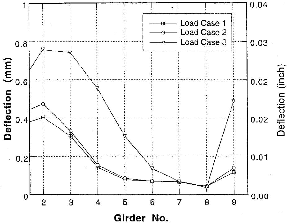
Figure 10-11 : Girder Distribution of Deflections for Loading in Lane 1 and 2.
