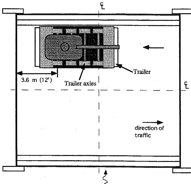
(b) Load Position 2 - Downstream Case.
