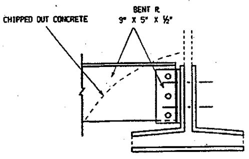
DIAPHRAGM DETAIL
