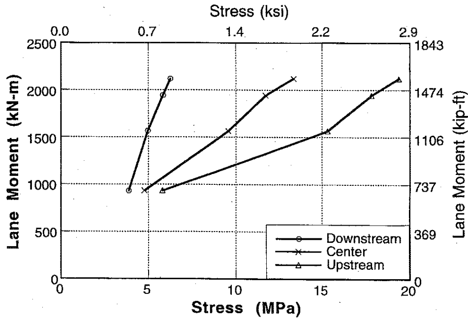
Figure A-38 : Stress vs Lane Moment for Bridge No. 2, Girder 2 and 3 at Mid Point.
