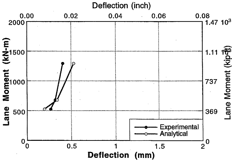
Figure A-177 : Experimental and Analytical Deflections for Bridge No. 5, Girder 3 and 4 for Lane 3 and 4 Loading.
