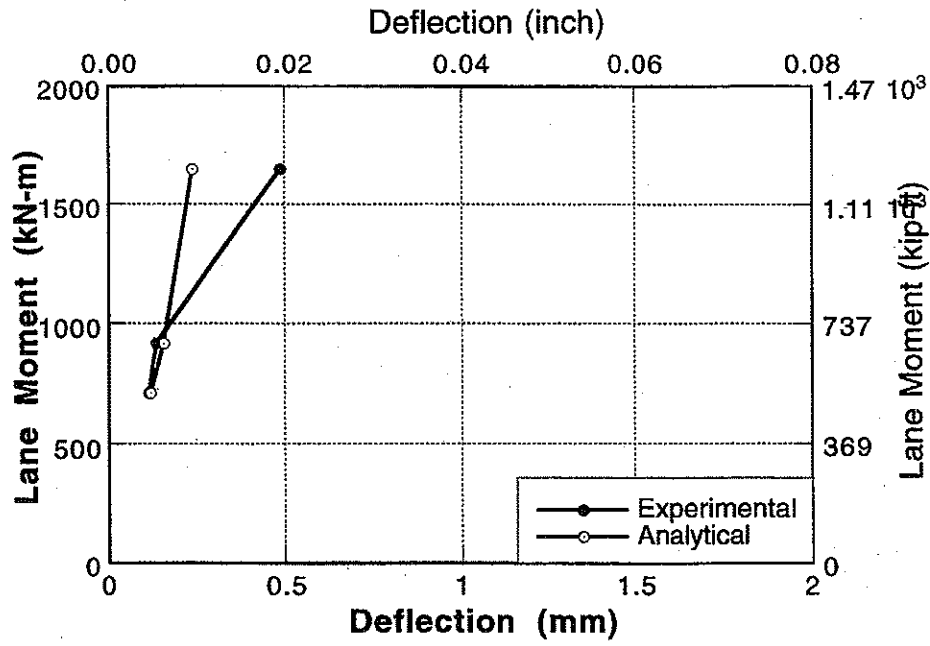
Figure A-170 : Experimental and Analytical Deflections for Bridge No. 5, Girder 9 for Lane 1 and 2 Loading.
