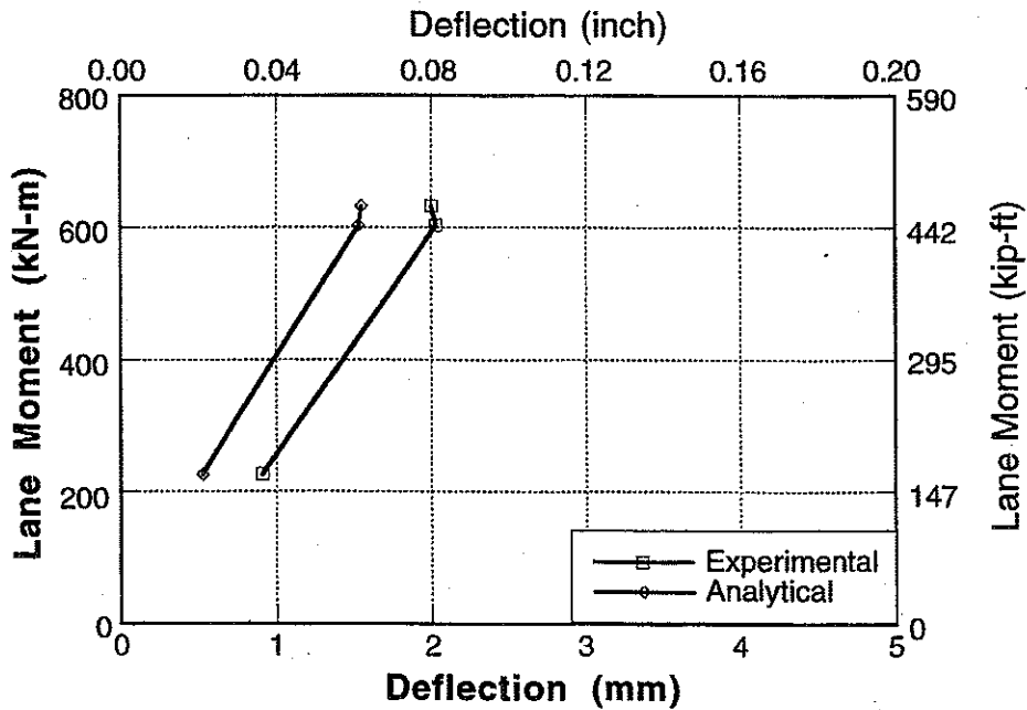
Figure A-11 : Experimental and Analytical Deflections for Bridge No. 1, Girder 3 and 4 for Upstream Loading.
