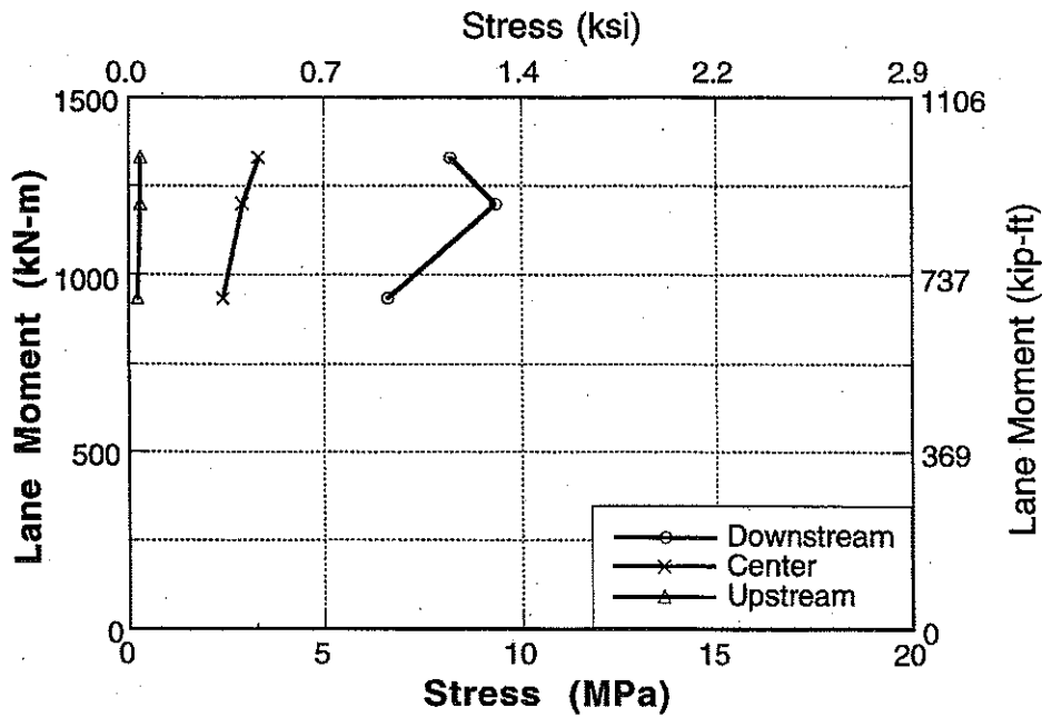
Figure A-134 : Stress vs Lane Moment for Bridge No. 4, Girder 8 and 9 at Mid Point.
