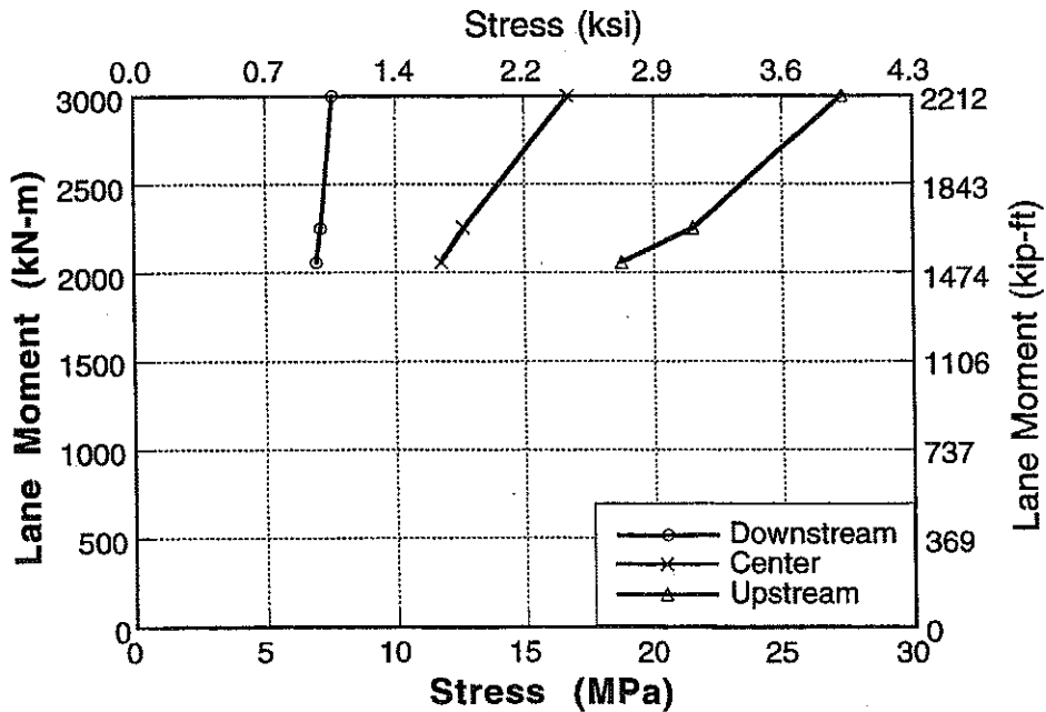
Figure A-84 : Stress vs Lane Moment for South Span of Bridge No. 3, Girder 2 and 3 at Mid Point.
