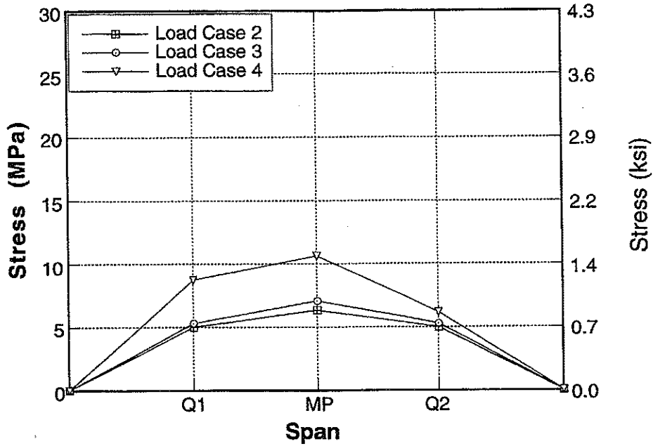
Figure A-78 : Longitudinal Distribution of Stresses for North Span of Bridge No. 3, Girder 5 due to Downstream Loading.
