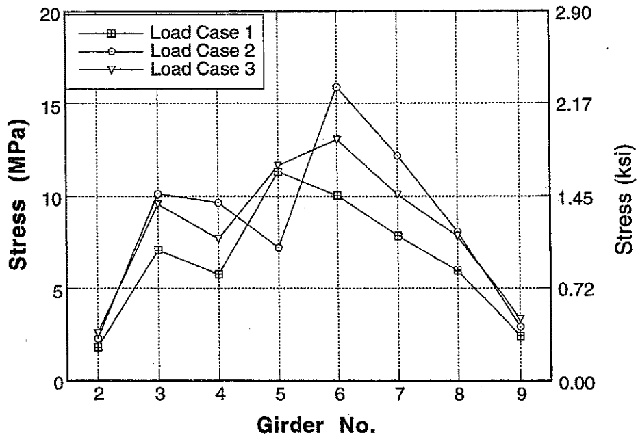
Figure A-147 : Girder Distribution of Stresses at Mid Point for Bridge No. 4 due to Center Loading.
