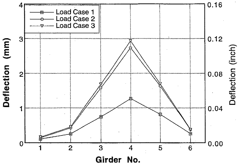
Figure 6-9 : Lateral Load Distribution for Downstream Loading on Bridge No. 1.
