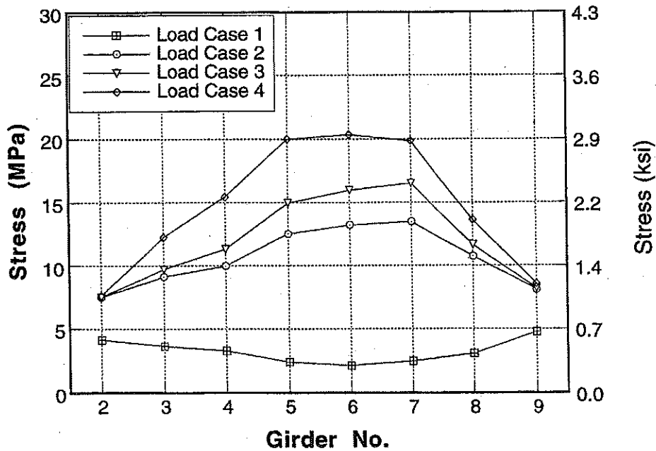
Figure A-76 : Girder Distribution of Stresses at Mid Point for North Span of Bridge No. 3 due to Center Loading.
