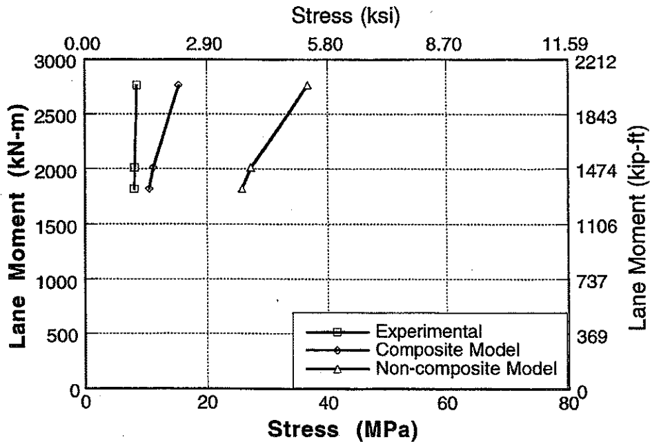
Figure A-70 : Experimental and Analytical Stresses for North Span of Bridge No. 3, Girder 8 and 9 for Center Loading.
