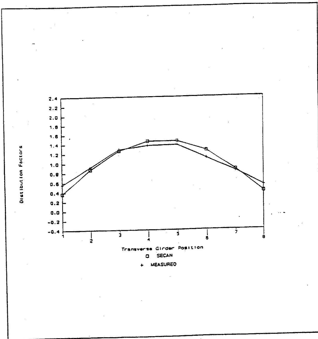
Figure 2.2/ Distribution Factors for Midspan Deflections (Central Load)
