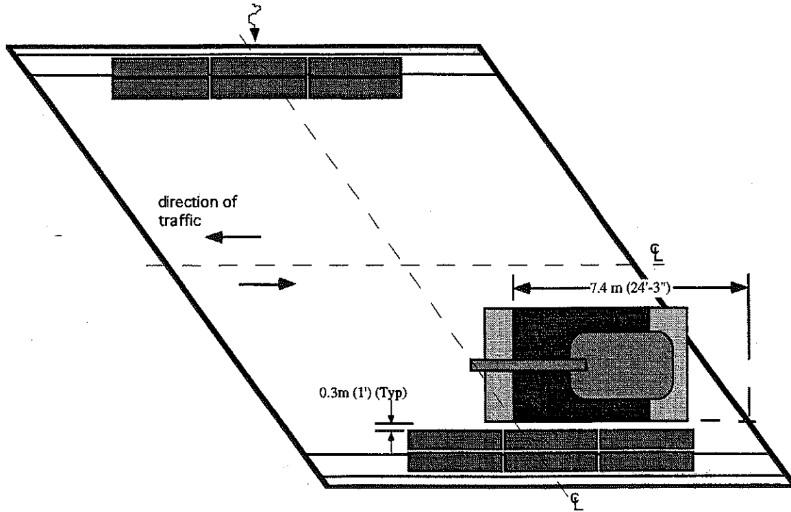
(b) Load Position 2 - Downstream Case.
