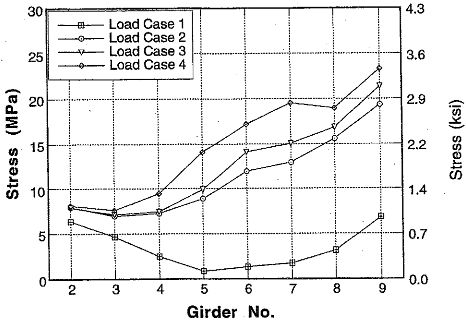
Figure A-100 : Girder Distribution of Stresses at Mid Point for South Span of Bridge No. 3 due to Downstream Loading.
