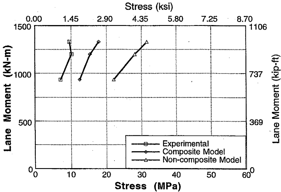
Figure A-138 : Experimental and Analytical Stresses for Bridge No. 4, Girder 2 and 3 for Center Loading.
