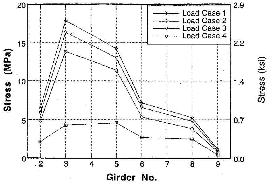
Figure A-52 : Girder Distribution of Stresses at Mid Point for Bridge No. 2 due to Upstream Loading.
