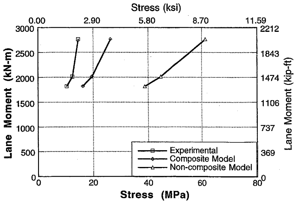
Figure A-66 : Experimental and Analytical Stresses for North Span of Bridge No. 3, Girder 8 and 9 for Downstream Loading.
