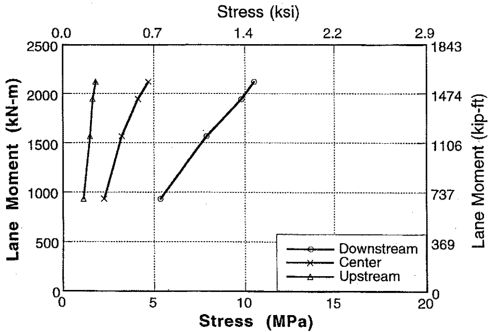
Figure A-40 : Stress vs Lane Moment for Bridge No. 2, Girder 8 and 9 at Mid Point.
