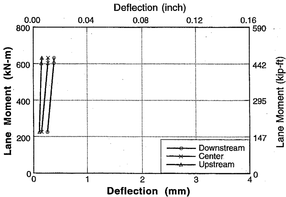
Figure A-3 : Deflection vs Lane Moment for Bridge No. 1, Girder 5 and 6.
