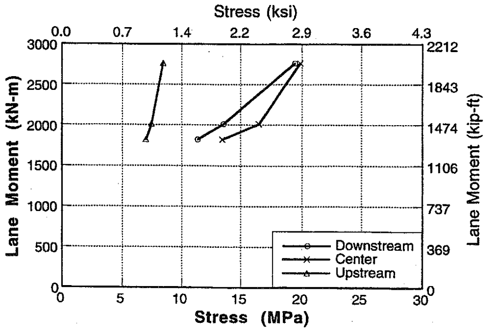
Figure A-61 : Stress vs Lane Moment for North Span of Bridge No. 3, Girder 6 and 7 at Mid Point.
