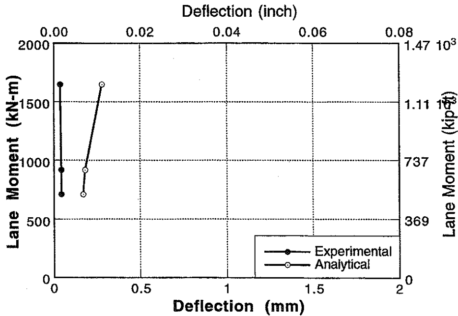
Figure A-169 : Experimental and Analytical Deflections for Bridge No. 5, Girder 7 and 8 for Lane 1 and 2 Loading.
