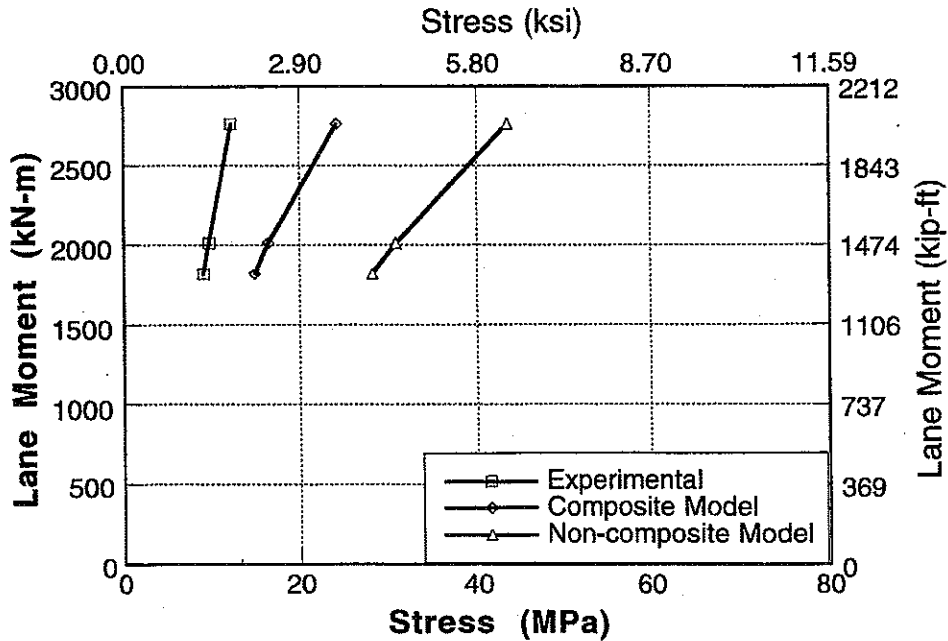
Figure A-67 : Experimental and Analytical Stresses for North Span of Bridge No. 3, Girder 2 and 3 for Center Loading.
