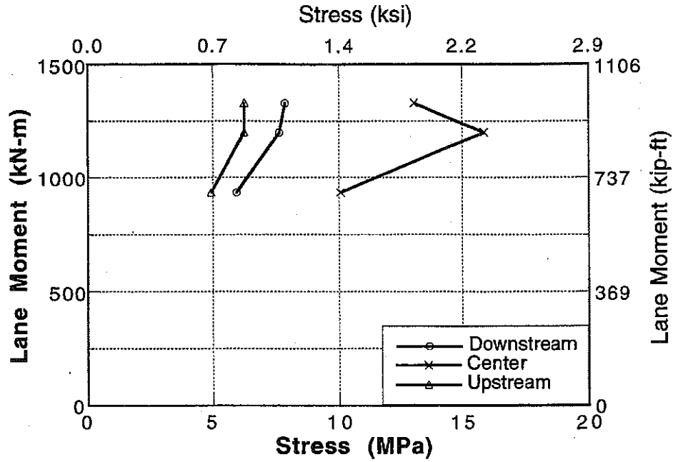
Figure 9-10 : Stresses at Mid-Span of Girder 6 of Bridge No. 4
