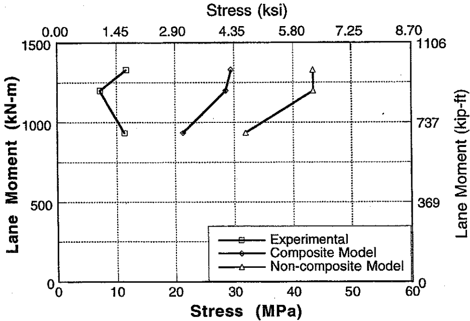
Figure A-139 : Experimental and Analytical Stresses for Bridge No. 4, Girder 4 and 5 for Center Loading.
