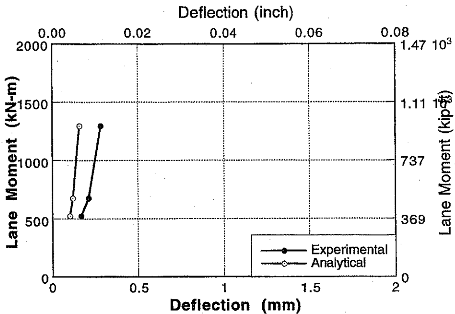
Figure A-180 : Experimental and Analytical Deflections for Bridge No. 5, Girder 9 for Lane 3 and 4 Loading.
