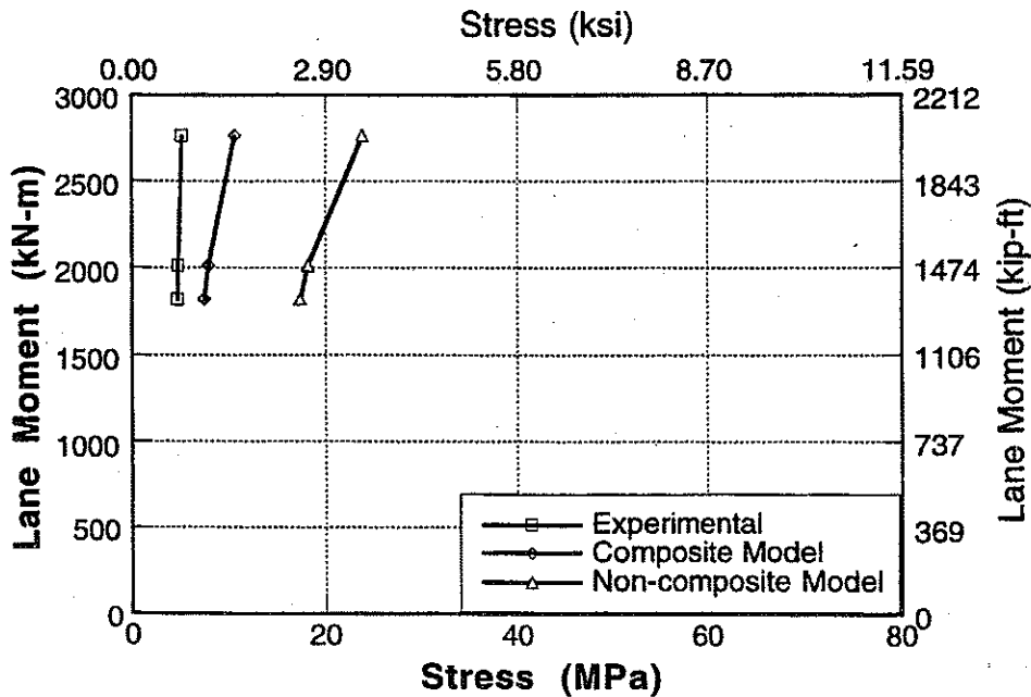
Figure A-63 : Experimental and Analytical Stresses for North Span of Bridge No. 3, Girder 2 and 3 for Downstream Loading.
