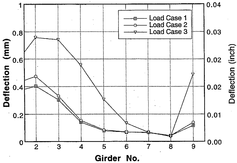
Figure A-186: Girder Distribution of Deflections for Bridge No. 5 due to Loading in Lane 1 and 2.
