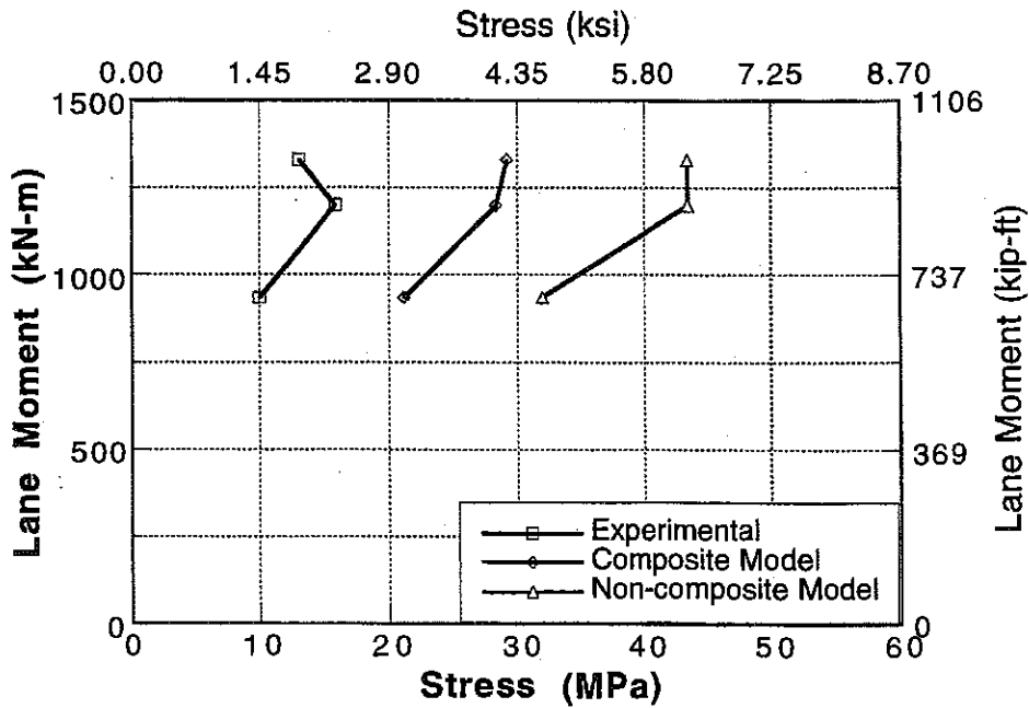
Figure 9-11 : Stresses at Mid-span of Girder 6 for Center Loading on Bridge No. 4.
