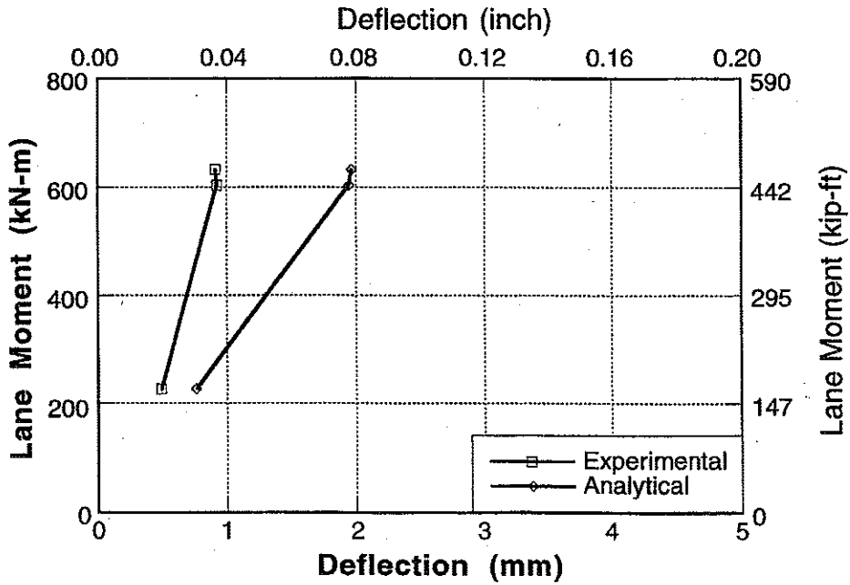
Figure A-7 : Experimental and Analytical Deflections for Bridge No. 1, Girder 1 and 2 for Center Loading.
