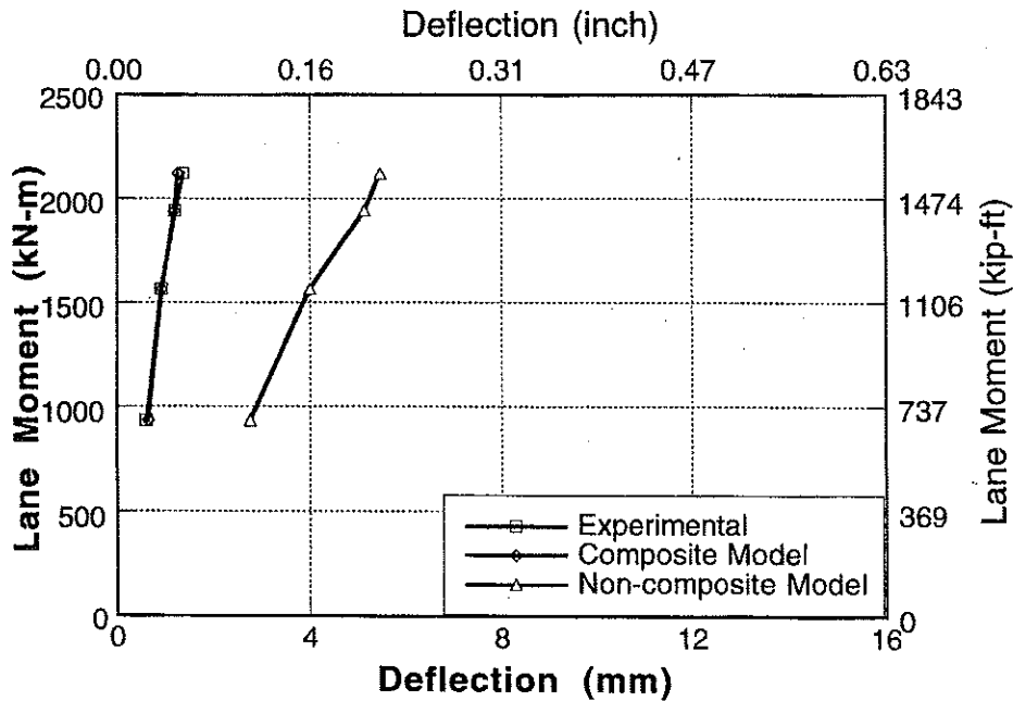
Figure A-27 : Experimental and Analytical Deflections for Bridge No. 2, Girder 8 and 9 for Center Loading.
