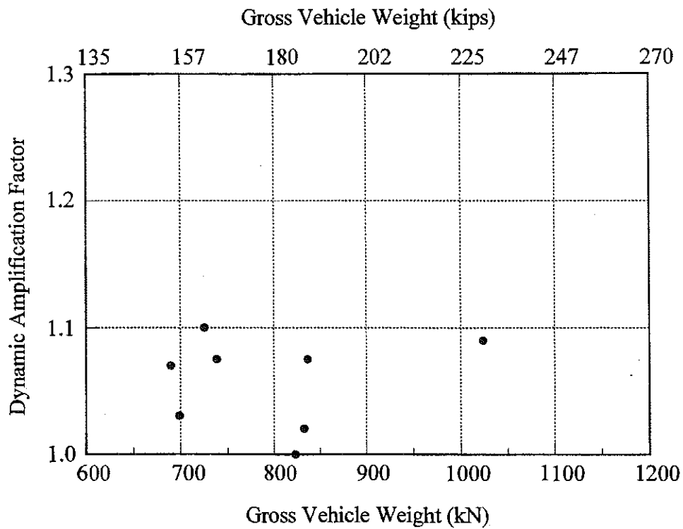
Figure 3-2 : Impact Factors for Heavy Vehicles (Nassif and Nowak, 1995).
