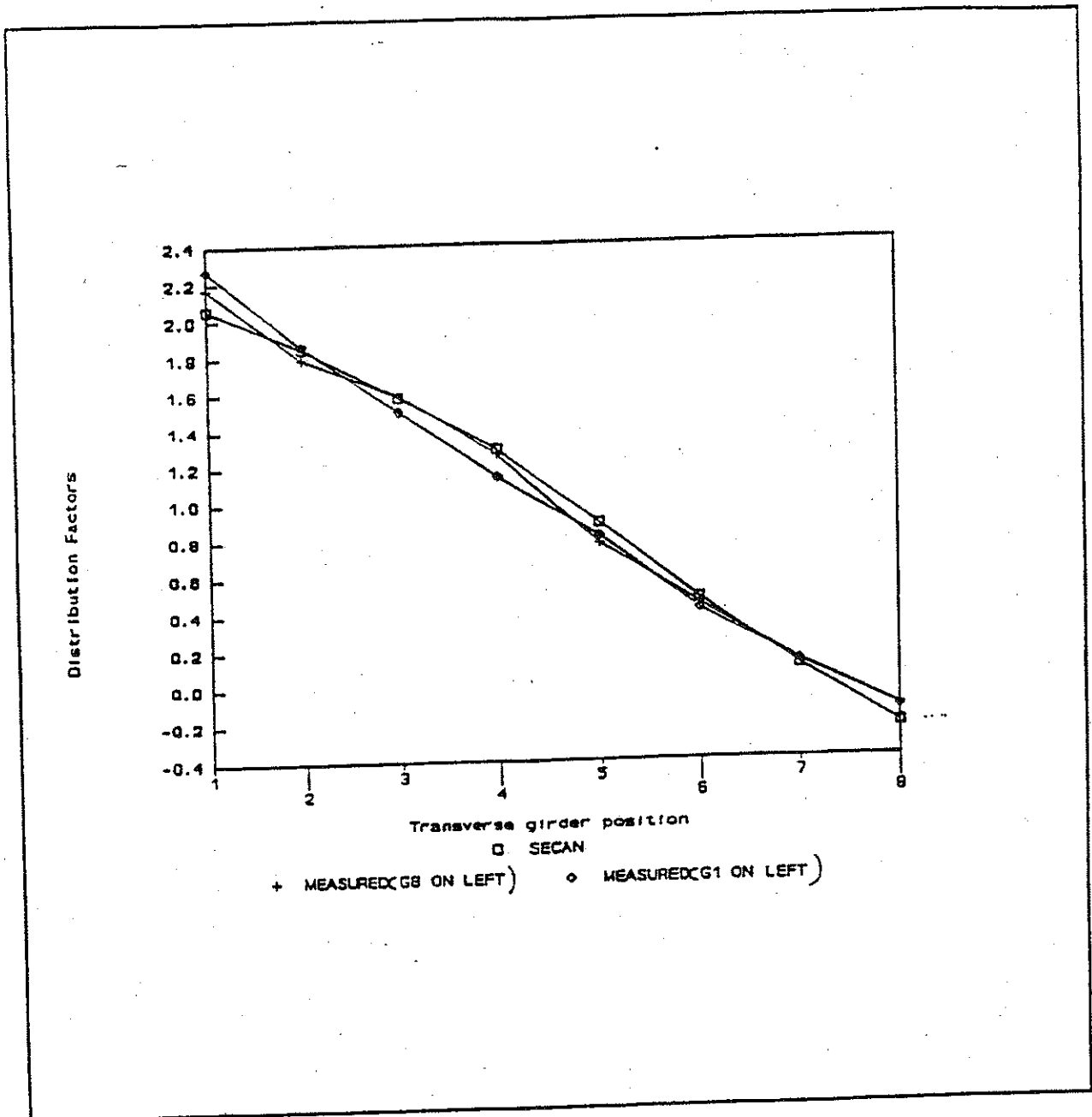
Figure 2.3/ Distribution Factors for Midspan Deflection (Eccentric load)
