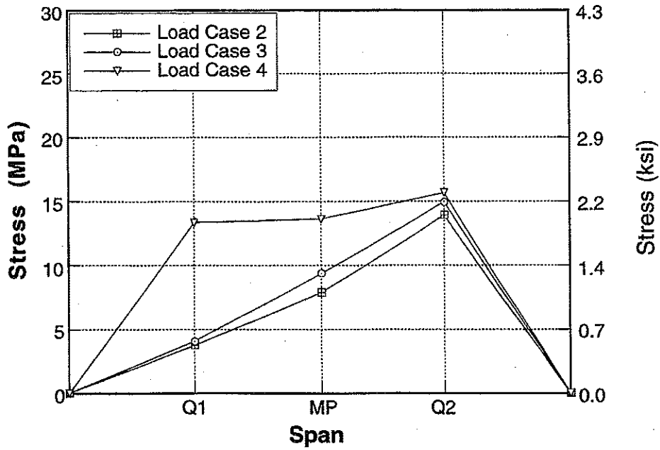
Figure A-81 : Longitudinal Distribution of Stresses for North Span of Bridge No. 3, Girder 6 due to Downstream Loading.
