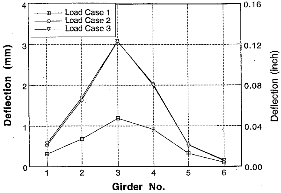
Figure A-15 : Girder Distribution of Deflections for Bridge No. 1 due to Upstream Loading.
