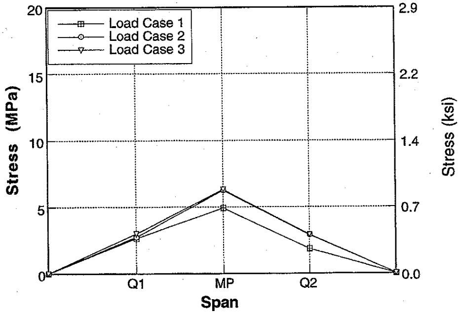
Figure A-157 : Longitudinal Distribution of Stresses for Bridge No. 4, Girder 6 due to Upstream Loading.
