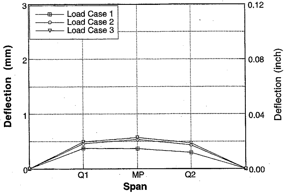
Figure A-128 : Longitudinal Distribution of Deflections for Bridge No. 4, Girder 5 due to Downstream Loading.
