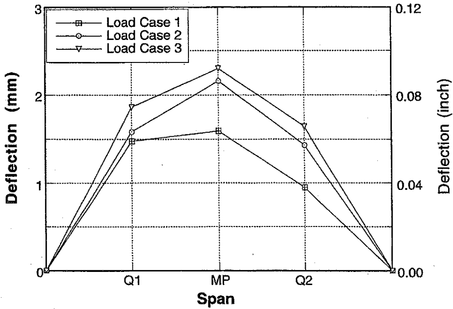
Figure A-129 : Longitudinal Distribution of Deflections for Bridge No. 4, Girder 5 due to Center Loading.
