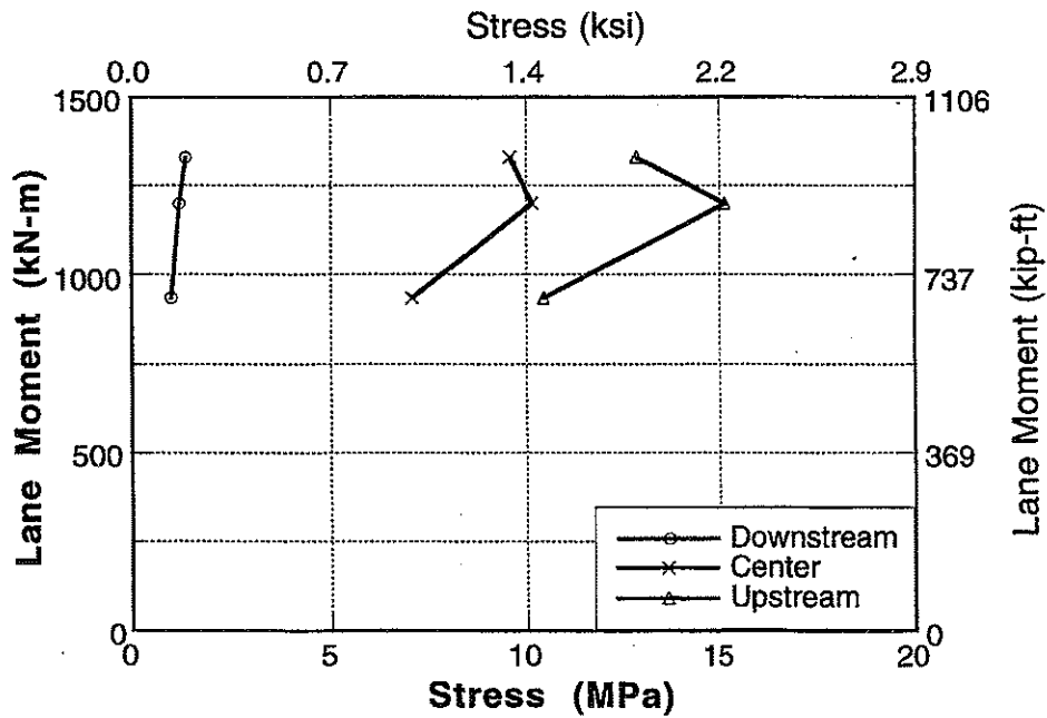
Figure A-131 : Stress vs Lane Moment for Bridge No. 4, Girder 2 and 3 at Mid Point.
