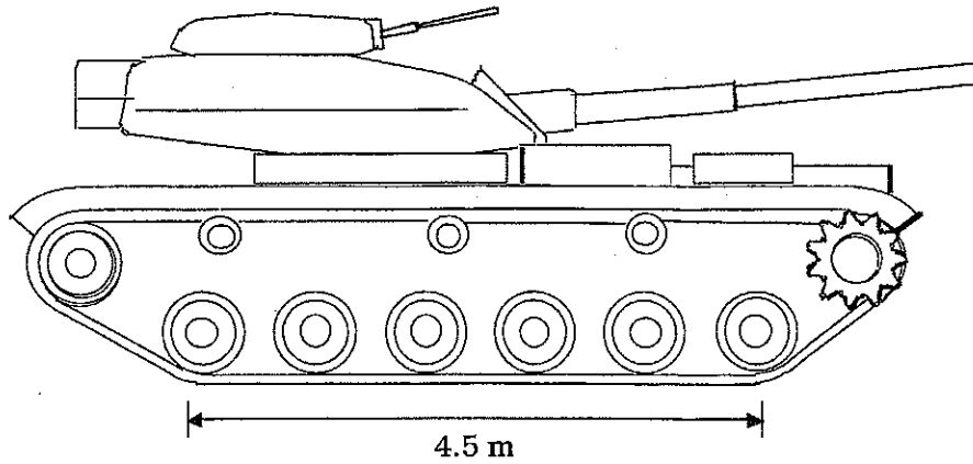
Figure 3-4 : Side Elevation of M-60 Tank.
