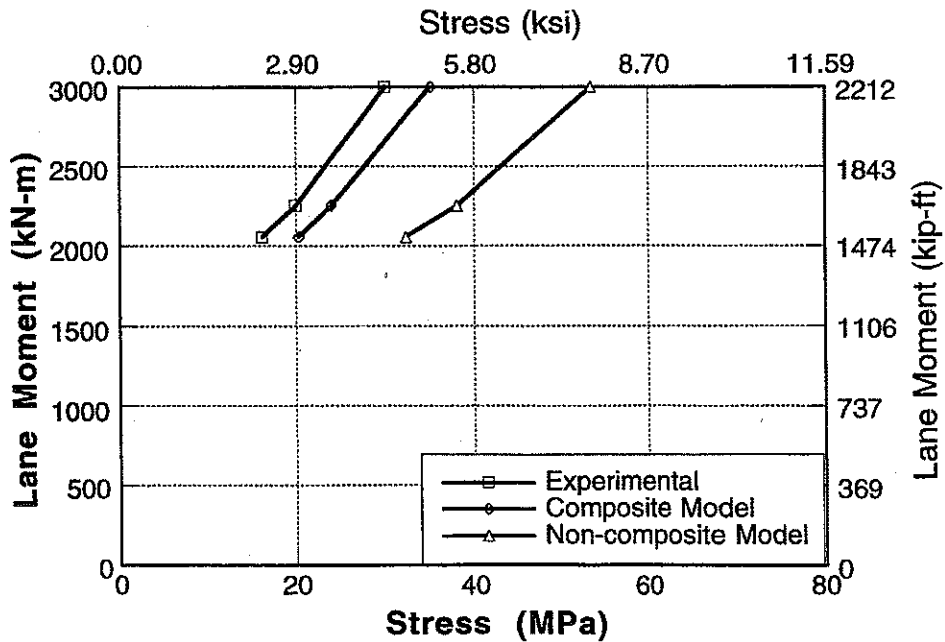
Figure A-93 : Experimental and Analytical Stresses for South Span of Bridge No. 3, Girder 4 and 5 for Center Loading.
