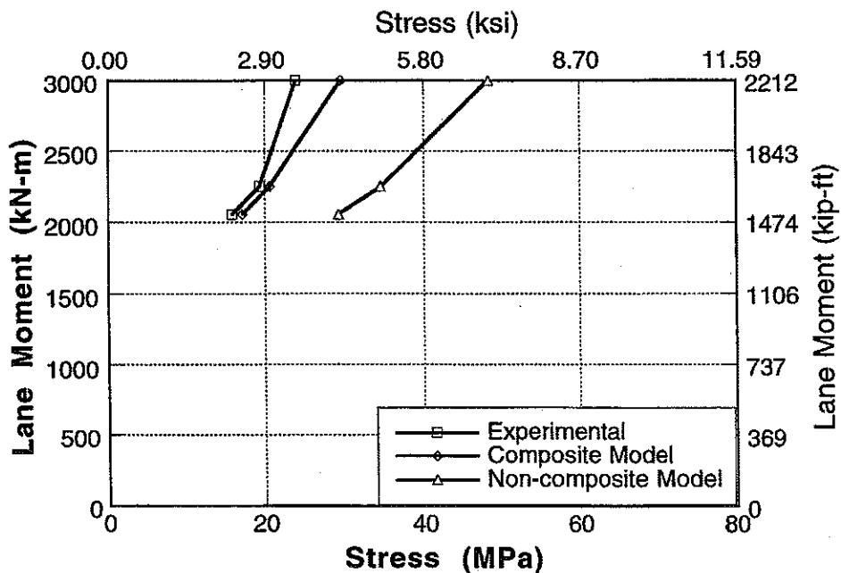
Figure A-97 : Experimental and Analytical Stresses for South Span of Bridge No. 3, Girder 4 and 5 for Upstream Loading.
