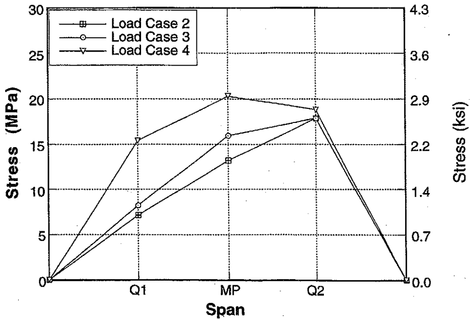
Figure A-82 : Longitudinal Distribution of Stresses for North Span of Bridge No. 3, Girder 6 due to Center Loading.
