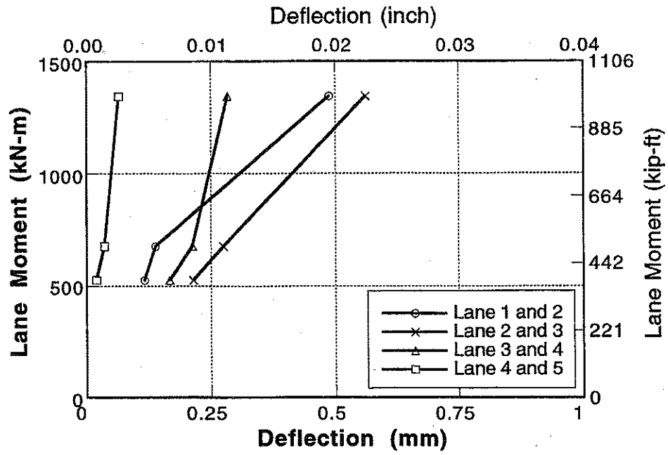
Figure A-165 : Deflection vs Lane Moment for Bridge No. 5, Girder 9.
