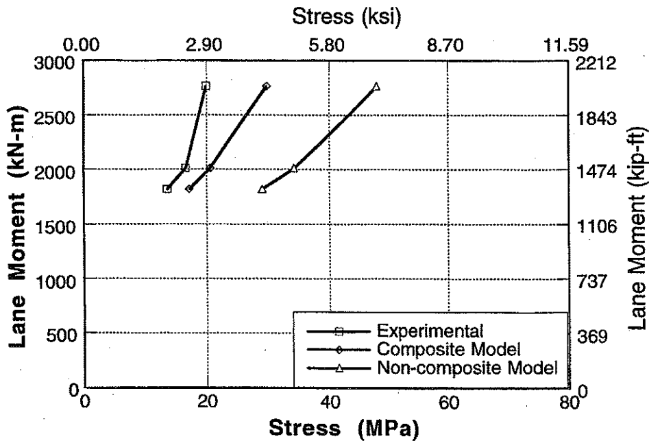
Figure A-69 : Experimental and Analytical Stresses for North Span of Bridge No. 3, Girder 6 and 7 for Center Loading.
