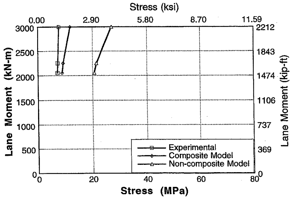
Figure A-88 : Experimental and Analytical Stresses for South Span of Bridge No. 3, Girder 2 and 3 for Downstream Loading.
