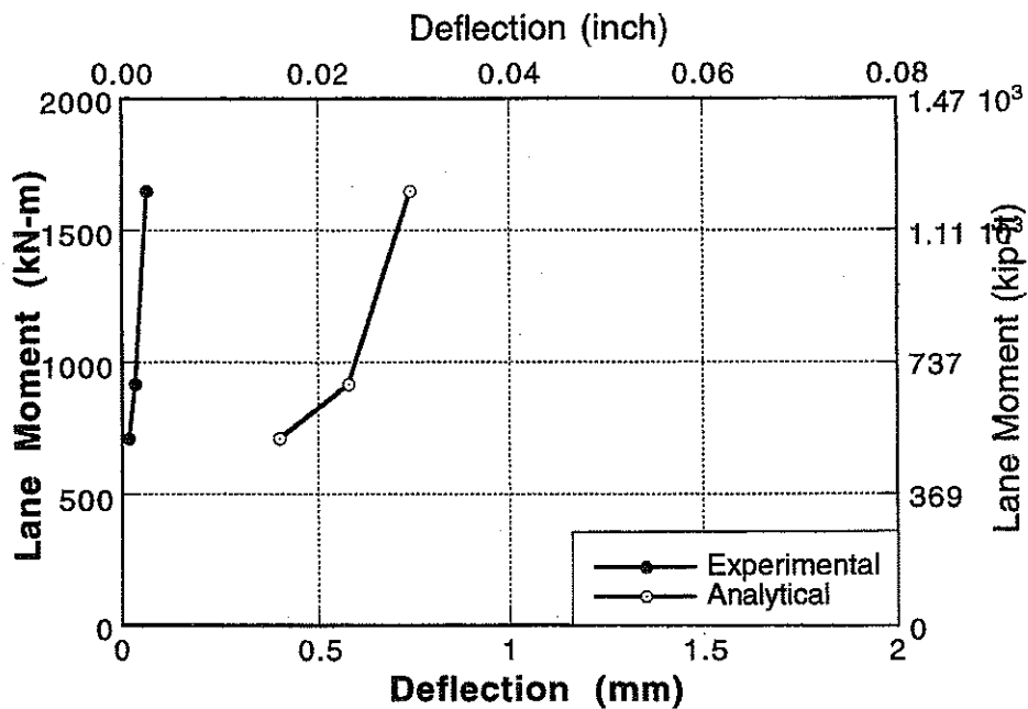
Figure A-185 : Experimental and Analytical Deflections for Bridge No. 5, Girder 9 for Lane 4 and 5 Loading.
