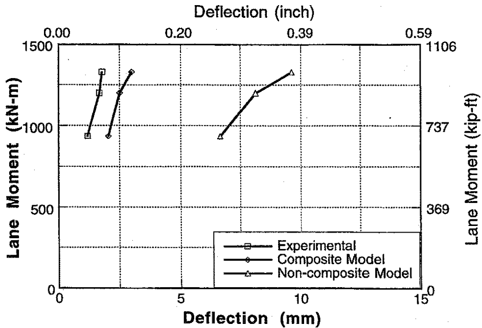
Figure A-117 : Experimental and Analytical Deflections for Bridge No. 4, Girder 3 and 4 for Center Loading.
