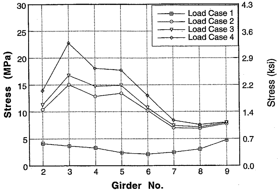
Figure A-77 : Girder Distribution of Stresses at Mid Point for North Span of Bridge No. 3 due to Upstream Loading.
