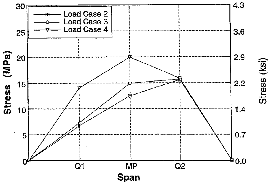
Figure A-79 : Longitudinal Distribution of Stresses for North Span of Bridge No. 3, Girder 5 due to Center Loading.
