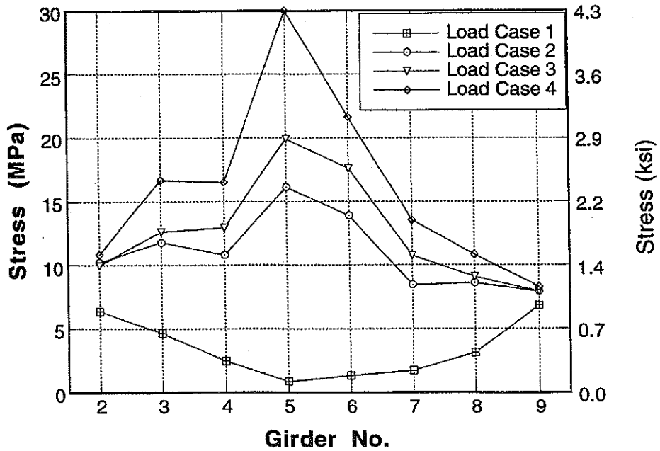
Figure A-101 : Girder Distribution of Stresses at Mid Point for South Span of Bridge No. 3 due to Center Loading.
