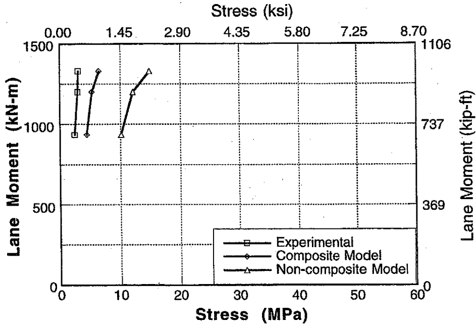
Figure A-144 : Experimental and Analytical Stresses for Bridge No. 4, Girder 6 and 7 for Upstream Loading.
