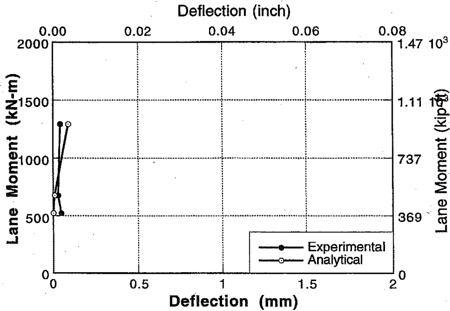
Figure A-176 : Experimental and Analytical Deflections for Bridge No. 5, Girder 1 and 2 for Lane 3 and 4 Loading.
