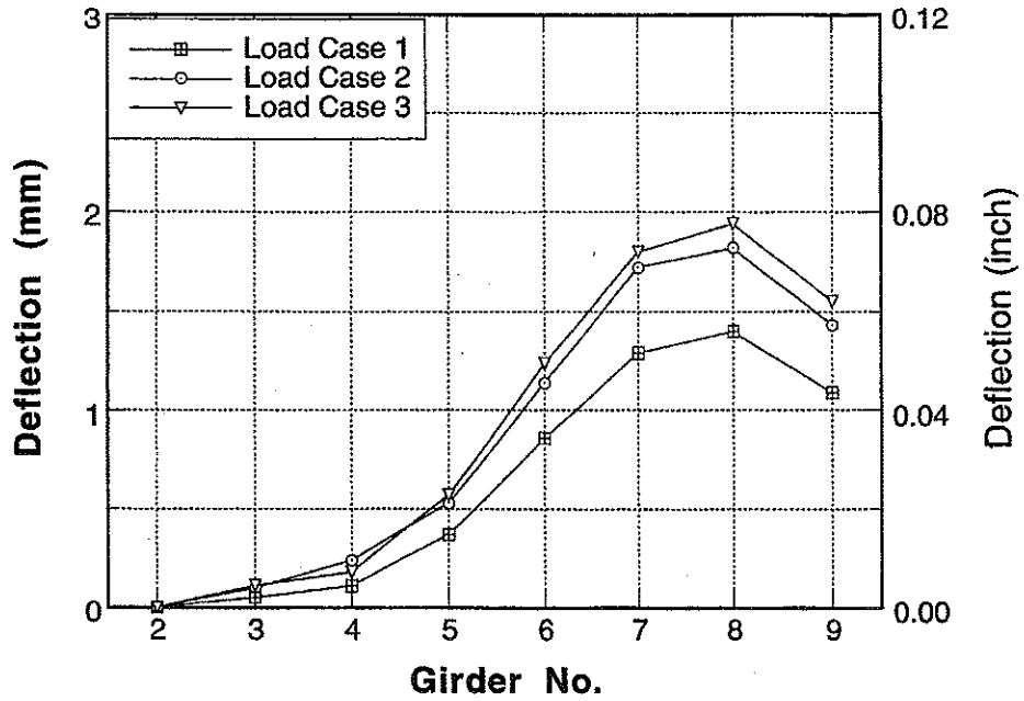
Figure A-125 : Girder Distribution of Deflections for Bridge No. 4 due to Downstream Loading.
