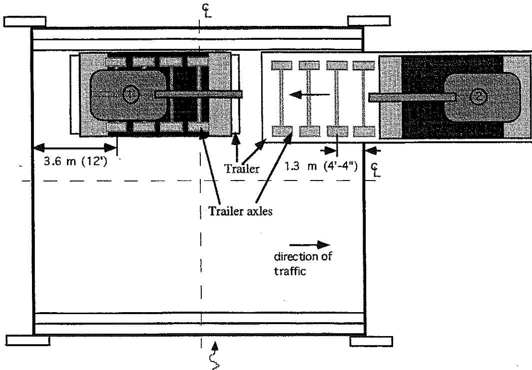
(c) Load Position 3 - Downstream Case.
