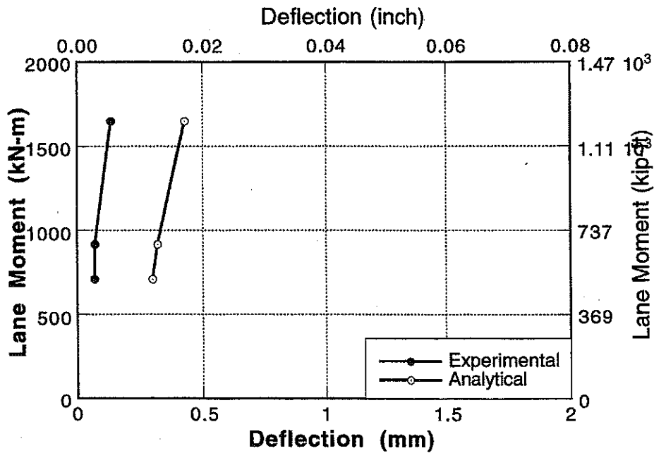
Figure A-168 : Experimental and Analytical Deflections for Bridge No. 5, Girder 5 and 6 for Lane 1 and 2 Loading.
