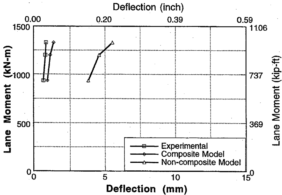
Figure A-122 : Experimental and Analytical Deflections for Bridge No. 4, Girder 5 and 6 for Upstream Loading.
