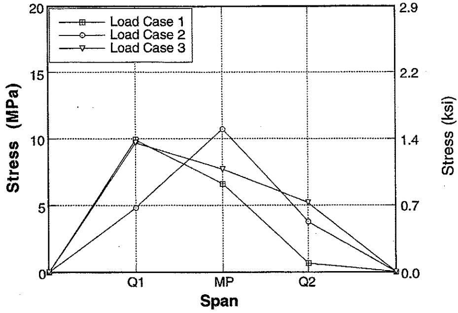
Figure A-151 : Longitudinal Distribution of Stresses for Bridge No. 4, Girder 4 due to Upstream Loading.
