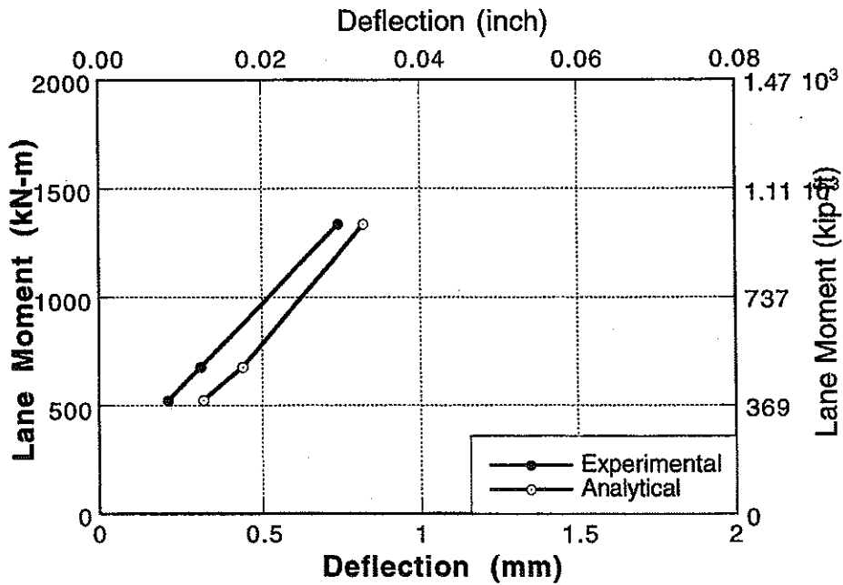
Figure A-172 : Experimental and Analytical Deflections for Bridge No. 5, Girder 3 and 4 for Lane 2 and 3 Loading.
