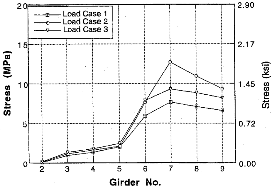
Figure 9-13 : Girder Distribution of Stresses due to Downstream Loading on Bridge No. 4.
