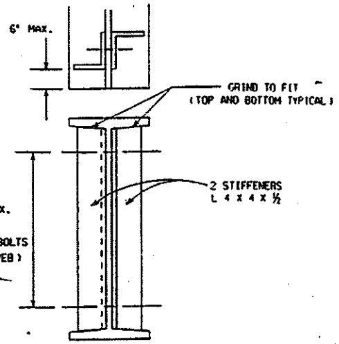
STIFFENER DETAIL [S]
