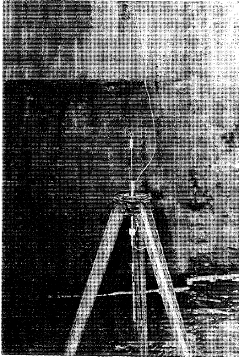
Figure 4-1 : Typical LVDT Setup.
