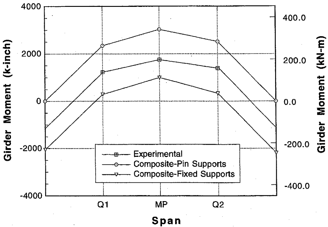
Figure 8-13 : Longitudinal Distribution of Stresses in Girder No. 5 due to the Center Loading on Bridge No. 3 - North Span.
