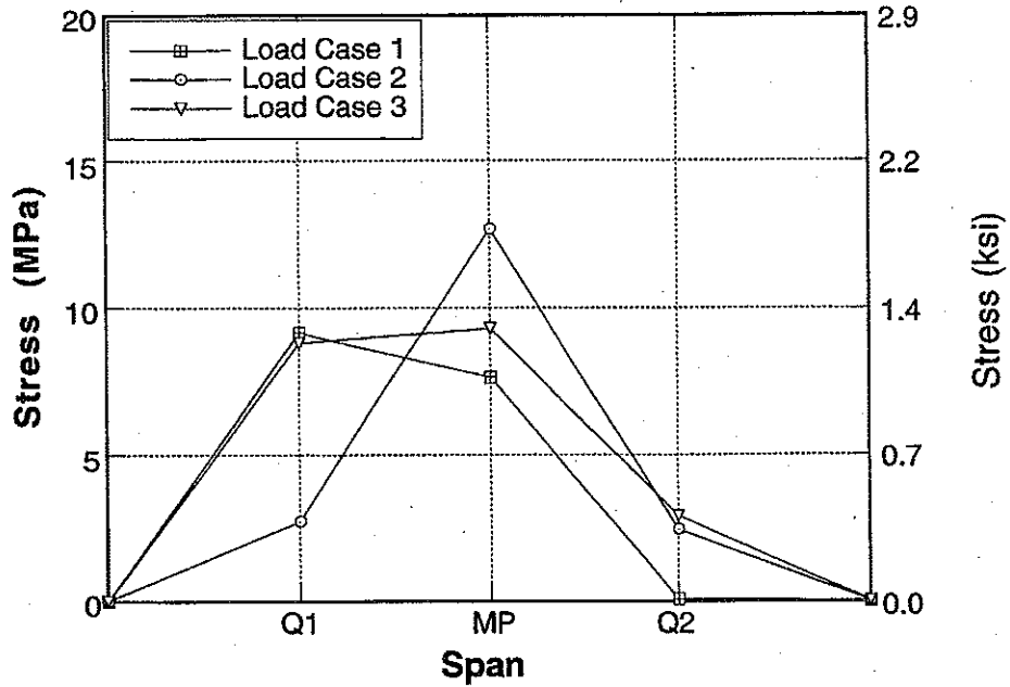
Figure A-158 : Longitudinal Distribution of Stresses for Bridge No. 4, Girder 7 due to Downstream Loading.
