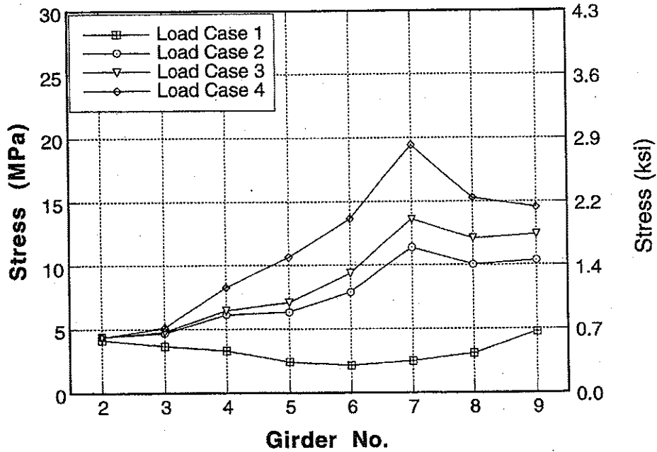
Figure A-75 : Girder Distribution of Stresses at Mid Point for North Span of Bridge No. 3 due to Downstream Loading.
