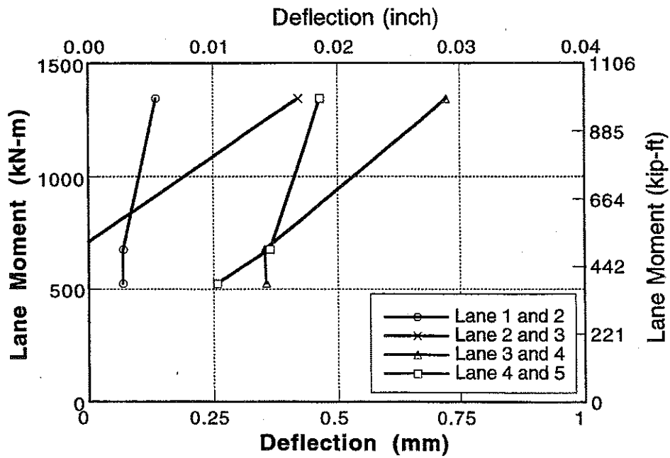
Figure A-163 : Deflection vs Lane Moment for Bridge No. 5, Girder 5 and 6.
