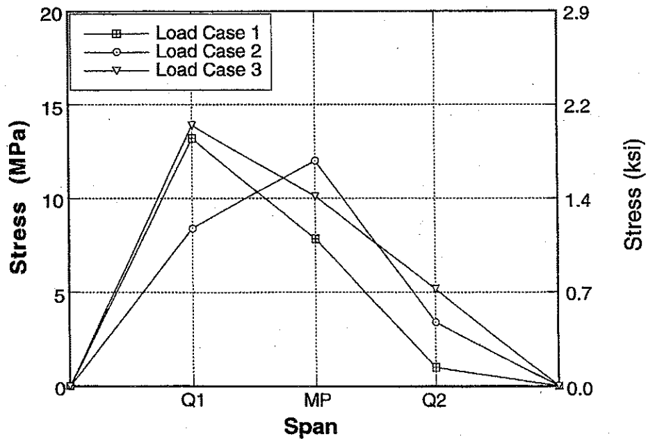
Figure A-159 : Longitudinal Distribution of Stresses for Bridge No. 4, Girder 7 due to Center Loading.
