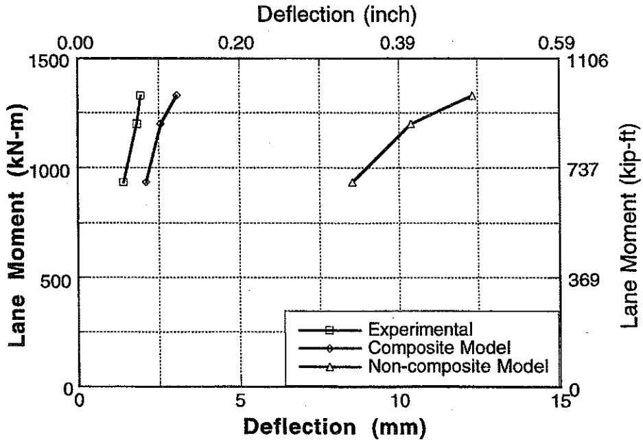
Figure A-115 : Experimental and Analytical Deflections for Bridge No. 4, Girder 7 and 8 for Downstream Loading.
