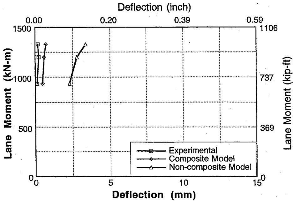
Figure A-113 : Experimental and Analytical Deflections for Bridge No. 4, Girder 3 and 4 for Downstream Loading.
