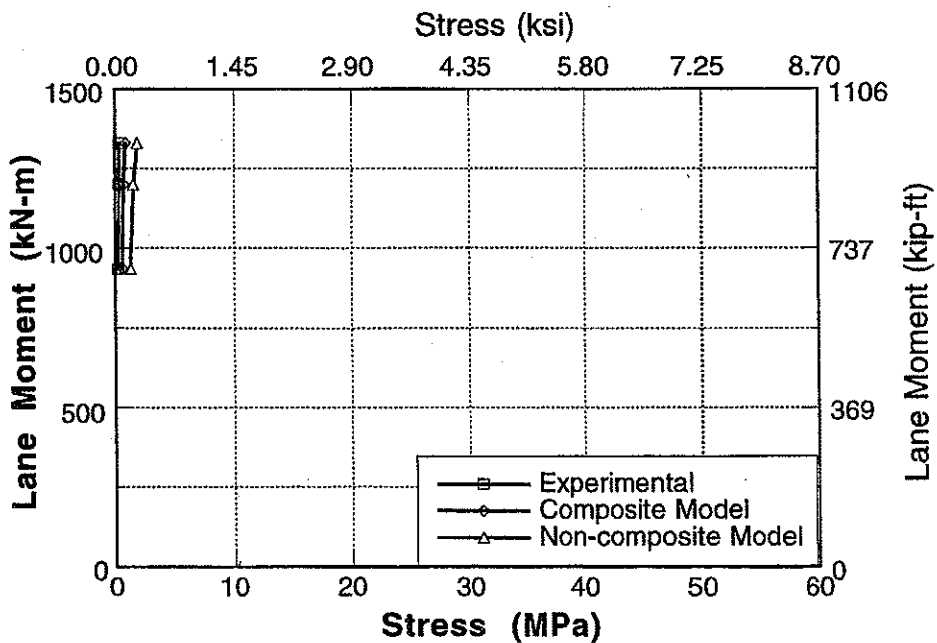
Figure A-145 : Experimental and Analytical Stresses for Bridge No. 4, Girder 8 and 9 for Upstream Loading.
