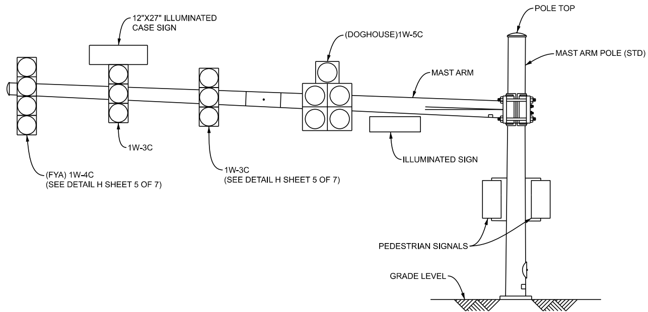
A DETAIL - TYPICAL SIGNAL DISPLAYS N.T.S.
