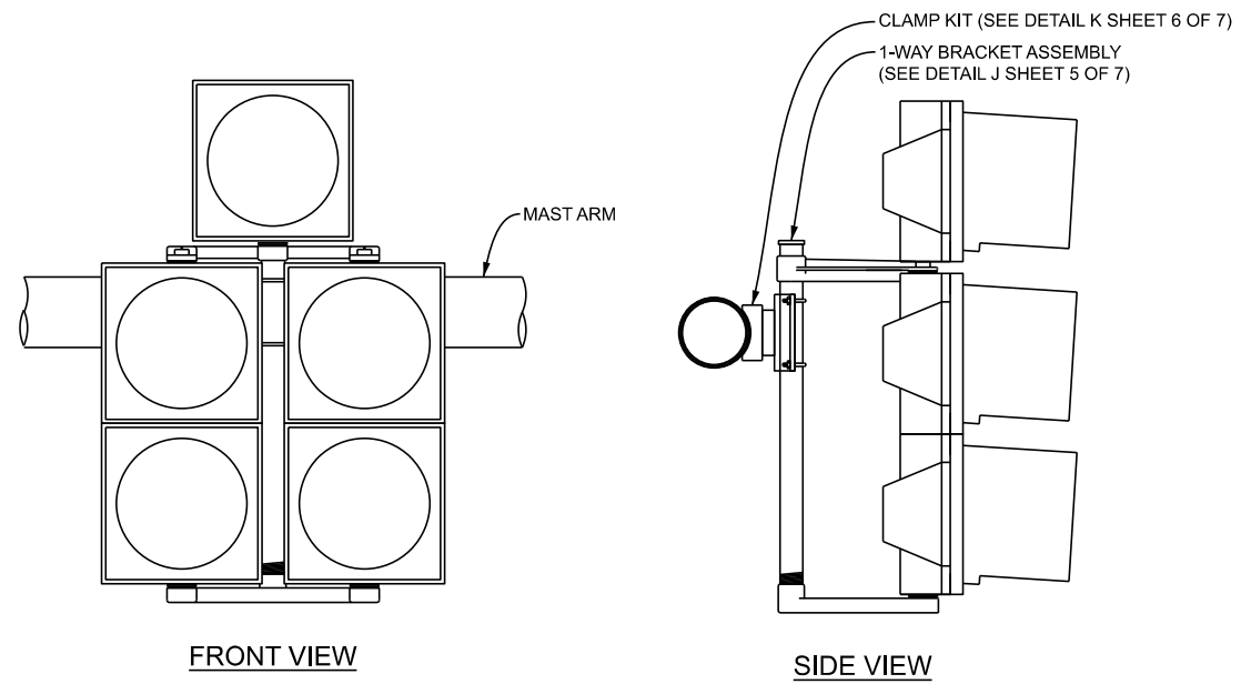
F DETAIL - 1W-5C (DOGHOUSE) N.T.S.
