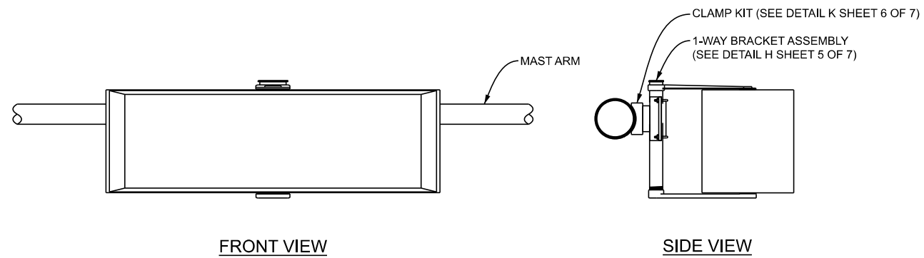
L DETAIL - 1W-ILLUMINATED STREET NAME SIGN N.T.S.
