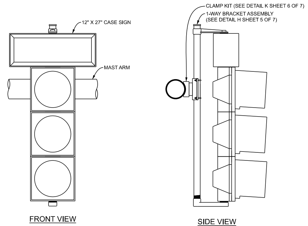
D DETAIL - 1W-3C WITH 12\"/>
