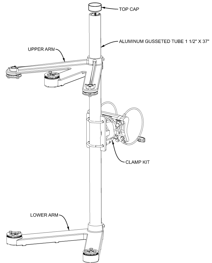
J DETAIL - 1-WAY 5-SECTION CLUSTER BRACKET ARM ASSEMBLY N.T.S.
