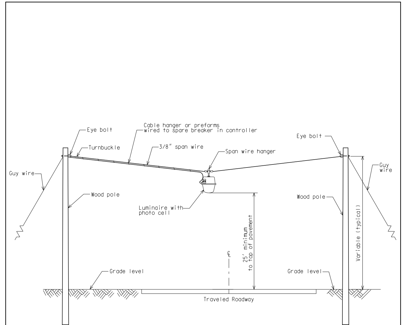
OVERHEAD LIGHTING DETAIL
