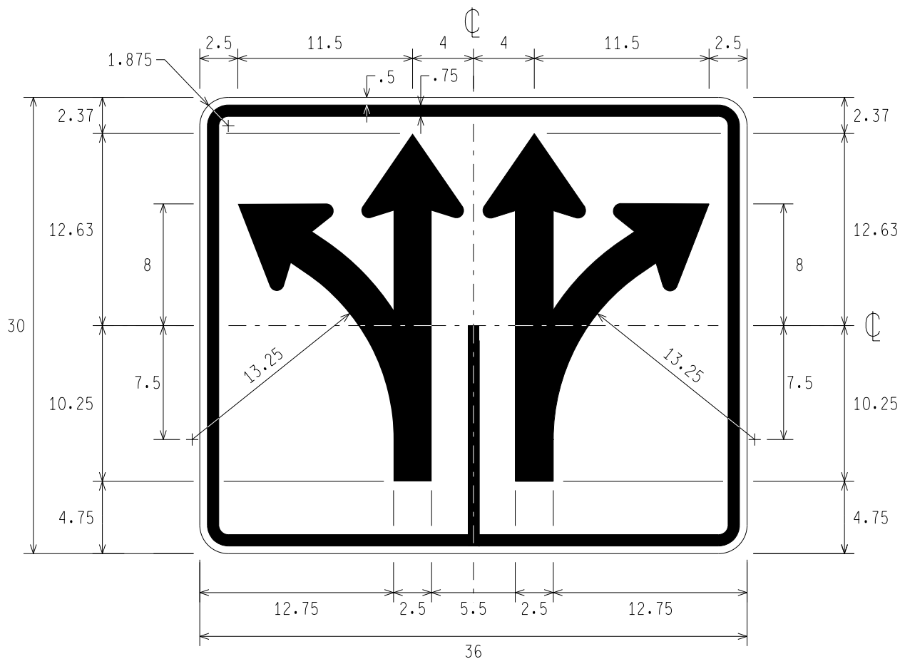
R3-8k LEFT AND THROUGH, THROUGH AND RIGHT
