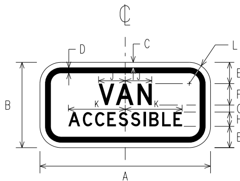
R7-8P VAN ACCESSIBLE PLAQUE
