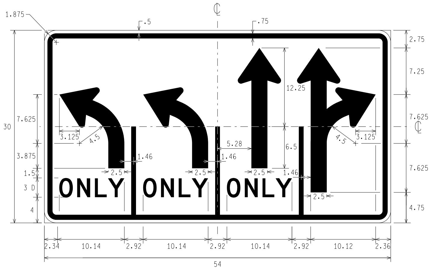
R3-8ai LEFT ONLY, LEFT ONLY, THROUGH ONLY, THROUGH AND RIGHT
