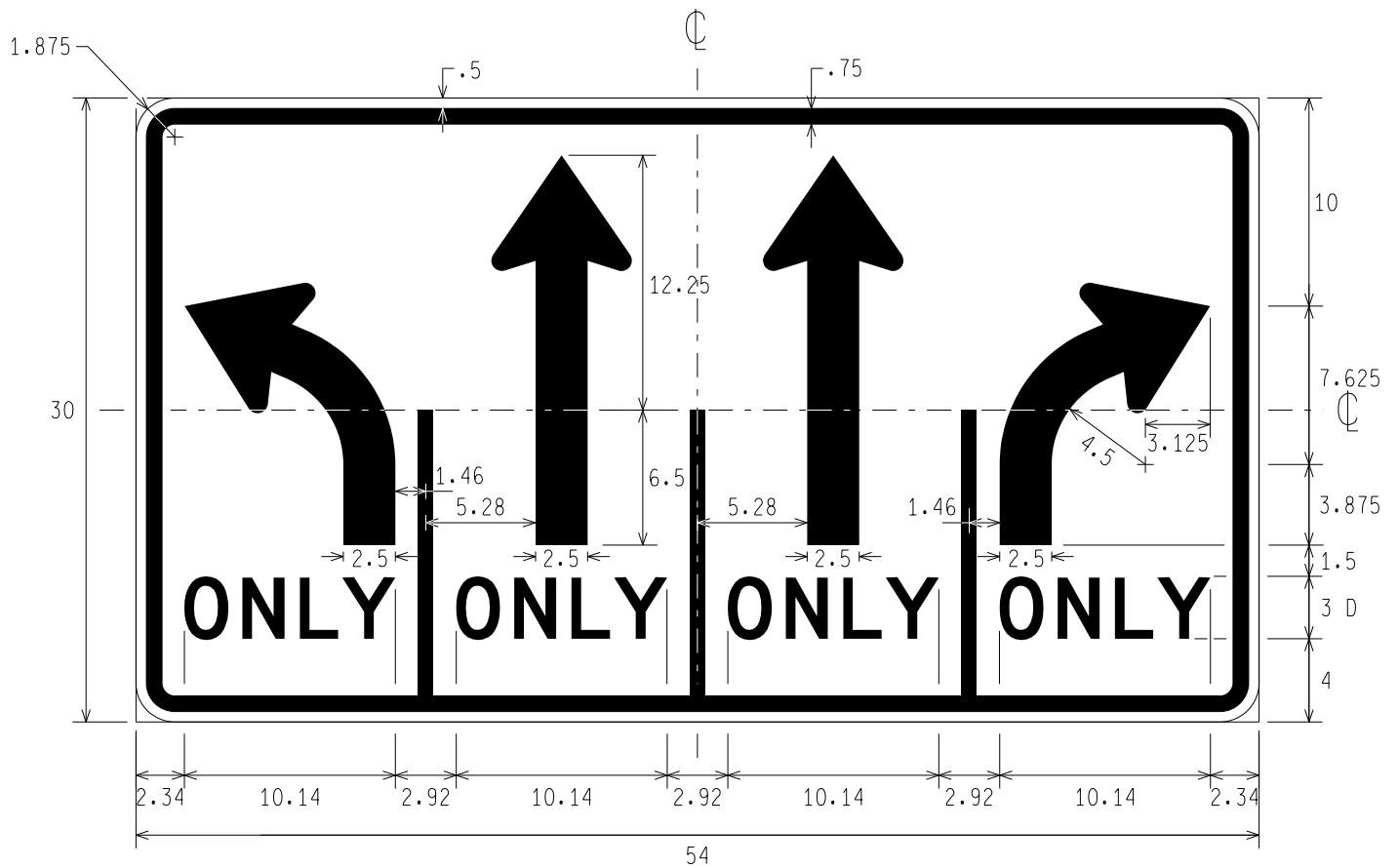
R3-8ad LEFT ONLY, THROUGH ONLY, THROUGH ONLY, RIGHT ONLY
