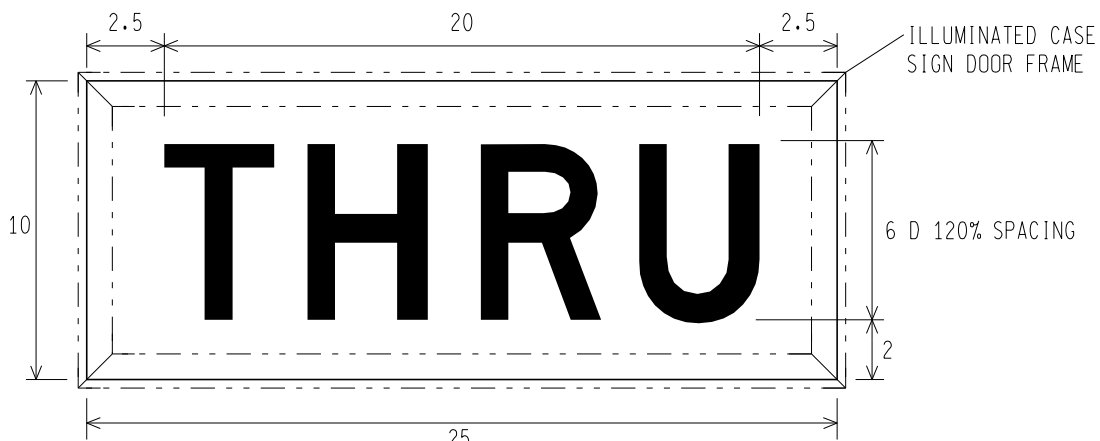
R3-34b THRU (ILLUMINATED CASE SIGN)
