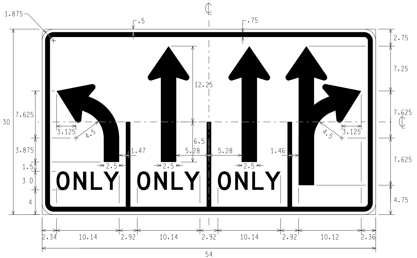
R3-8ae LEFT ONLY, THROUGH ONLY, THROUGH ONLY, THROUGH AND RIGHT
