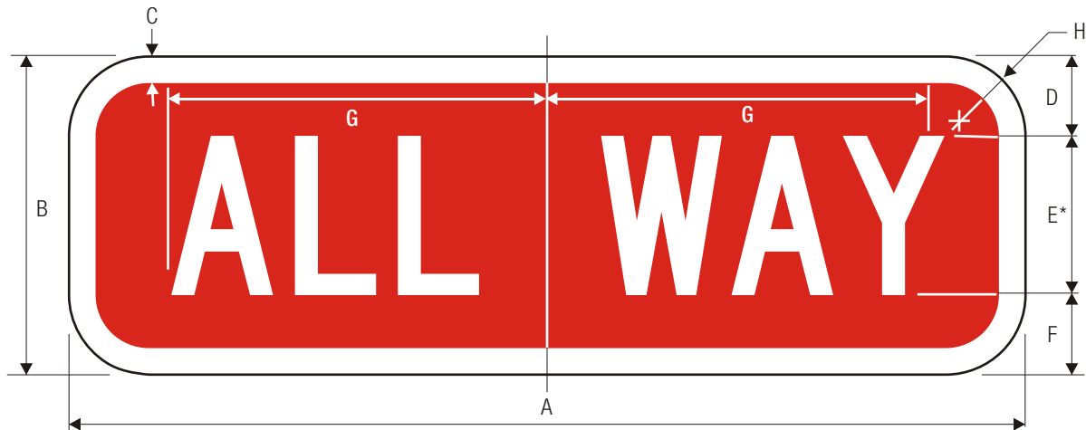
R1-3P ALL WAY
