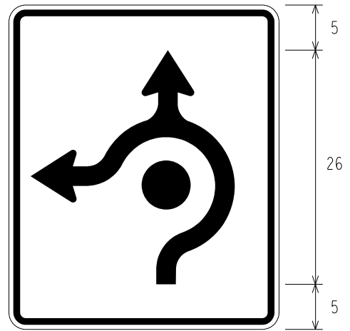
R3-5k (L, THRU)
