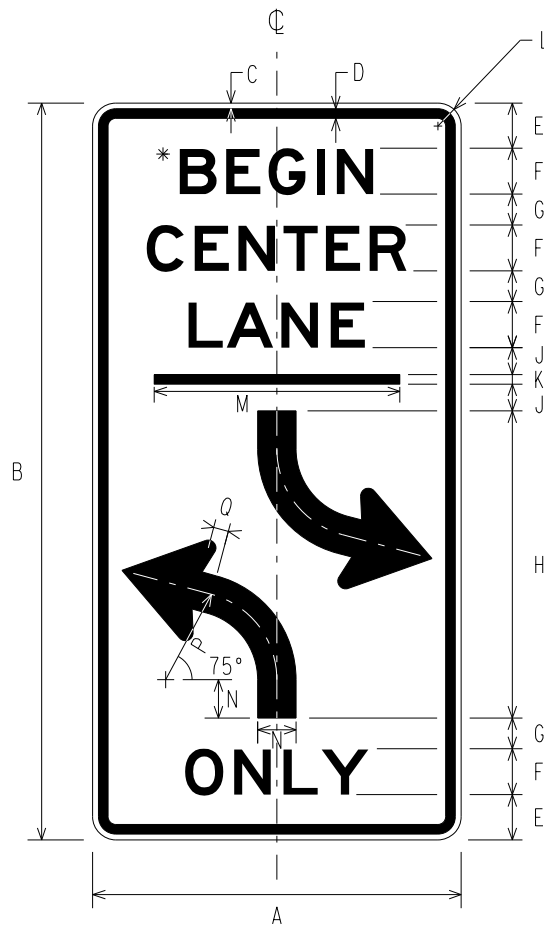
R3-9c GROUND MOUNT BEGIN CENTER LANE TWO-WAY LEFT TURN ONLY
