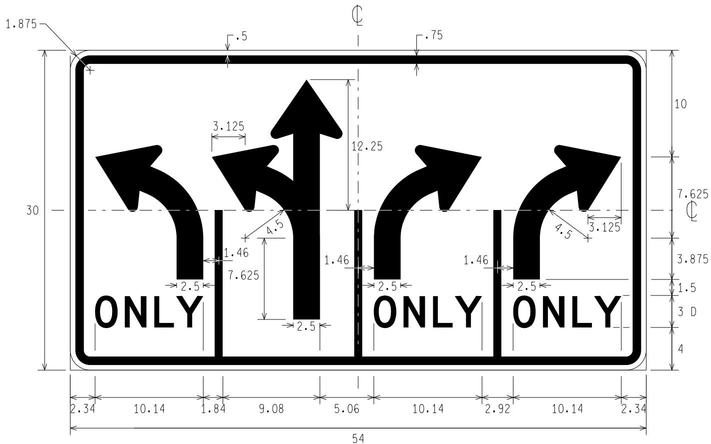
R3-8ak LEFT ONLY, LEFT AND THROUGH, RIGHT ONLY, RIGHT ONLY
