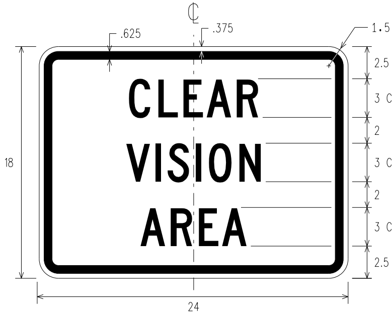
R8-3jP CLEAR VISION AREA
