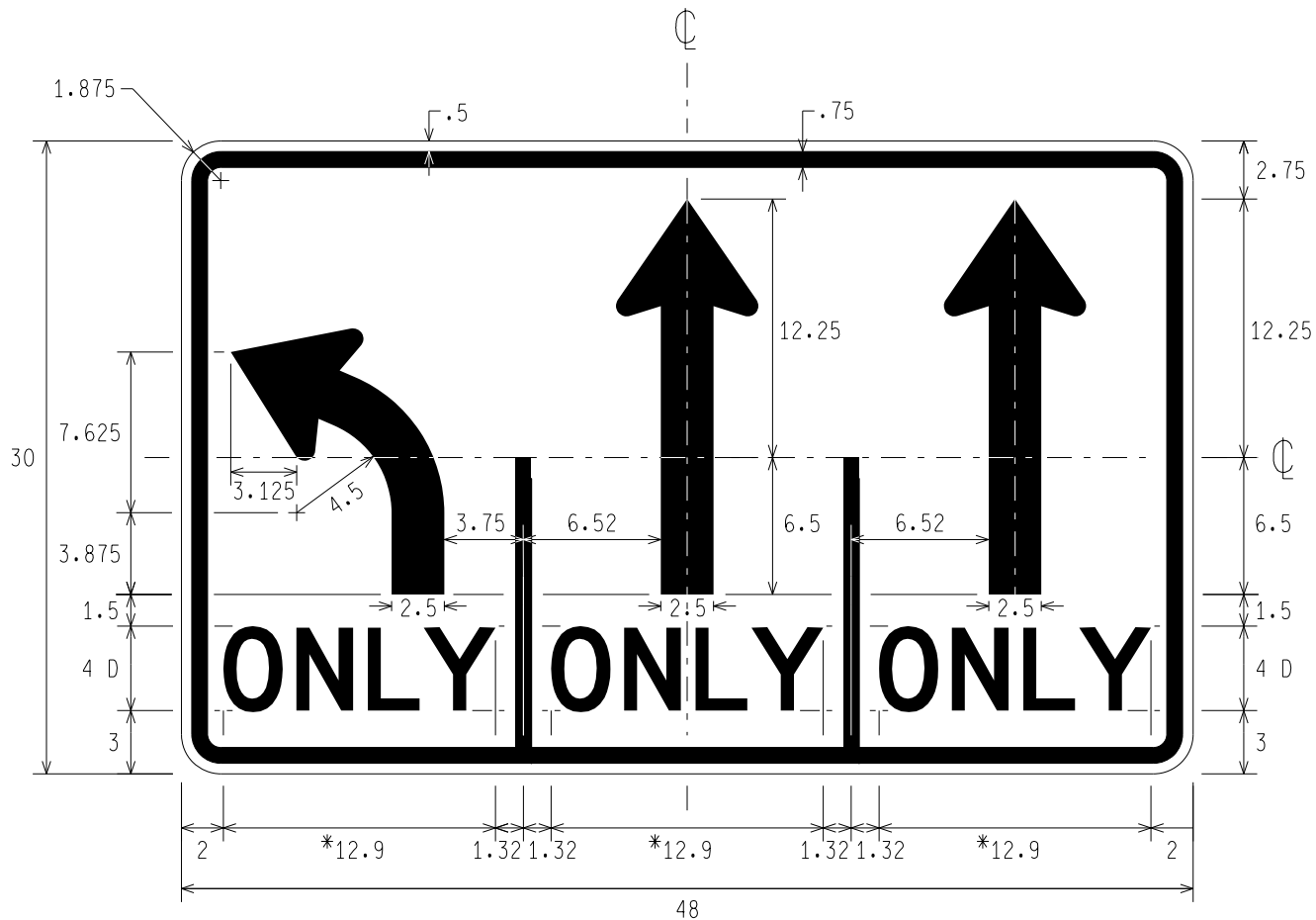
R3-8p LEFT ONLY, THROUGH ONLY, THROUGH ONLY
