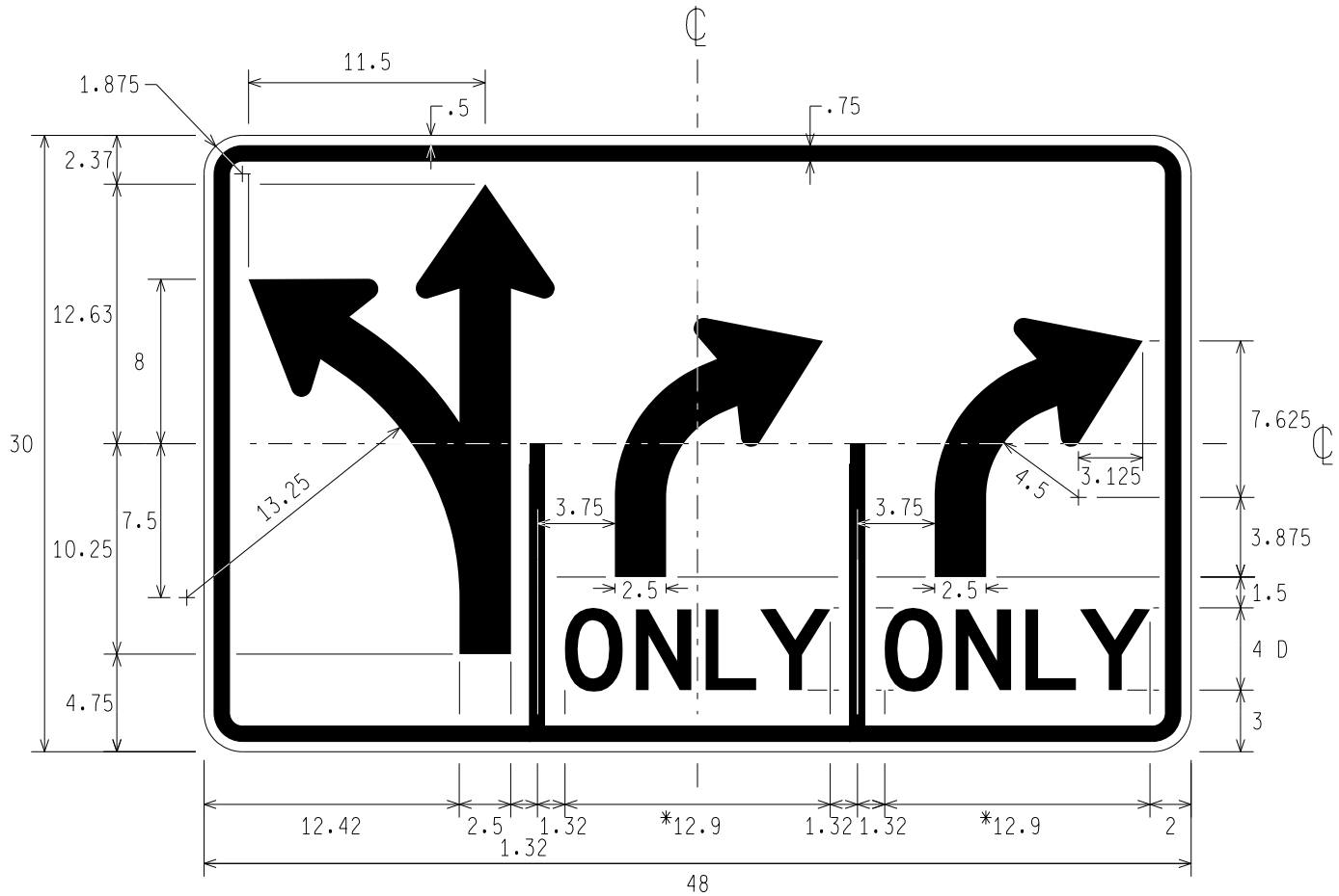
R3-8v LEFT AND THROUGH, RIGHT ONLY, RIGHT ONLY
