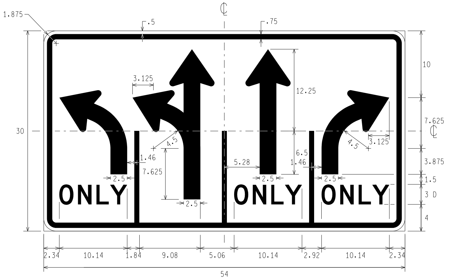
R3-8aj LEFT ONLY, LEFT AND THROUGH, THROUGH ONLY, RIGHT ONLY
