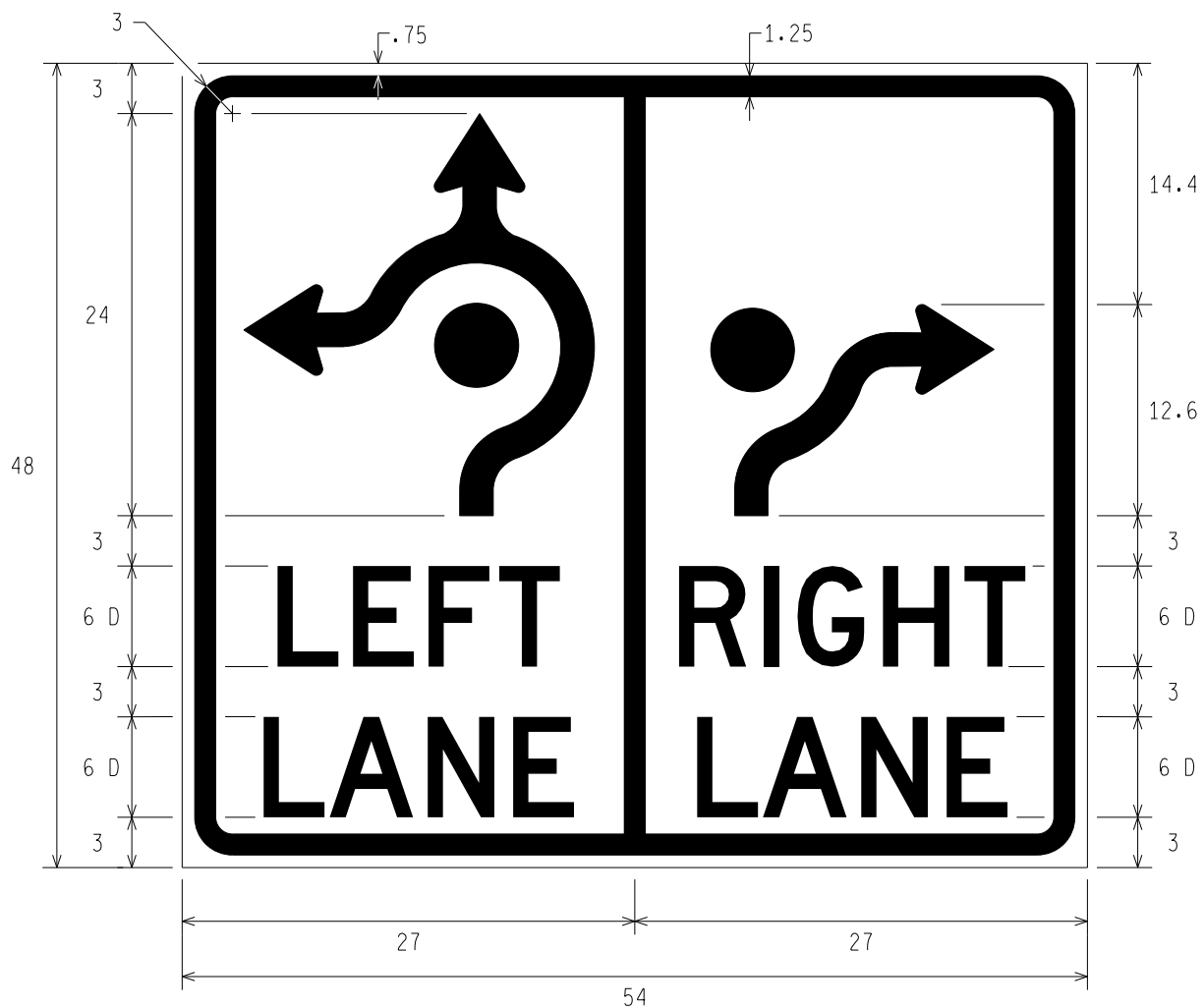
R3-8as-R ROUNDABOUT LEFT LANE, ROUNDABOUT RIGHT LANE
