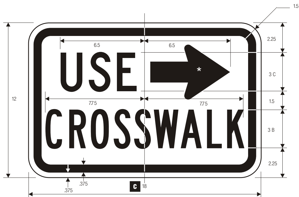
R9-3bP USE CROSSWALK
