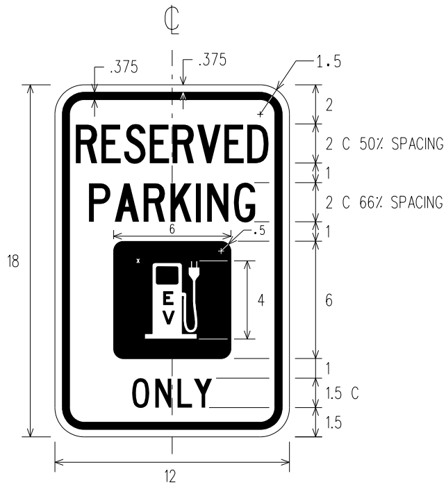
R7-8c RESERVED PARKING ELECTRIC VEHICLE CHARGING SYMBOL
