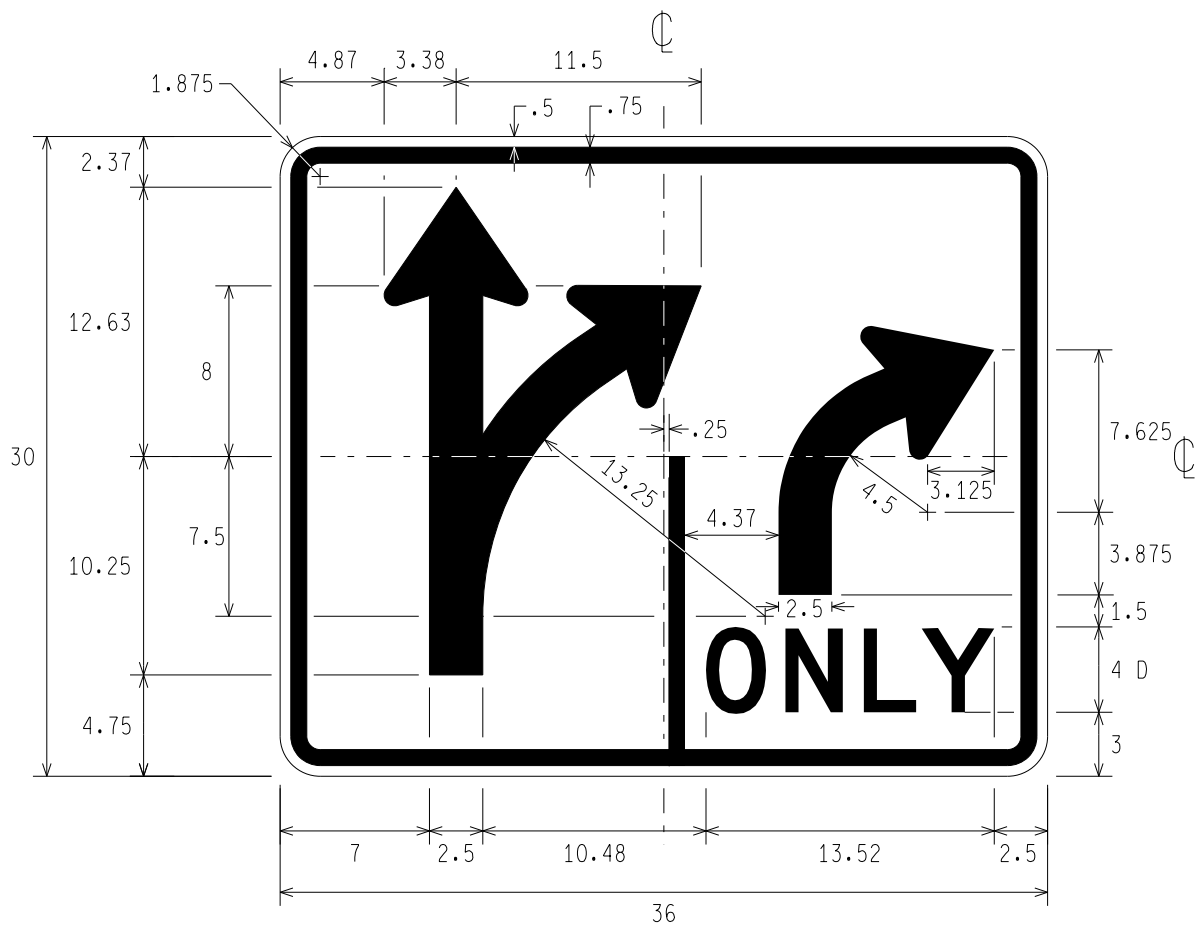
R3-8j THROUGH AND RIGHT, RIGHT ONLY
