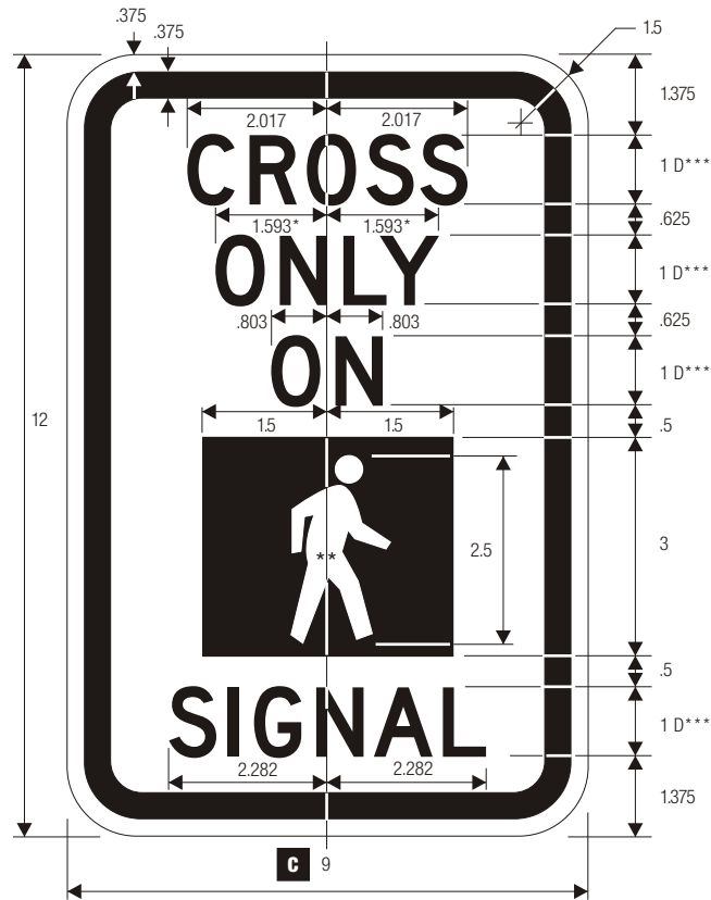
R10-2 CROSS ONLY ON WALK SIGNAL
