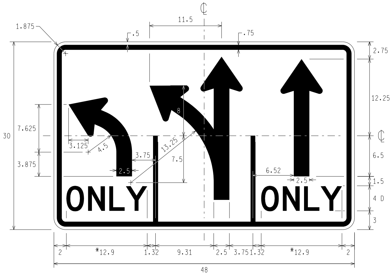
R3-8y LEFT ONLY, LEFT & THROUGH, THROUGH ONLY
