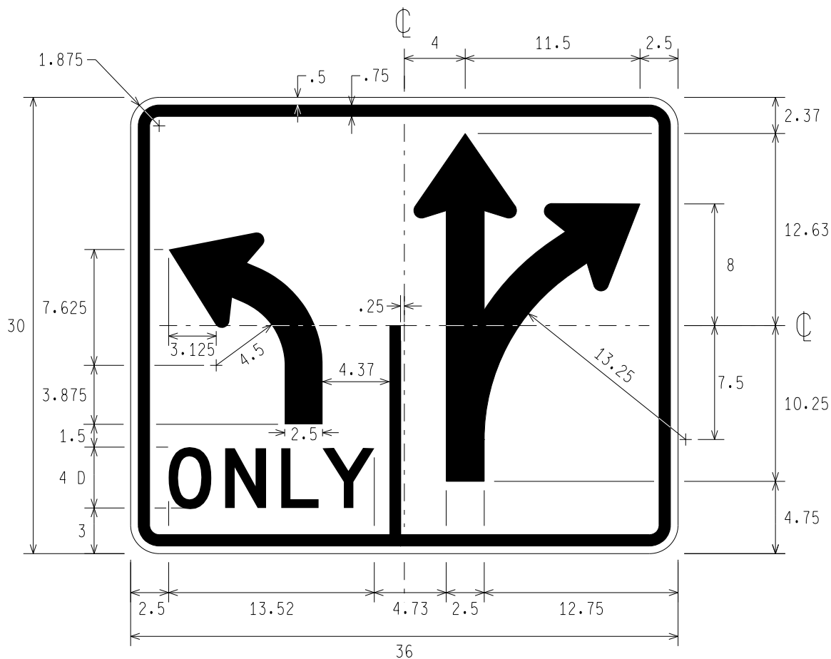
R3-8h LEFT ONLY, THROUGH AND RIGHT
