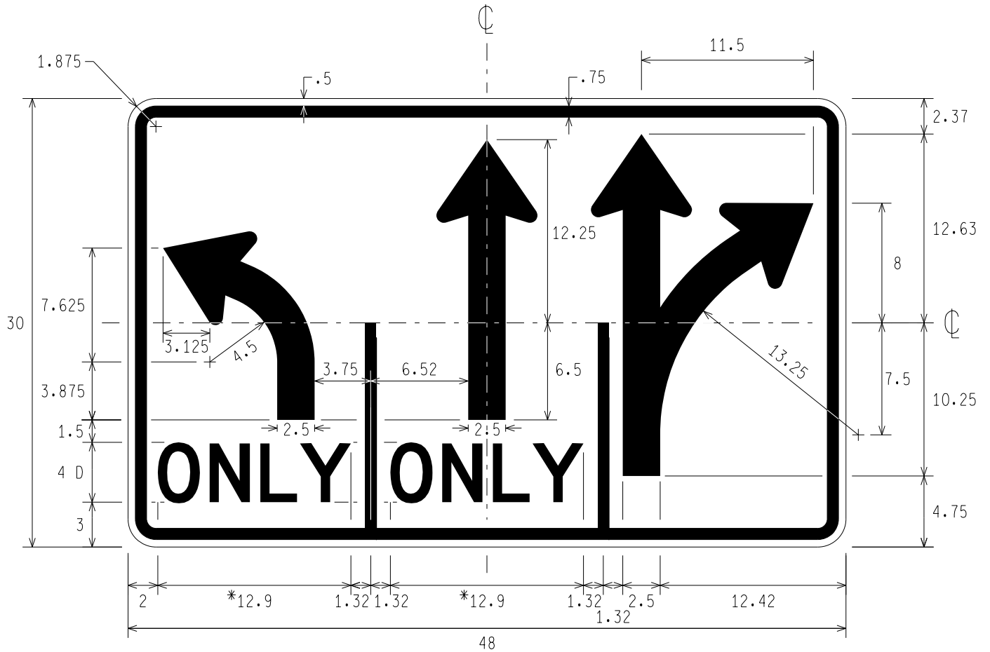
R3-8w LEFT ONLY, THROUGH ONLY, THROUGH & RIGHT
