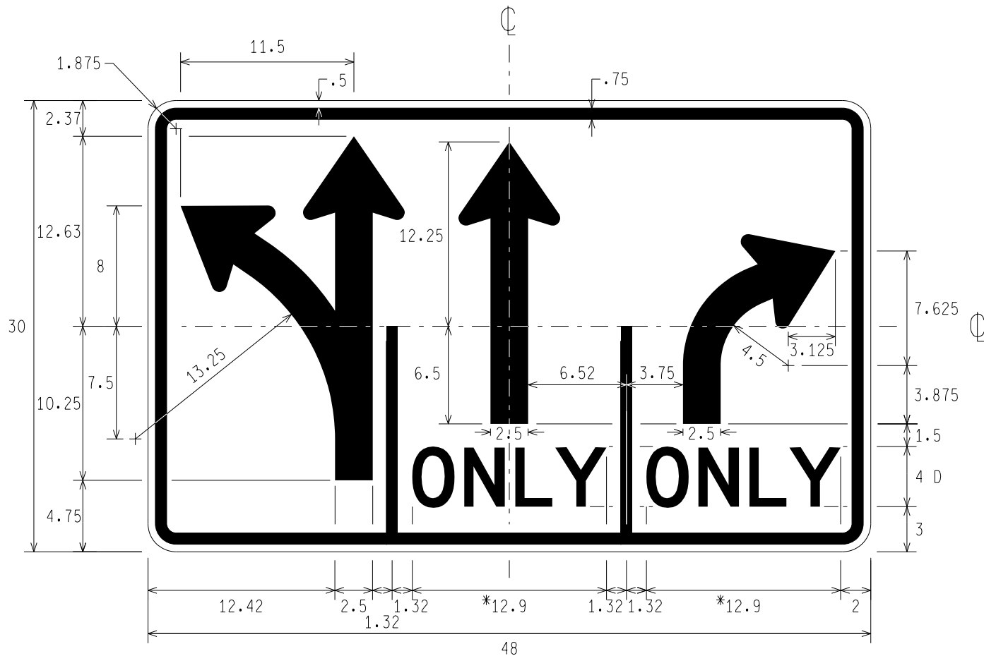
R3-8x LEFT AND THROUGH, THROUGH ONLY, RIGHT ONLY
