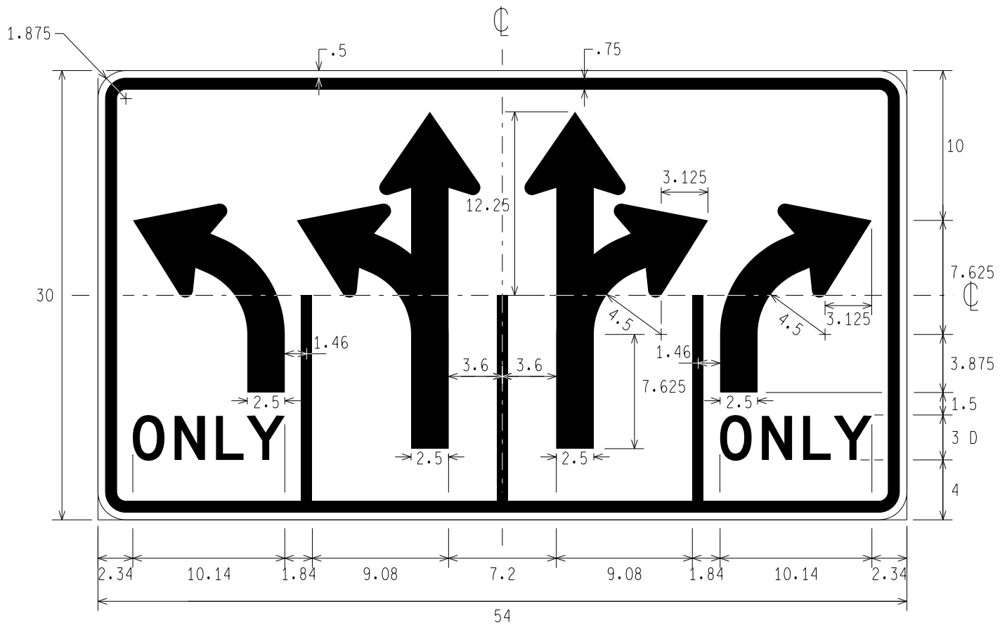
R3-8am LEFT ONLY, LEFT AND THROUGH, THROUGH AND RIGHT, RIGHT ONLY
