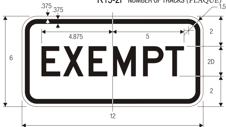
R15-3P / W10-1aP EXEMPT (PLAQUE)
