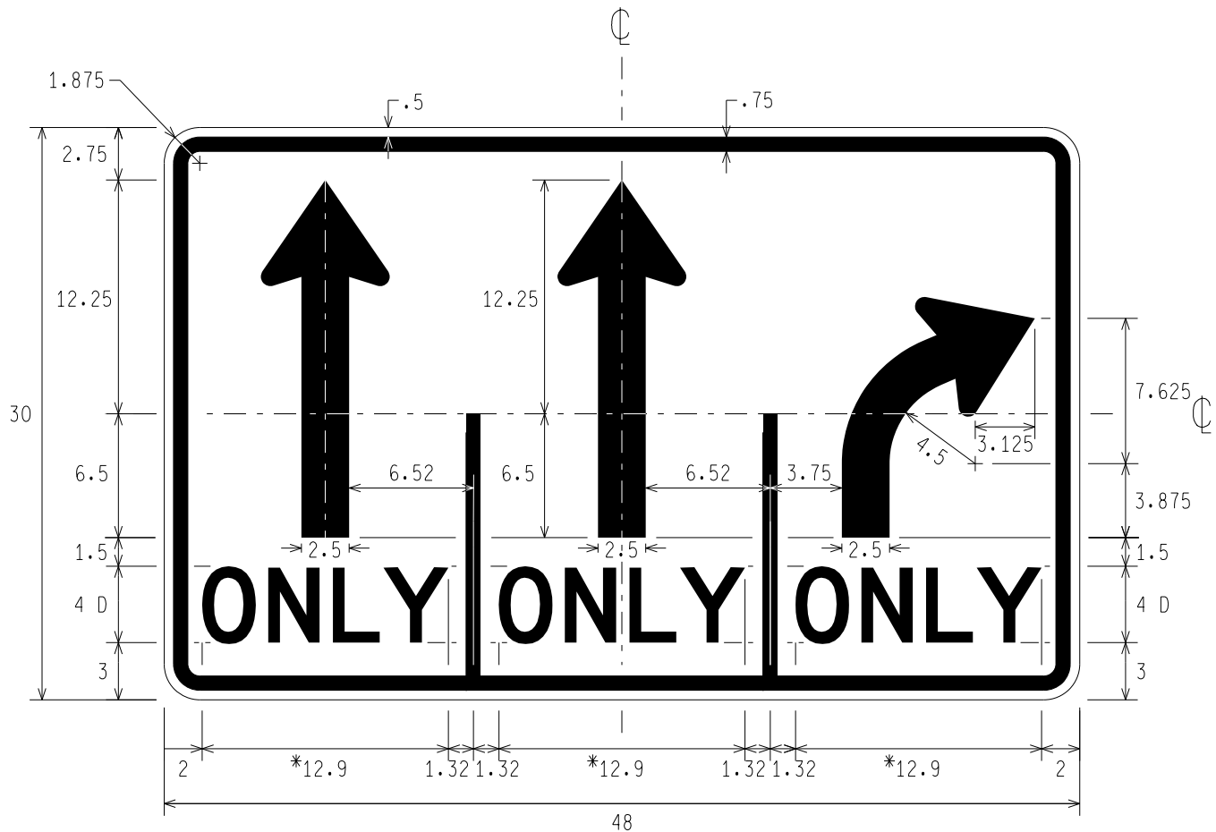
R3-8q THROUGH ONLY, THROUGH ONLY, RIGHT ONLY
