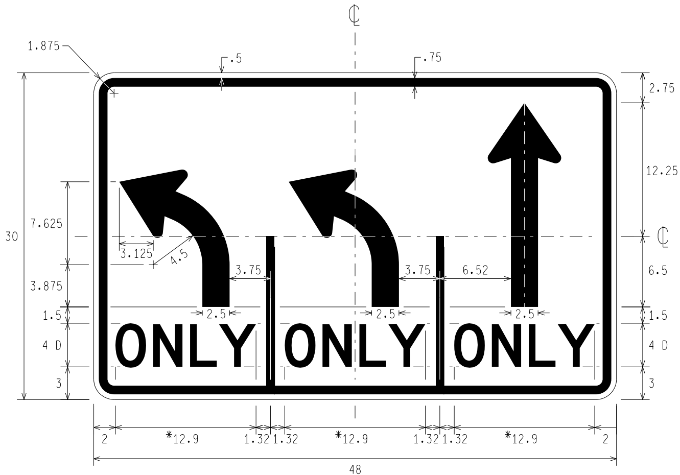
R3-8s LEFT ONLY, LEFT ONLY, THROUGH ONLY
