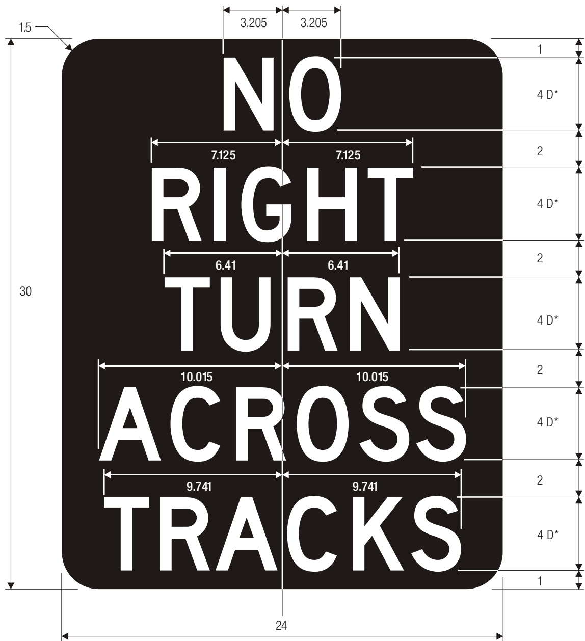
R3-1a ACTIVATED BLANK-OUT
