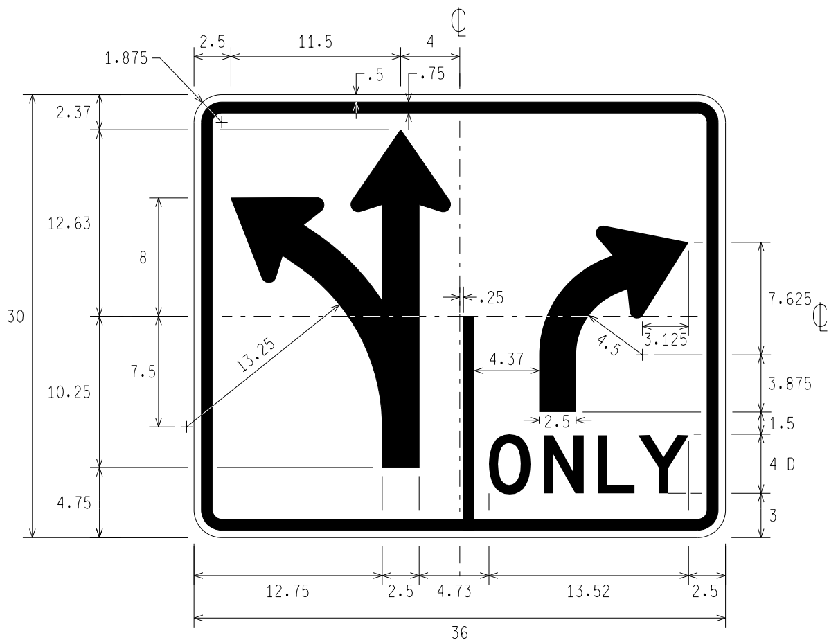
R3-8i LEFT AND THROUGH, RIGHT ONLY
