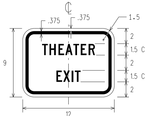
R8-3kP THEATER EXIT
