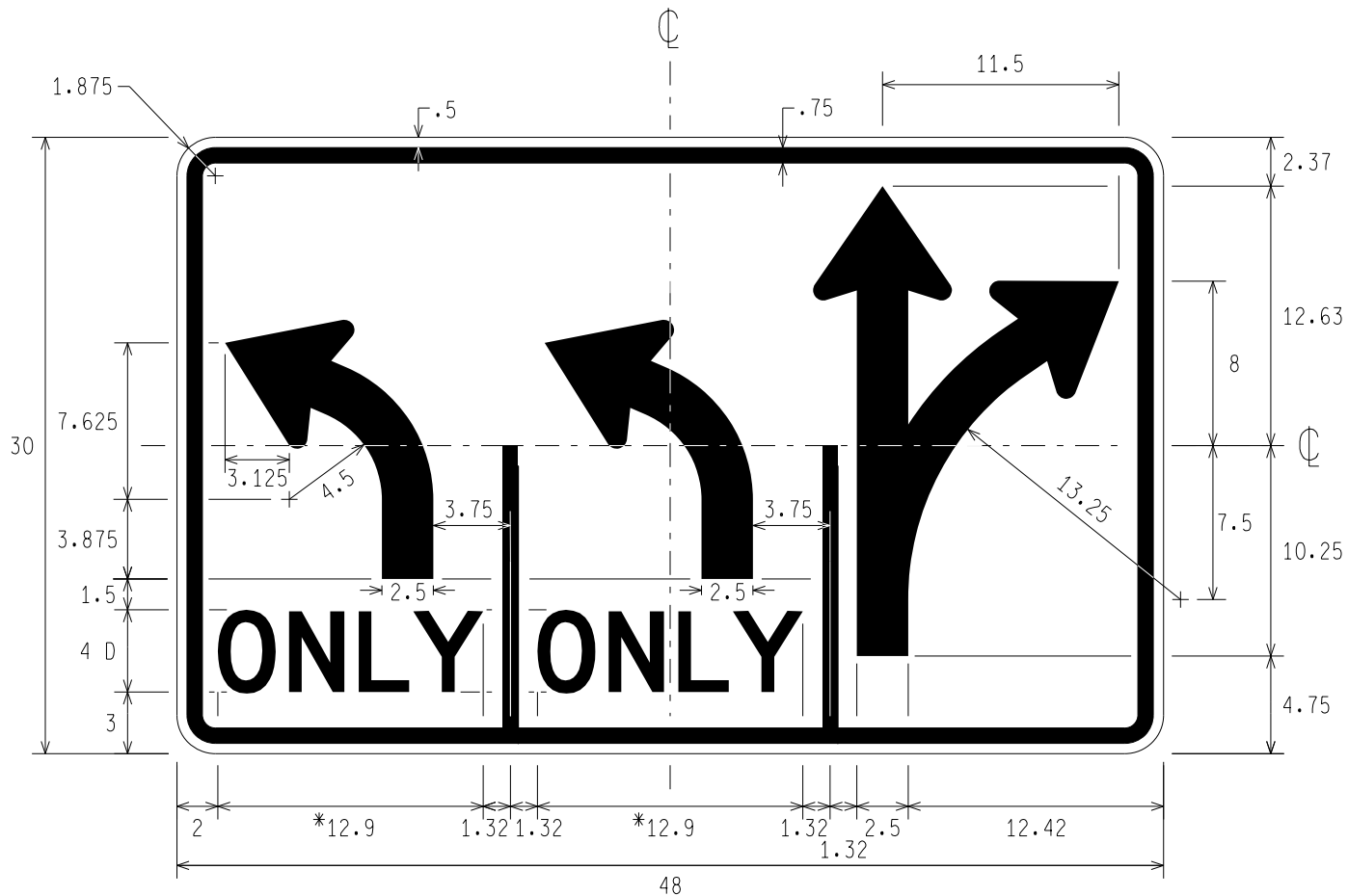
R3-8u LEFT ONLY, LEFT ONLY, THROUGH AND RIGHT
