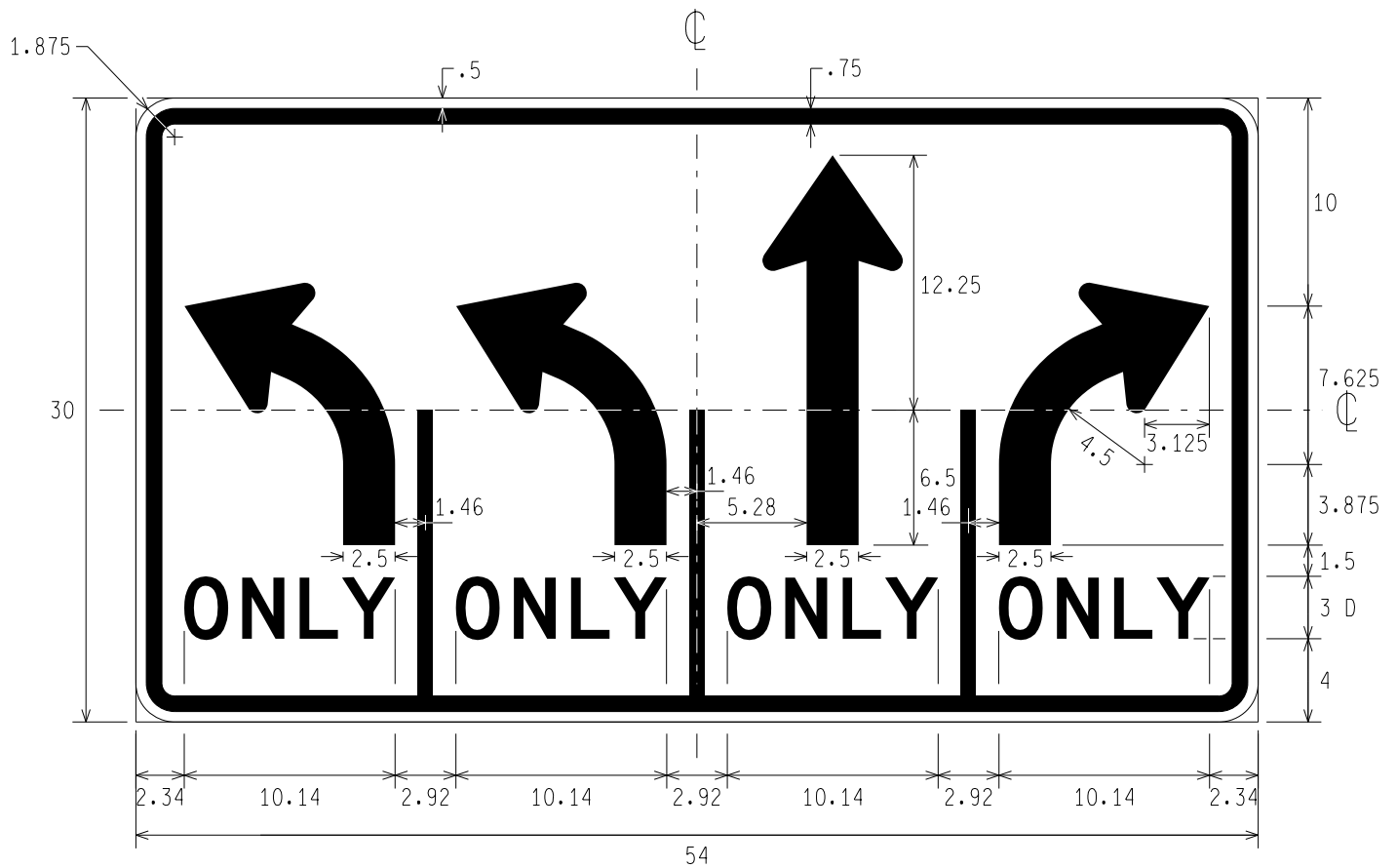
R3-8ah LEFT ONLY, LEFT ONLY, THROUGH ONLY, RIGHT ONLY
