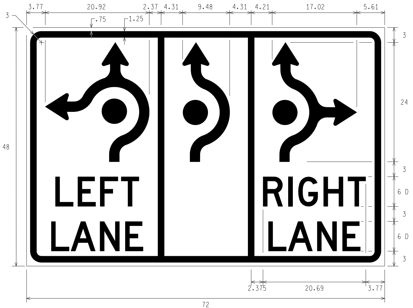
R3-8at-R ROUNDABOUT LEFT LANE, ROUNDABOUT THROUGH LANE, ROUNDABOUT RIGHT LANE
