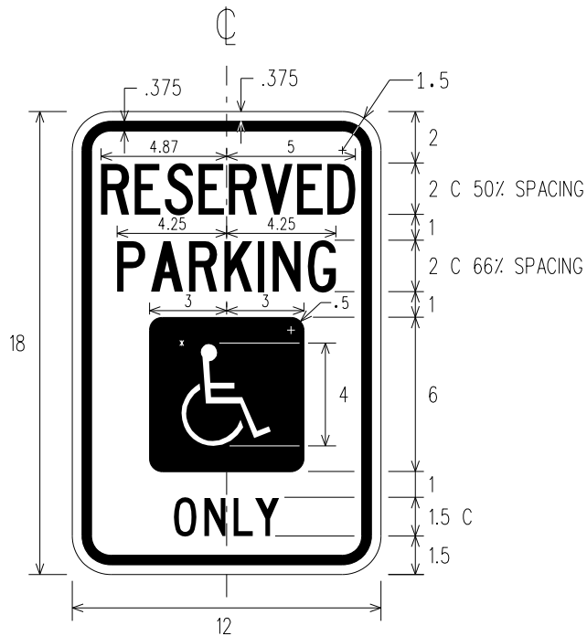
R7-8 RESERVED PARKING ACCESSIBLE SYMBOL
