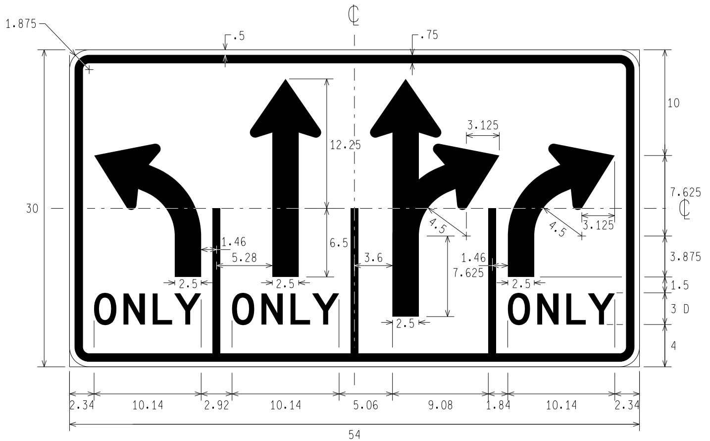
R3-8ag LEFT ONLY, THROUGH ONLY, THROUGH AND RIGHT, RIGHT ONLY
