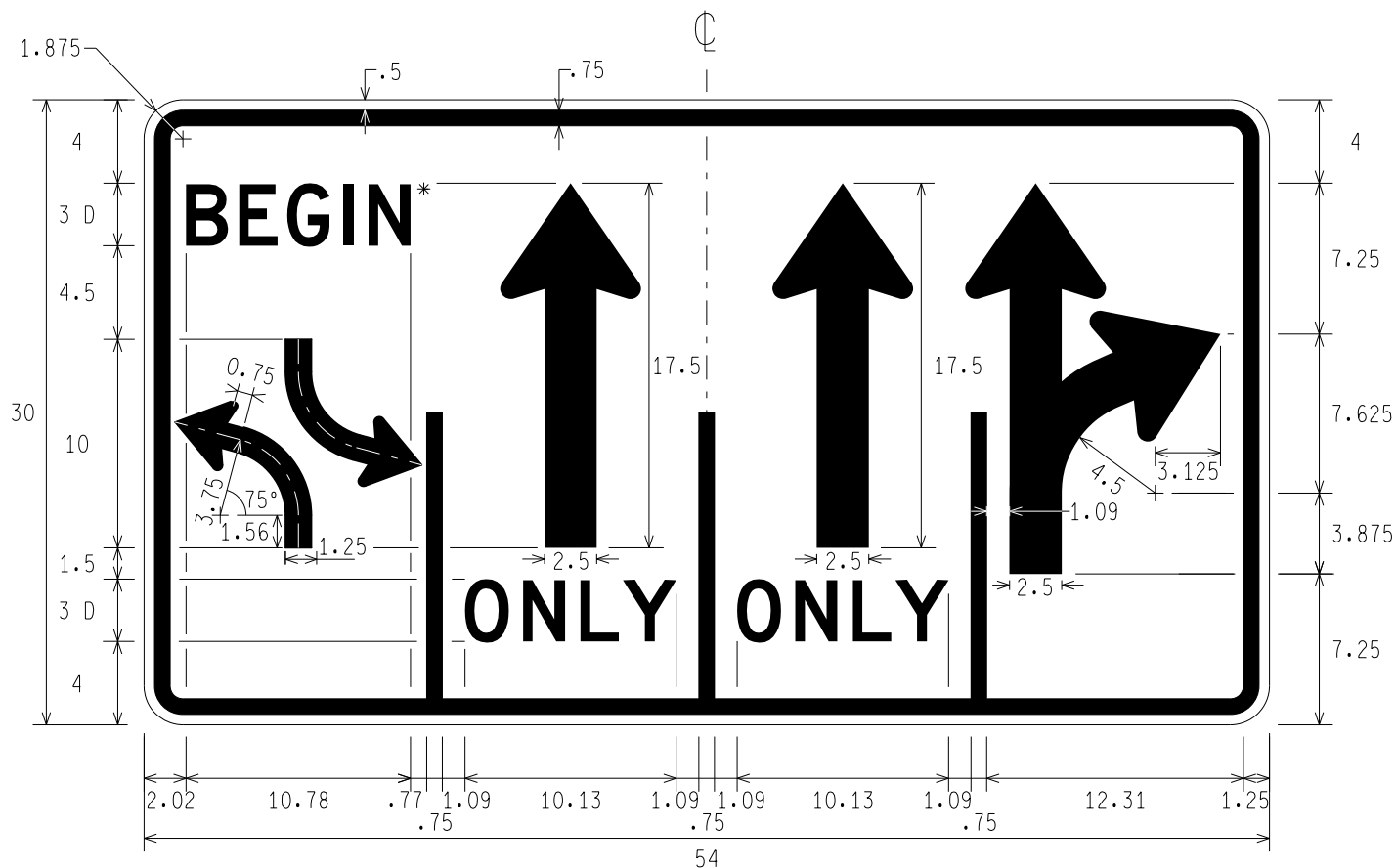
R3-9q BEGIN CENTER TURN LANE, THROUGH ONLY, THROUGH ONLY, THROUGH & RIGHT
