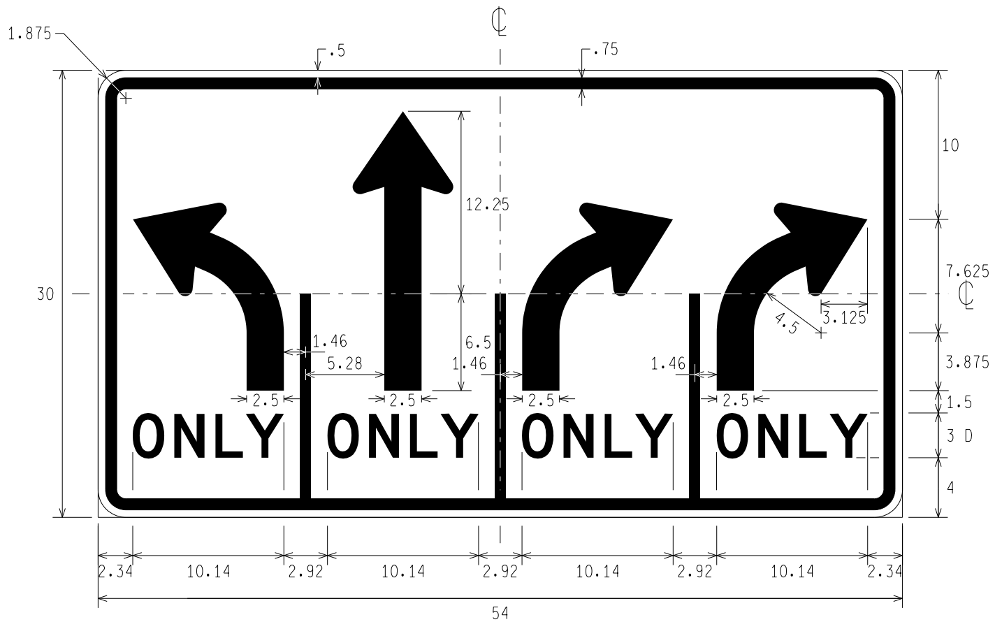
R3-8af LEFT ONLY, THROUGH ONLY, RIGHT ONLY, RIGHT ONLY
