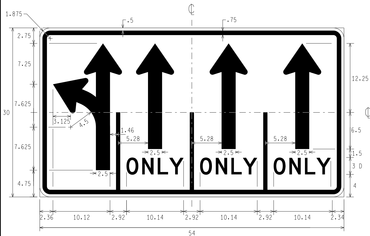
R3-8aa LEFT AND THROUGH, THROUGH ONLY, THROUGH ONLY, THROUGH ONLY
