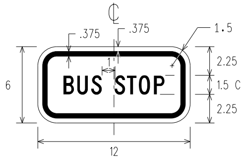
R8-3iP BUS STOP
