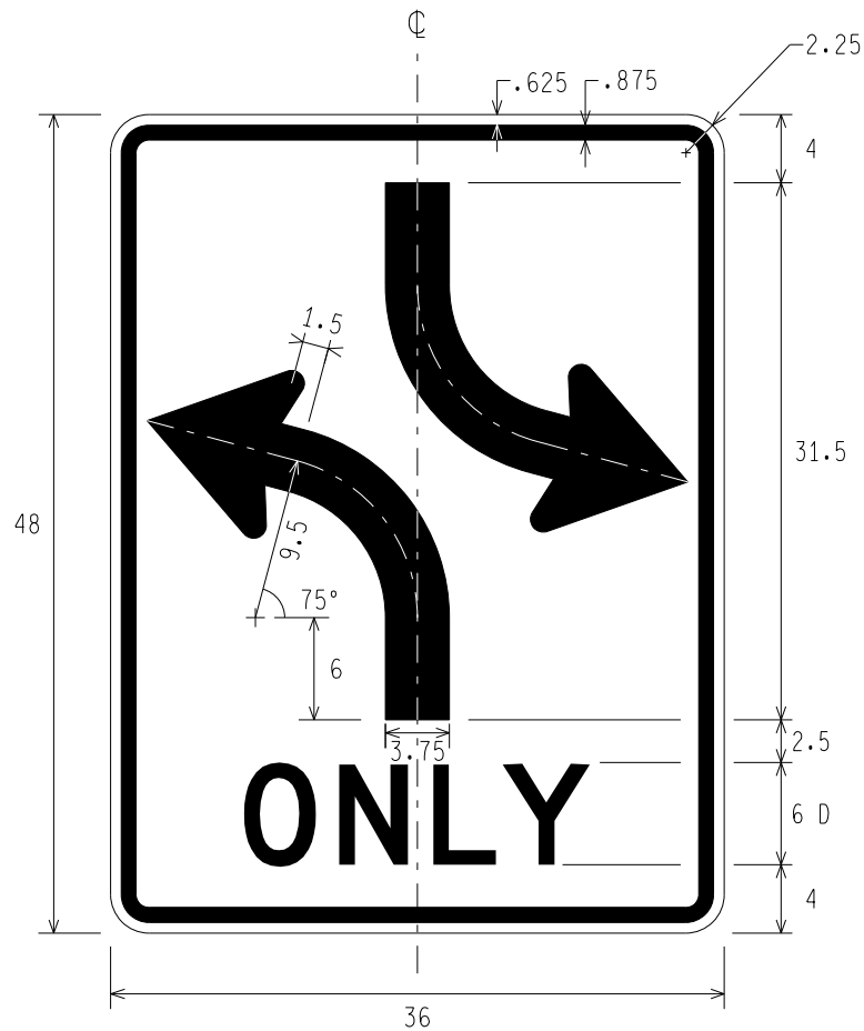
R3-9a OVERHEAD TWO-WAY LEFT TURN ONLY
