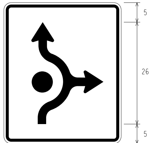
R3-5m (THRU, R)
