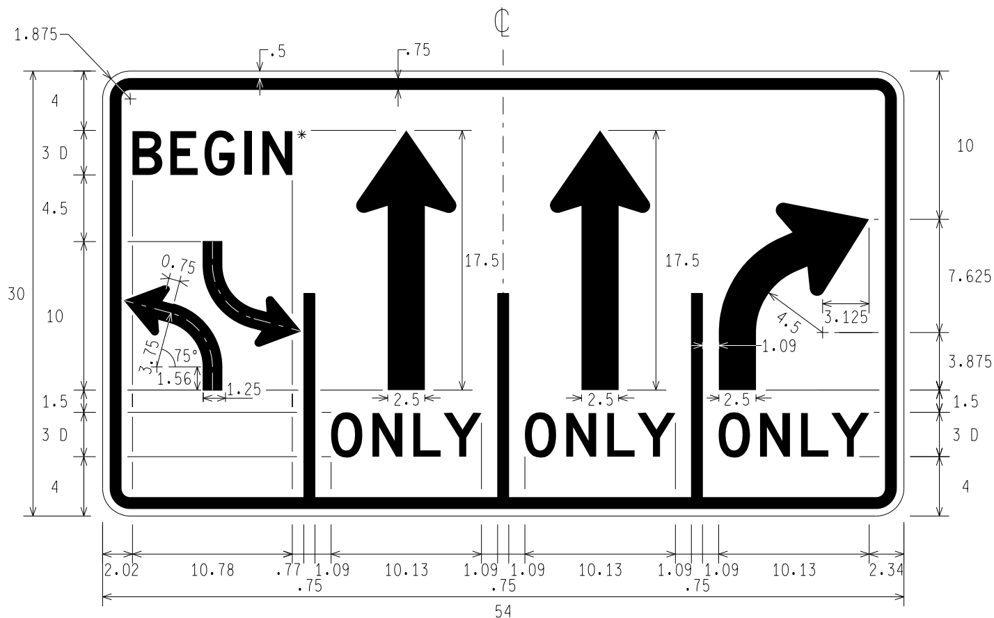
R3-9r BEGIN CENTER TURN LANE, THROUGH ONLY, THROUGH ONLY, RIGHT ONLY
