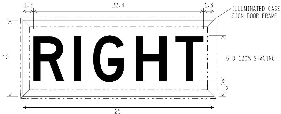
R3-34 RIGHT (ILLUMINATED CASE SIGN)
