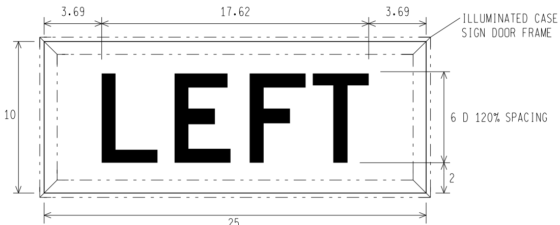
R3-34a LEFT (ILLUMINATED CASE SIGN)
