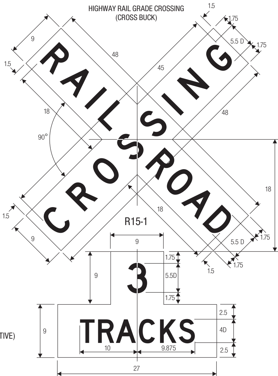
NUMBER OF TRACKS (PLAQUE)
