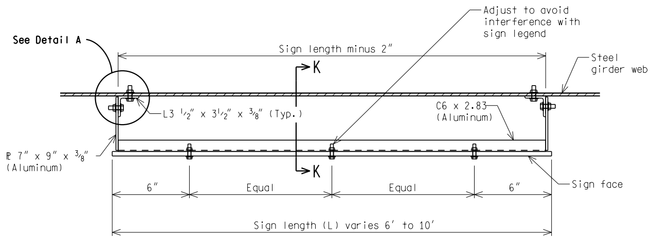
PLAN 0° CONNECTION
