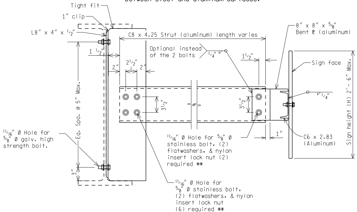
SECTION M-M
