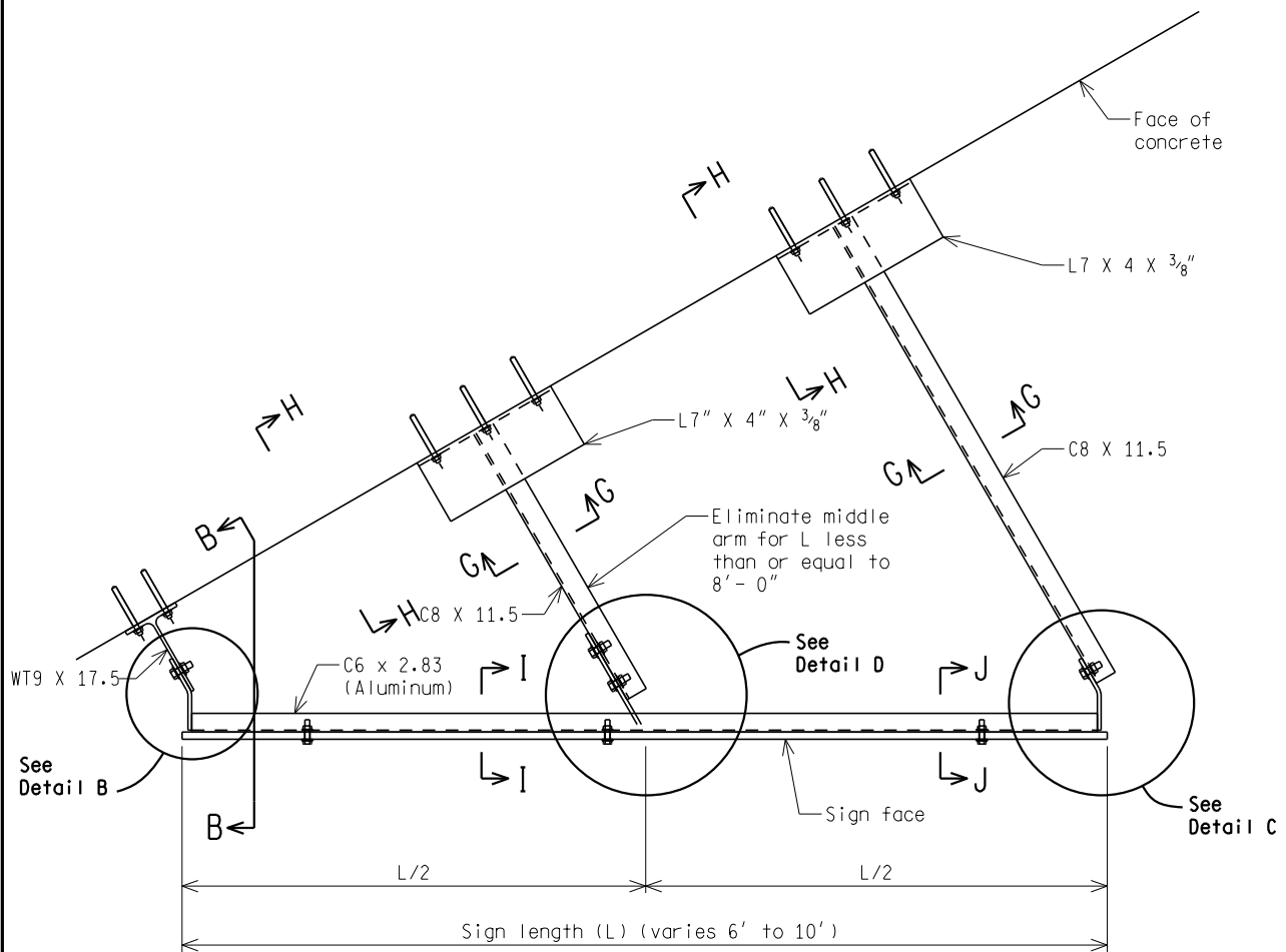
PLAN 5° - 40° CONNECTION (CONCRETE T-BEAMS & CONCRETE BARRIERS)
