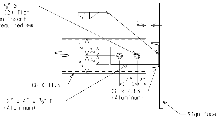
SECTION I-I
