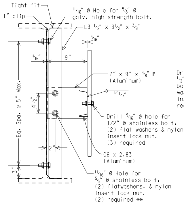
SECTION K-K
