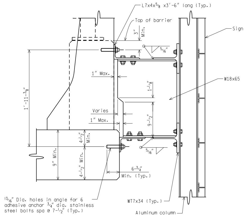
DETAIL OF CONNECTION
