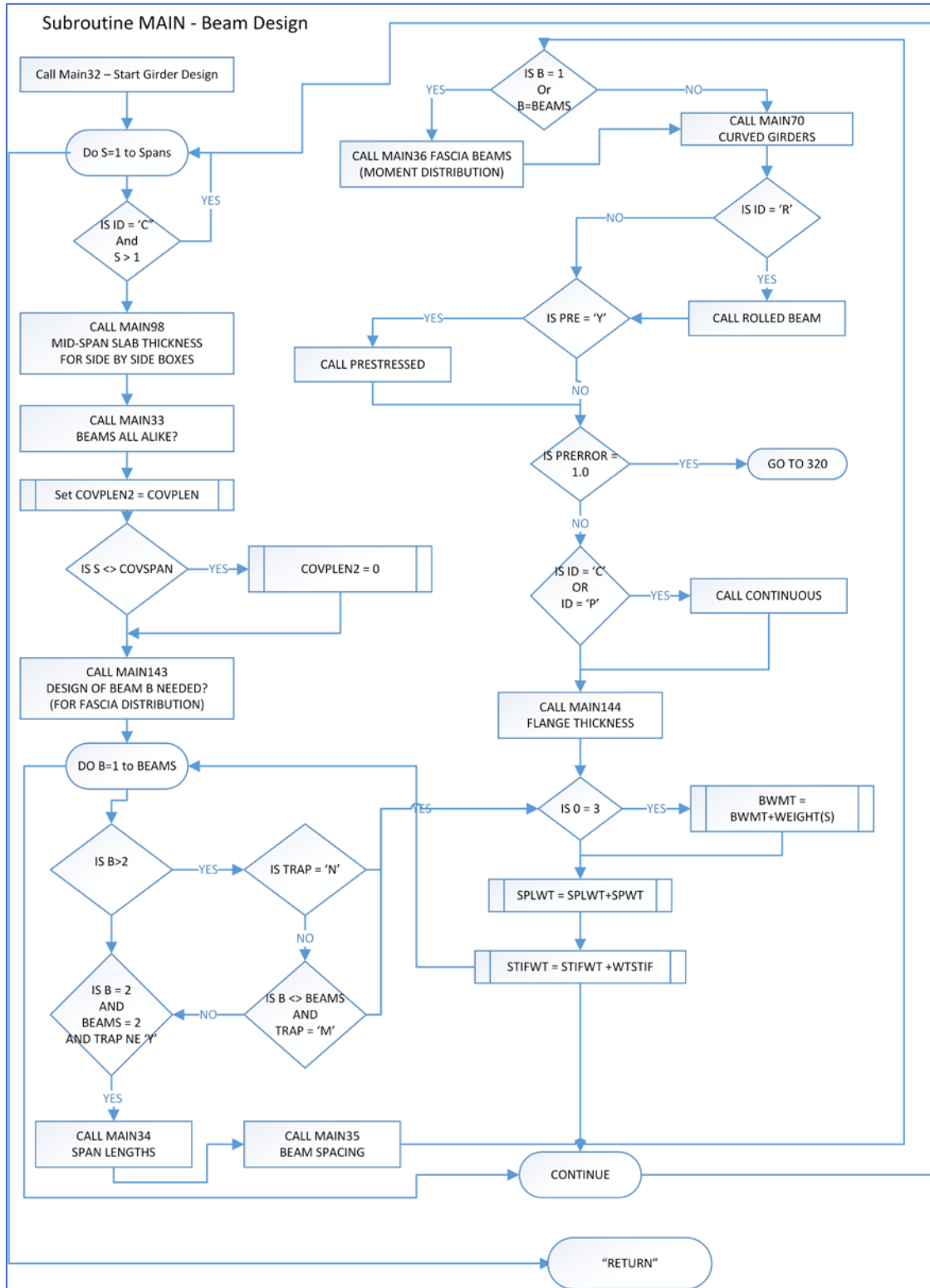
Figure 5: Logic Diagram for Beam Design (A Component of Main)
