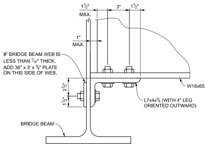
DETAIL D
