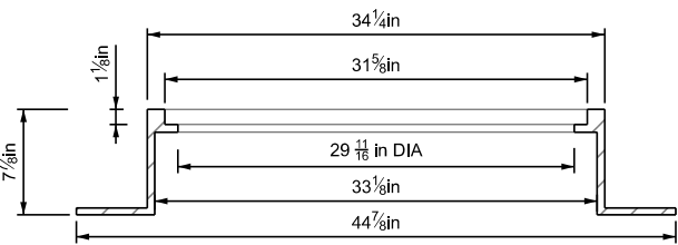
P DETAIL - MANHOLE FRAME N.T.S. FRAME SECTION (HEAVY DUTY)
