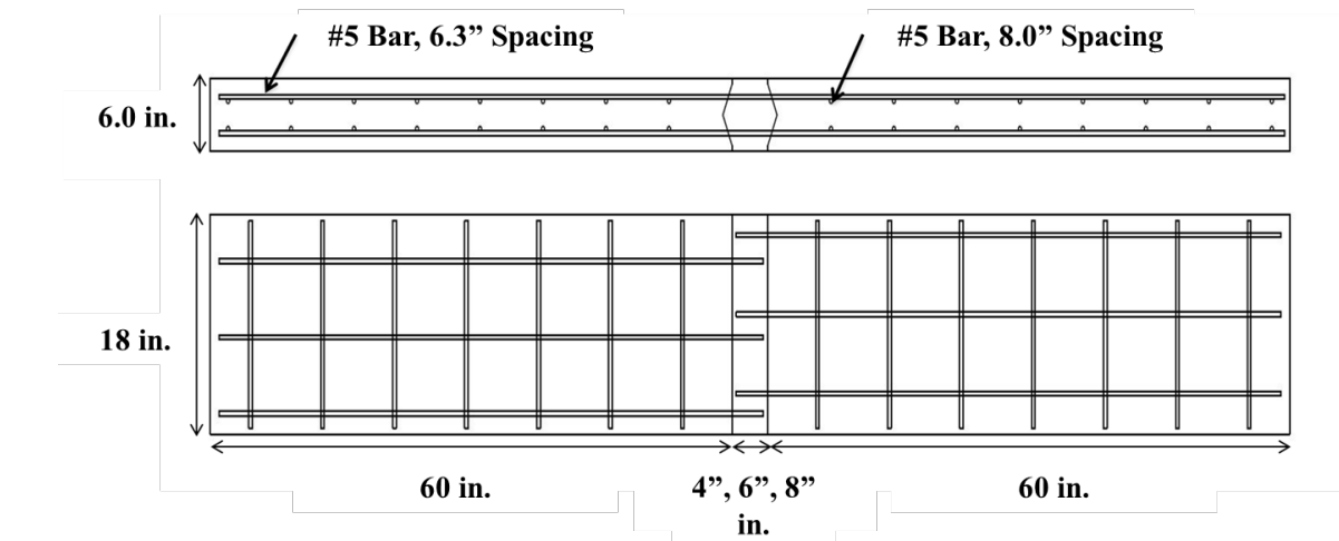
(a) Pure flexure specimens
