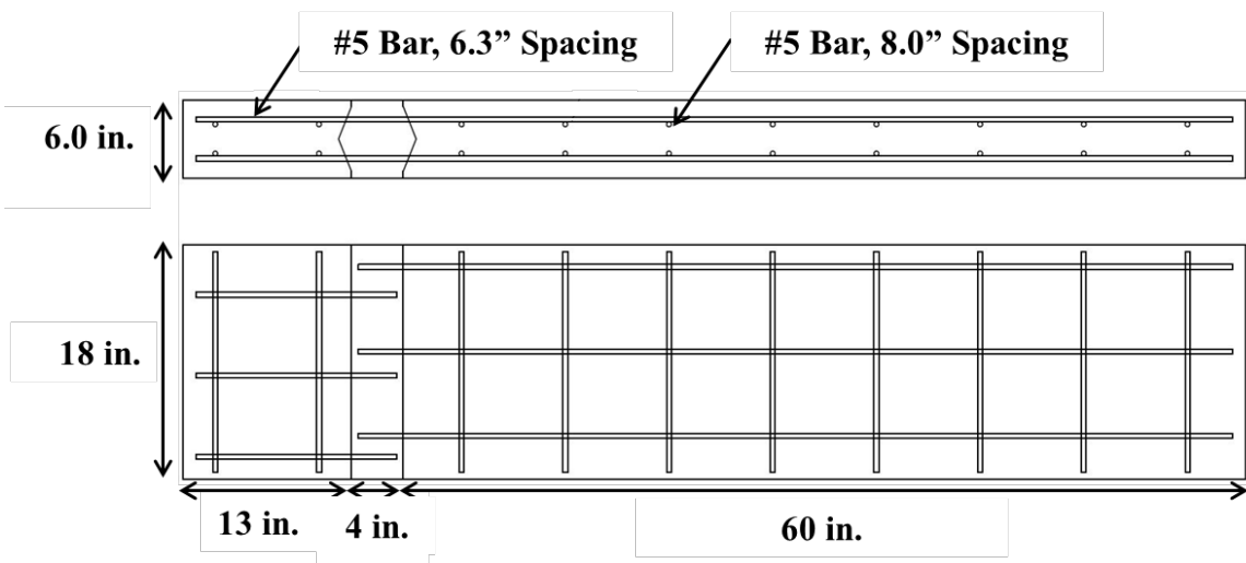
(b) Combined shear/flexure specimens
