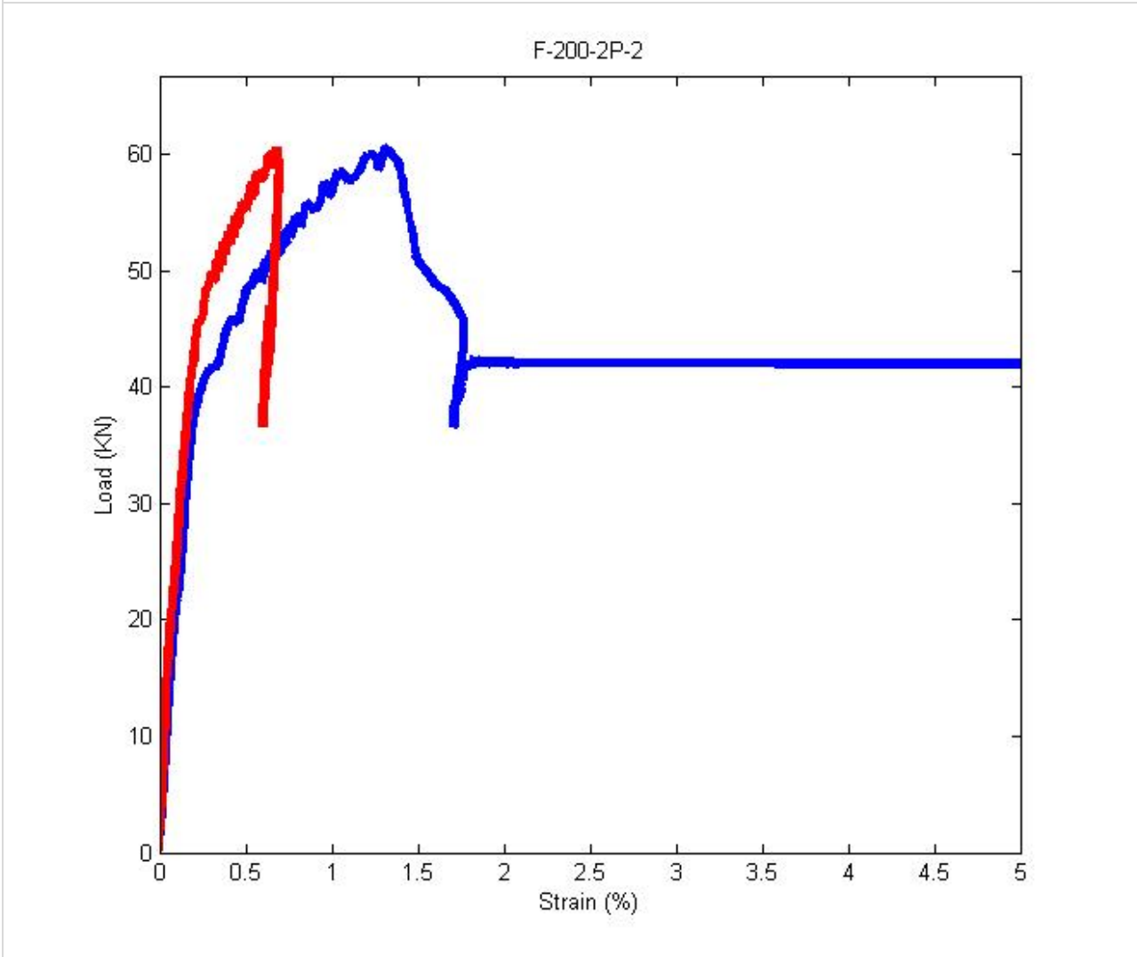
Strain (%) in Bars vs. Load (KN)
