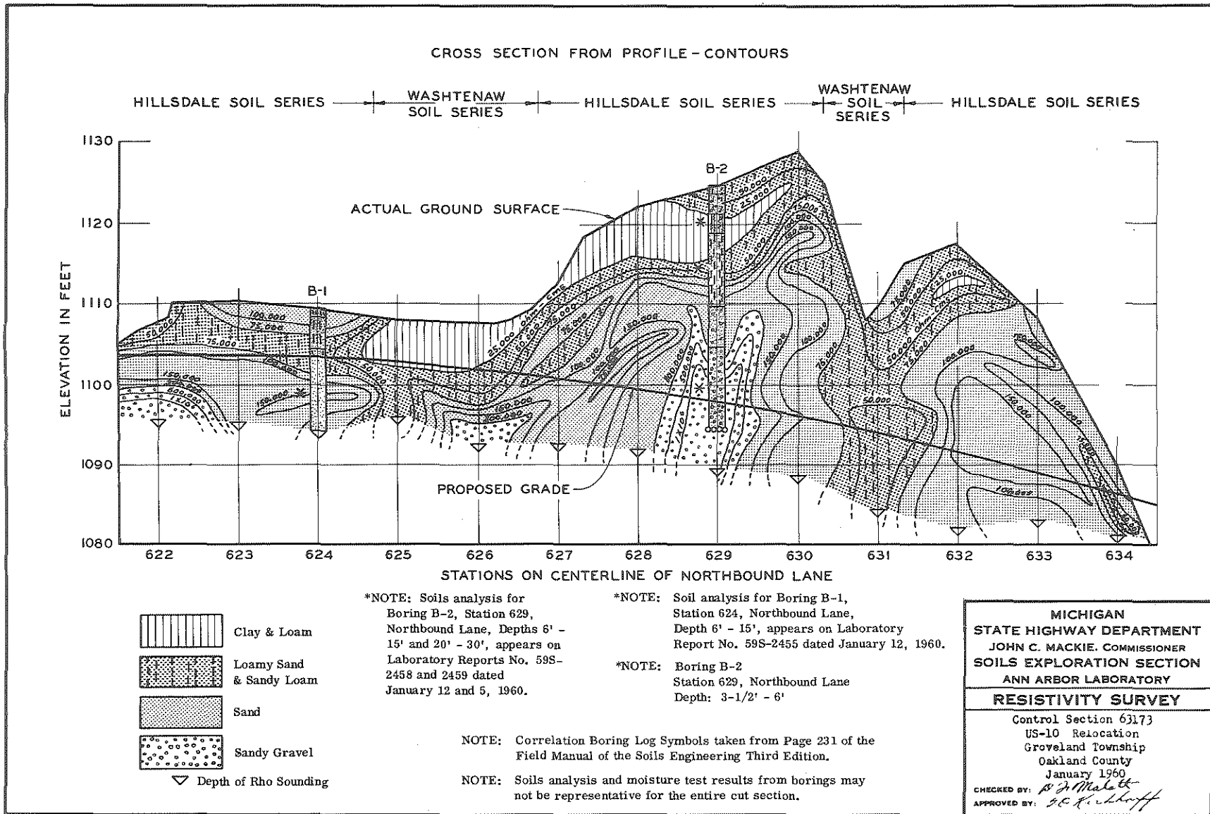
Figure 5. Typical resistivity survey.
