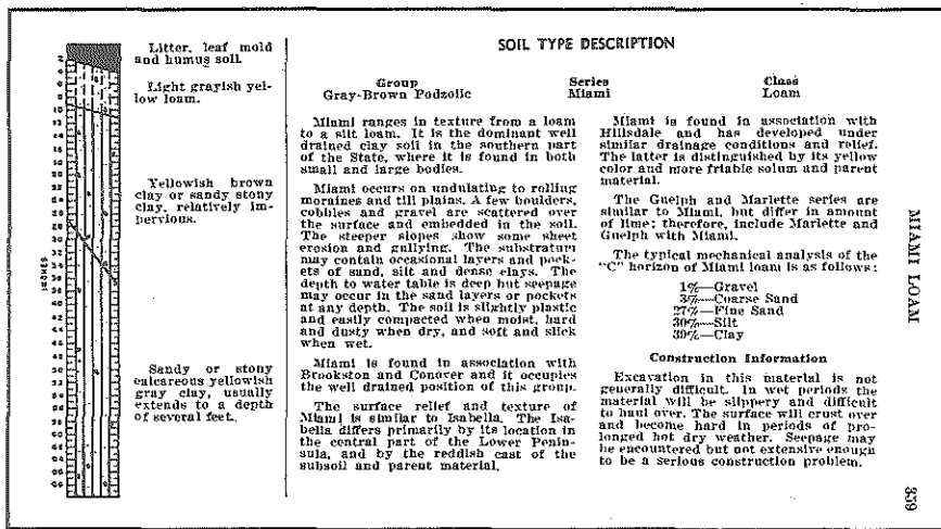
Figure 1. Soil series profiles from Field Manual of Soil Engineering (Fourth Edition) .
