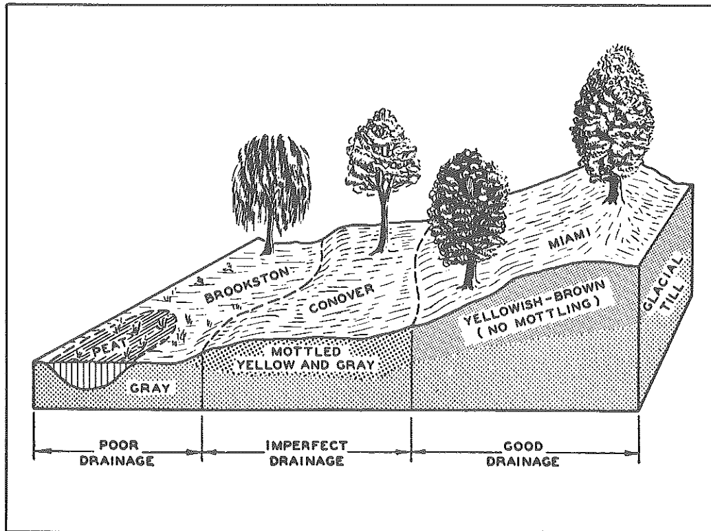
Figure 2. The drainage and relief characteristics of a soil catena (Miami - Conover - Brookston shown).
