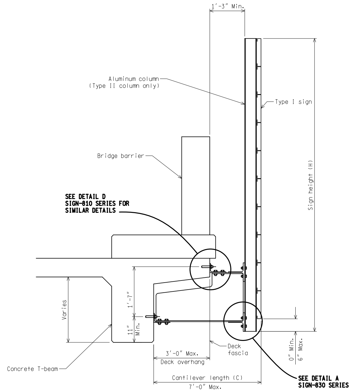
SECTION THRU BRIDGE (SEE DETAIL NEXT SHEET)
