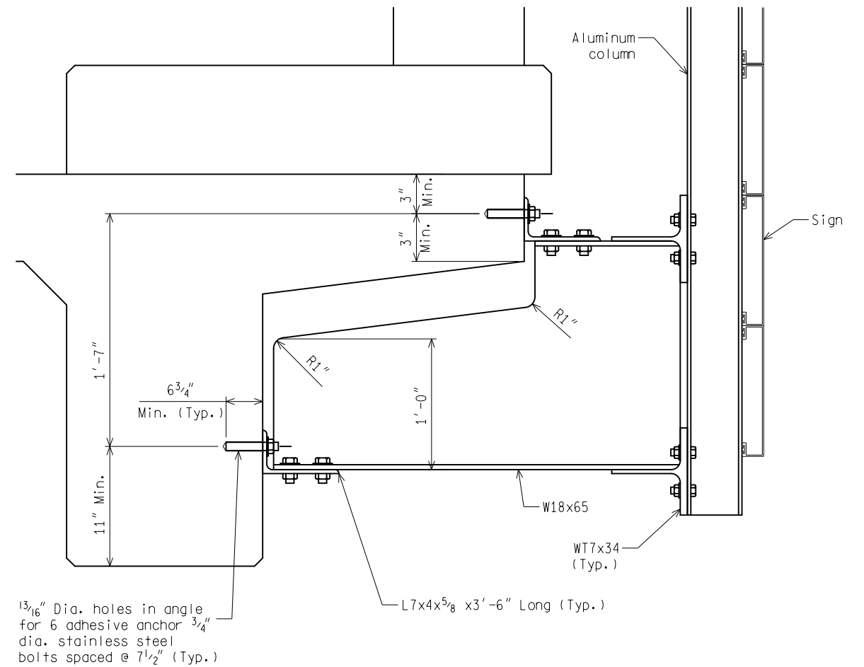
DETAIL OF CONNECTION
