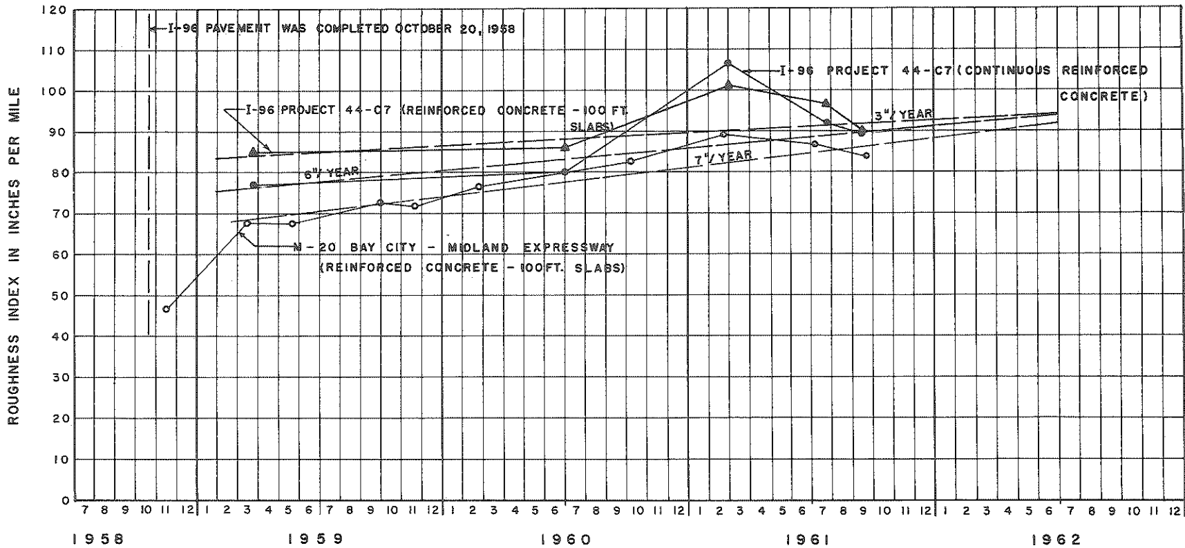
CUMULATIVE CHANGE IN ROUGHNESS ON SPECIFIC PROJECTS
