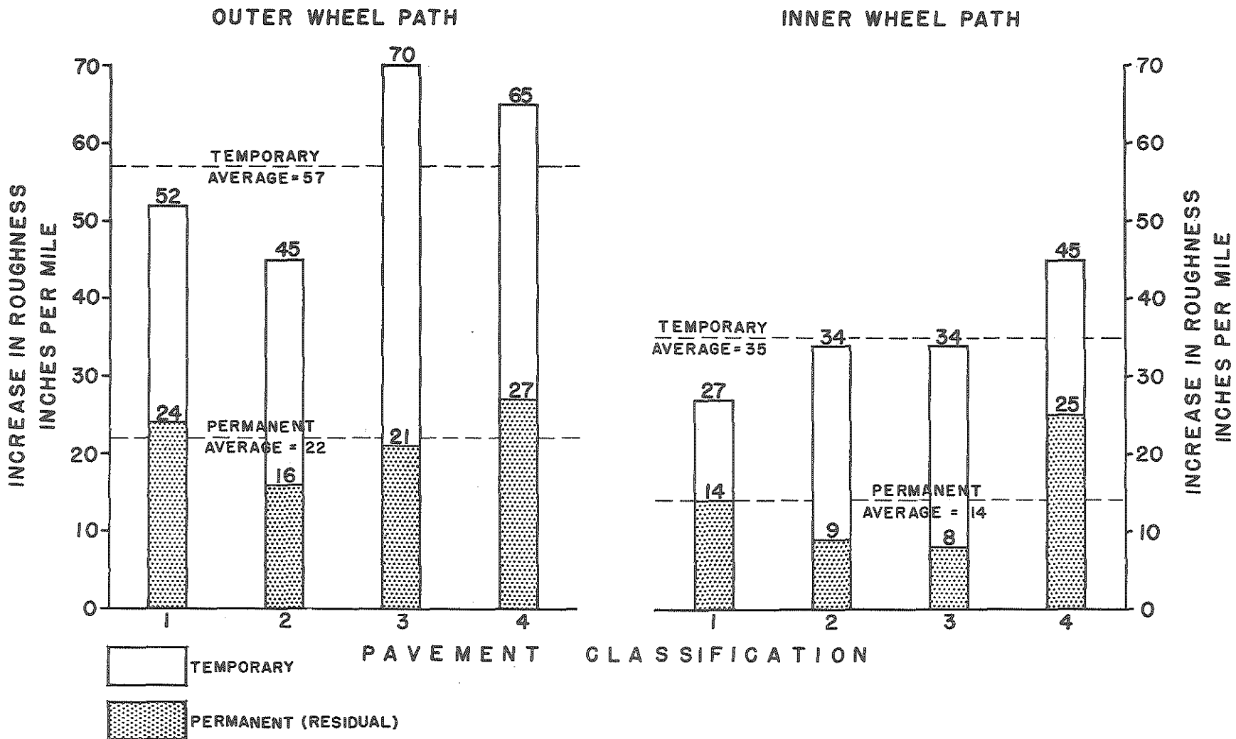
SEASONAL FLUCTUATION IN PAVEMENT PROFILE
