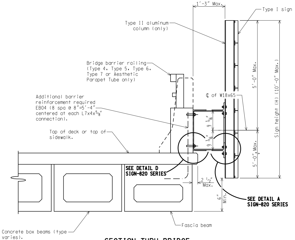
SECTION THRU BRIDGE (SEE DETAIL ON NEXT SHEET)
