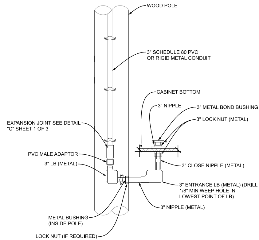
F CONTROLLER CABINET MOUNTED ON WOOD POLE N.T.S.
