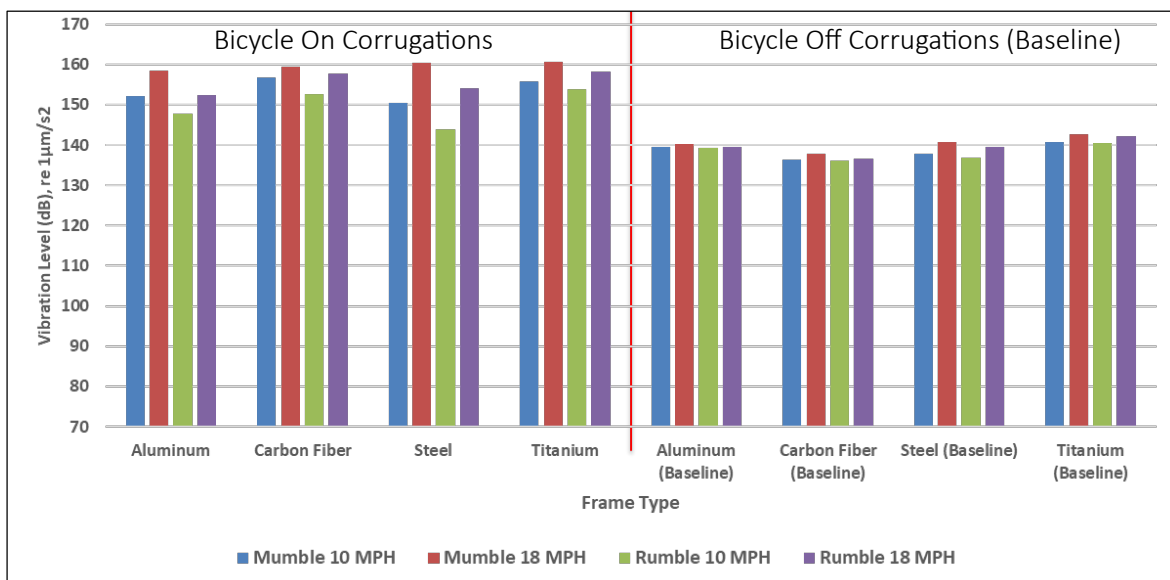
Figure 32. Maximum Total Handlebar Vibration
