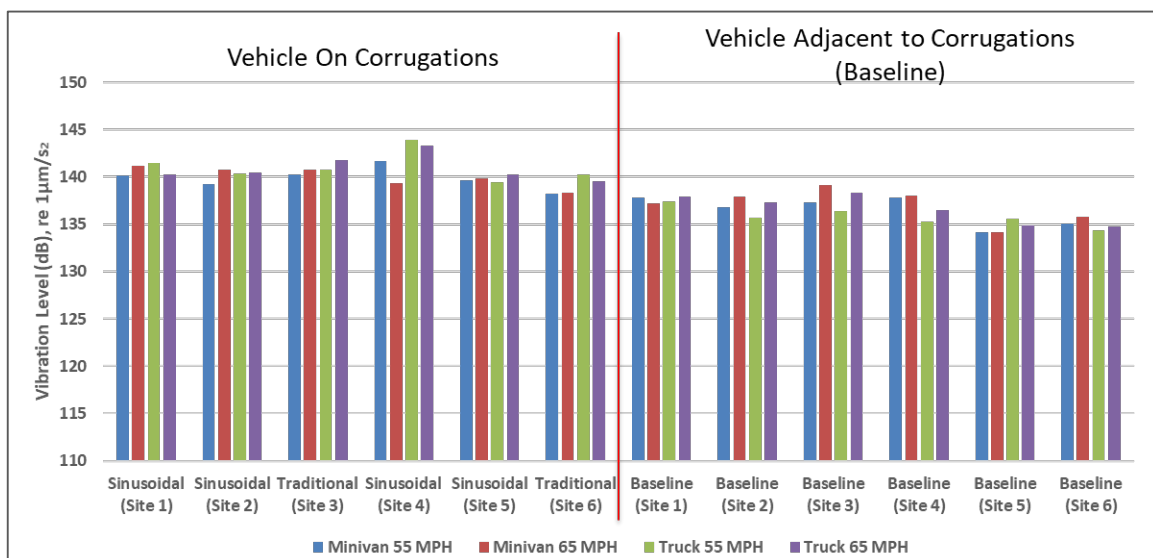
Figure 18. Maximum Vibration at Steering Column in Vertical (Z) Direction
