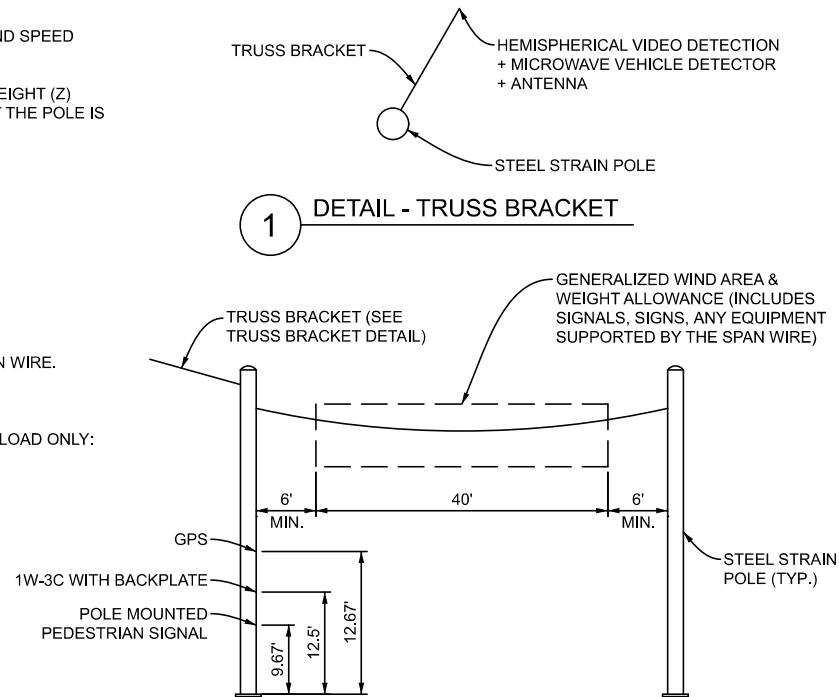
2 DETAIL - STRAIN POLE LOADING ELEVATION VIEW
