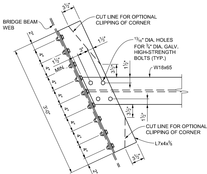
DETAIL B
