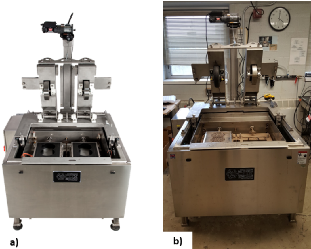
Figure 4-14 HWT device a) before modification (image from Jamescoxandsons.com) and b) after modification.
