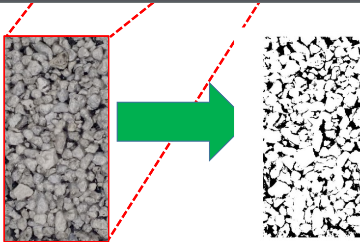
Figure 7-1 Illustration of image processing for calculating the percent binder area.
