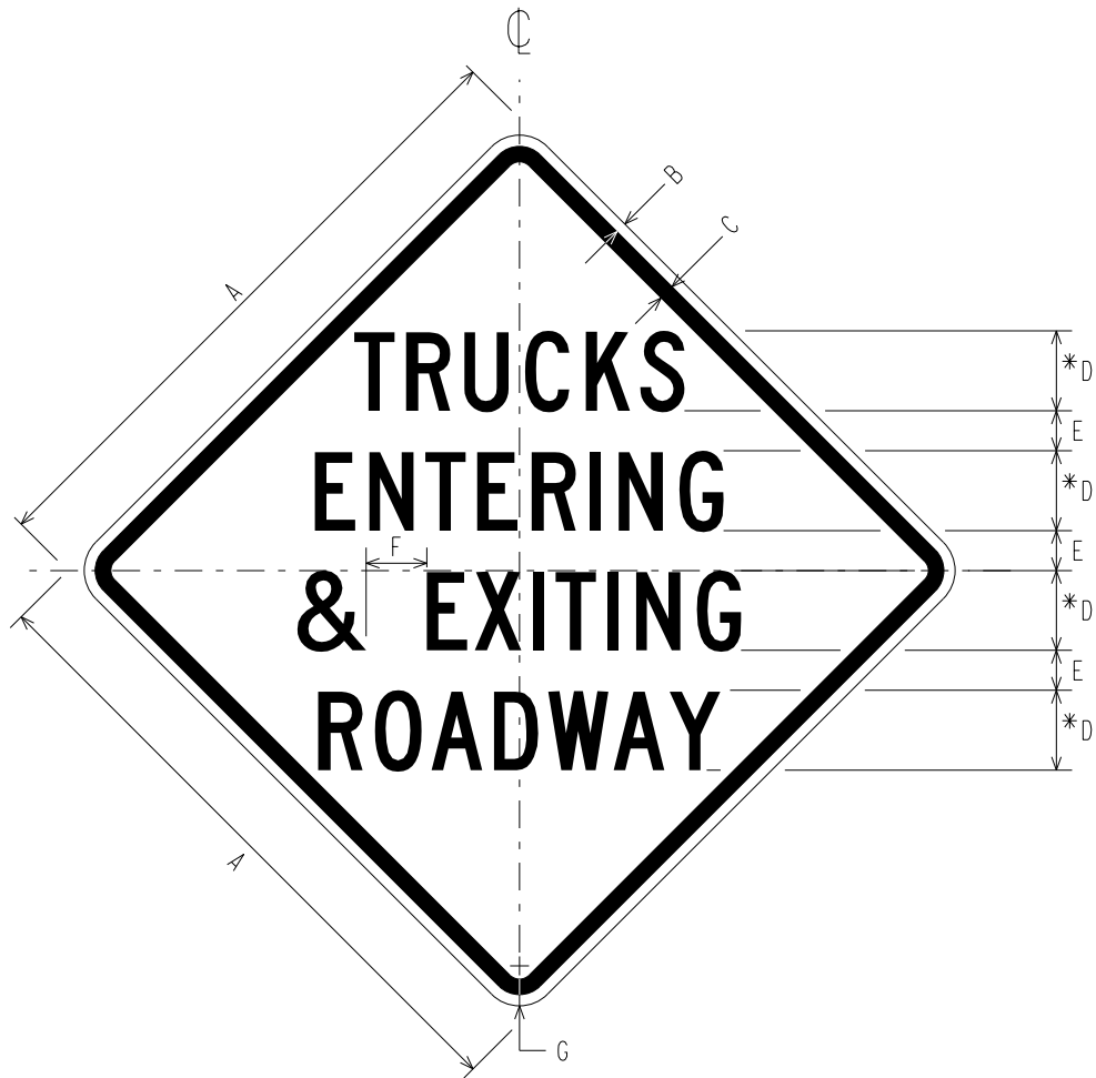
W20-16 TRUCK ENTERING & EXITING ROADWAY
