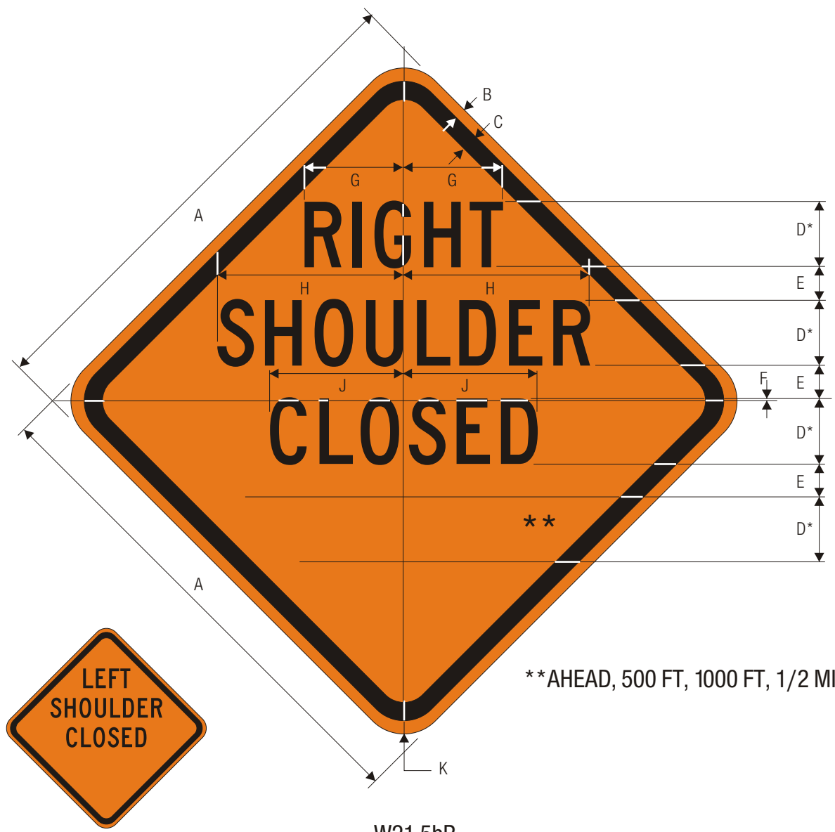
W21-5bL W21-5bR RIGHT (LEFT) SHOULDER CLOSED
