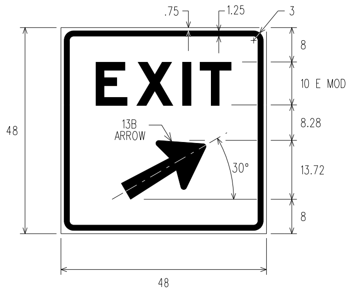
E5-1f EXIT GORE SIGN WITH ARROW
