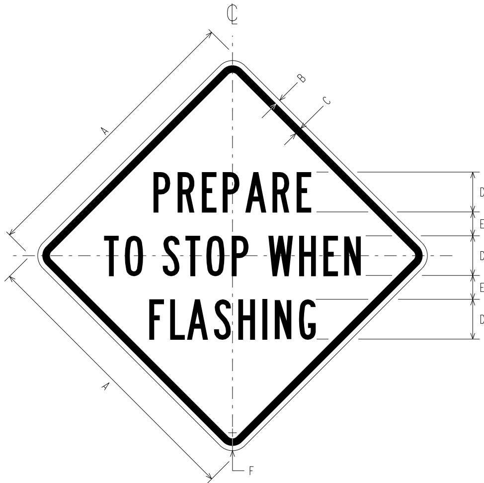
W3-4b PREPARE TO STOP WHEN FLASHING
