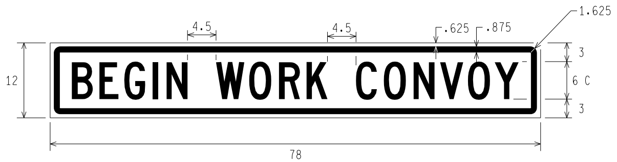
R5-18d BEGIN WORK CONVOY
