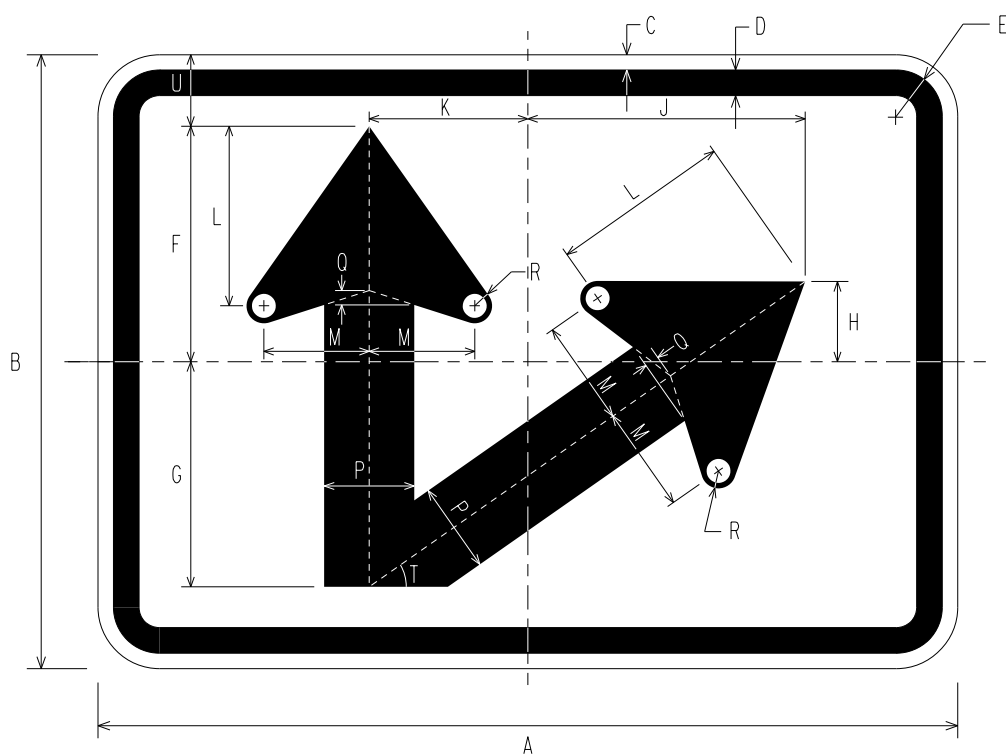
M6-7 BI-DIRECTIONAL ARROW AUXILIARY
