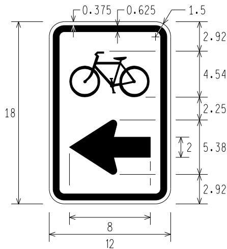
M4-9dL (R) BICYCLE SYMBOL LEFT/RIGHT ARROW DETOUR
