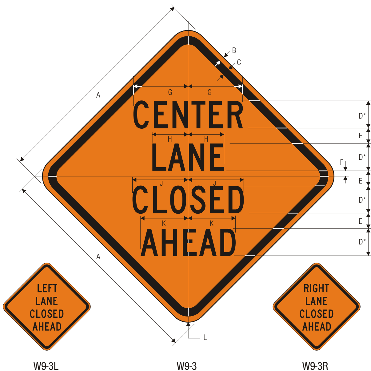
CENTER (RIGHT) (LEFT) LANE CLOSED AHEAD
