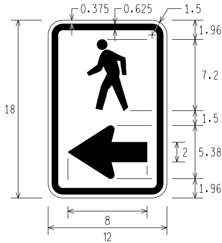
M4-9gL (R) PEDESTRIAN SYMBOL LEFT/RIGHT ARROW DETOUR
