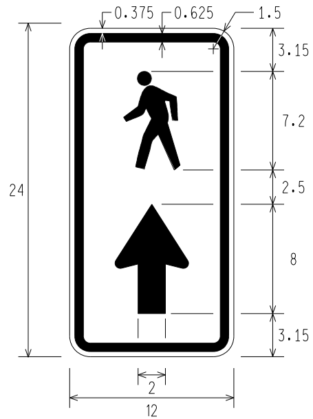
M4-9h PEDESTRIAN SYMBOL UP ARROW DETOUR
