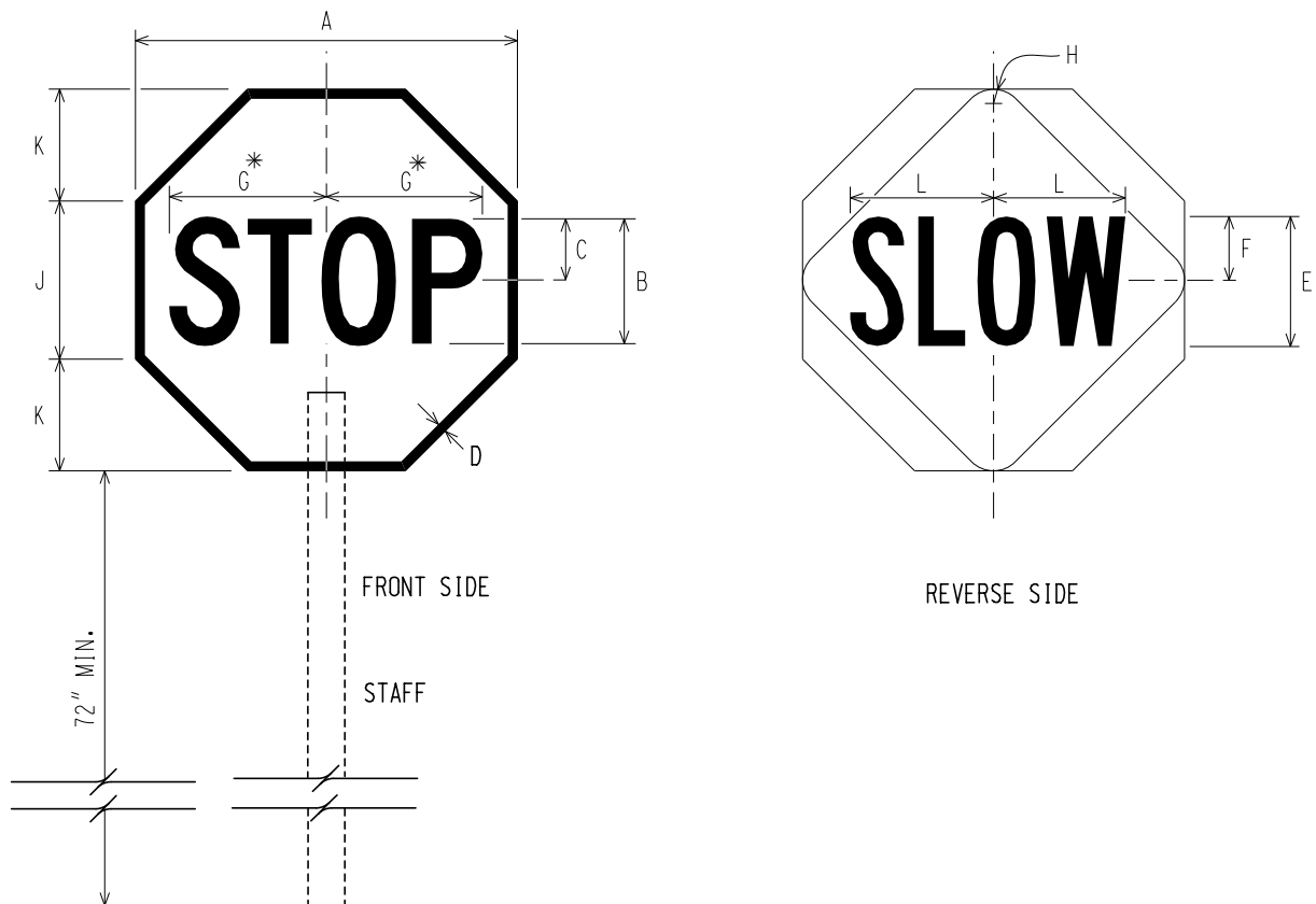
R1-1a STOP-SLOW PADDLE
