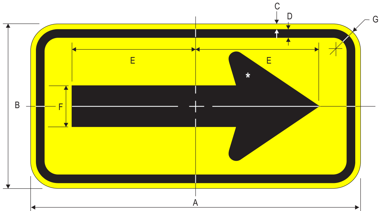
W1-6R DIRECTION LARGE ARROW
