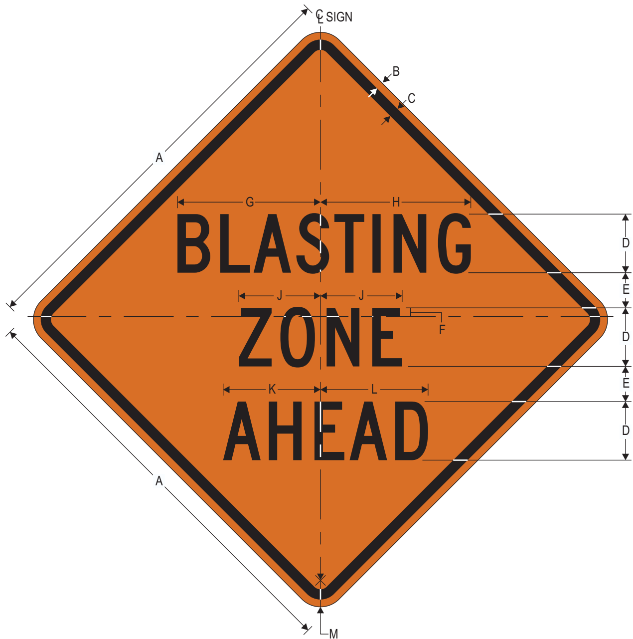
W22-1 BLASTING ZONE AHEAD
