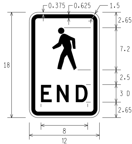
M4-9i PEDESTRIAN SYMBOL END DETOUR
