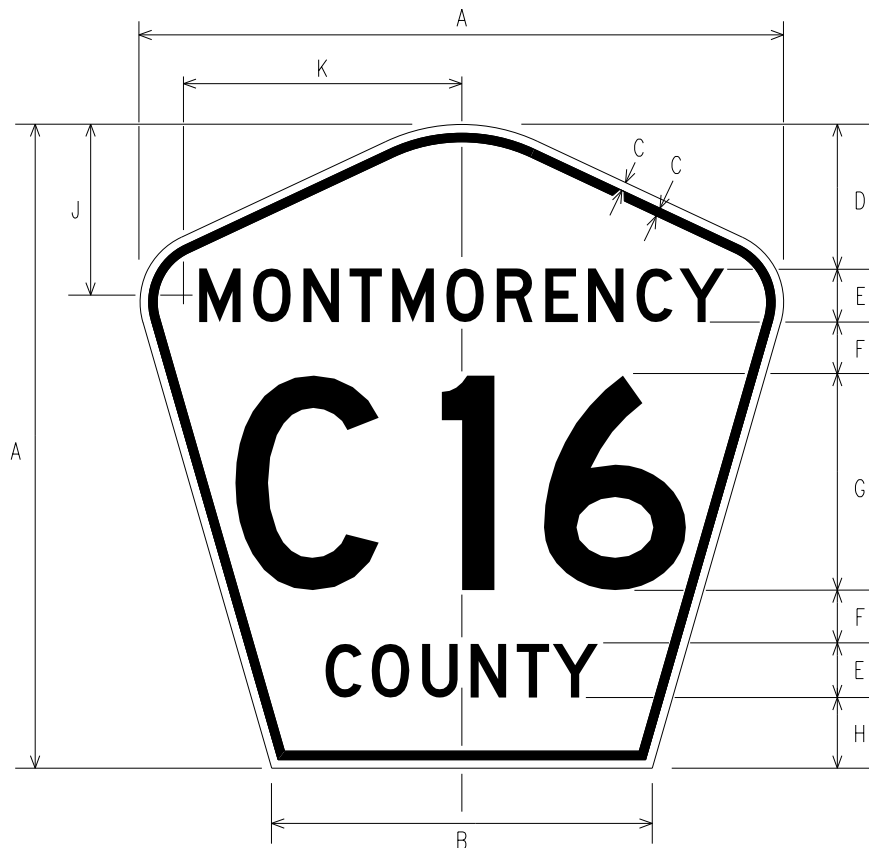
M1-5 COUNTY ROUTE MARKER
