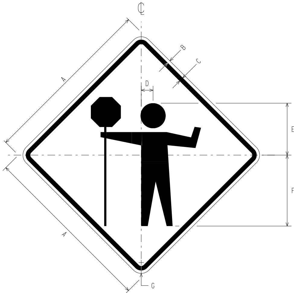
W20-7a TRAFFIC REGULATOR SYMBOL
