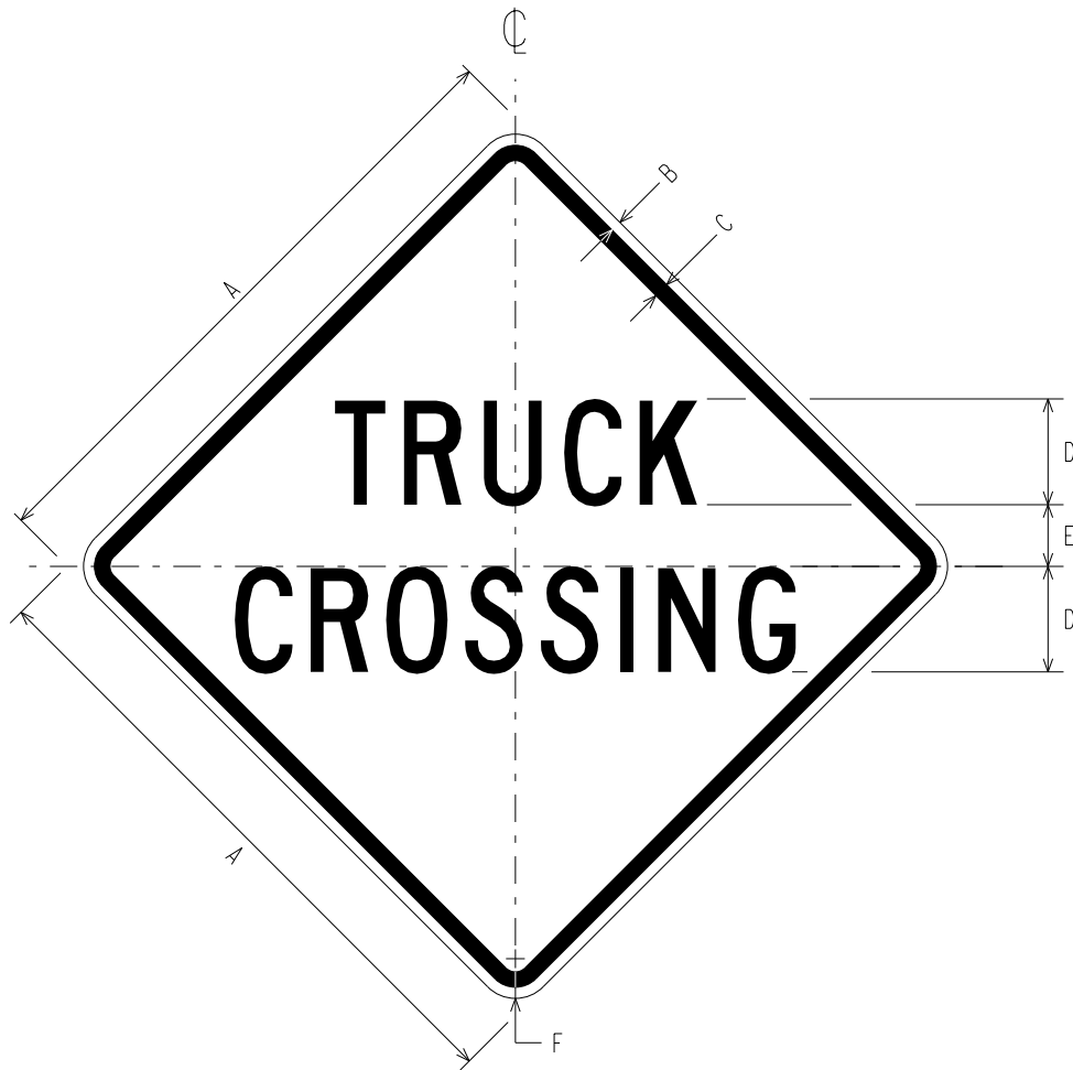
W11-10a TRUCK CROSSING TEXT
