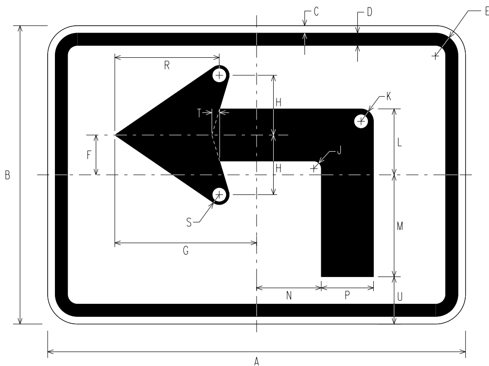
M5-1 (L) ADVANCE TURN ARROW AUXILIARY
