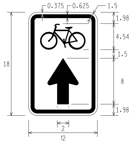
M4-9e BICYCLE SYMBOL UP ARROW DETOUR
