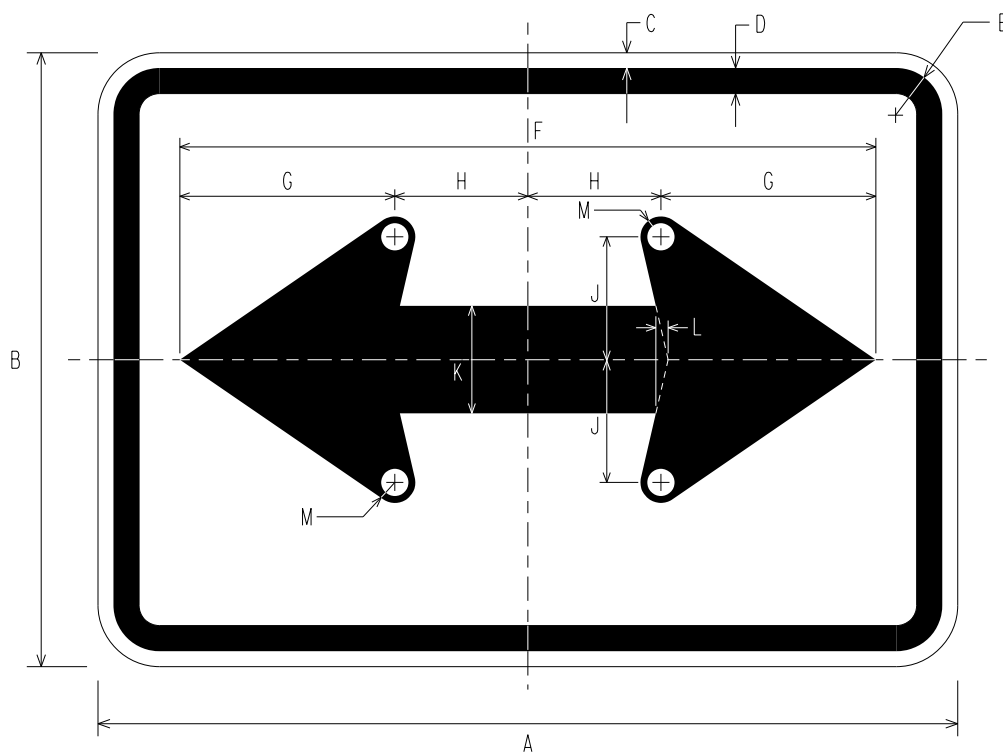
M6-4 BI-DIRECTIONAL ARROW AUXILIARY
