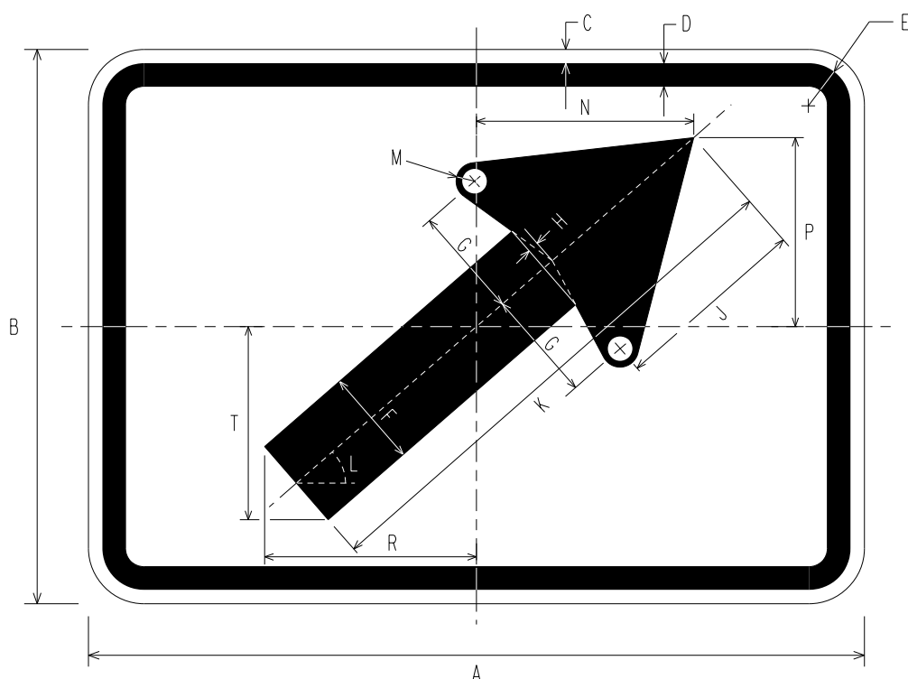
M6-2 ( R ) DIRECTIONAL ARROW AUXILIARY
