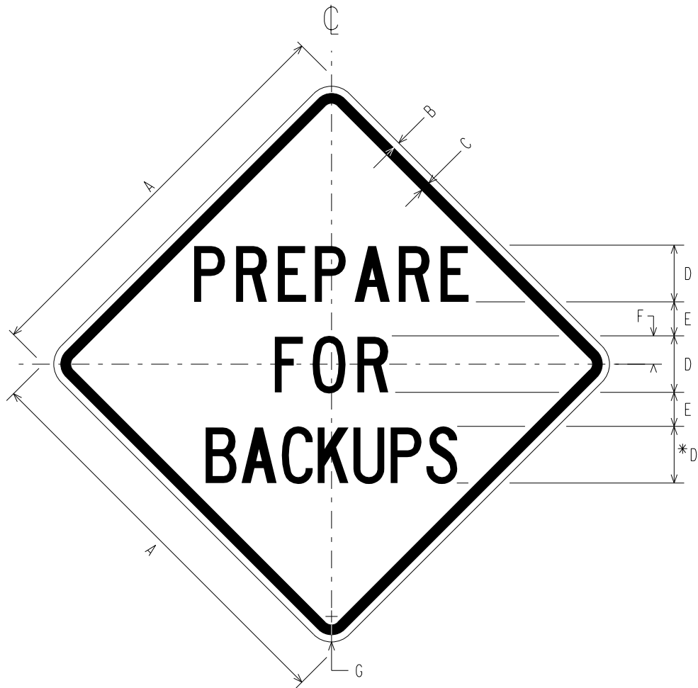
W20-15a PREPARE FOR BACKUPS
