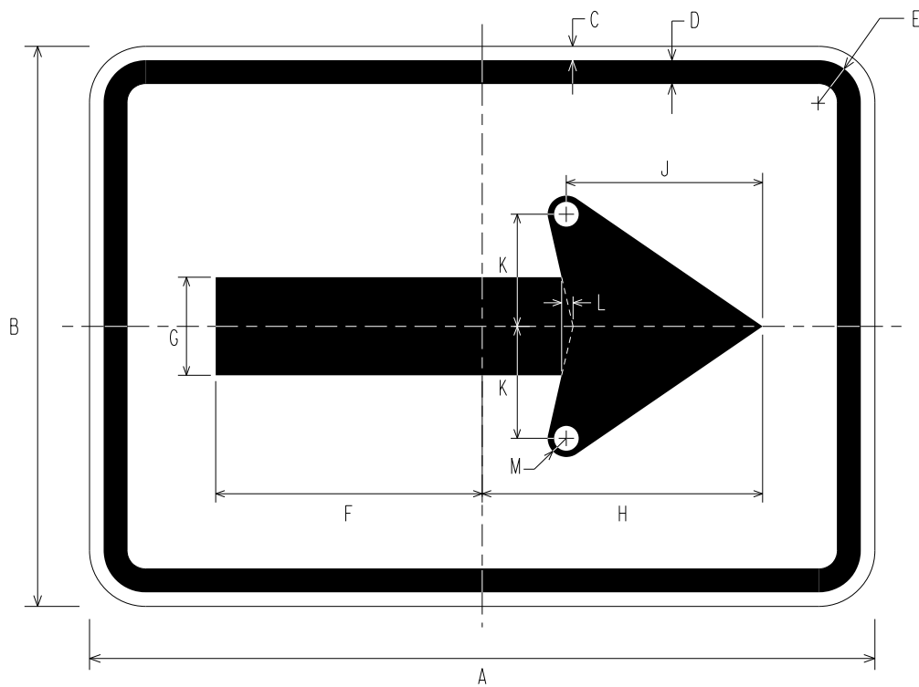
M6-1 ( R ) DIRECTIONAL ARROW AUXILIARY
