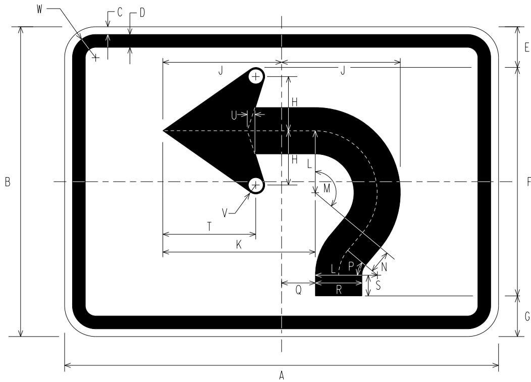
M5-3 ADVANCE TURN ARROW AUXILIARY - CIRCULAR INTERSECTION
