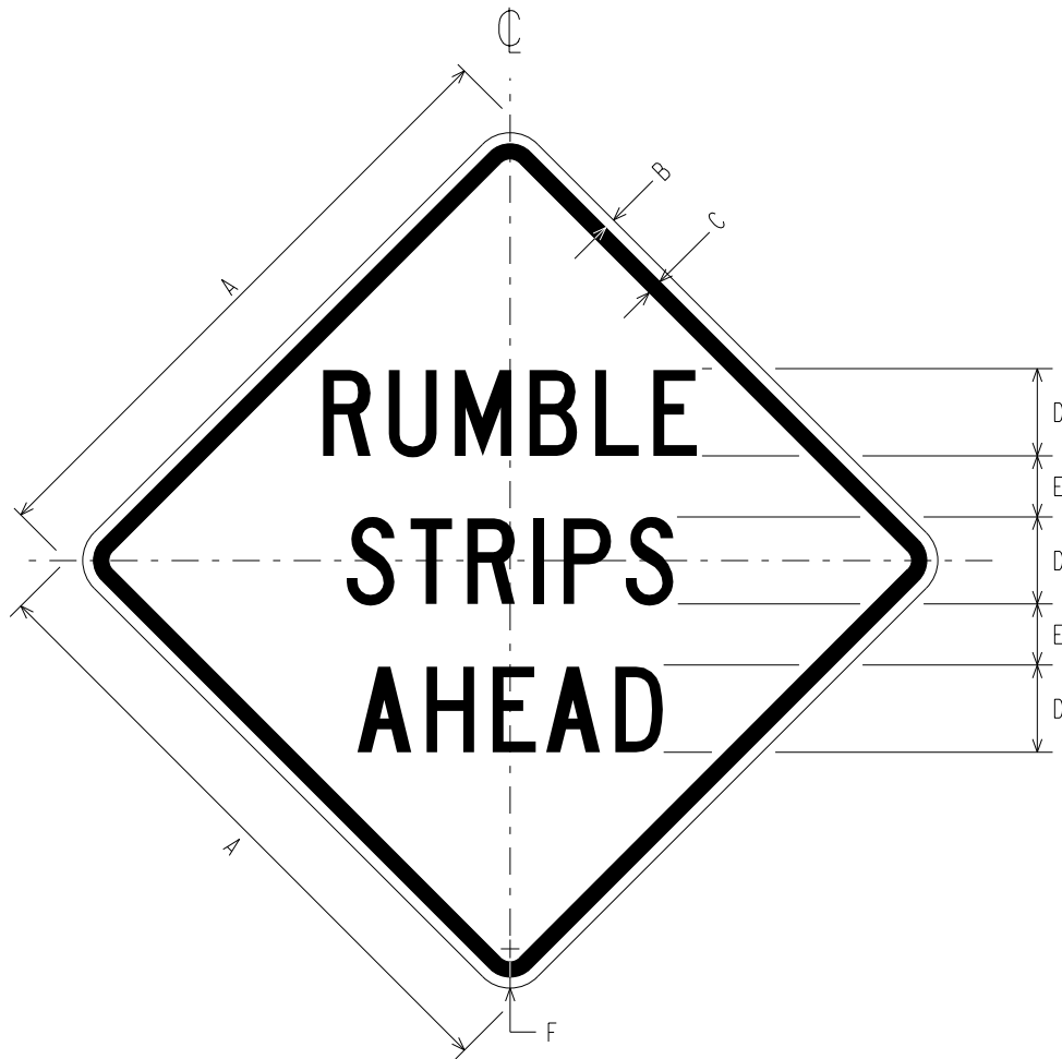
W8-26 RUMBLE STRIPS AHEAD
