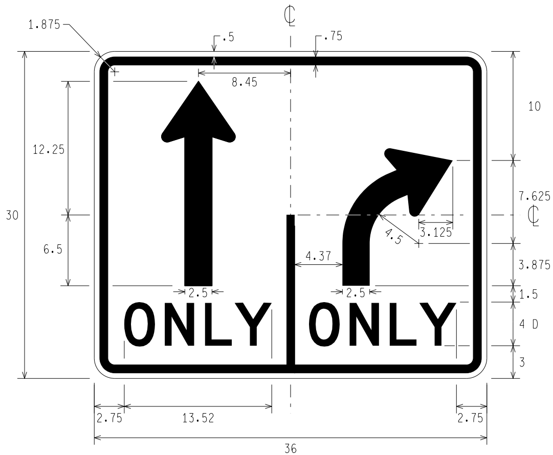
R3-8d THROUGH ONLY, RIGHT ONLY
