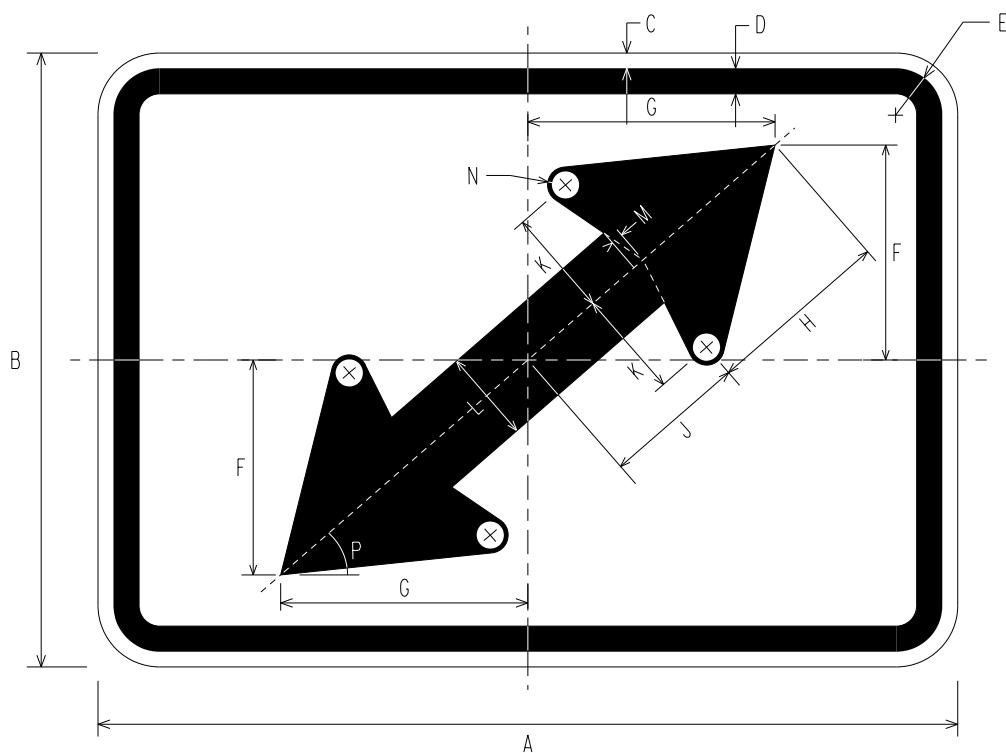
M6-5 BI-DIRECTIONAL ARROW AUXILIARY
