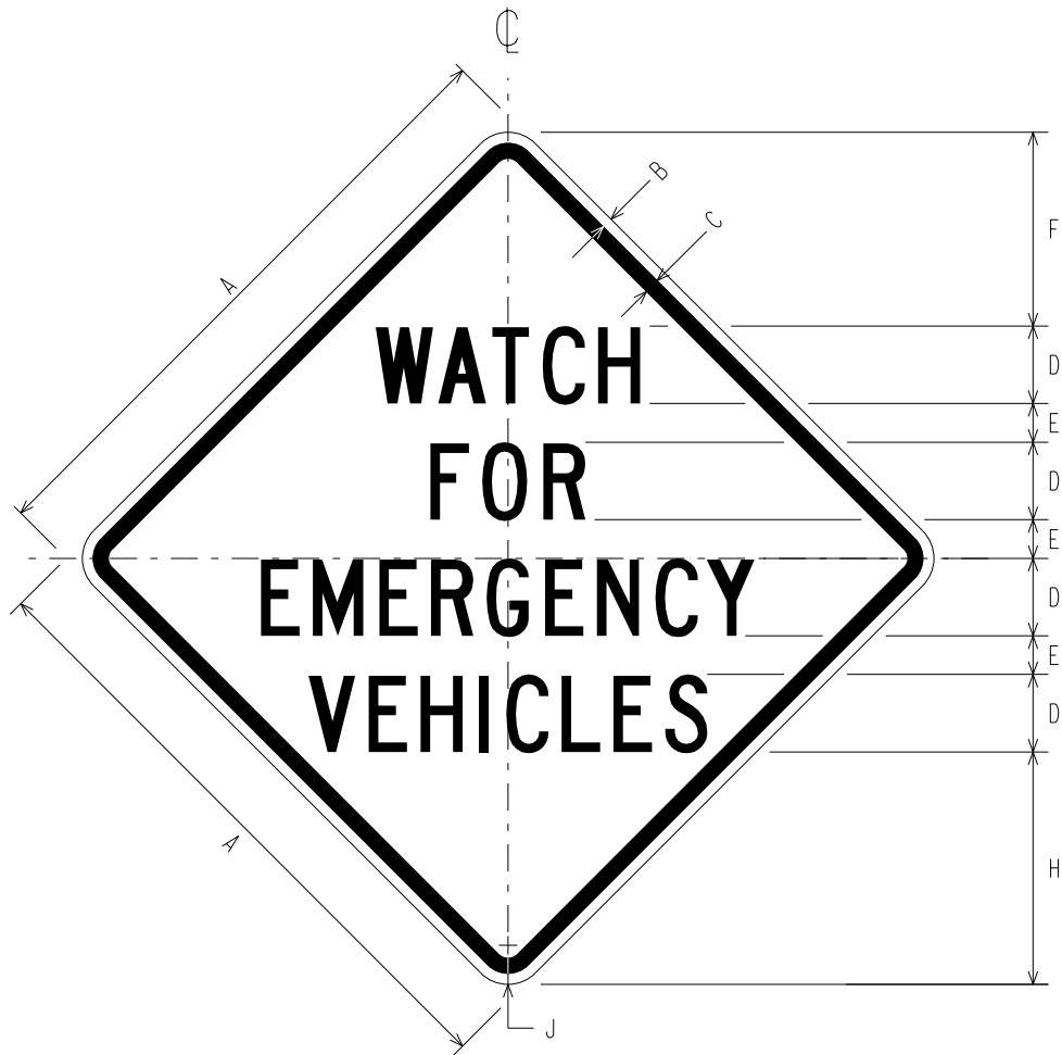
W20-4c WATCH FOR EMERGENCY VEHICLES
