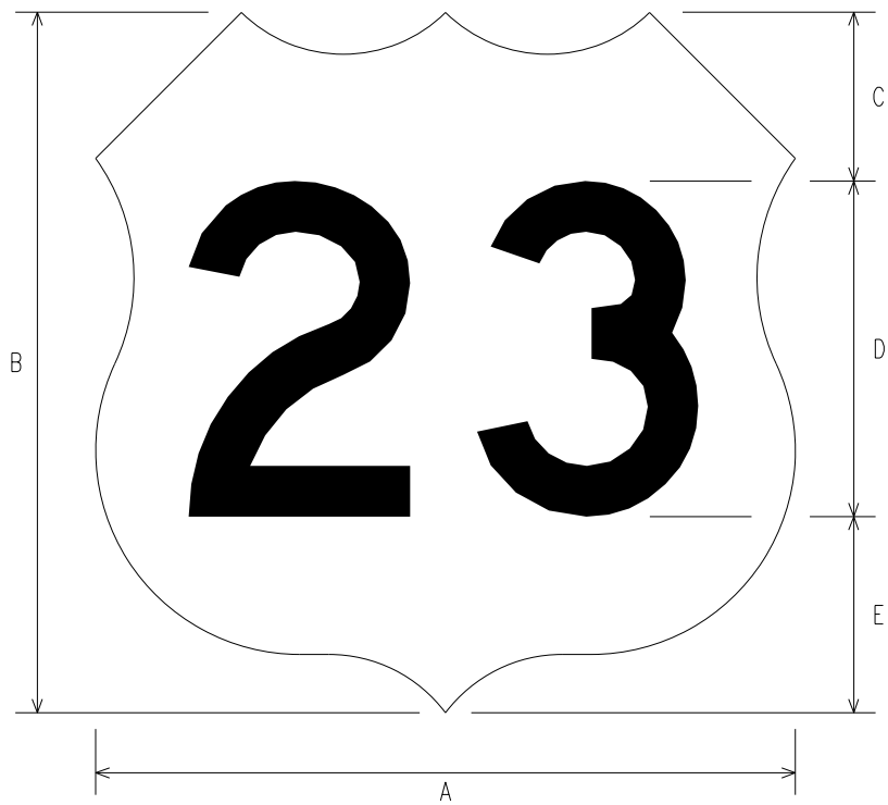
M1-4a U.S. ROUTE MARKER (FOR GUIDE SIGN USE)
