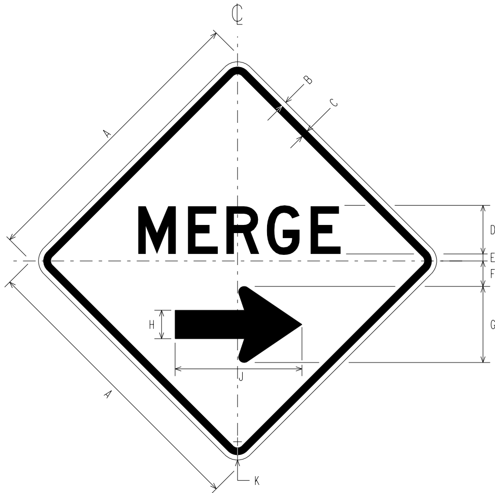
W20-14 LATE MERGE
