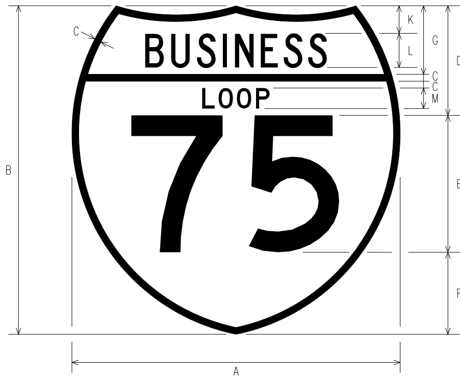
M1-2 OFF-INTERSTATE BUSINESS ROUTE (LOOP) MARKER
