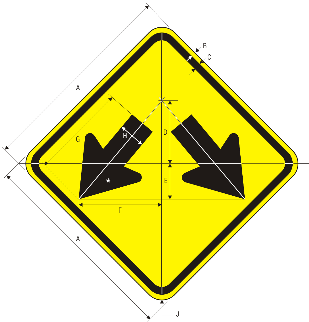
W12-1 DOUBLE ARROW
