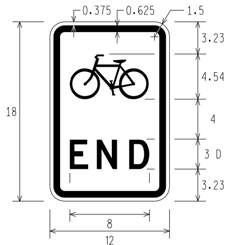
M4-9f BICYCLE SYMBOL END DETOUR
