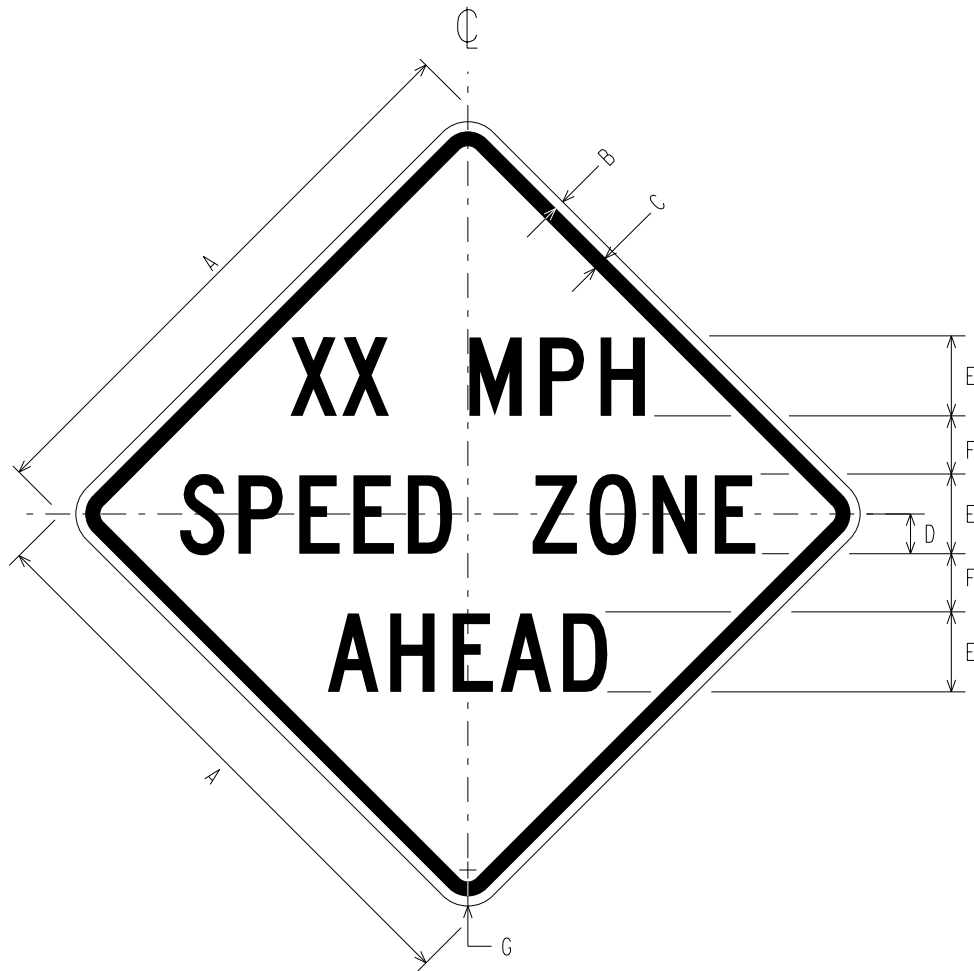
W3-5a SPEED REDUCTION
