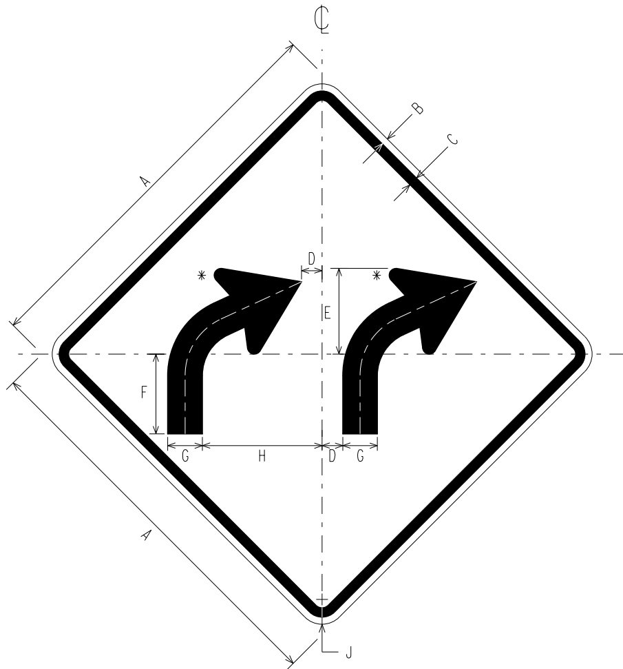
W1-2b TWO LANE CURVE SIGN
