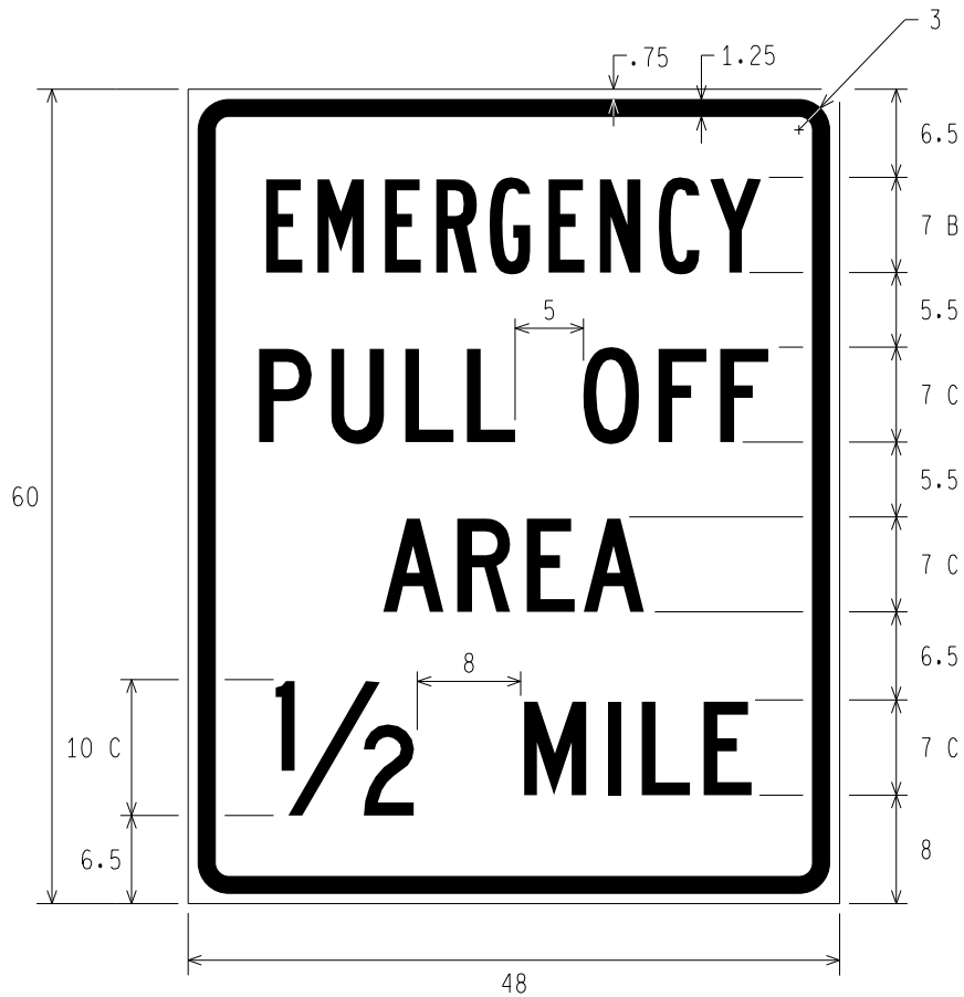
W20-18 EMERGENCY PULL OFF AREA 1/2 MILE
