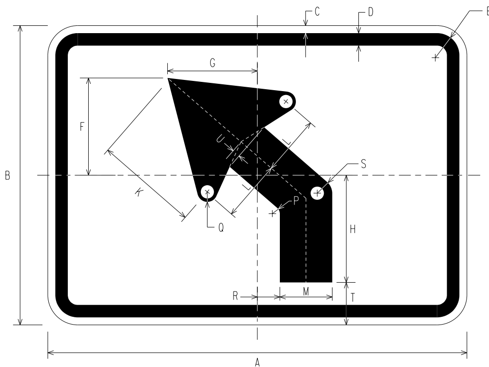
M5-2(L) ADVANCE TURN ARROW AUXILIARY
