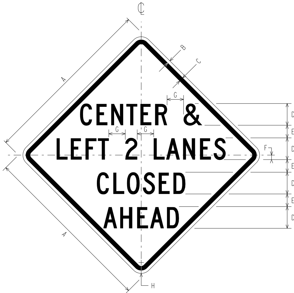
W9-3b CENTER & LEFT 2 LANES CLOSED AHEAD
