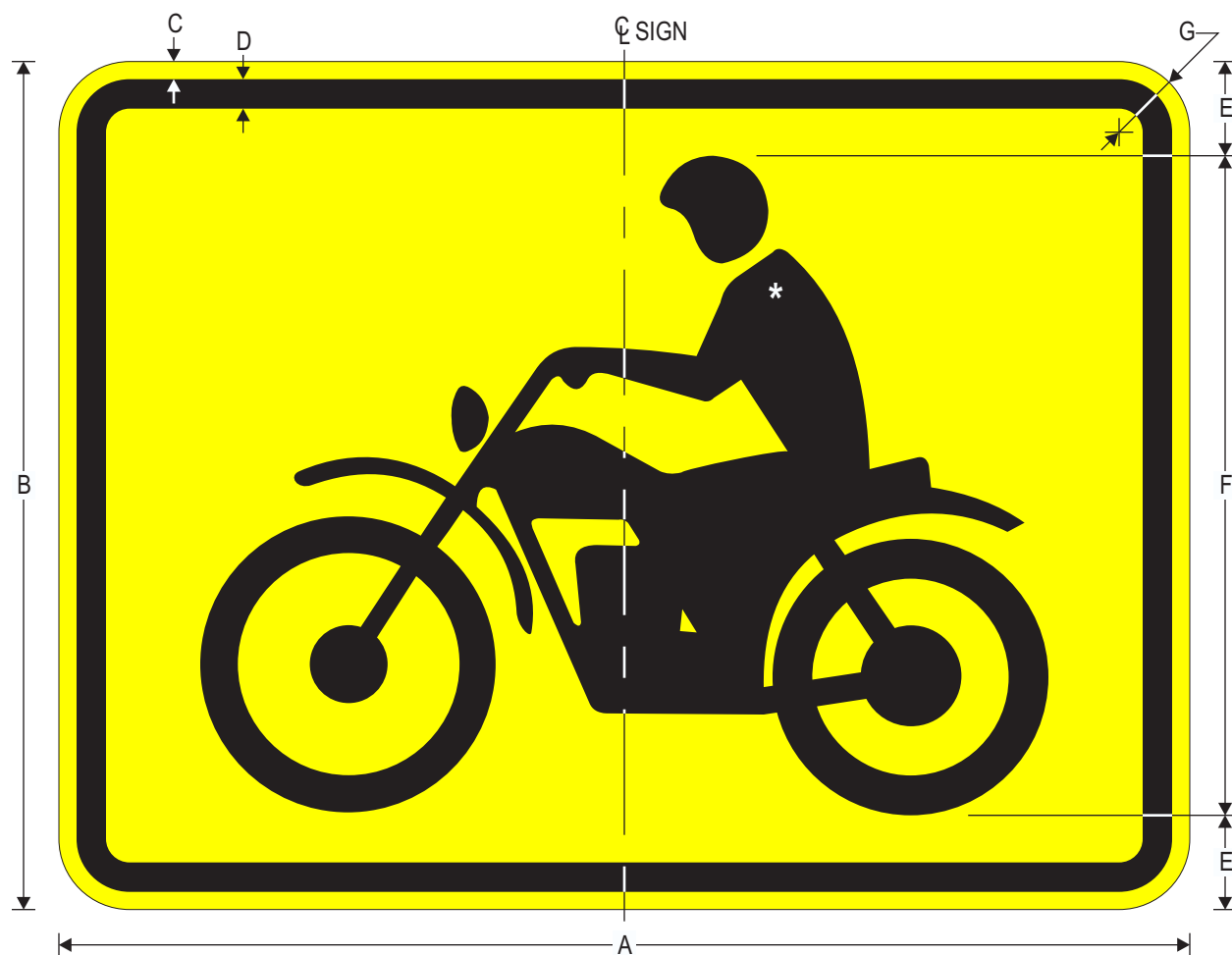
W8-15P MOTORCYCLE (PLAQUE)
