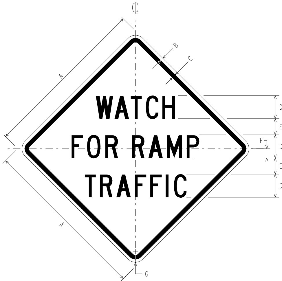
W11-24 WATCH FOR RAMP TRAFFIC
