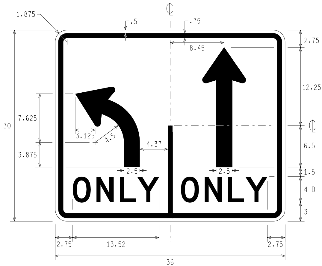
R3-8c LEFT ONLY, THROUGH ONLY
