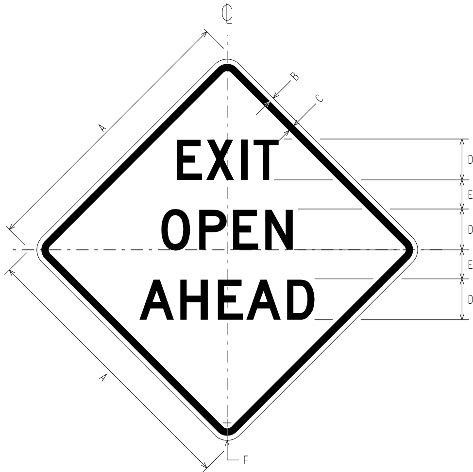
W20-17 EXIT OPEN AHEAD
