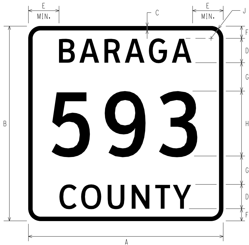
M1-5a INTER COUNTY ROUTE MARKER
