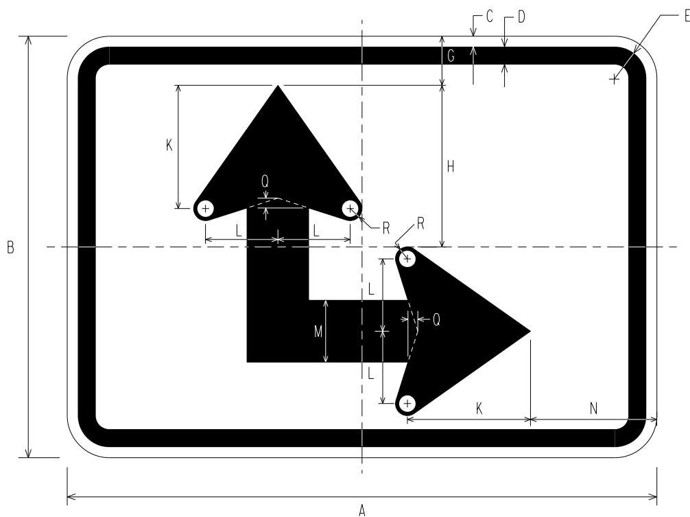
M6-6 BI-DIRECTIONAL ARROW AUXILIARY
