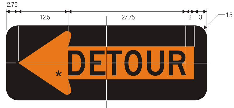
M4-10L DETOUR (INSIDE ARROW)
