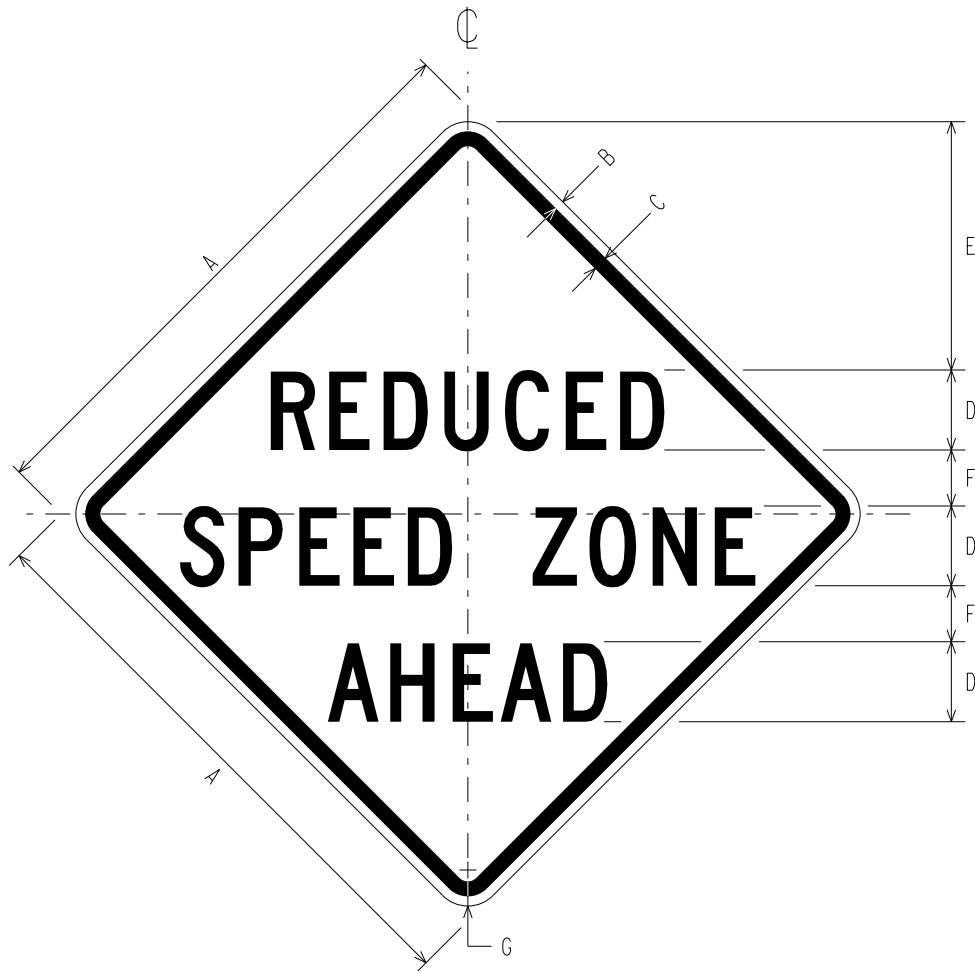
W3-5b REDUCED SPEED ZONE AHEAD
