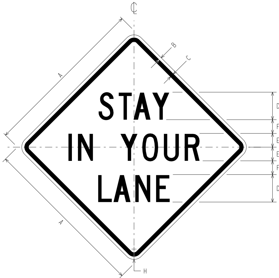
W20-15 STAY IN YOUR LANE
