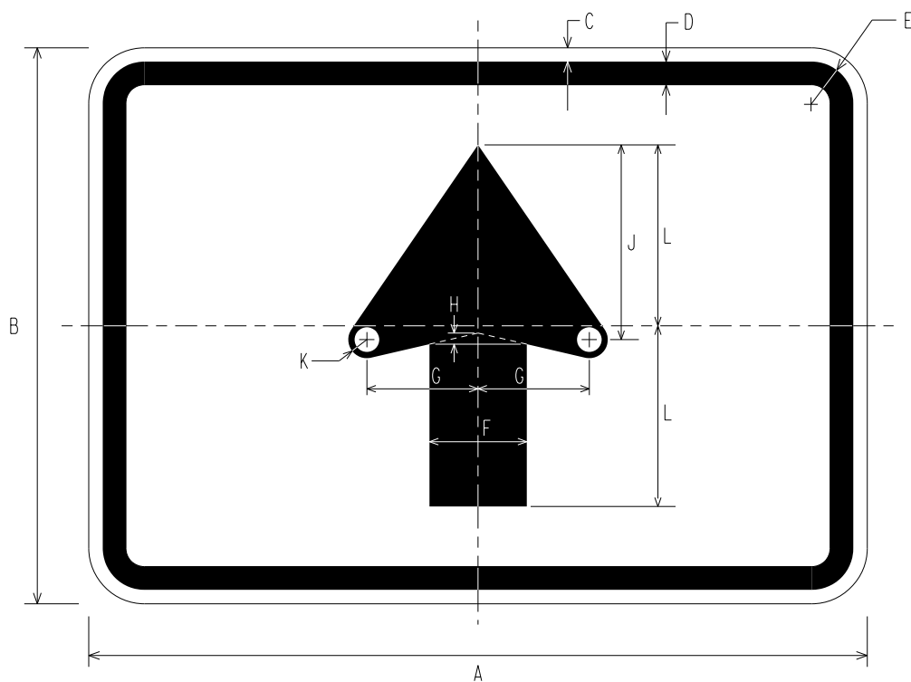
M6-3 DIRECTIONAL ARROW AUXILIARY
