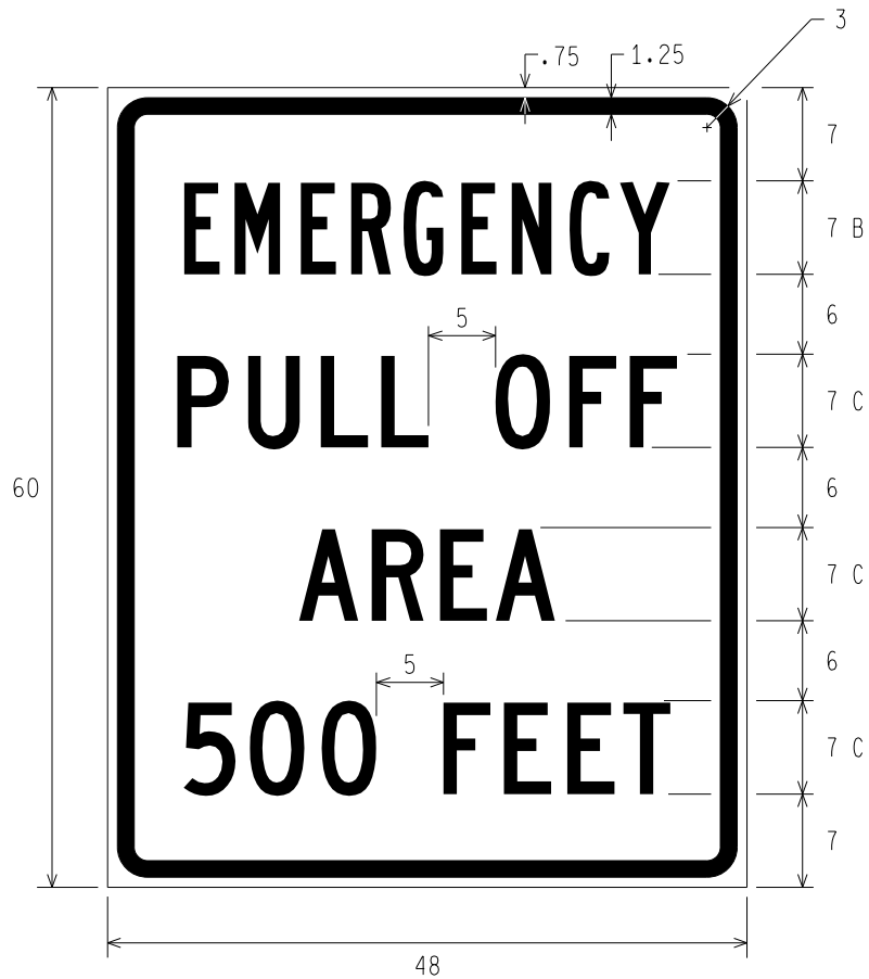
W20-18a EMERGENCY PULL OFF AREA 500 FEET
