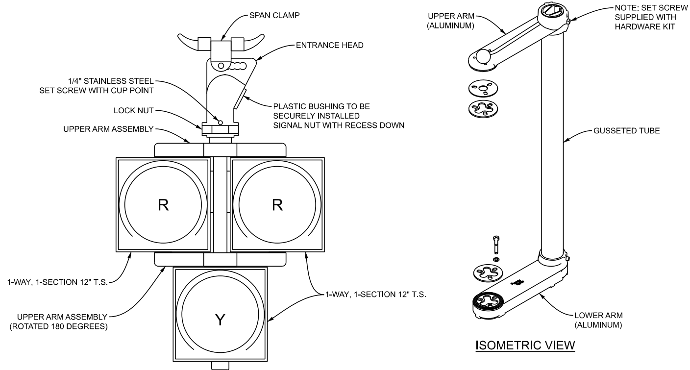
SPAN WIRE DISPLAY
