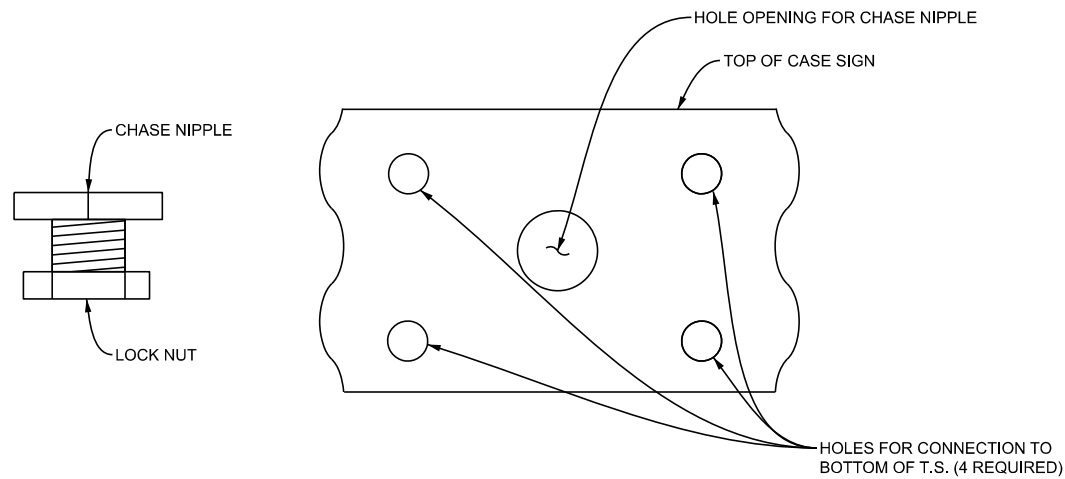
A DETAIL - ALTERNATE SIGNAL JOINER DETAIL N.T.S.
