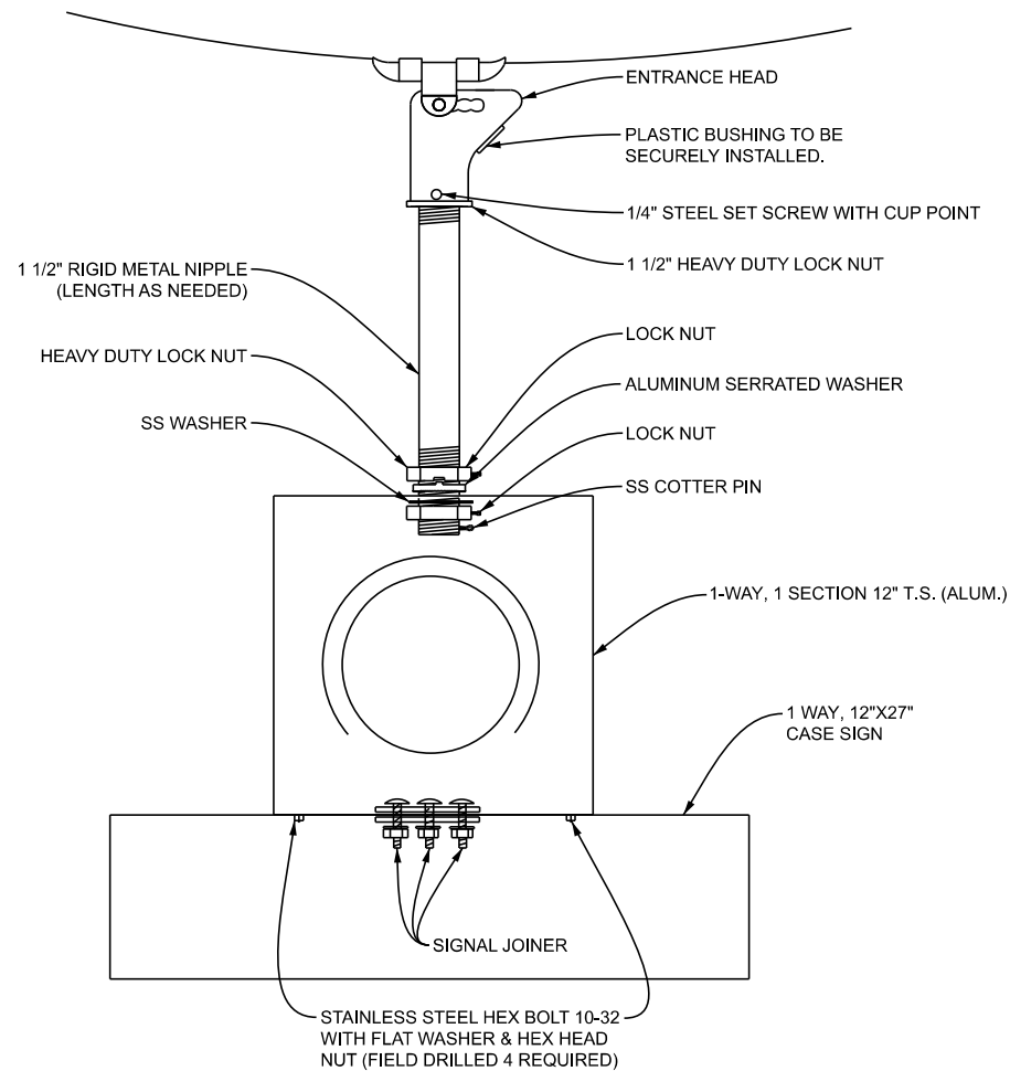
B DETAIL - T.S. MOUNTED ON CASE SIGN N.T.S.
