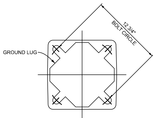
B DETAIL - SQUARE BASE BOTTOM PLAN N.T.S.
