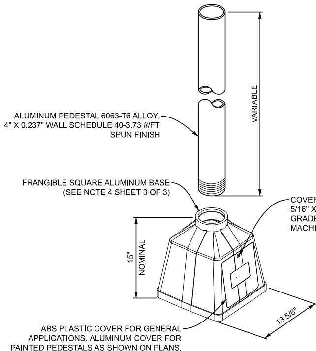
A DETAIL - SQUARE ALUMINUM BASE N.T.S.
