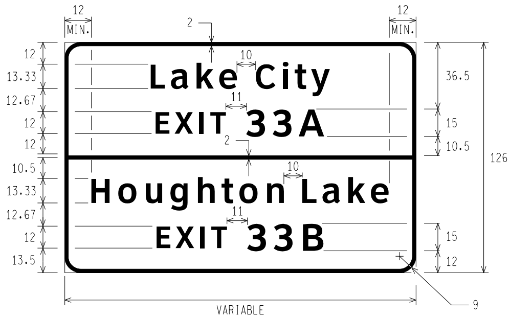
E3-1e DESTINATION NEXT RIGHT DESTINATION SECOND RIGHT
