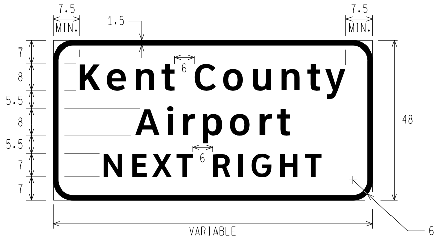
E3-1i VARIABLE (2 LINES) NEXT RIGHT
