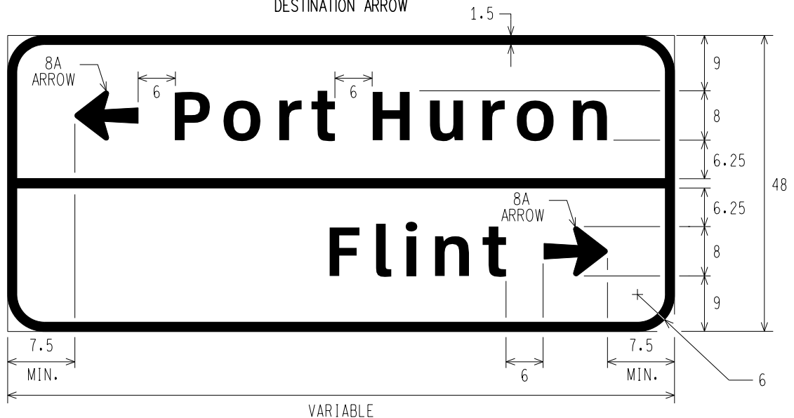
E11-4b DOUBLE DESTINATION AND ARROW
