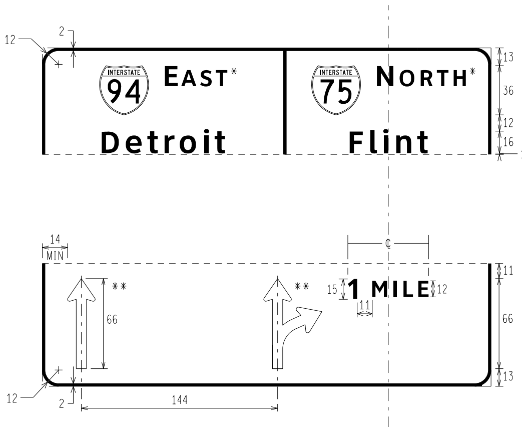
E1-1p PANEL I ROUTE MARKER CARDINAL DIRECTION DESTINATION DISTANCE TWO ARROW ASSIGNMENTS
