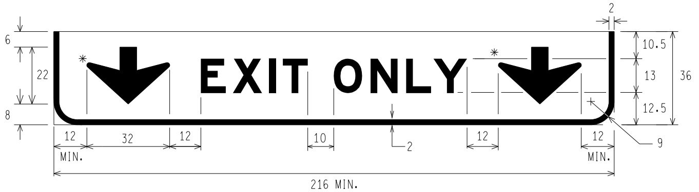
E11-1f LANE ARROW EXIT ONLY LANE ARROW
