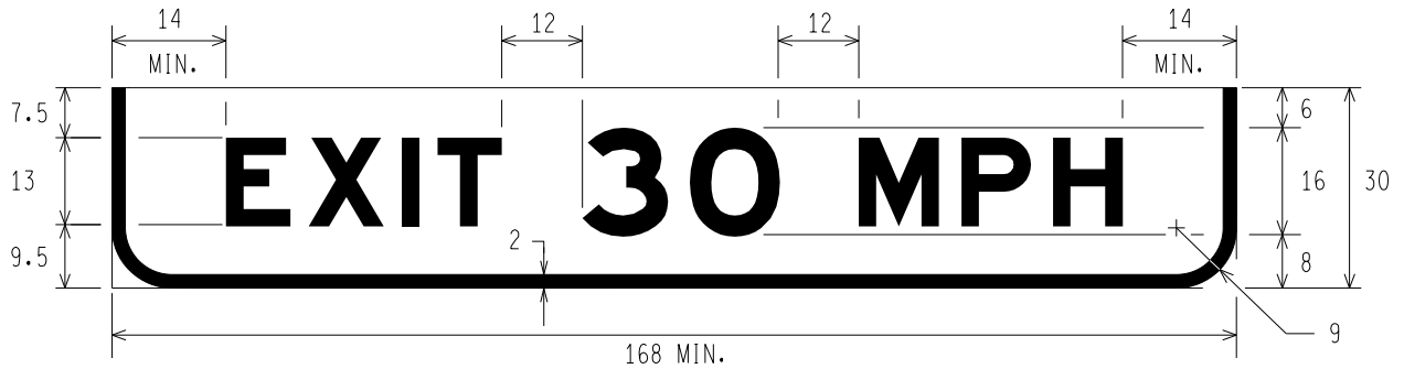
E13-2 EXIT SPEED ADVISORY
