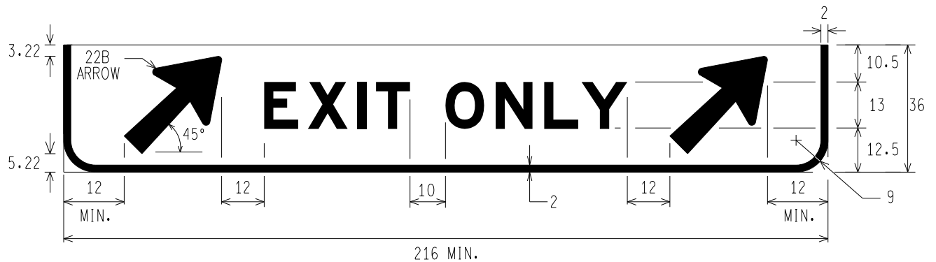
E11-1e ANGLED ARROW EXIT ONLY ANGLED ARROW
