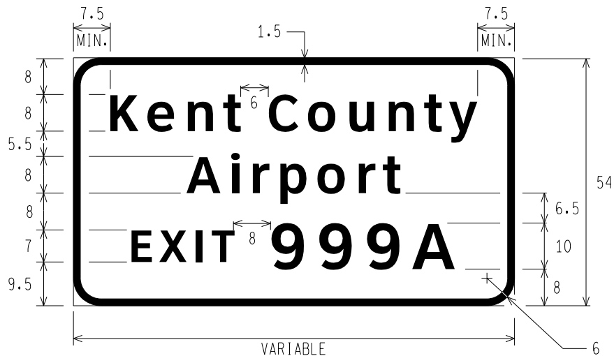
E3-1j VARIABLE (2 LINES) EXIT
