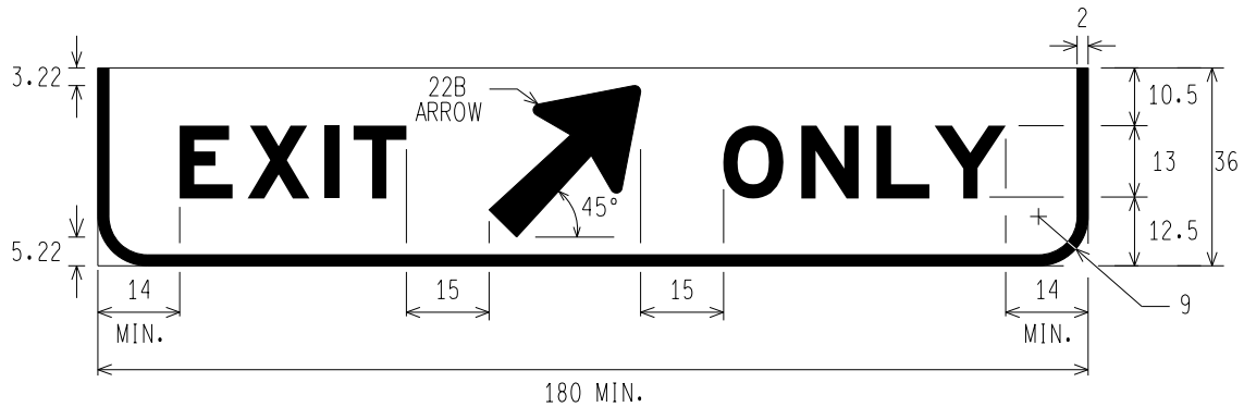
E11-1d EXIT ANGLED ARROW ONLY
