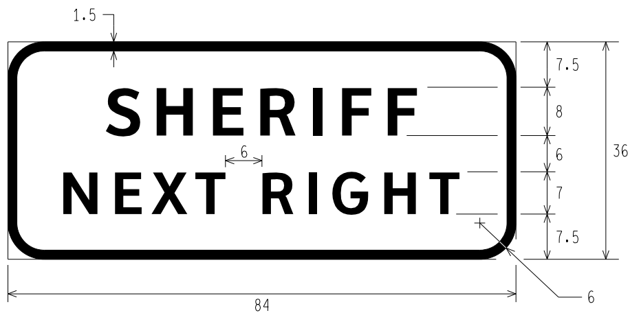
E11-9d SHERIFF NEXT RIGHT
