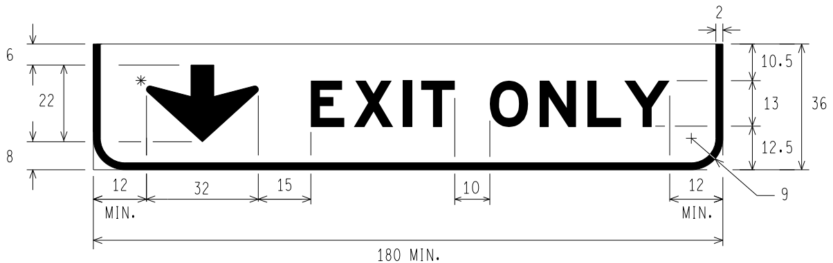
E11-1g LANE ARROW EXIT ONLY
