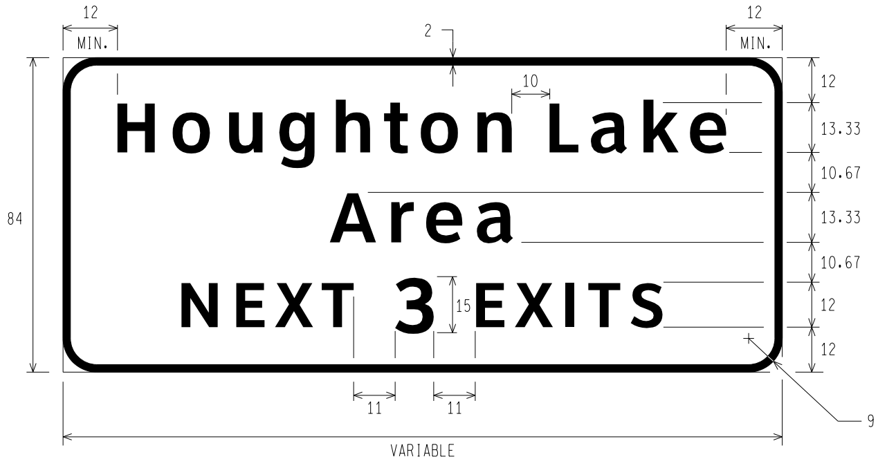
E9-1b TWO LINE DESTINATION NEXT EXITS
