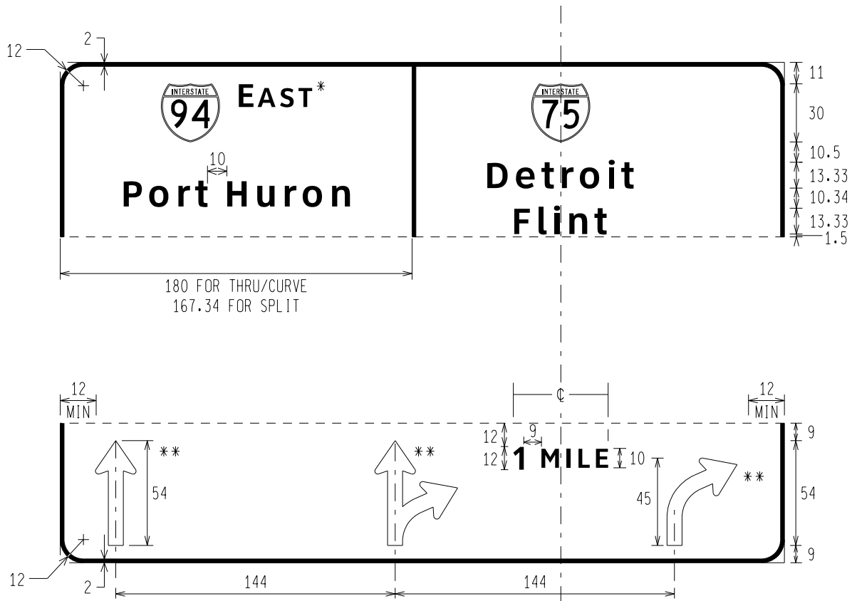
E1-1t PANEL II ROUTE MARKER CARDINAL DIRECTION DOUBLE DESTINATION DISTANCE THREE ARROW ASSIGNMENTS
