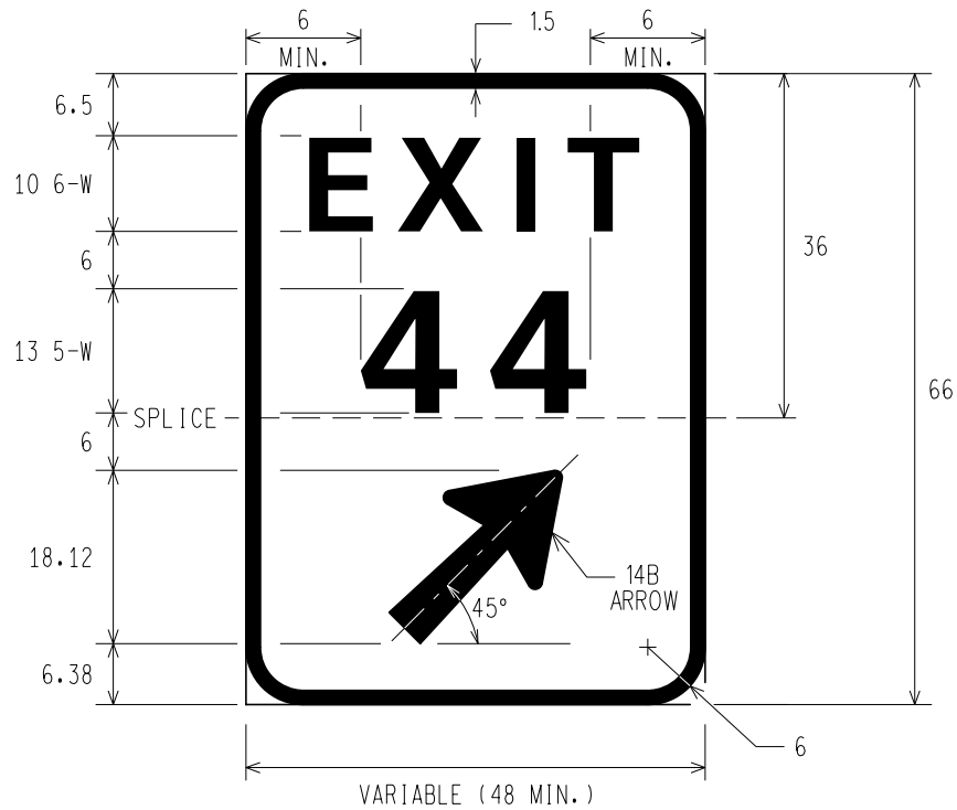
E5-1e EXIT GORE SIGN ADDITIONAL OPTION
