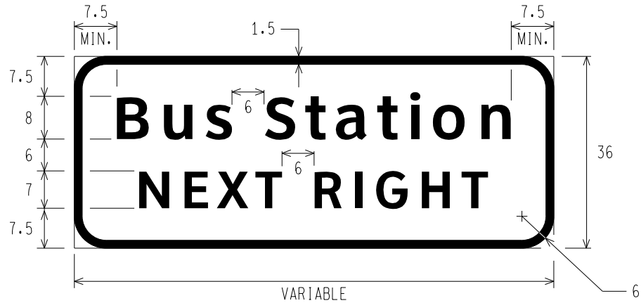
E3-1g VARIABLE (1 LINE) NEXT RIGHT
