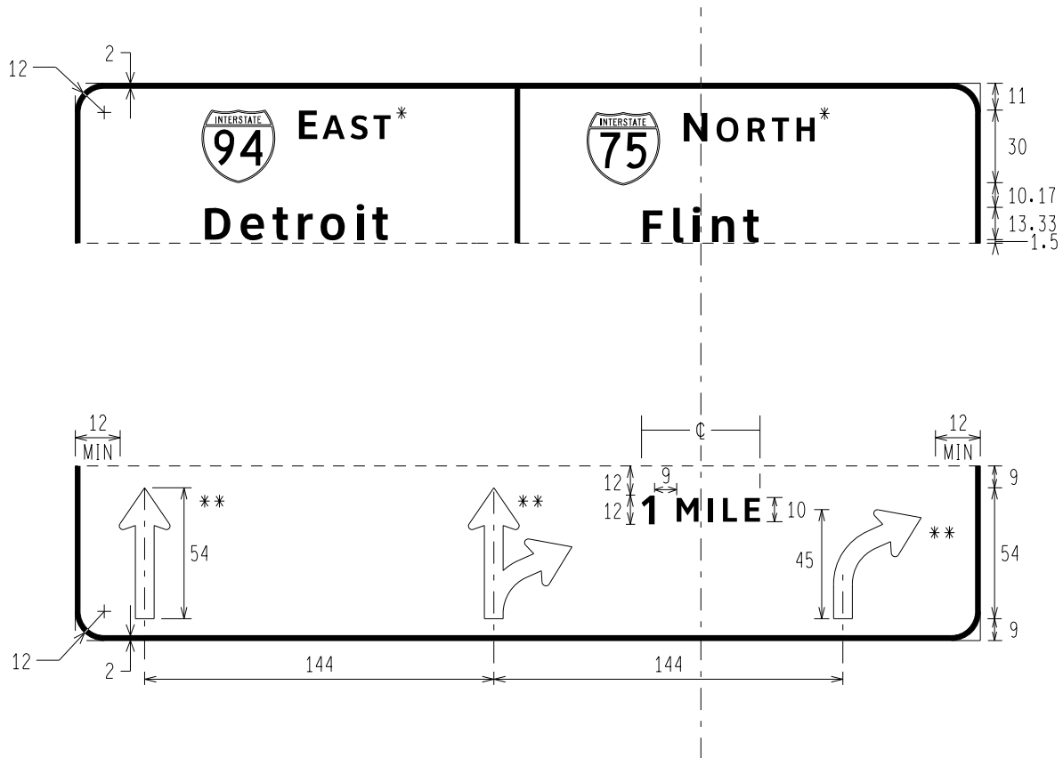
E1-1s PANEL II ROUTE MARKER CARDINAL DIRECTION DESTINATION DISTANCE THREE ARROW ASSIGNMENTS
