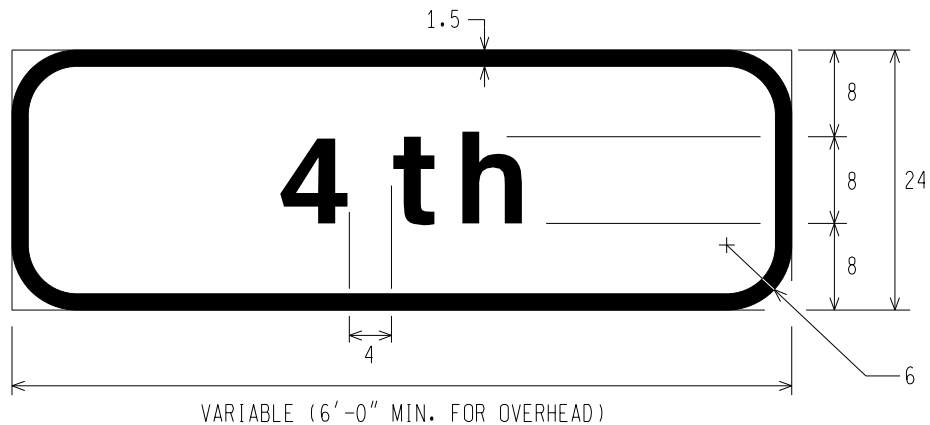
E11-3 DETAIL 1 ROAD NAME SPACING DETAIL
