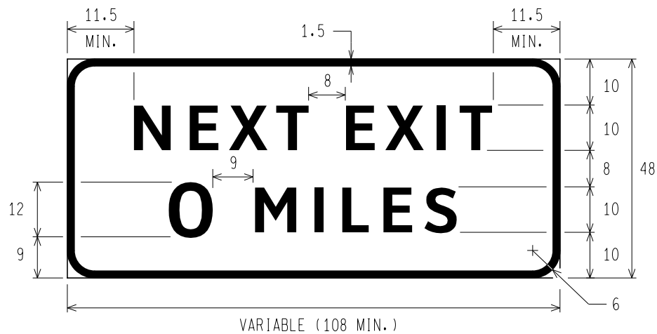
E2-1a NEXT EXIT DISTANCE (2 LINES)
