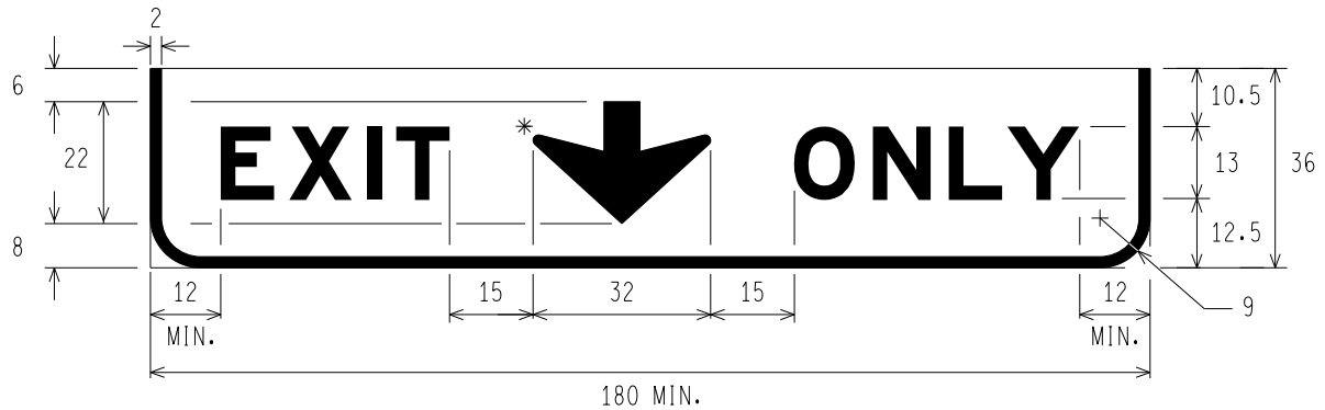
E11-1 EXIT LANE ARROW ONLY
