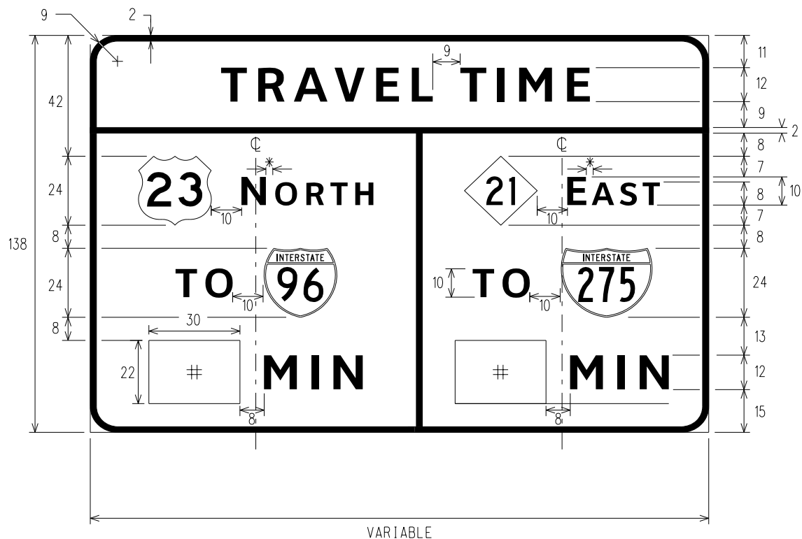
E14-3 TRAVEL TIME ROUTES AS DESTINATIONS TWO ROUTES
