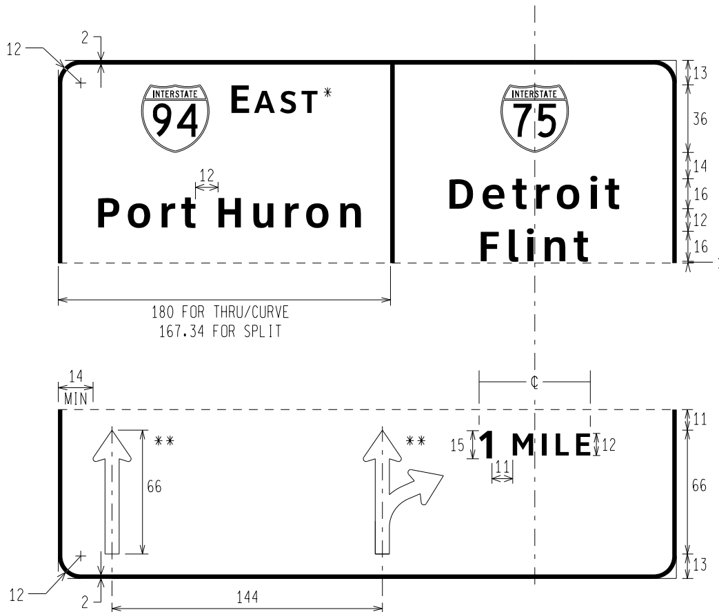
E1-1q PANEL I ROUTE MARKER CARDINAL DIRECTION DOUBLE DESTINATION DISTANCE TWO ARROW ASSIGNMENTS
