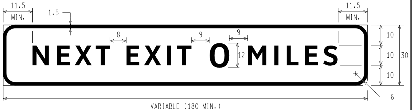
E2-1 NEXT EXIT DISTANCE (1 LINE)
