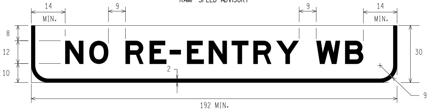
E13-2b NO RE-ENTRY DIRECTION ADVISORY
