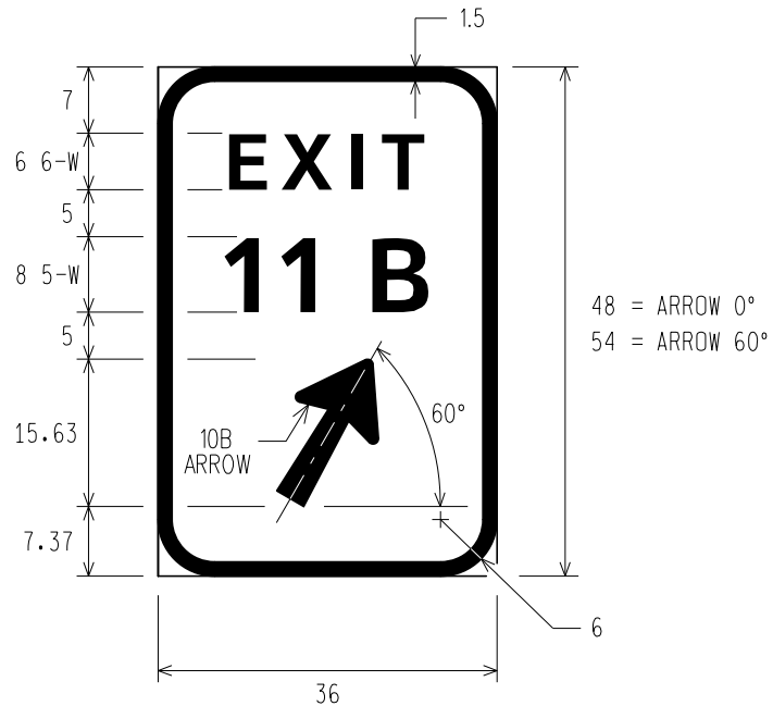
E5-1d MAINTENANCE EXIT GORE SIGN
