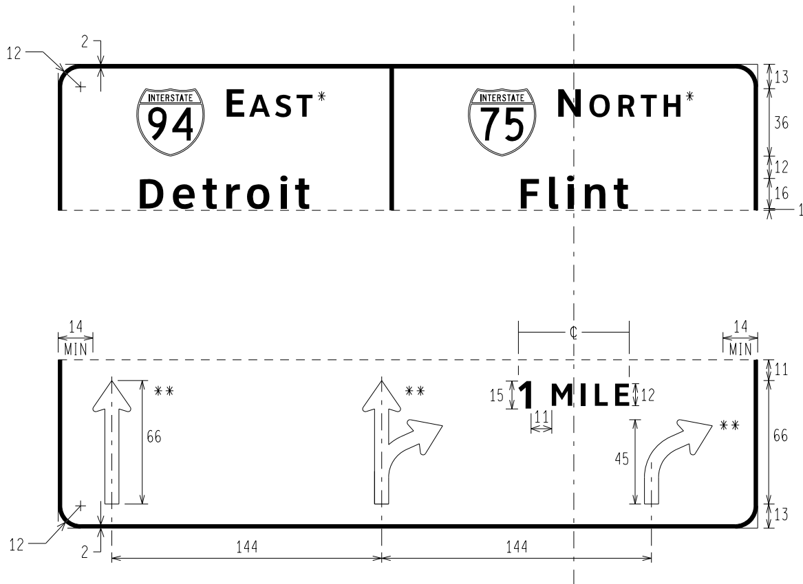
E1-1s PANEL I ROUTE MARKER CARDINAL DIRECTION DESTINATION DISTANCE THREE ARROW ASSIGNMENTS
