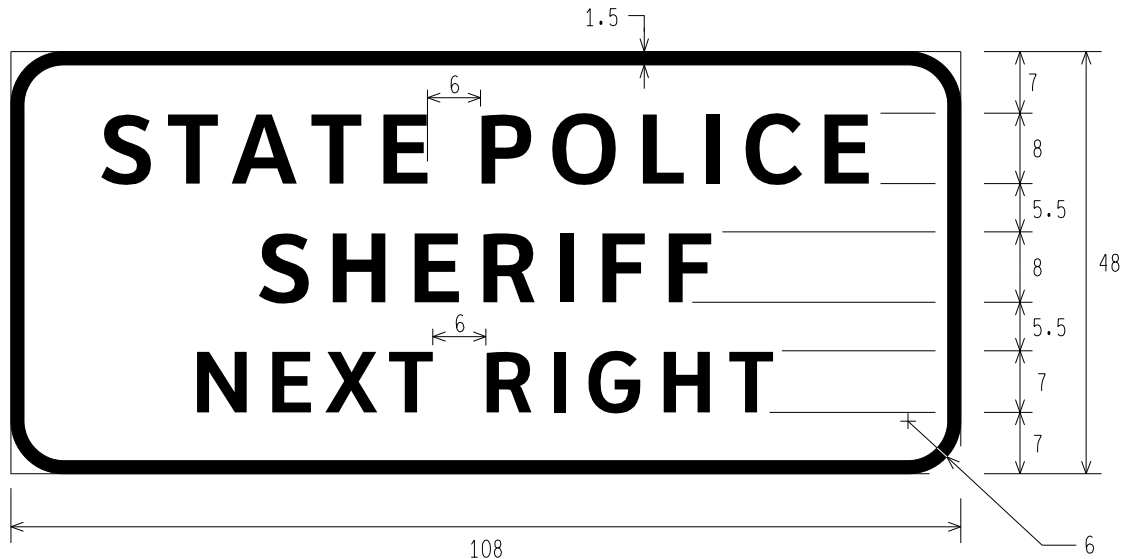
E 11-9a STATE POLICE SHERIFF NEXT RIGHT
