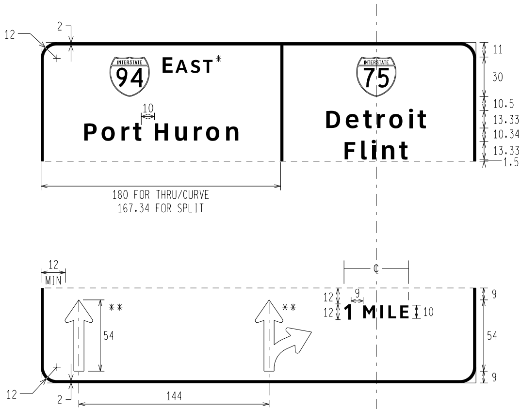
E1-1q PANEL II ROUTE MARKER CARDINAL DIRECTION DOUBLE DESTINATION DISTANCE TWO ARROW ASSIGNMENTS
