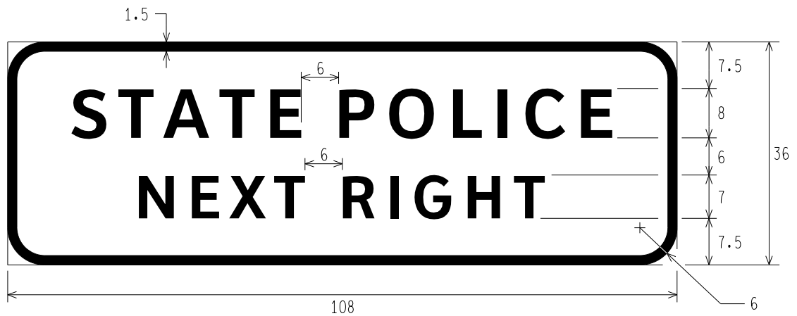
E11-9c STATE POLICE NEXT RIGHT
