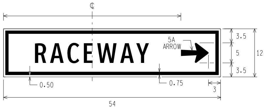
E11-15p [RACEWAY] 2-W
