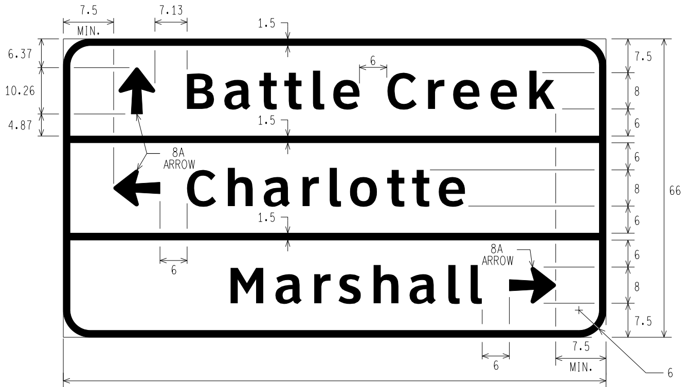
VARIABLE E11-4f TRIPLE DESTINATION AND ARROW
