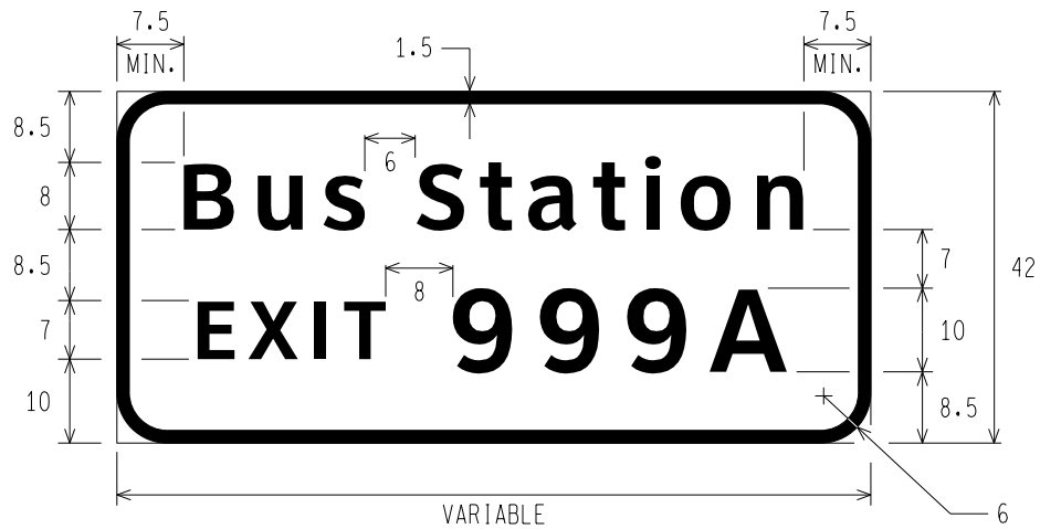
E3-1h VARIABLE (1 LINE) EXIT
