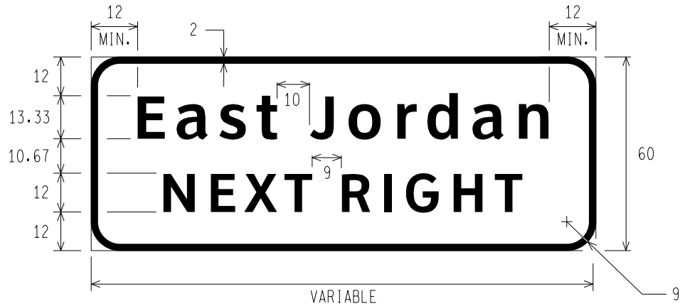
E3-1a DESTINATION (1 LINE) NEXT RIGHT
