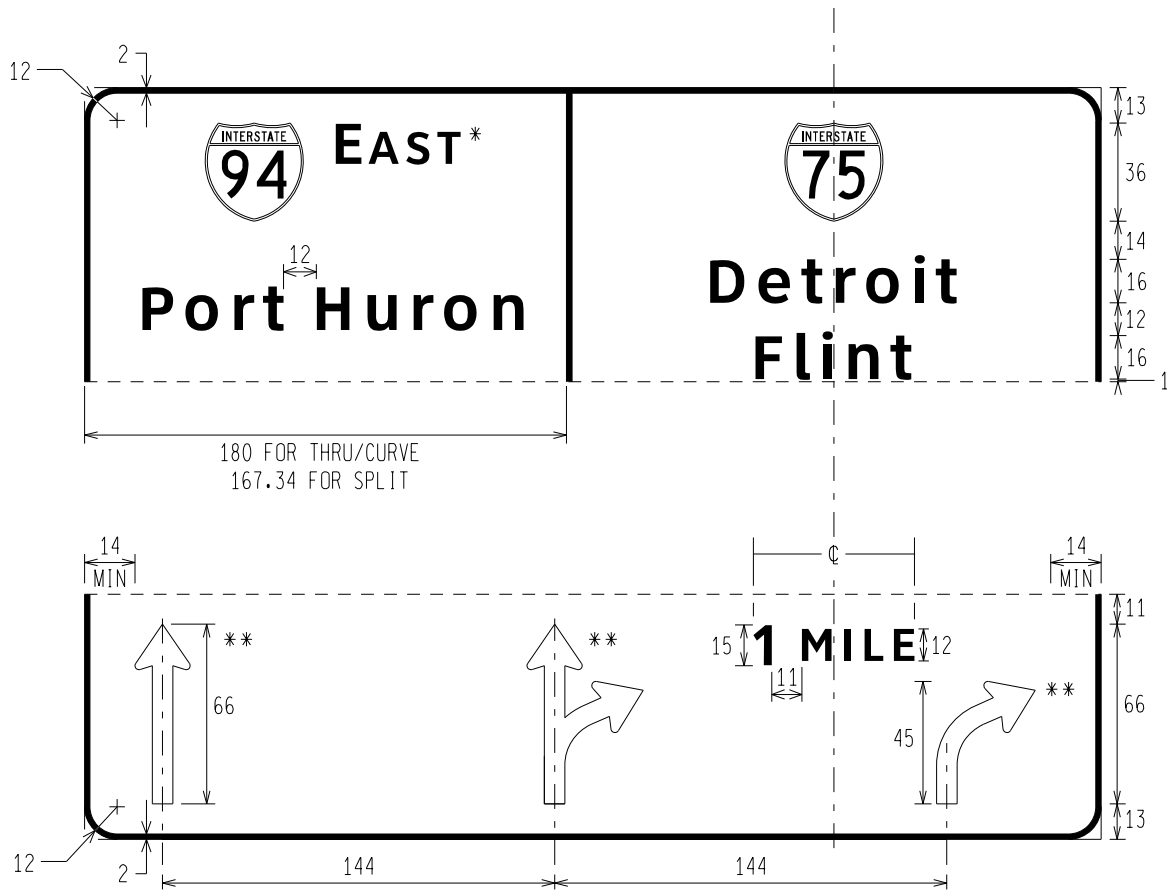
E1-1t PANEL I ROUTE MARKER CARDINAL DIRECTION DOUBLE DESTINATION DISTANCE THREE ARROW ASSIGNMENTS
