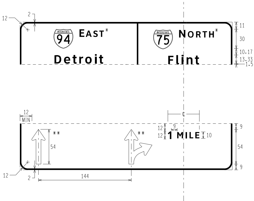
E1-1p PANEL II ROUTE MARKER CARDINAL DIRECTION DESTINATION DISTANCE TWO ARROW ASSIGNMENTS
