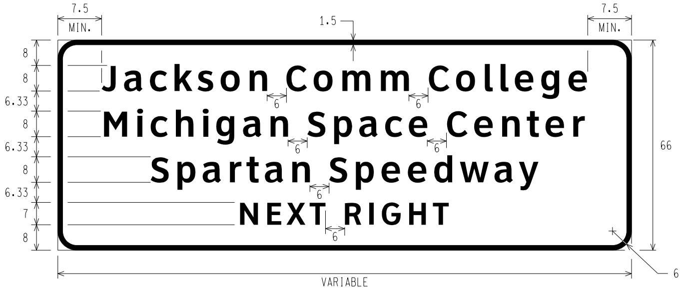
E3-1k VARIABLE (3 LINES) NEXT RIGHT
