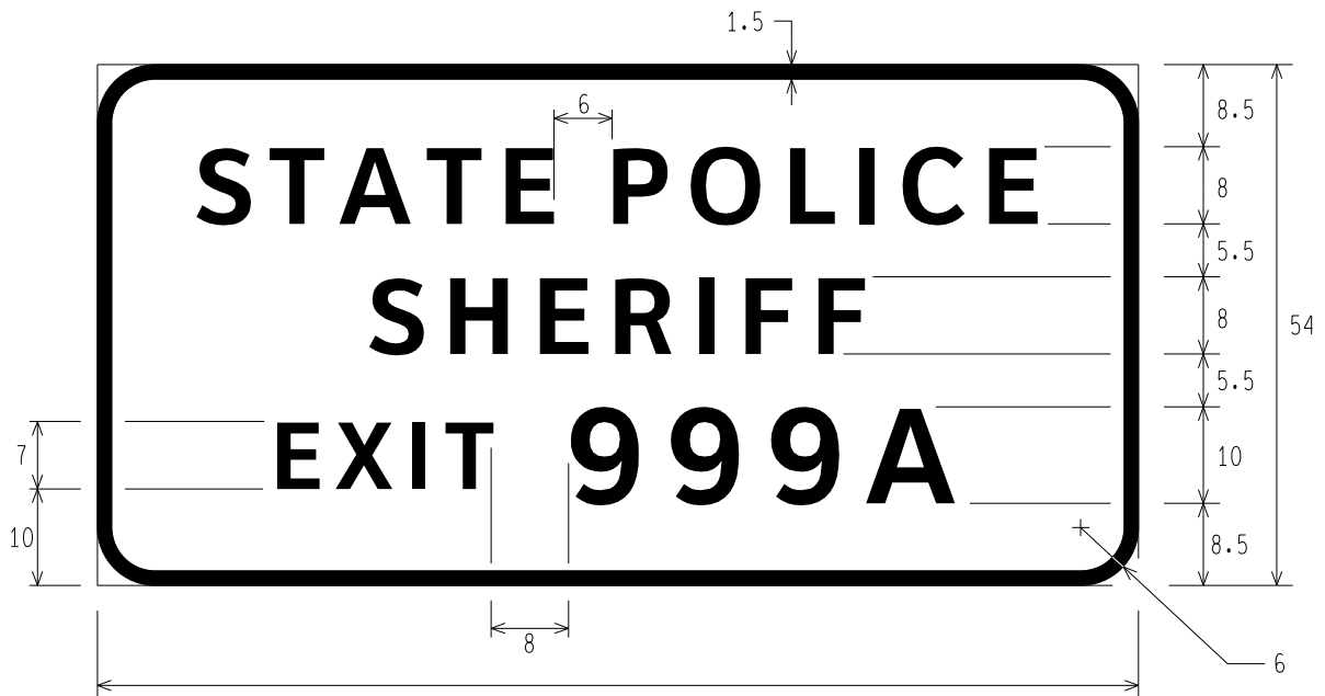
E 11-9b STATE POLICE SHERIFF EXIT
