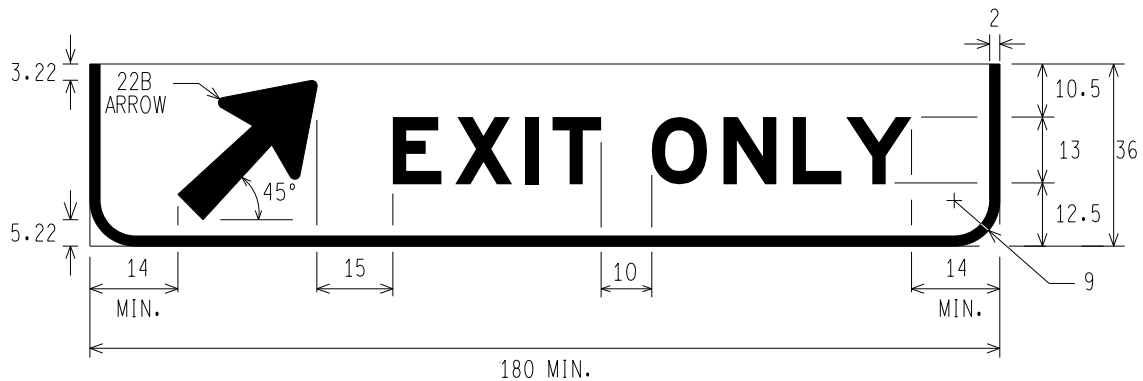
E11-1h ANGLED ARROW EXIT ONLY
