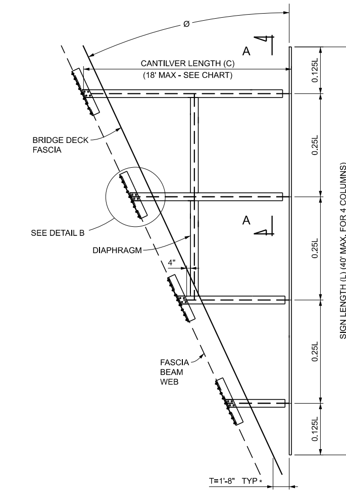
PLAN VIEW TYPE J1: 4 COLUMN SIGN CONNECTION
