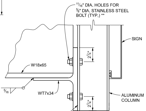
PLAN VIEW TYPE J1: 4 COLUMN SIGN CONNECTION
