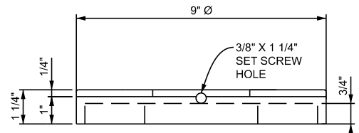
M DETAIL - FRONT VIEW N.T.S. (ROUND ALUMINUM BASE PLATE)
