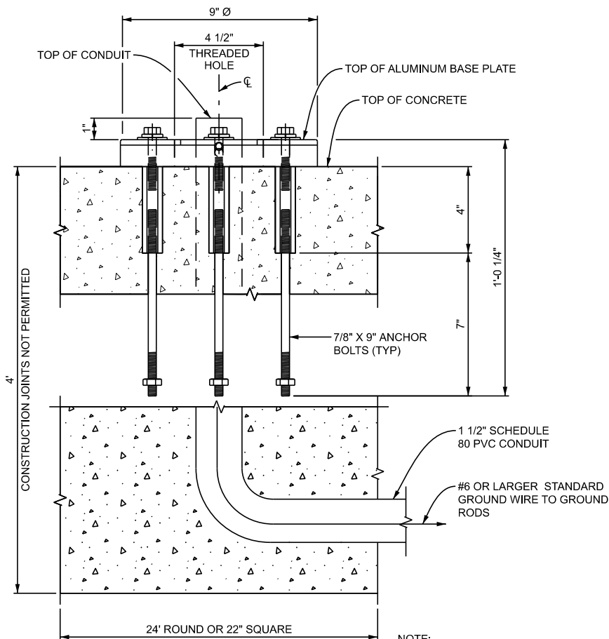
L DETAIL - TOP VIEW N.T.S. (ASSEMBLED)
