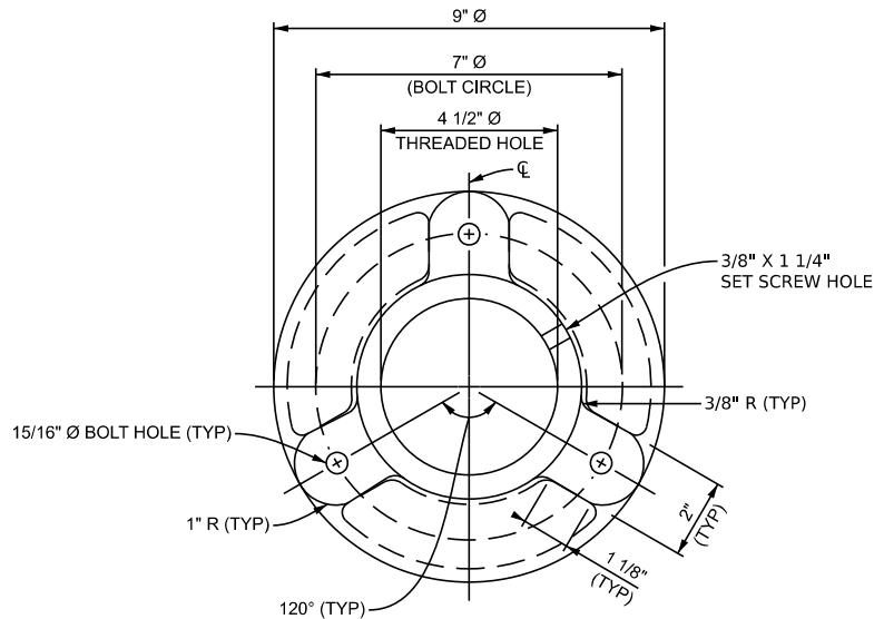
K DETAIL - TOP VIEW N.T.S. (ROUND ALUMINUM BASE PLATE)
