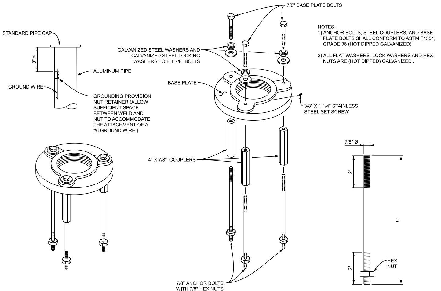
C 7/8" GALVANIZED DETAIL - STEEL ANCHOR BOLTS N.T.S. (3 REQUIRED)
