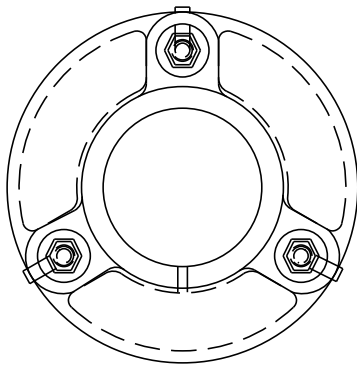
J DETAIL - TOP VIEW N.T.S. (ASSEMBLED)
