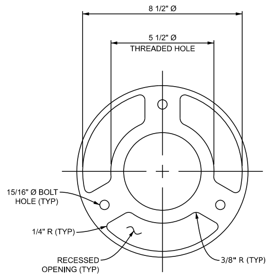
N DETAIL - BOTTOM VIEW N.T.S. (ROUND ALUMINUM BASE PLATE)
