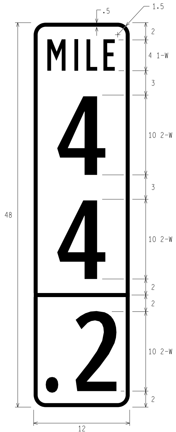
D10-2a INTERMEDIATE REFERENCE LOCATION (2-DIGIT)
