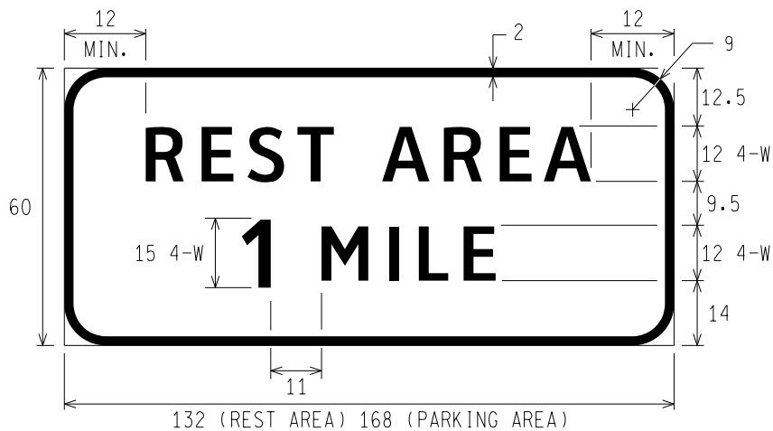
D5-1a REST AREA DISTANCE (FREEWAY) ALTERNATE LEGEND: PARKING AREA
