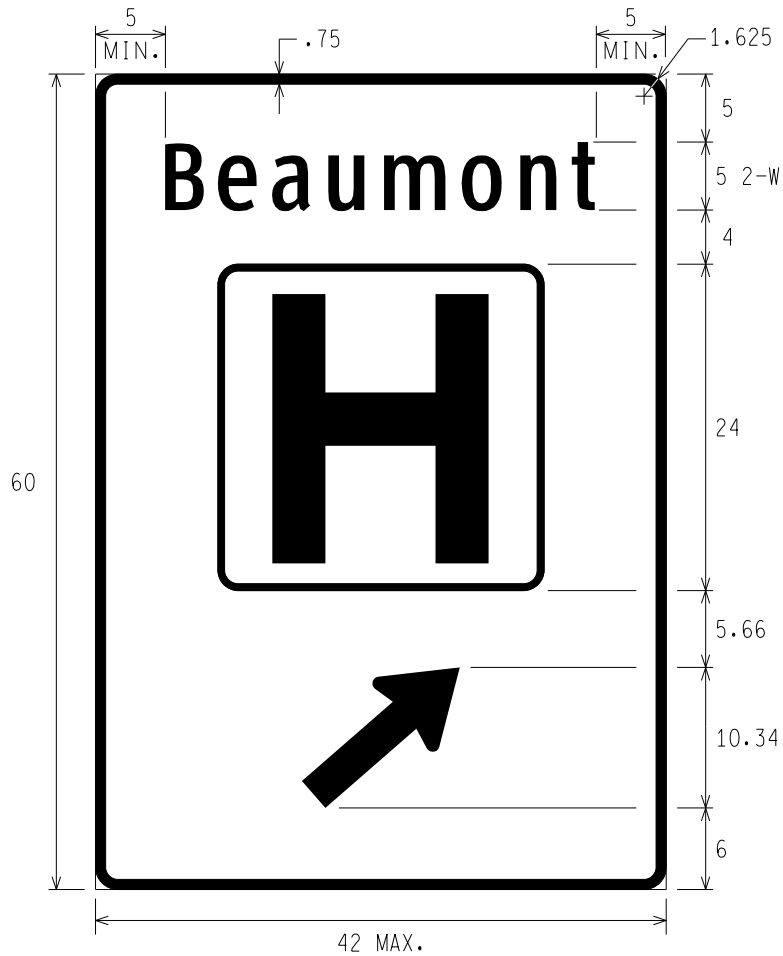
D9-2b HOSPITAL NAME AND SYMBOL WITH ANGLED ARROW
