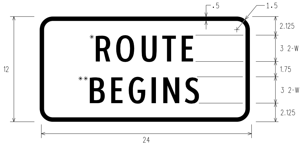
PANEL 2 ROUTE BEGINS PANEL
