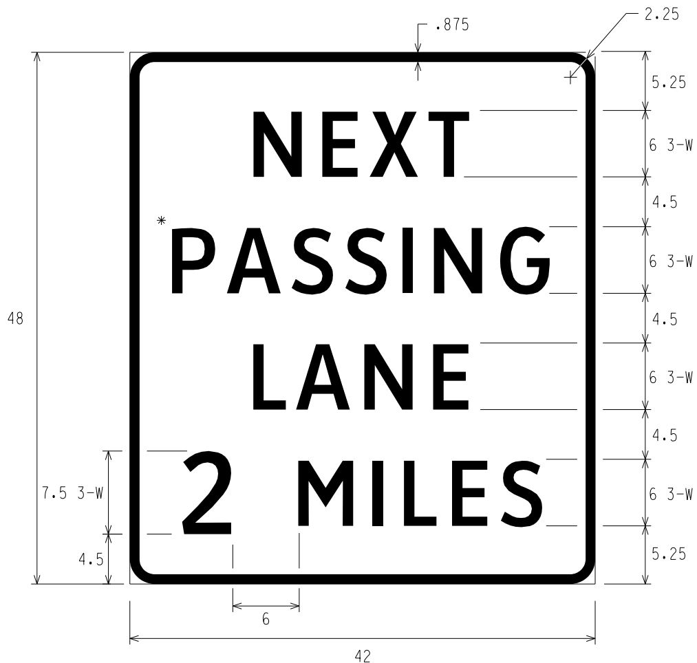
D17-1 NEXT PASSING LANE DISTANCE
