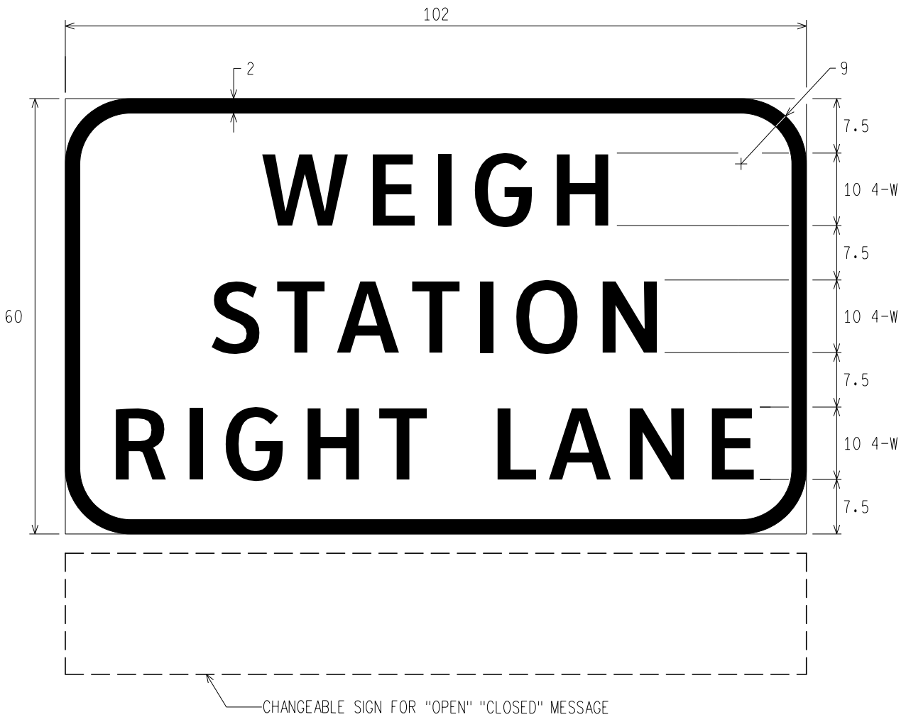
D8-2 WEIGH STATION RIGHT LANE (LEFT LANE)
