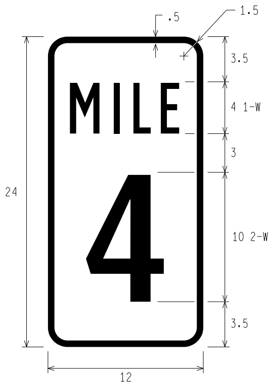
D10-1 REFERENCE LOCATION (1-DIGIT)
