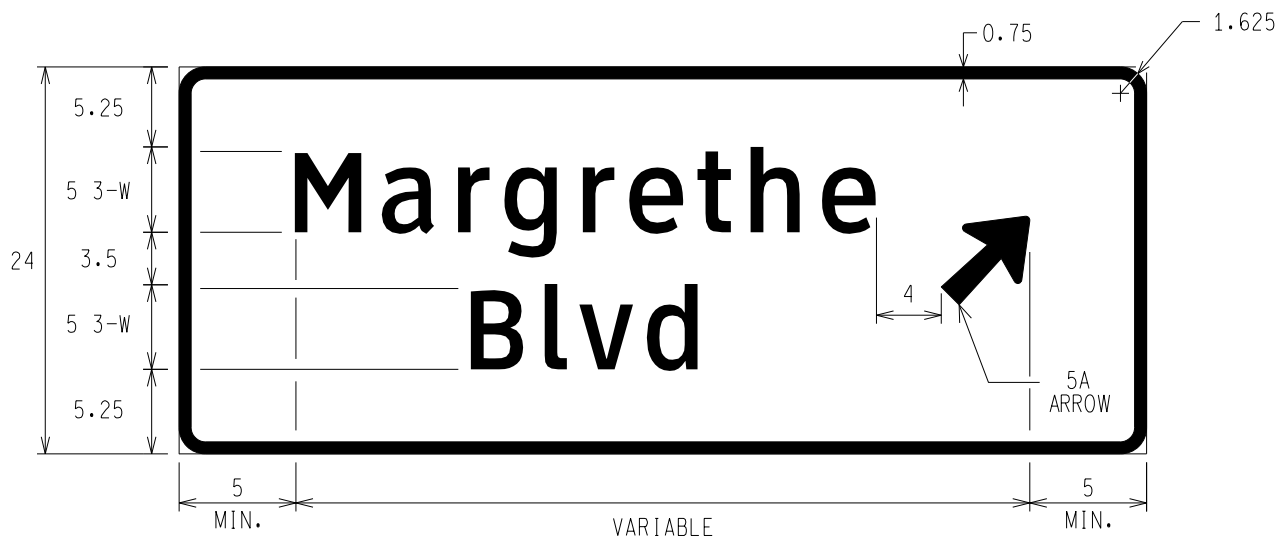
D1-1c ROAD NAME WITH ANGLED ARROW (2 LINES) FOR ROUNDABOUT USE ONLY
