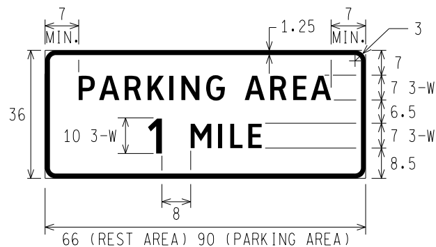
D5-1b PARKING AREA DISTANCE (NON-FREEWAY) ALTERNATE LEGEND: REST AREA
