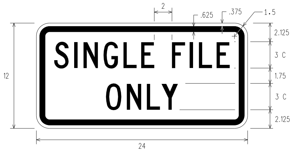
PANEL 5 SINGLE FILE ONLY PANEL
