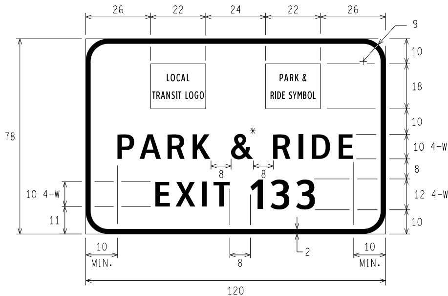
D4-2b PARK AND RIDE (EXIT)
