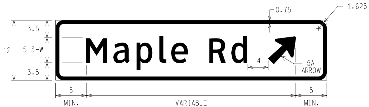
D1-1b ROAD NAME WITH ANGLED ARROW (1 LINE) FOR ROUNDABOUT USE ONLY
