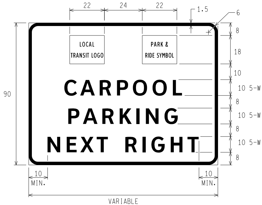
D4-2d LOCAL TRANSIT CARPOOL PARKING (NEXT)
