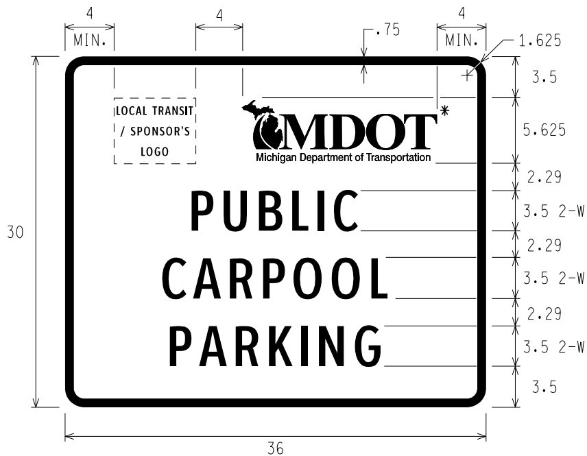
D4-4a LOCAL TRANSIT AND MDOT PUBLIC CARPOOL PARKING
