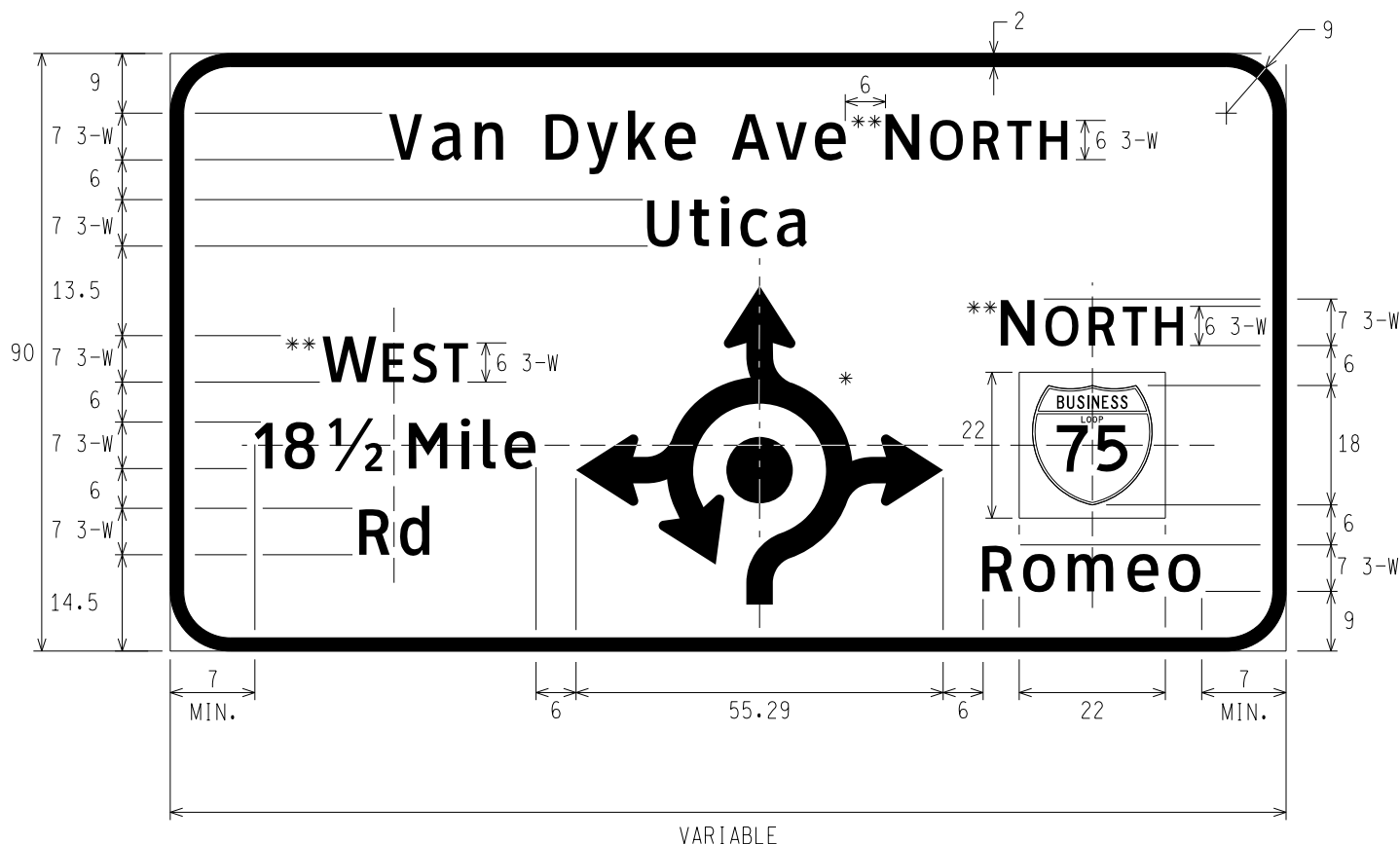
D1-5 ROUNDABOUT EXIT DESTINATIONS FOR ROUNDABOUT USE ONLY
