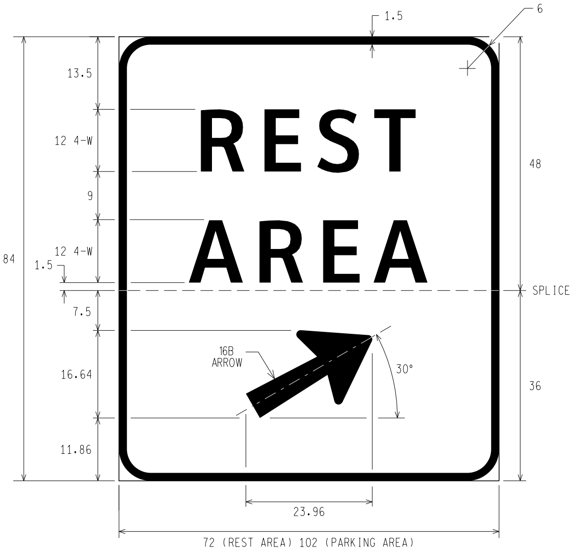
D5-2a REST AREA GORE
