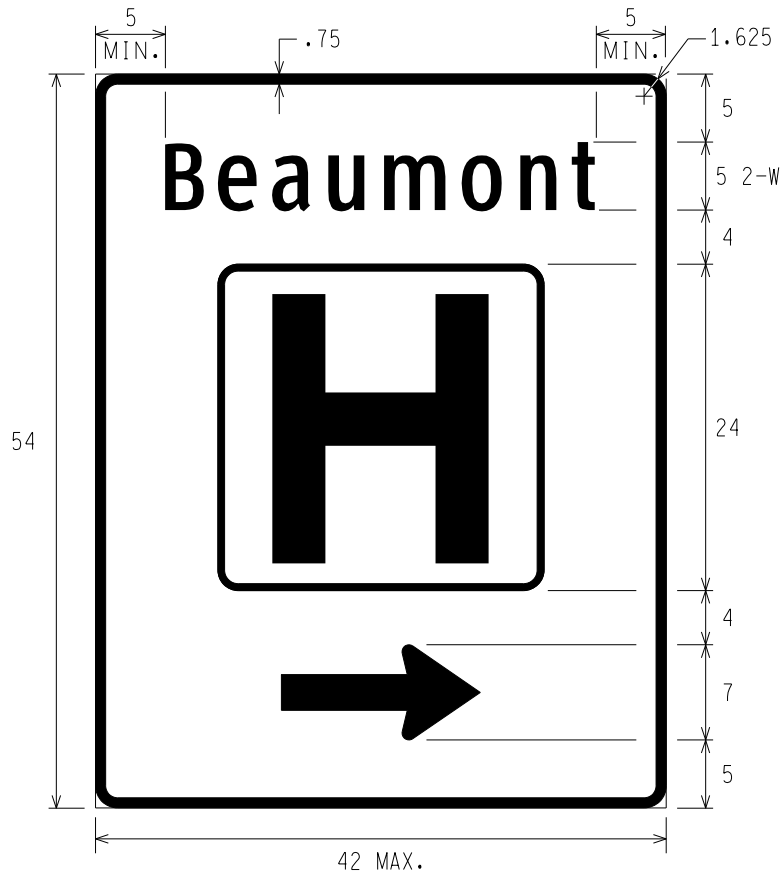
D9-2a HOSPITAL NAME AND SYMOBL WITH RIGHT (LEFT) ARROW
