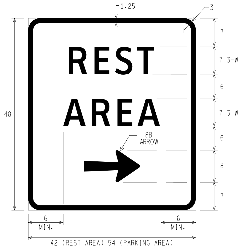
D5-5 REST AREA (WITH HORIZONTAL ARROW)
