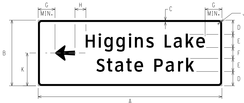
D7-1a RECREATION AREA DIRECTION SIGN (TWO LINES)
