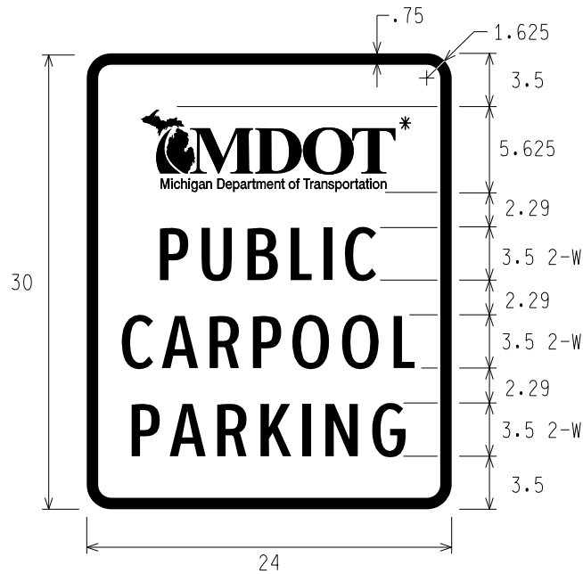
D4-4 MDOT PUBLIC CARPOOL PARKING
