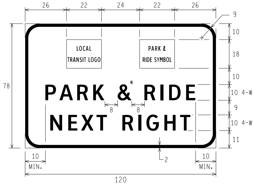
D4-2a PARK AND RIDE (NEXT)
