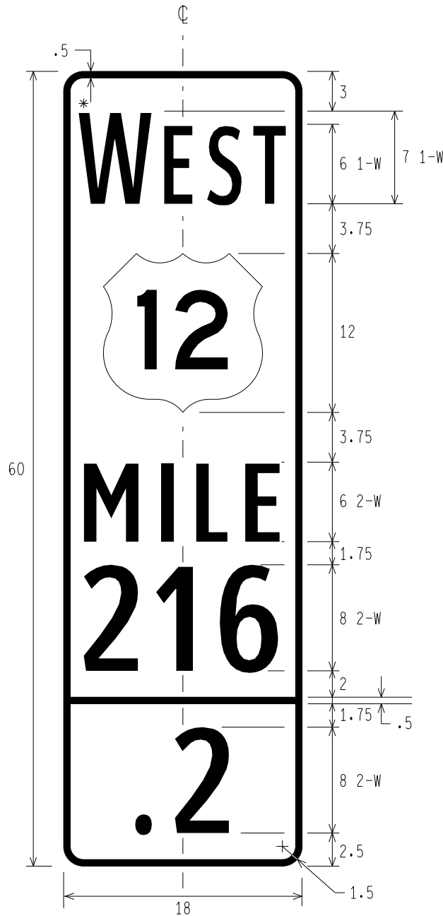
D10-5 INTERMEDIATE ENHANCED REFERENCE LOCATION
