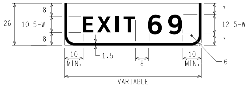
DETAIL 1 SUPPLEMENTAL PANEL 1
