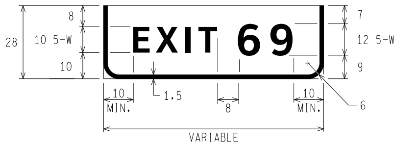
DETAIL 1 SUPPLEMENTAL PANEL 1
