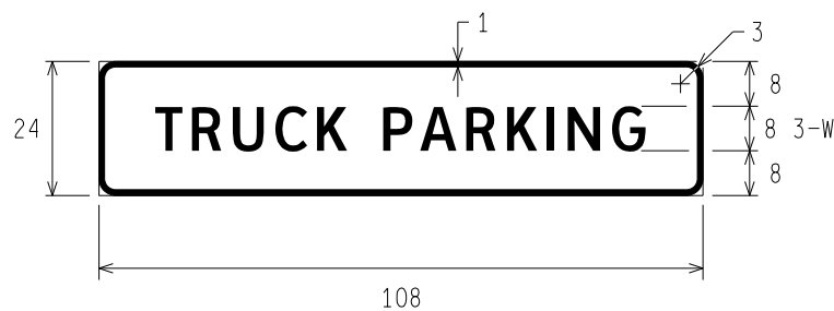
D5-3b TRUCK PARKING
