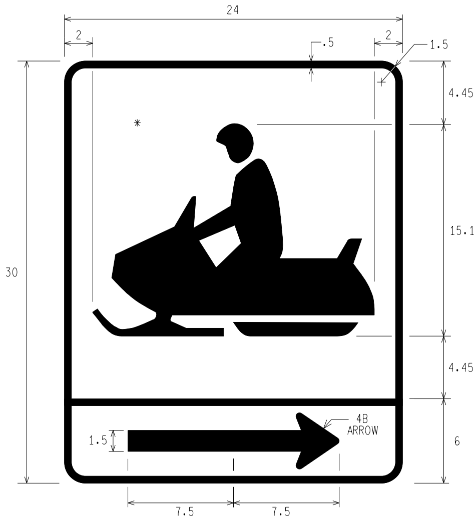
D11-5a COMBINED SNOWMOBILE ROUTE SYMBOL AND PANEL
