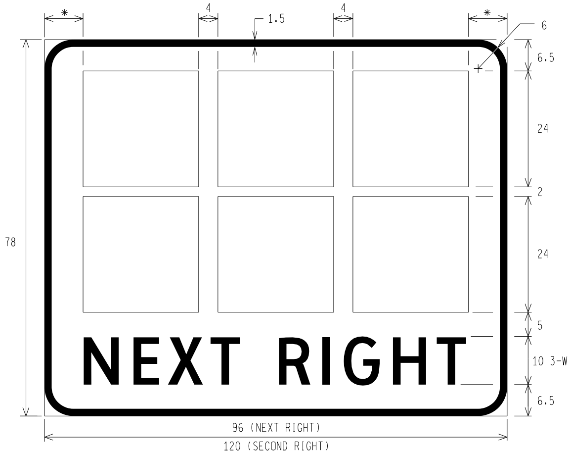
D9-18 MOTORIST SERVICES SIGN 6 SYMBOLS NEXT RIGHT
