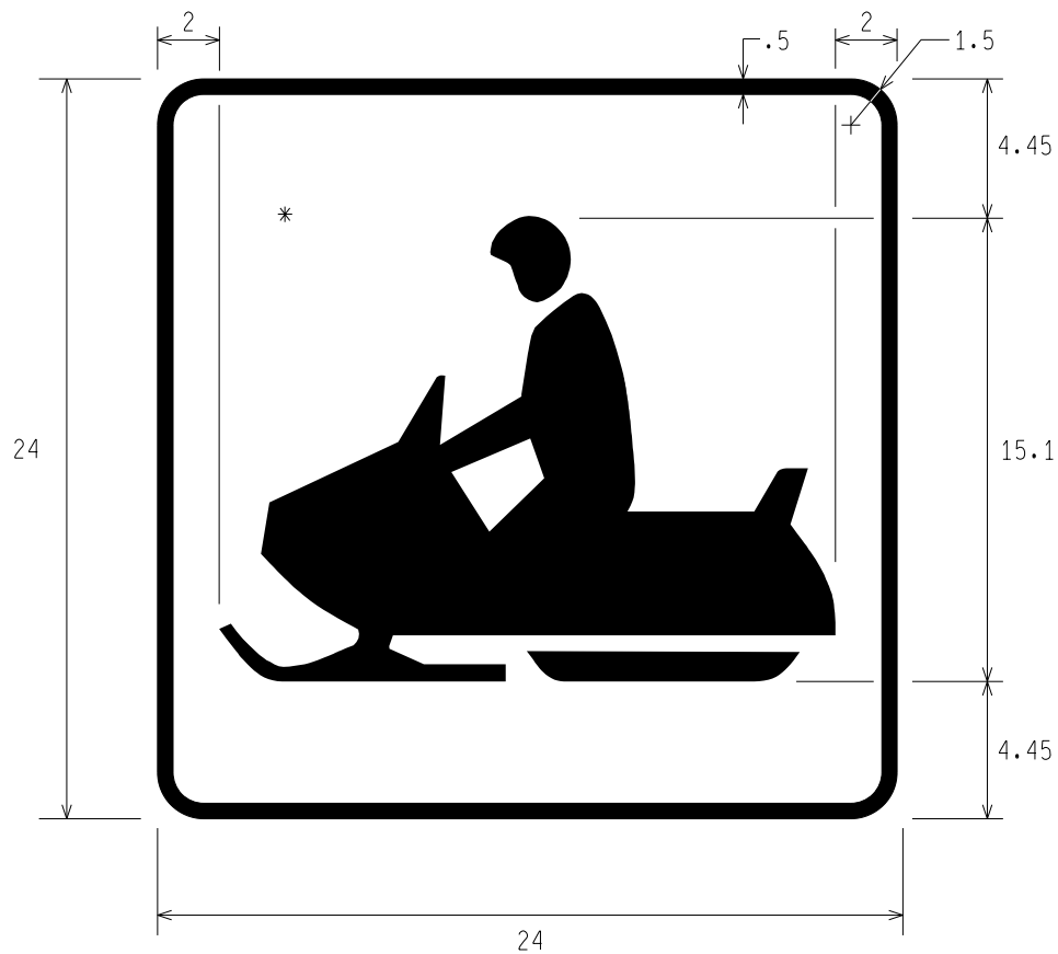
D11-5 SNOWMOBILE ROUTE SYMBOL
