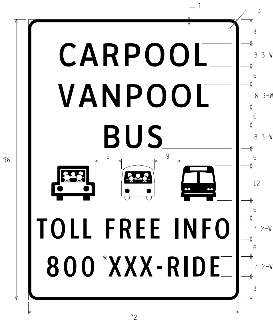
D12-2c CARPOOL VANPOOL BUS INFORMATION
