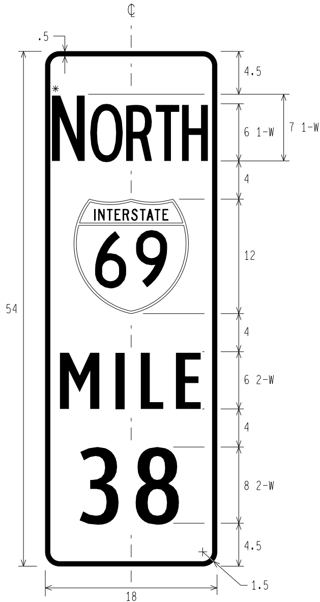
D10-4 ENHANCED REFERENCE LOCATION
