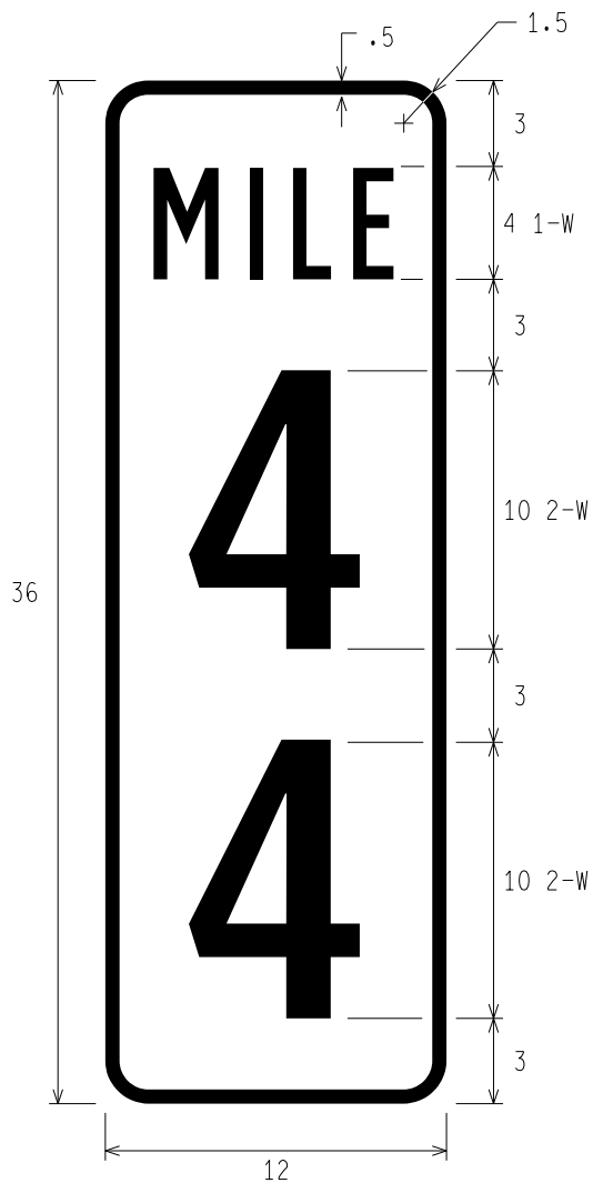
D10-2 REFERENCE LOCATION (2-DIGIT)
