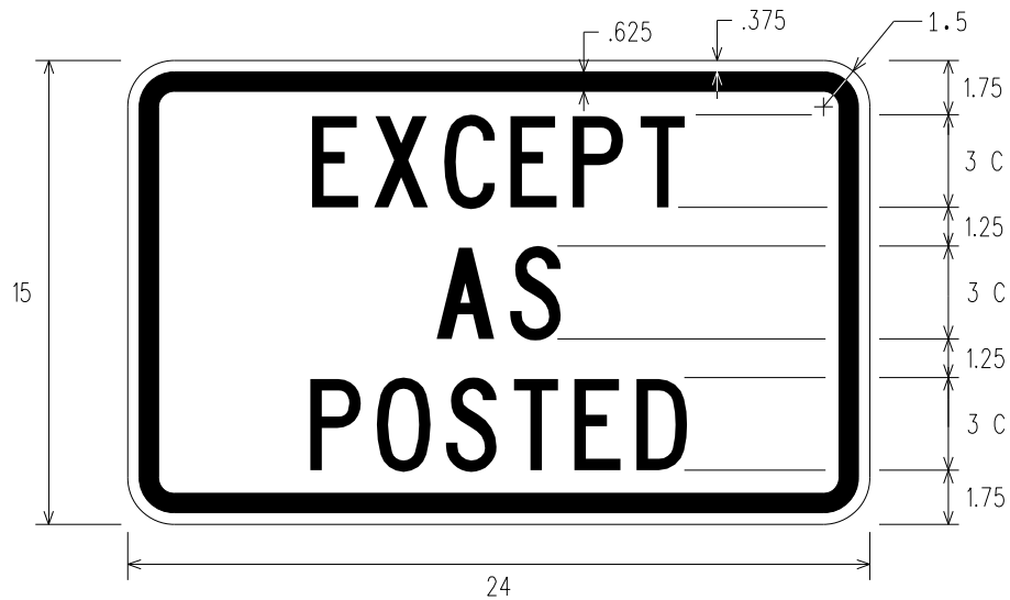
PANEL 8 EXCEPT AS POSTED PANEL
