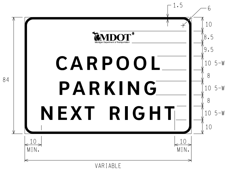
D4-2c MDOT CARPOOL PARKING (NEXT)
