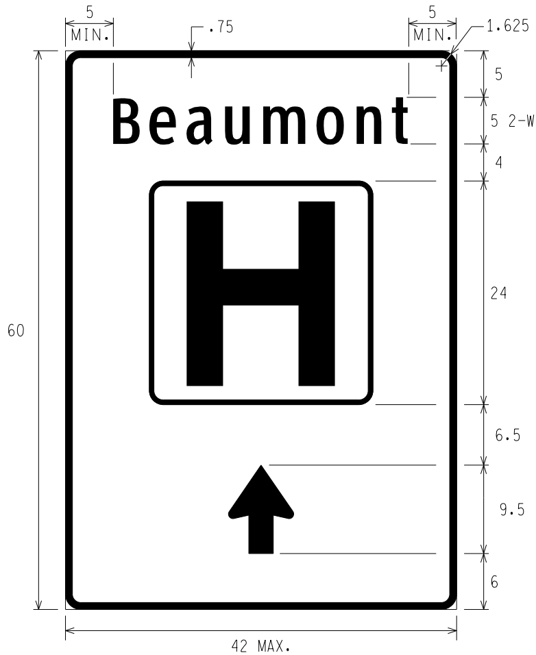
D9-2c HOSPITAL NAME AND SYMBOL WITH UP ARROW
