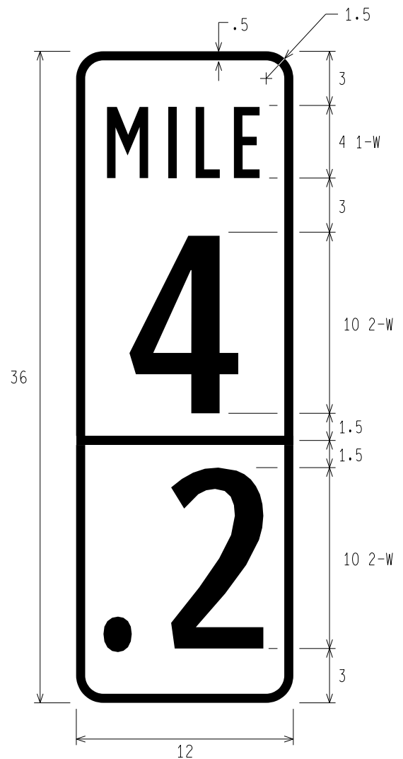
D10-1a INTERMEDIATE REFERENCE LOCATION (1-DIGIT)
