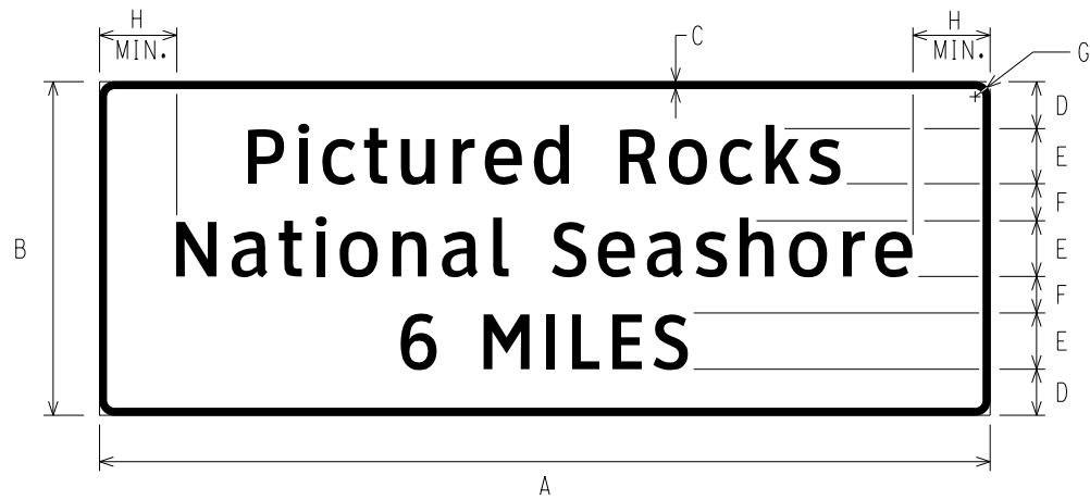
D7-1 RECREATION AREA DISTANCE SIGN
