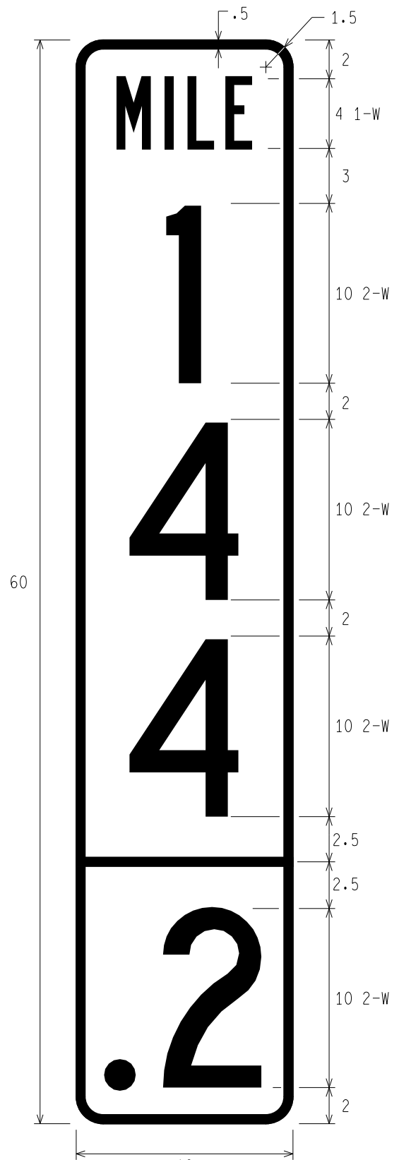
D10-3a INTERMEDIATE REFERENCE LOCATION (3-DIGIT)
