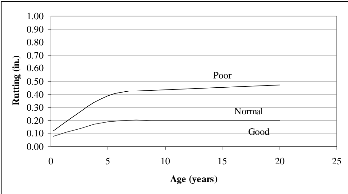
Figure 8.9. Performance criteria for Rutting
