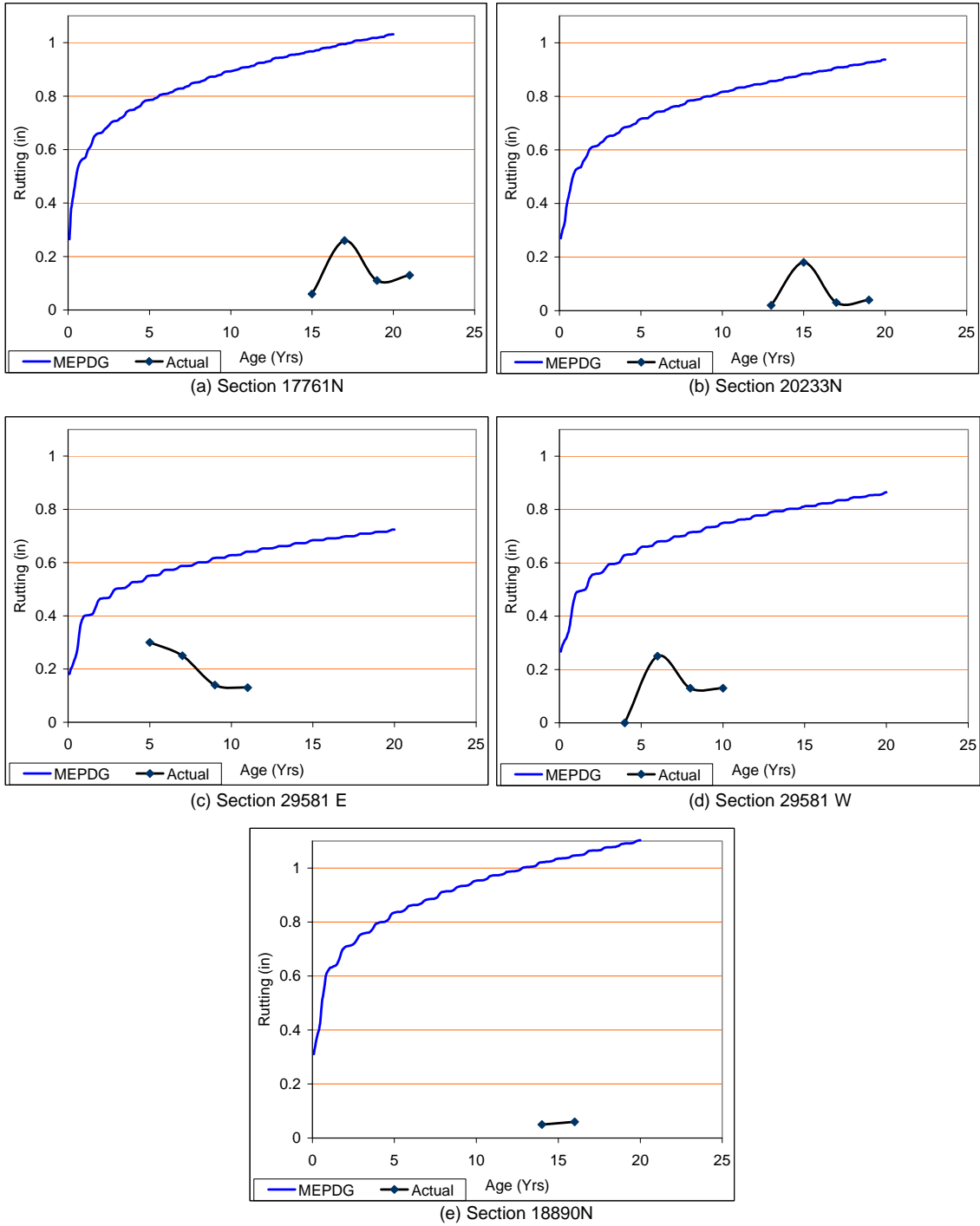
Figure 10.23. Observed rutting versus that predicted by M-E PDG for SPS-1 sections
