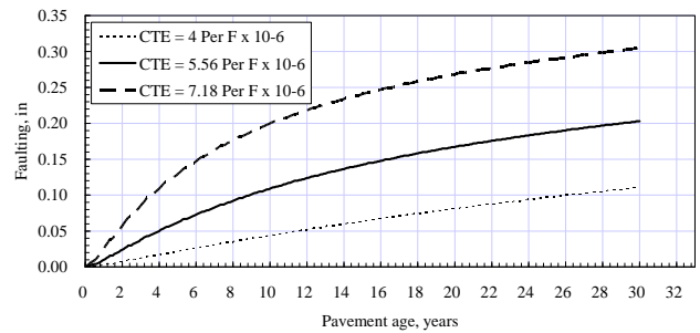
(a) Faulting
