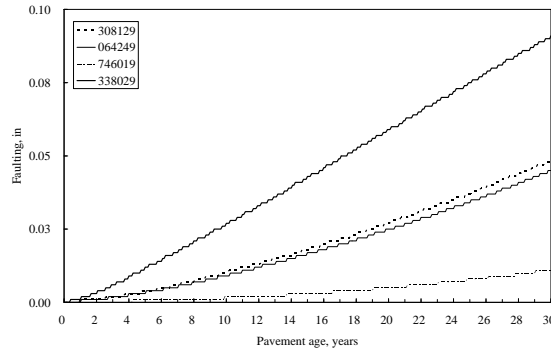
(a) faulting
