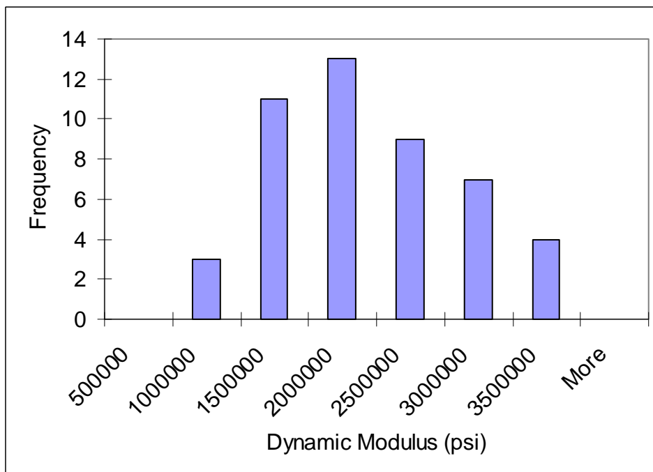
Figure B-10: Distribution of asphalt mix dynamic modulus at 0 F
