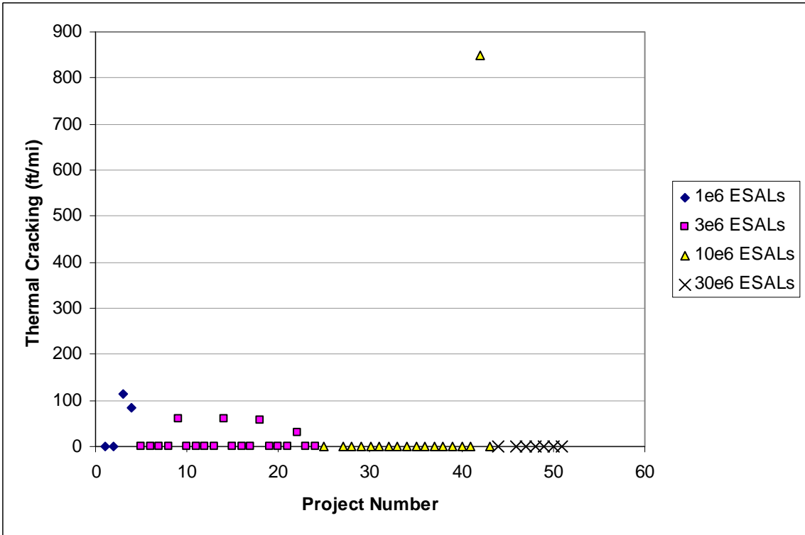
Figure 10.5. Predicted thermal cracking at the end of 20 years (in-situ air voids = 9%)
