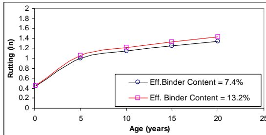
(c) Effect of AC binder content on rutting
