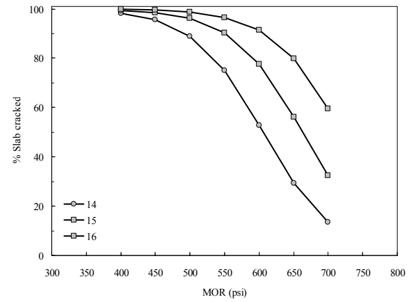
(f) Effect of MOR and joint spacing
