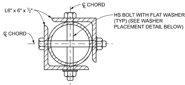
SECTION G-G
