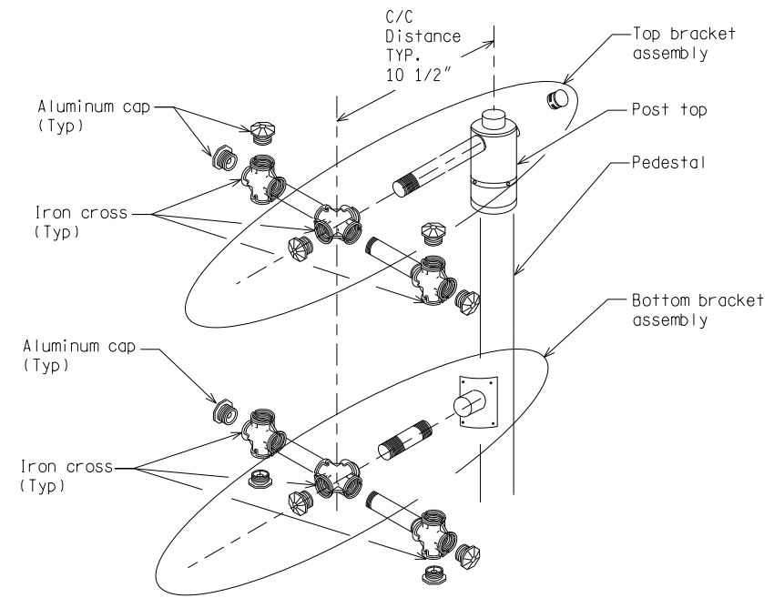
SIGNAL MOUNTING HARDWARE FOR BACKSIDE BRACKET
