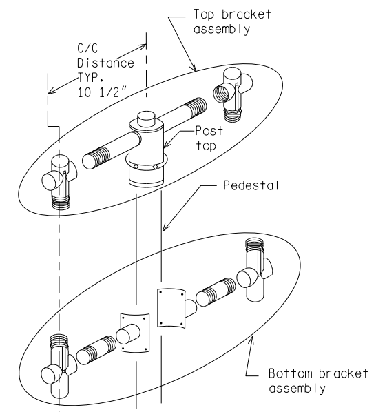
SIGNAL MOUNTING HARDWARE - STANDARD BRACKET
