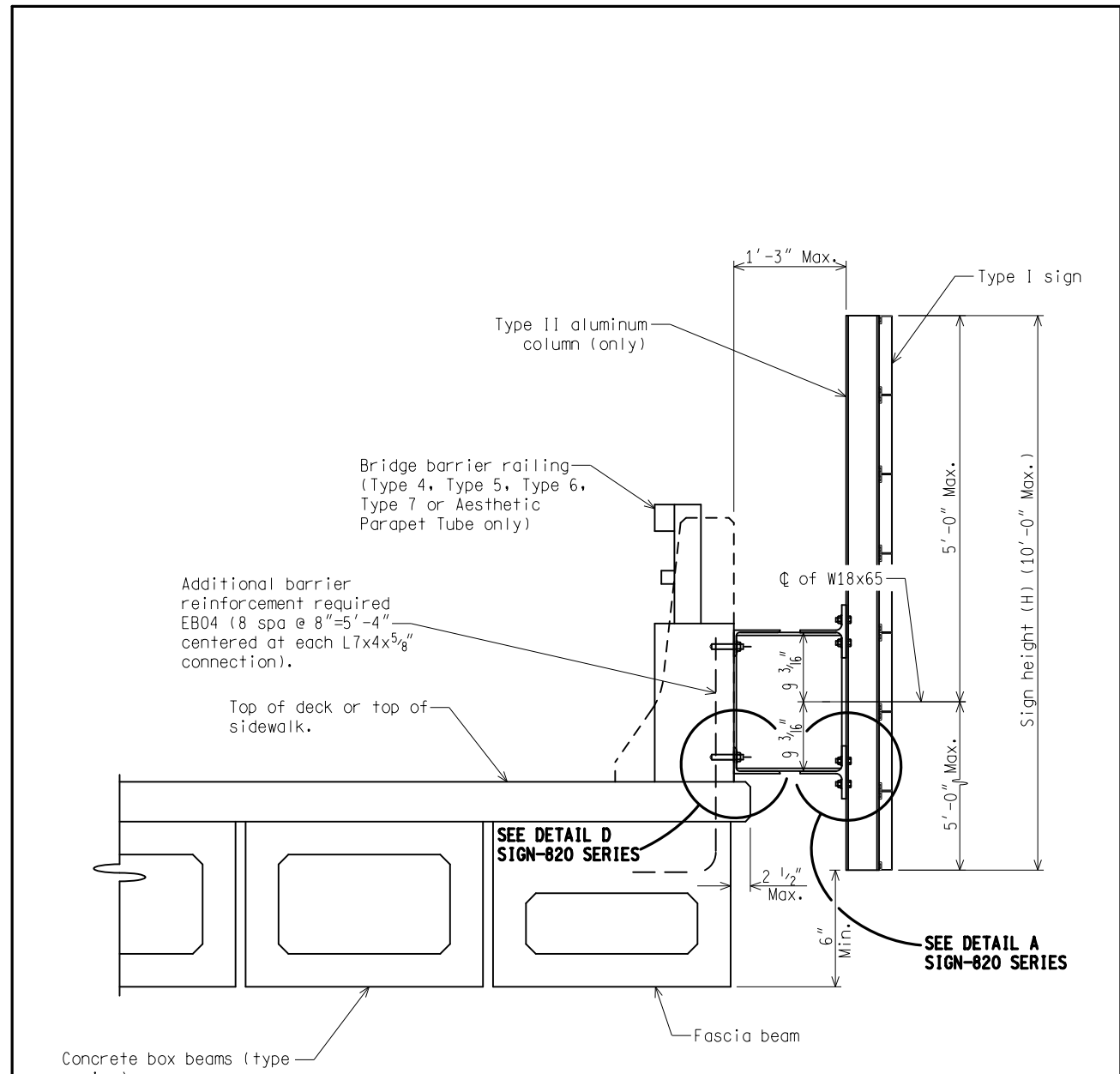
SECTION THRU BRIDGE (SEE DETAIL ON NEXT SHEET)
