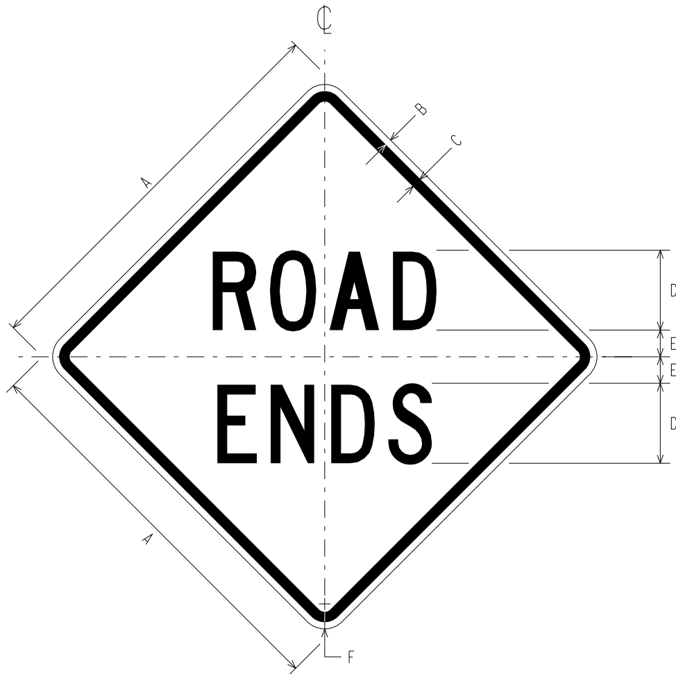
W14-2b ROAD ENDS
