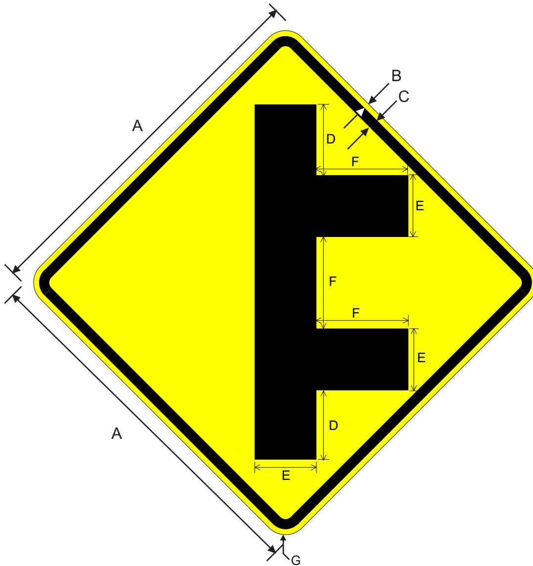
W2-8R(L) DOUBLE SIDE ROAD
