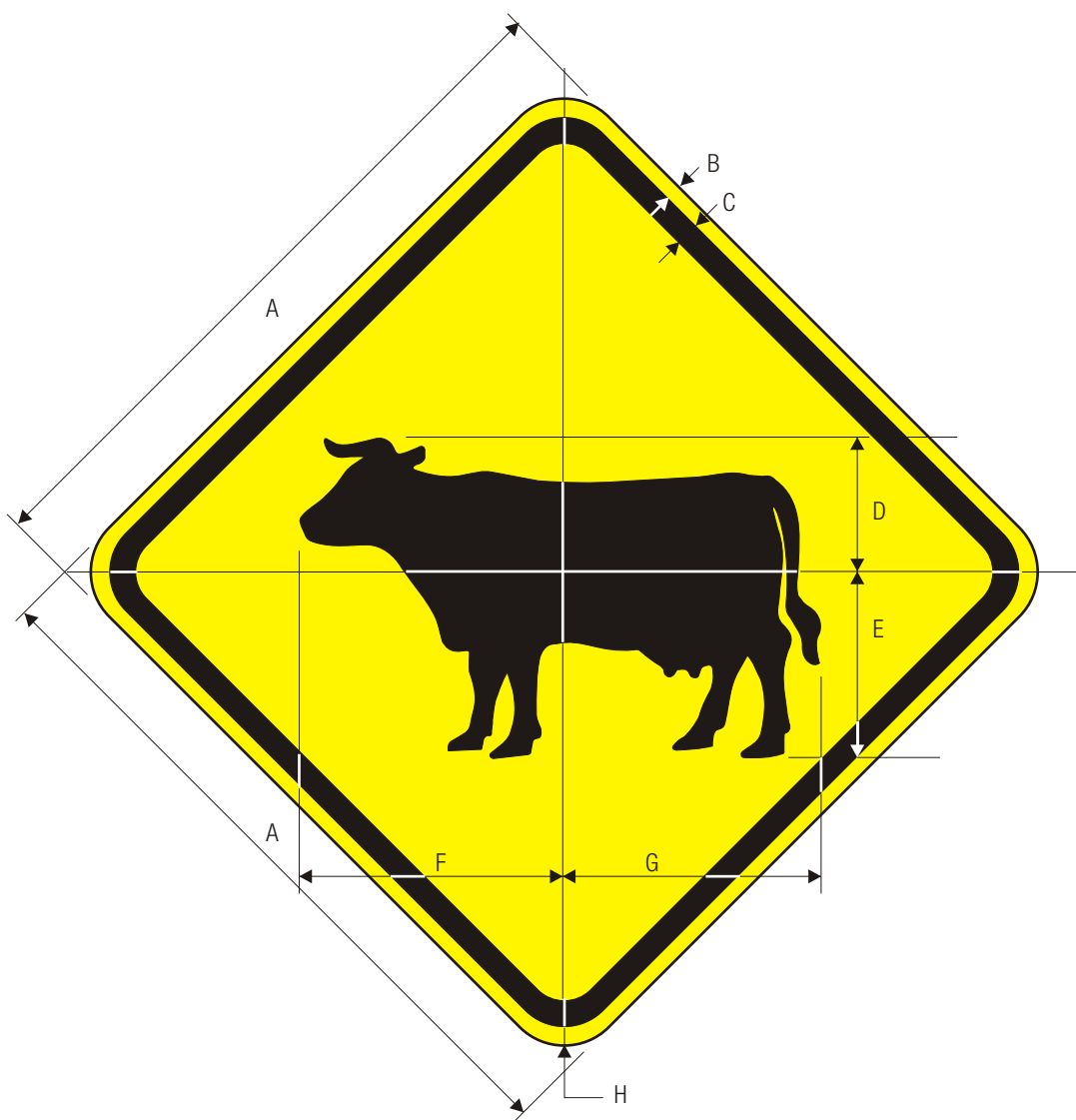
W11-4 CATTLE TRAFFIC
