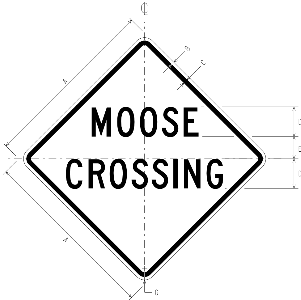
W11-21a MOOSE CROSSING TEXT
