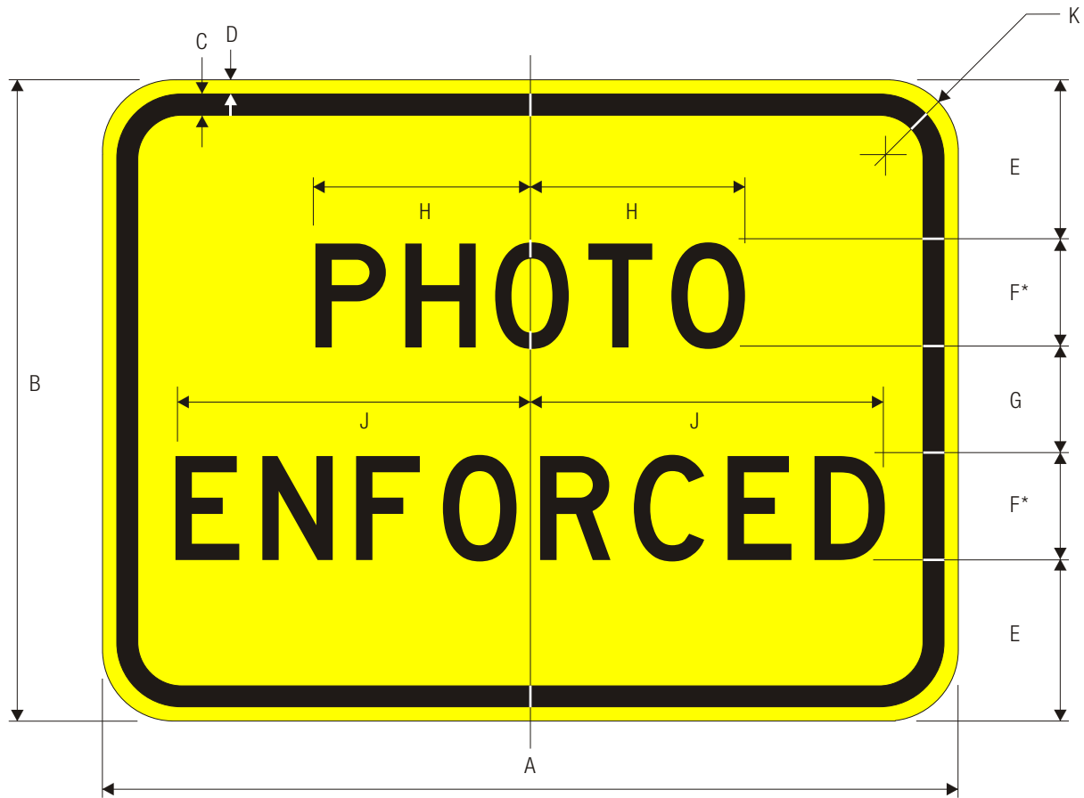
W16-10aP PHOTO ENFORCED
