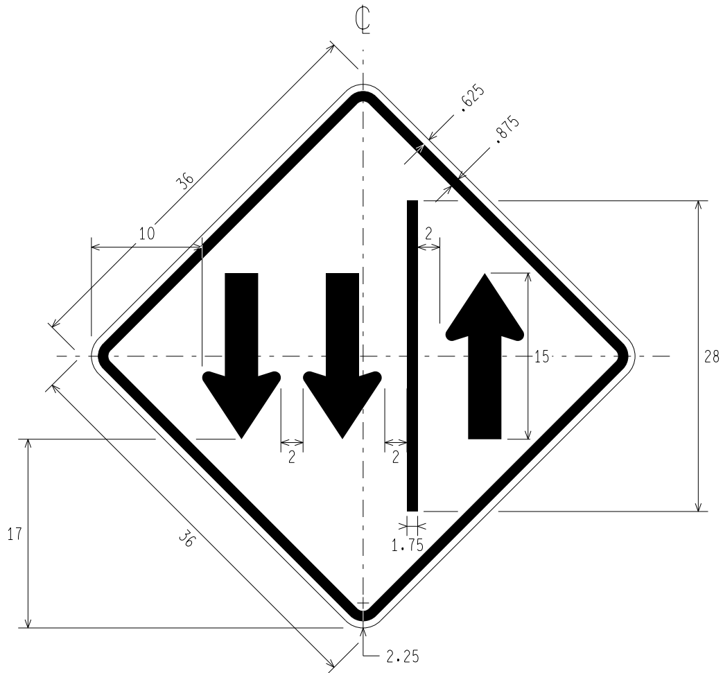
W6-5 TRIPLE ARROW
