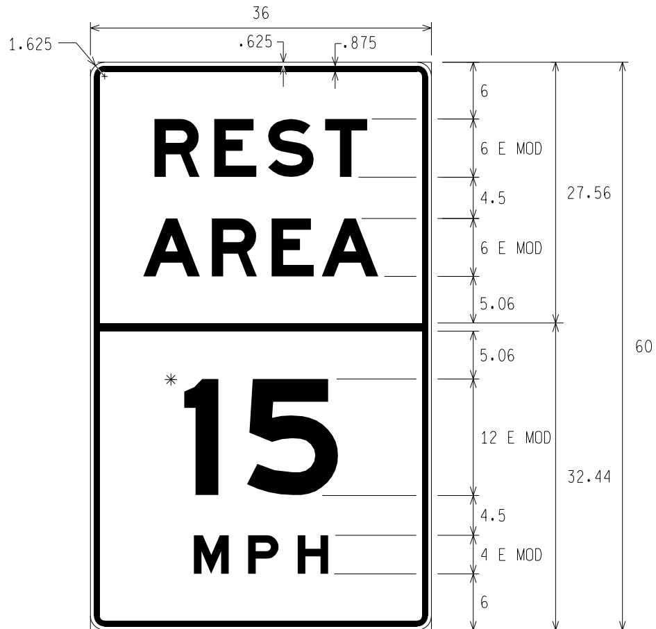
W13-3c REST AREA ADVISORY SPEED
