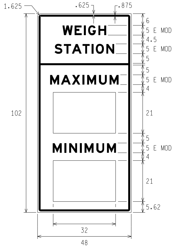
W13-3d WEIGH STATION MAXIMUM AND MINIMUM SPEED
