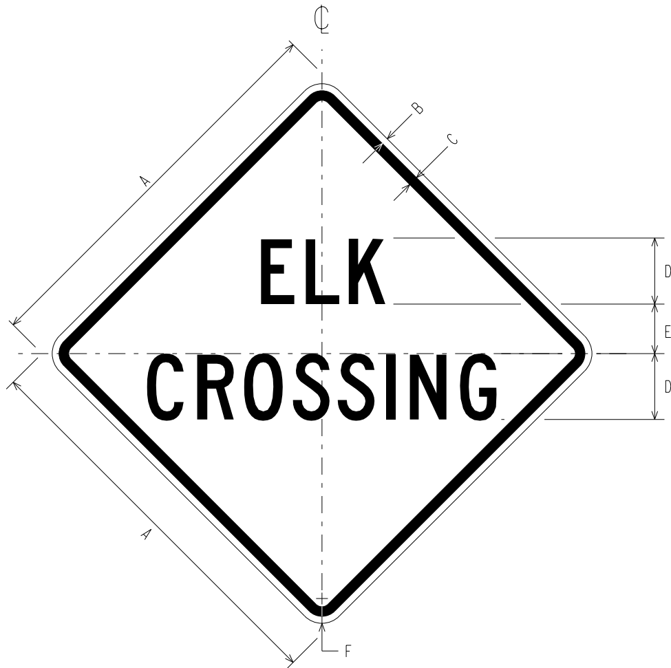
W11-20a ELK CROSSING TEXT
