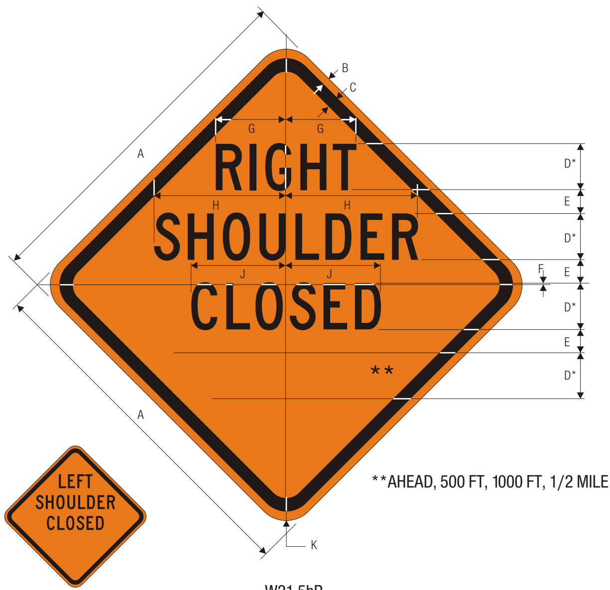
W21-5bL RIGHT (LEFT) SHOULDER CLOSED
