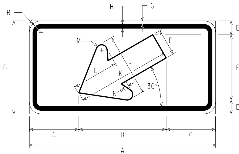
W16-7P(L) ANGLED-DOWN ARROW
