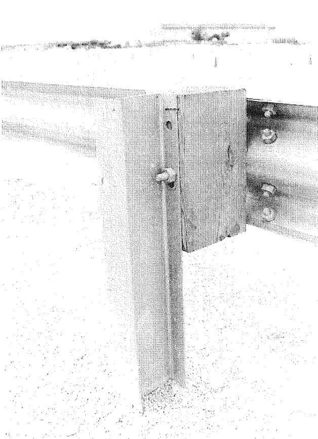
Figure 4. Post-to-Rail Attachment for the Type B (W-beam) Longitudinal Barrier System
