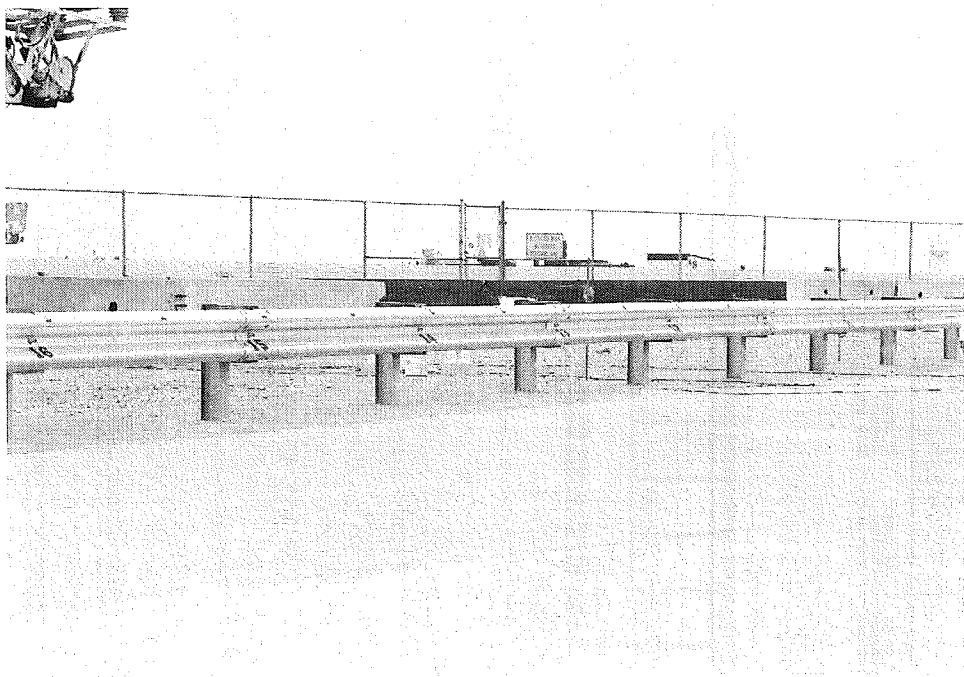
Figure 2. Modified Type B (W-beam) Longitudinal Barrier System
