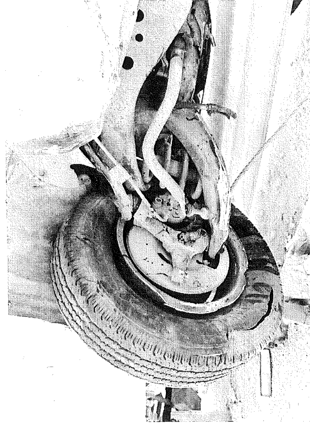
Figure 27. Front-End Vehicle and Rear-Tire Damage, Test MIW-2
