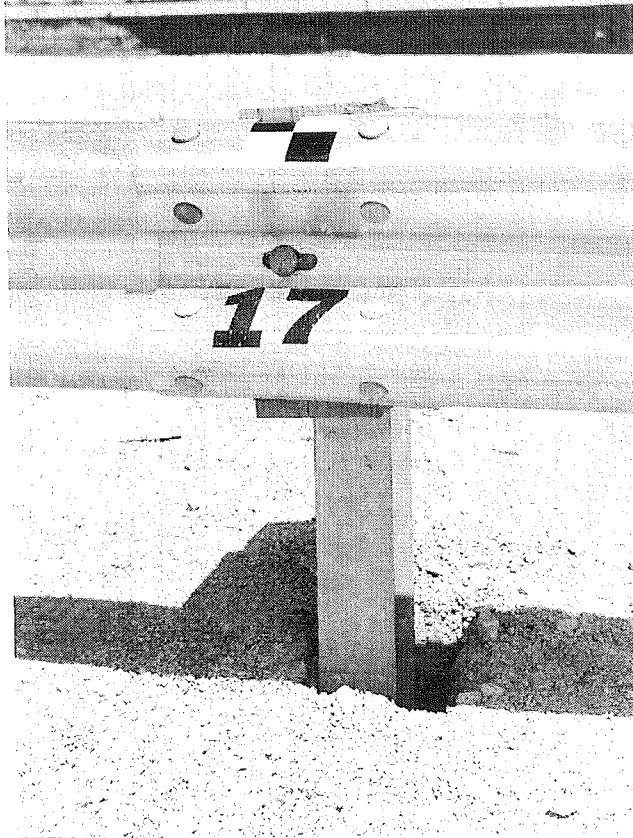
Figure 21. Type B Longitudinal Barrier Rail and Post Damage, Test MIW-2
