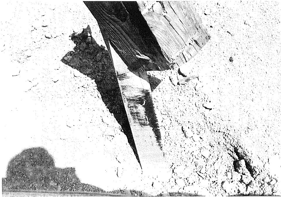
Figure 20. Type B Longitudinal Barrier Rail and Post Damage, Test MIW-2
