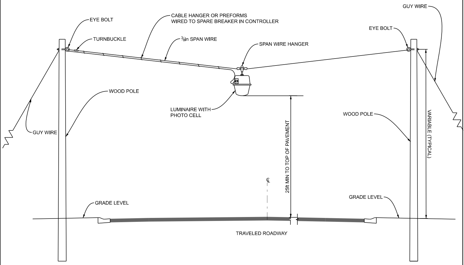
OVERHEAD LIGHTING DETAIL
