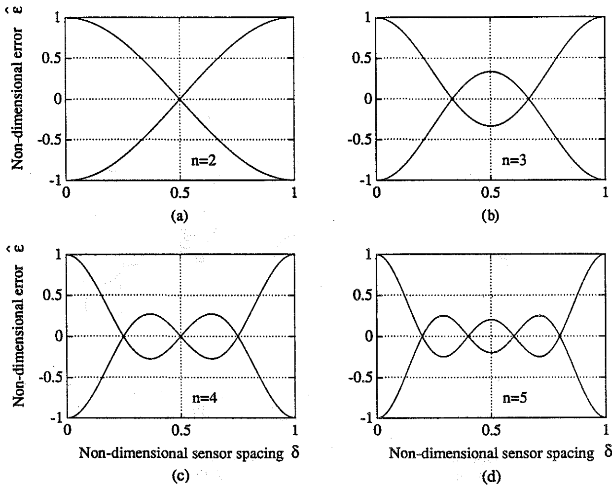
Fig 4.3. Plots of the envelope error \hat{\epsilon} from equation 4.7 (a) n=2 , (b) n=3 , (c) n=4 , (d) n=5 .
