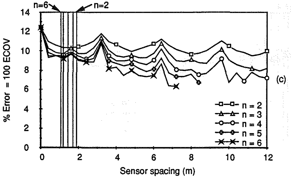
Fig. 5.20 WIM array error vs sensor spacing Vehicle S2, Speed = 9.5 m/s (34 km/h) (a) Axle 1 (b) Axle 3 (c) Axle 5
