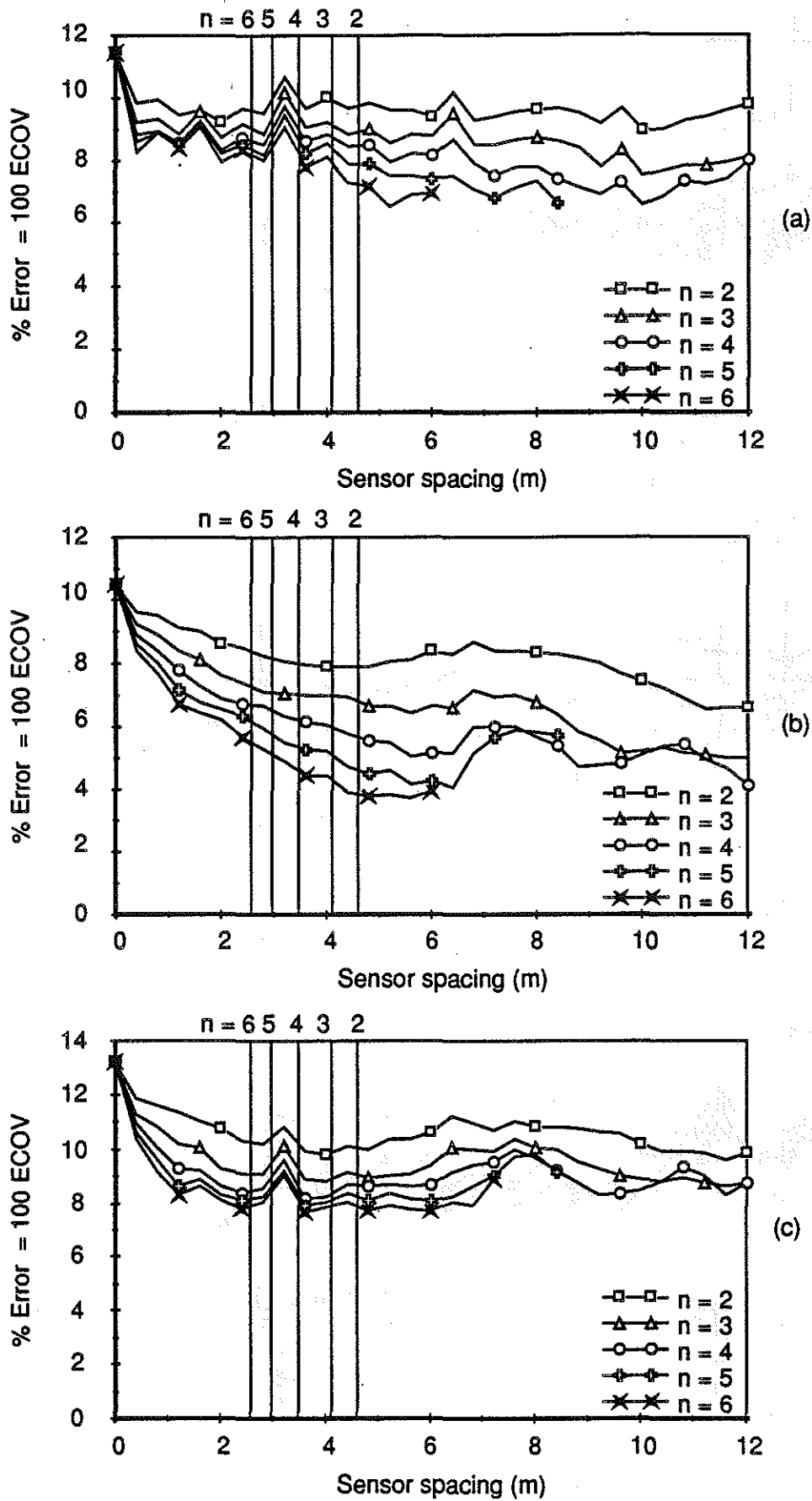
Fig. 5.23 WIM array error vs sensor spacing Vehicle S2, Speed = 23.0 m/s (83 km/h) (a) Axle 1 (b) Axle 3 (c) Axle 5
