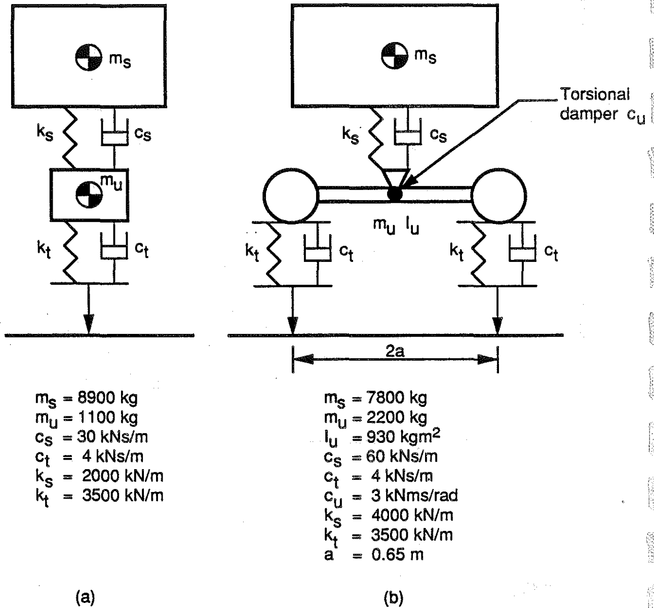
Fig. 4.5 Schematic diagrams of the two vehicle models (a) Model 1: 2 degrees of freedom, '1/4-car' (b) Model 2: 3 degrees of freedom, 'walking-beam.'
