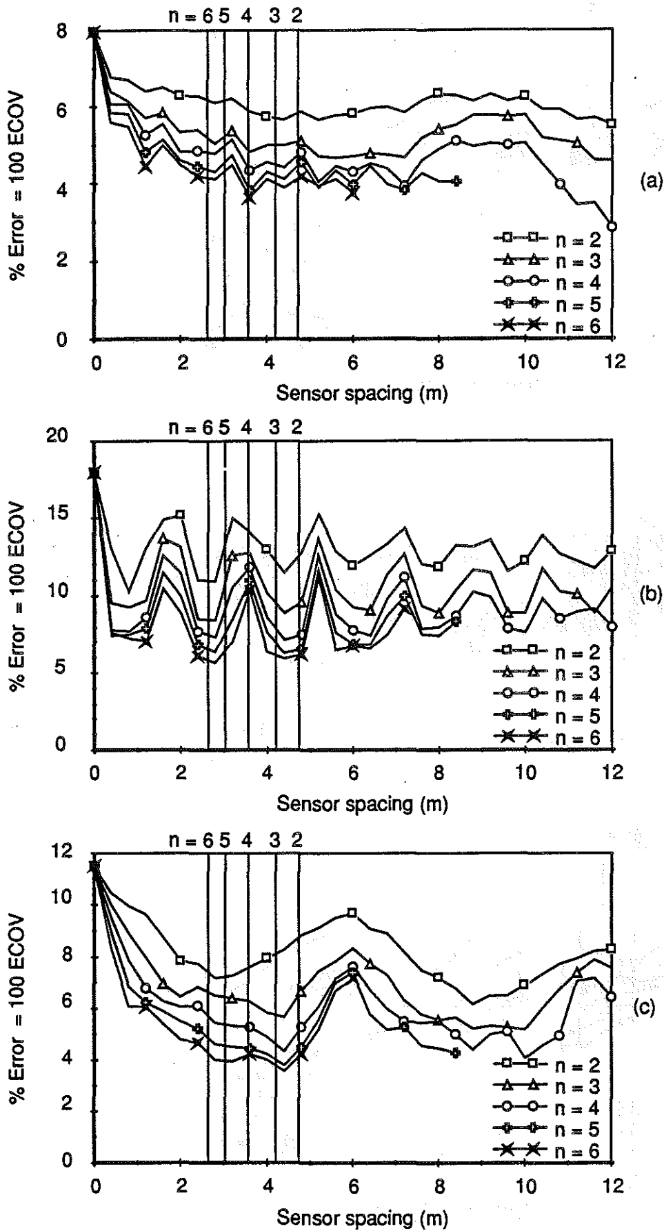
Fig. 5.35 WIM array error vs sensor spacing Vehicle S4, Speed = 23.7 m/s (85 km/h) (a) Axle 1 (b) Axle 3 (c) Axle 5
