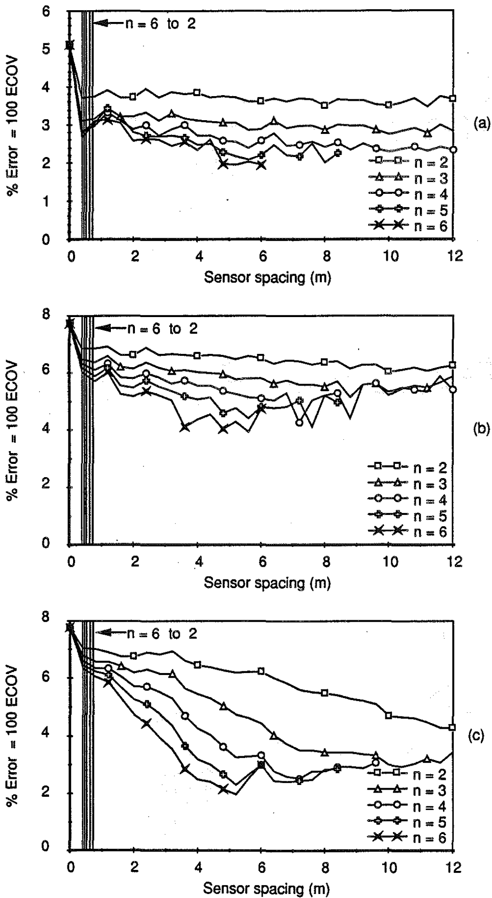
Fig. 5.43 WIM array error vs sensor spacing Vehicle S6, Speed = 3.6 m/s (13 km/h) (a) Axle 1 (b) Axle 3 (c) Axle 5
