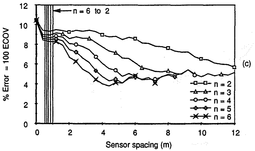
Fig. 5.37 WIM array error vs sensor spacing Vehicle S5, Speed = 4.9 m/s (18 km/h) (a) Axle 1 (b) Axle 3 (c) Axle 5
