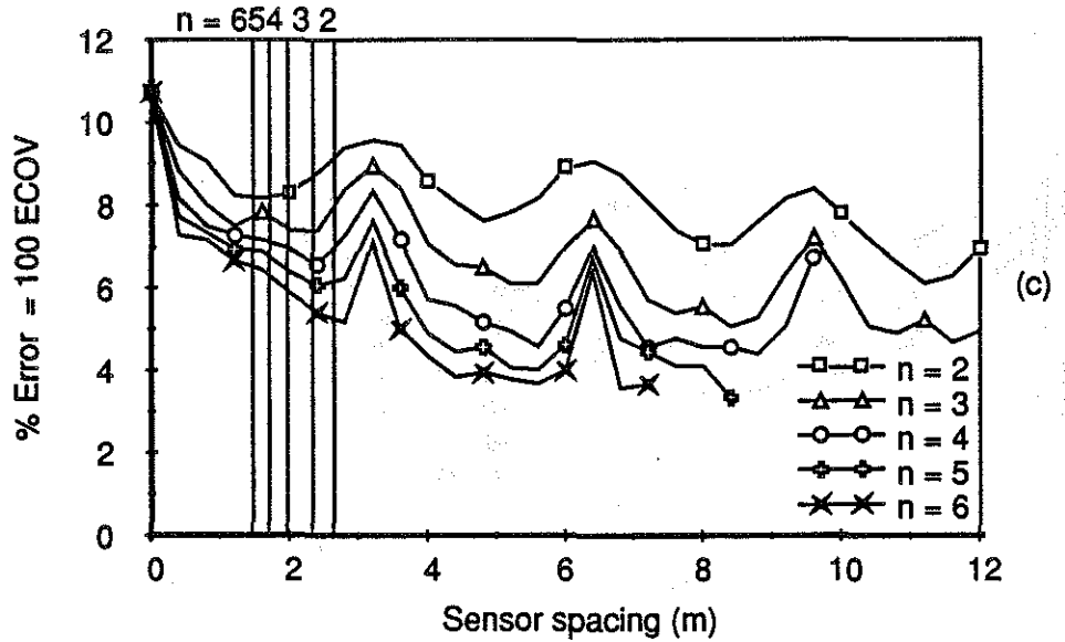
Fig. 5.45 WIM array error vs sensor spacing Vehicle S6, Speed = 13.2 m/s (47 km/h) (a) Axle 1 (b) Axle 3 (c) Axle 5
