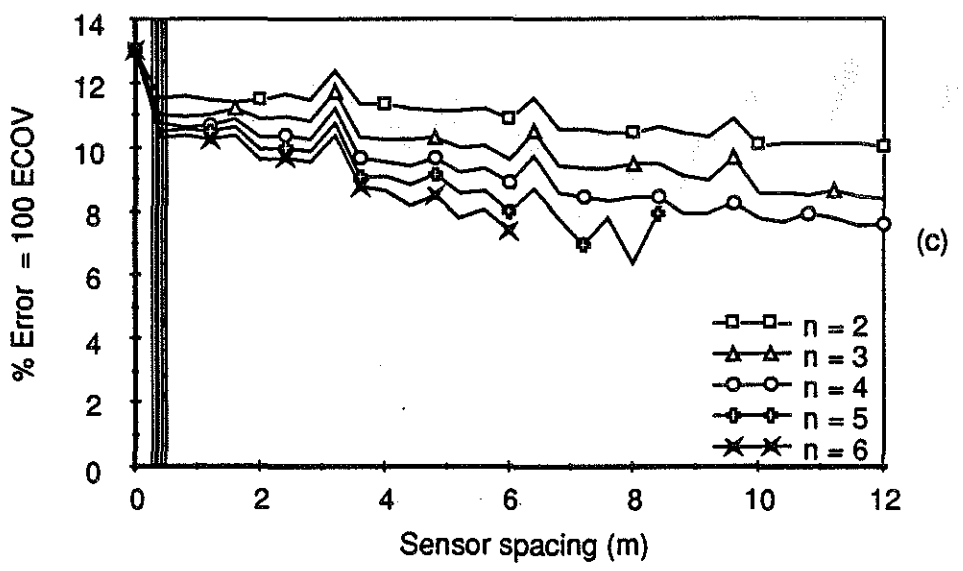
Fig. 5.12 WIM array error vs sensor spacing Vehicle S1, Speed = 2.5 m/s (9 km/h) (a) Axle 1 (b) Axle 3 (c) Axle 5
