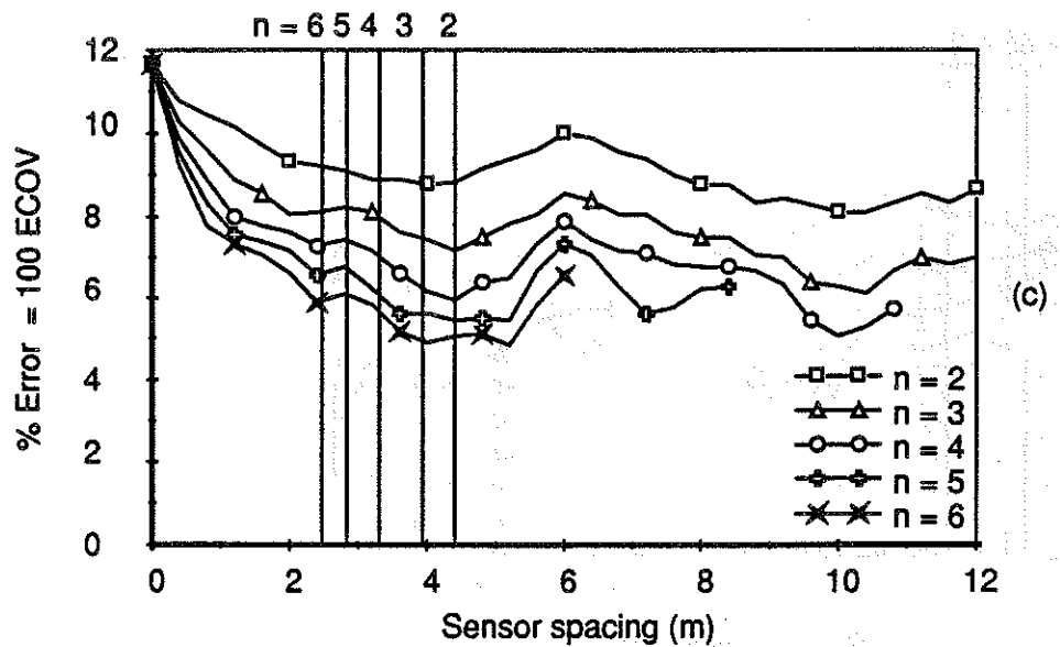
Fig. 5.47 WIM array error vs sensor spacing Vehicle S6, Speed = 22 m/s (79 km/h) (a) Axle 1 (b) Axle 3 (c) Axle 5
