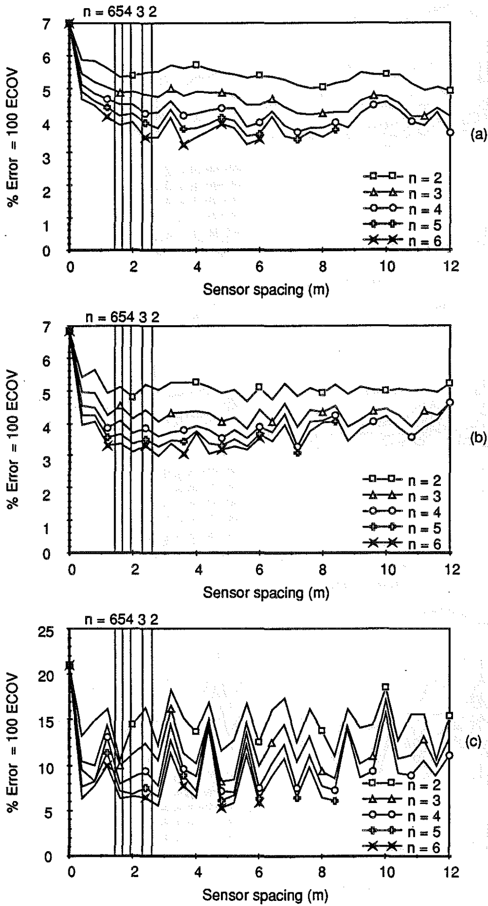
Fig. 5.27 WIM array error vs sensor spacing Vehicle S3, Speed = 13.0 m/s (47 km/h) (a) Axle 1 (b) Axle 3 (c) Axle 5
