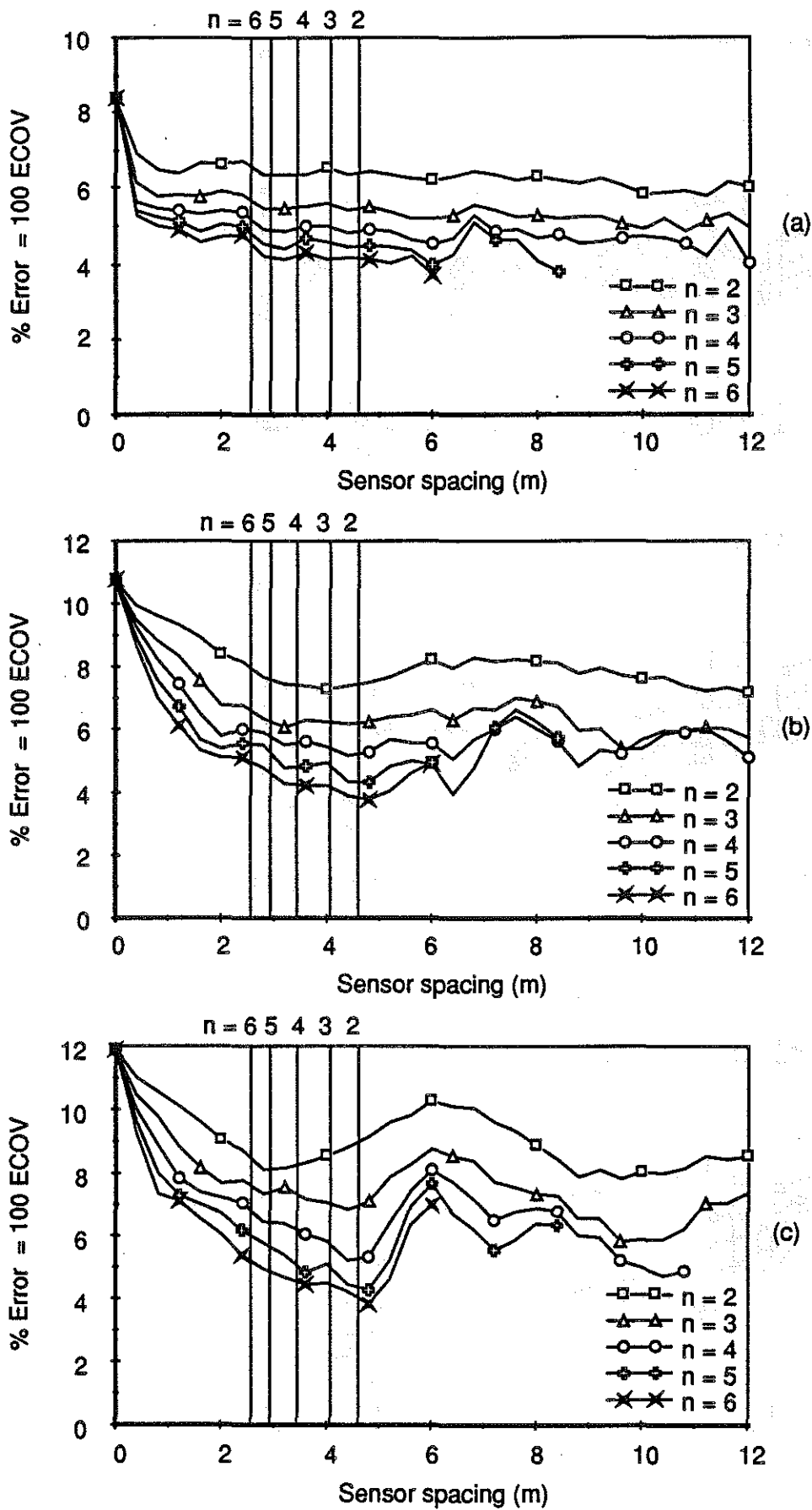
Fig. 5.41 WIM array error vs sensor spacing Vehicle S5, Speed = 23.0 m/s (83 km/h) (a) Axle 1 (b) Axle 3 (c) Axle 5
