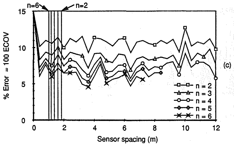
Fig. 5.26 WIM array error vs sensor spacing Vehicle S3, Speed = 9.1 m/s (33 km/h) (a) Axle 1 (b) Axle 3 (c) Axle 5
