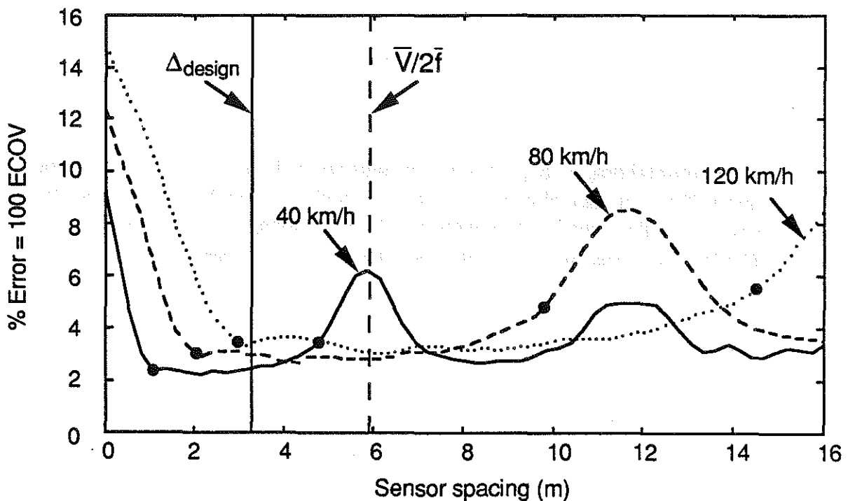
Fig. 5.10 Theoretical graph of \rho vs \Delta , for n = 6 and speeds of 40, 80 and 120 km/h. The design spacing was calculated using an average speed of 80 km/h and an average frequency of 1.9 Hz. The 'solid' circles on each curve correspond to \delta = 1/6 and \delta = 5/6 .
