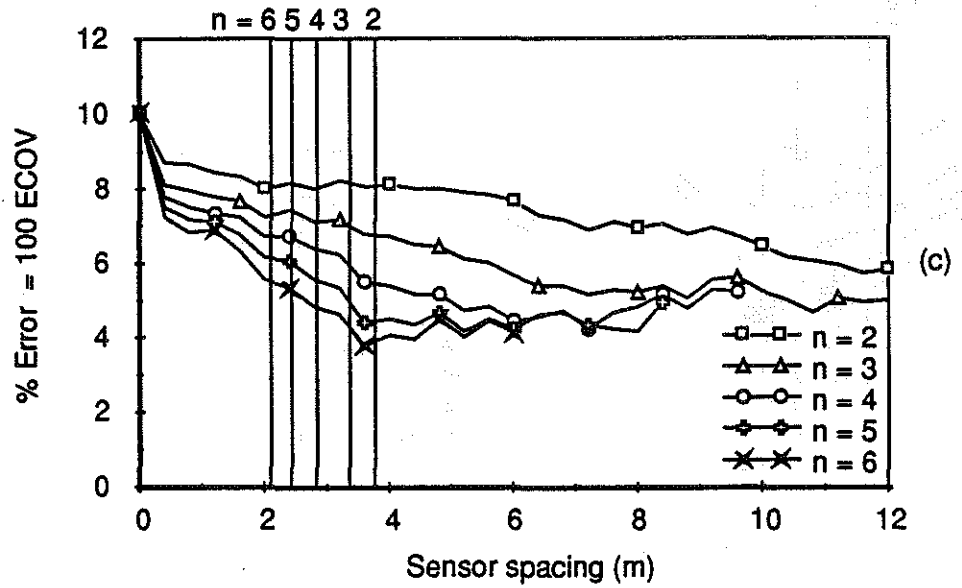
Fig. 5.40 WIM array error vs sensor spacing Vehicle S5, Speed = 18.9 m/s (68 km/h) (a) Axle 1 (b) Axle 3 (c) Axle 5
