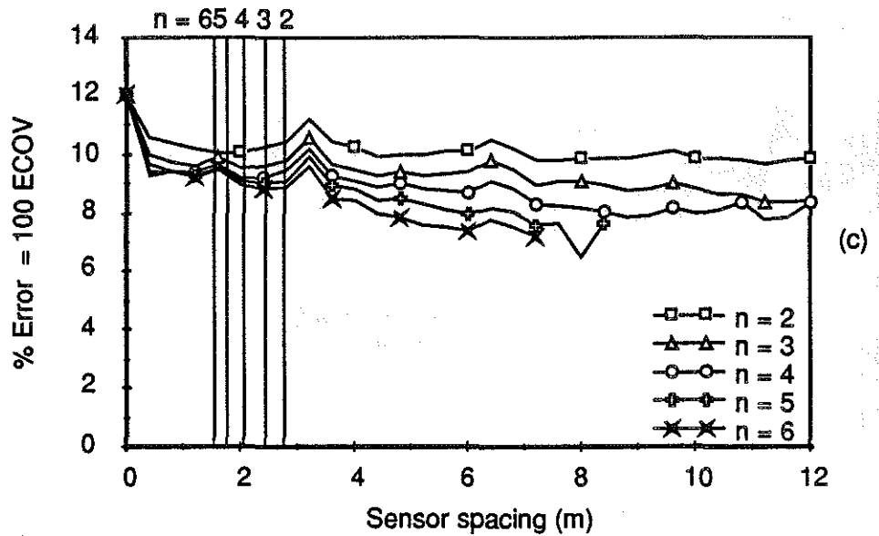
Fig. 5.21 WIM array error vs sensor spacing Vehicle S2, Speed = 13.8 m/s (50 km/h) (a) Axle 1 (b) Axle 3 (c) Axle 5
