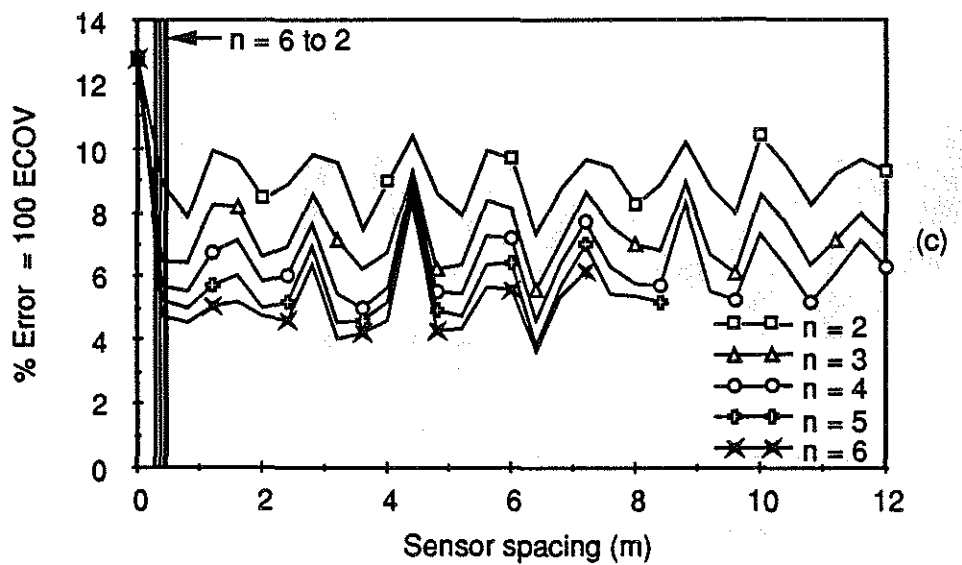
Fig. 5.24 WIM array error vs sensor spacing Vehicle S3, Speed = 2.4 m/s (8.5 km/h) (a) Axle 1 (b) Axle 3 (c) Axle 5
