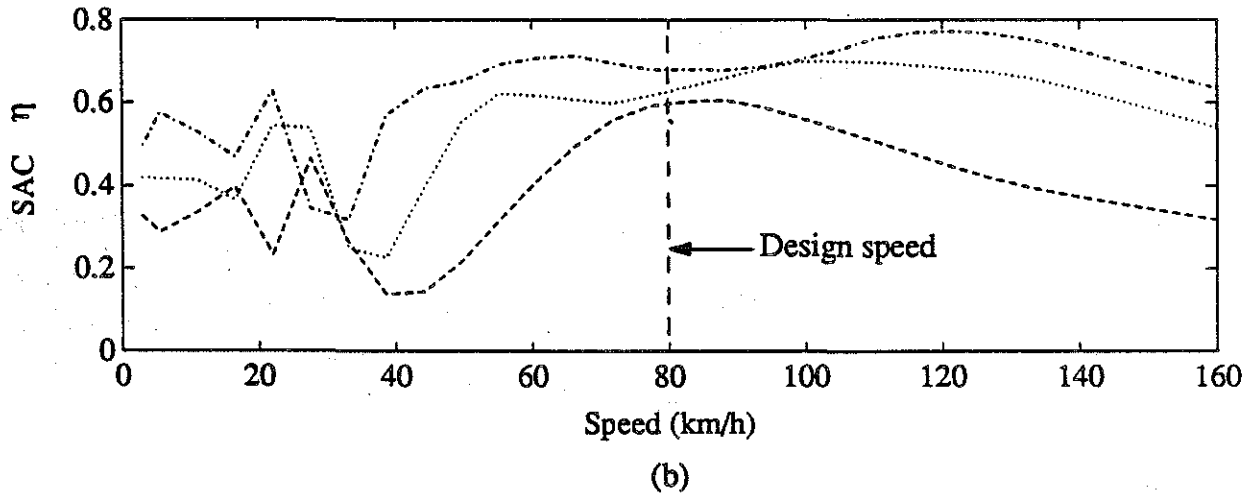
Fig. 4.9 Influence of speed on the performance of 2-, 3- and 4-sensor WIM systems, designed for an average traffic speed of 80 km/h, traversed by vehicle model 1. (a) Error Coefficient of Variation \rho . (b) Static Accuracy Coefficient \eta . — n=1 (DLC), - - - n=2 , ..... n=3 , - · - · - n=4 .
