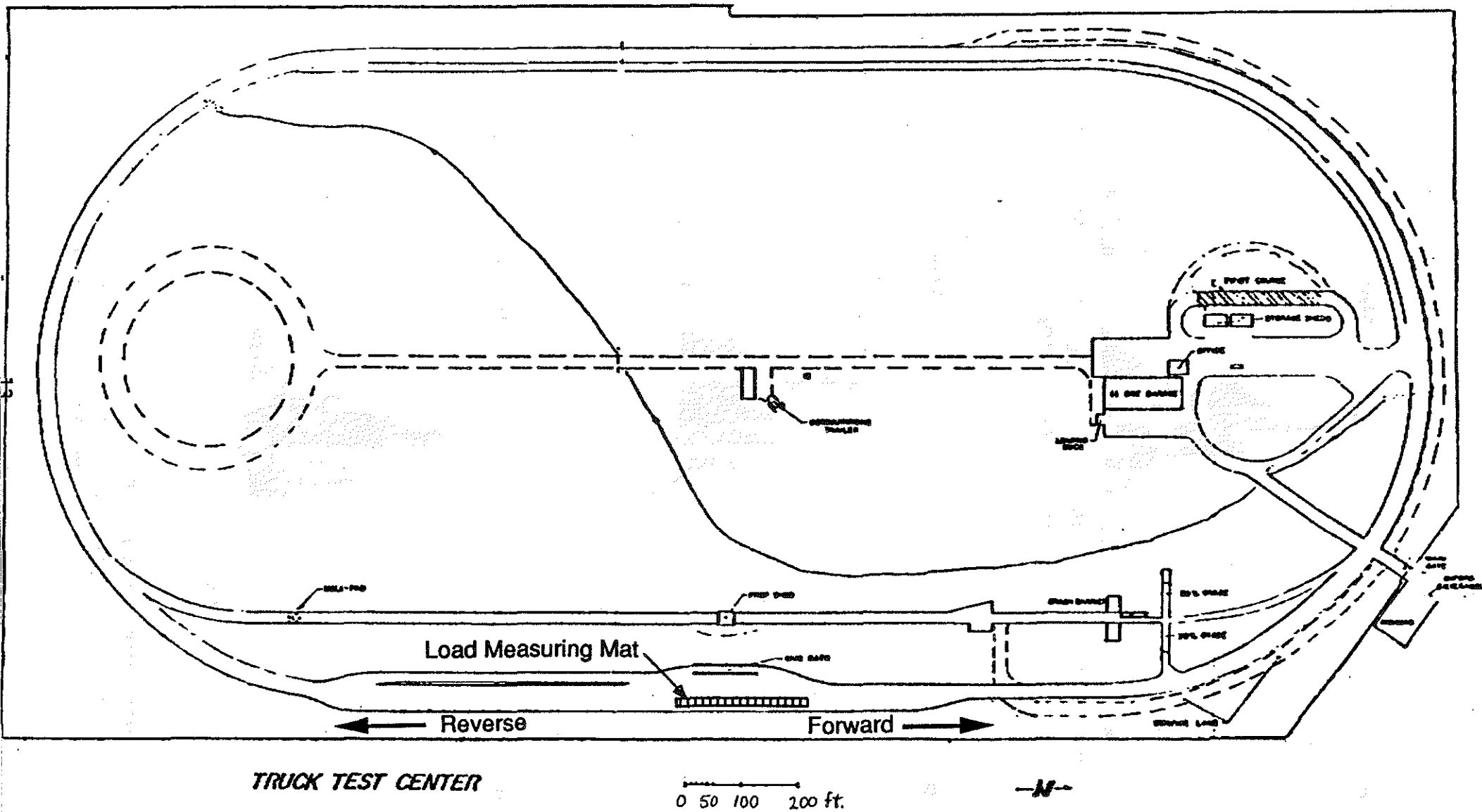
Fig. 2.2 Plan of the Navistar Test Track, showing the site of the mat installation.
