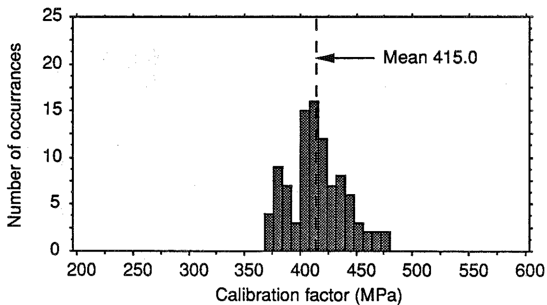
Fig. 2.3 Histograms of sensor calibration factors (a) Bare sensor calibrator (b) 'In-situ' calibrator (c) Field calibration with steer axles of 6 vehicles
