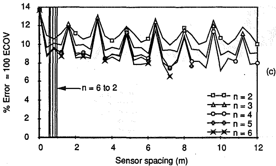
Fig. 5.19 WIM array error vs sensor spacing Vehicle S2, Speed = 4.8 m/s (17 km/h) (a) Axle 1 (b) Axle 3 (c) Axle 5
