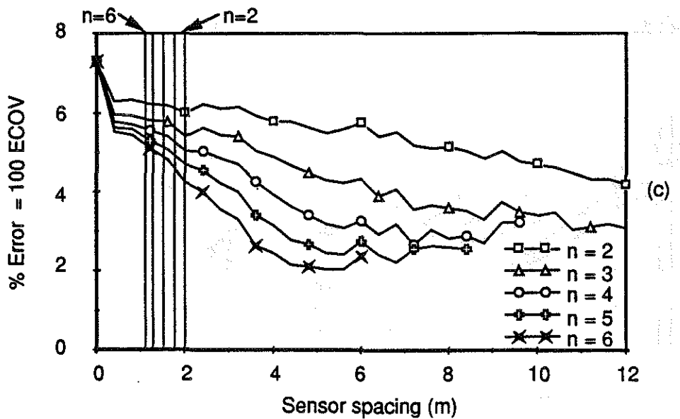
Fig. 5.32 WIM array error vs sensor spacing Vehicle S4, Speed = 9.9 m/s (36 km/h) (a) Axle 1 (b) Axle 3 (c) Axle 5
