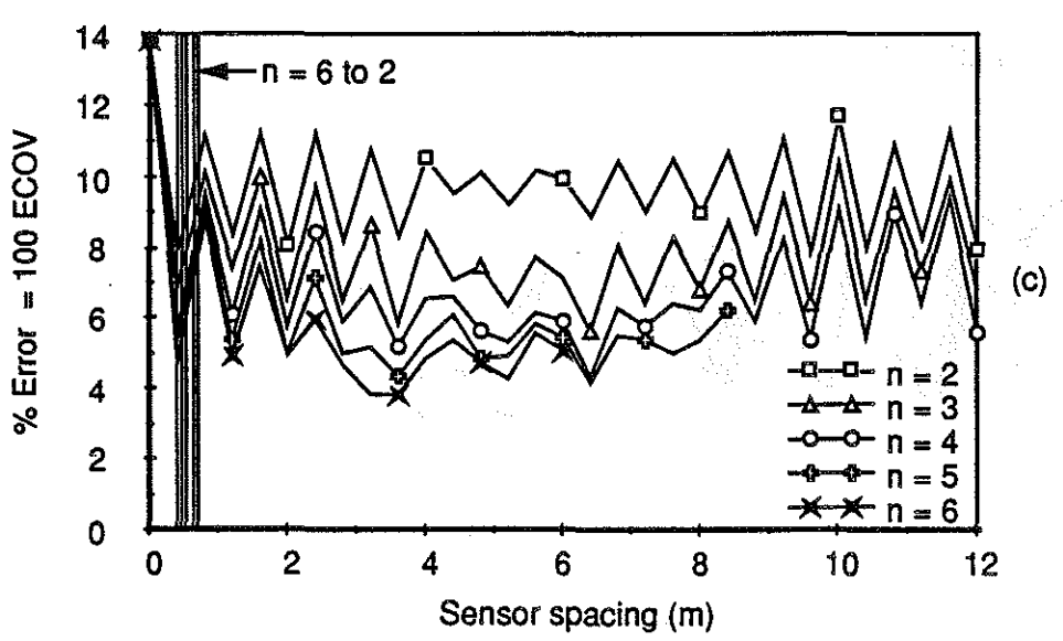
Fig. 5.25 WIM array error vs sensor spacing Vehicle S3, Speed = 3.5 m/s (13 km/h) (a) Axle 1 (b) Axle 3 (c) Axle 5
