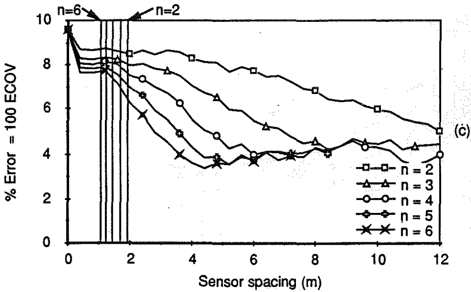
Fig. 5.38 WIM array error vs sensor spacing Vehicle S5, Speed = 9.6 m/s (35 km/h) (a) Axle 1 (b) Axle 3 (c) Axle 5
