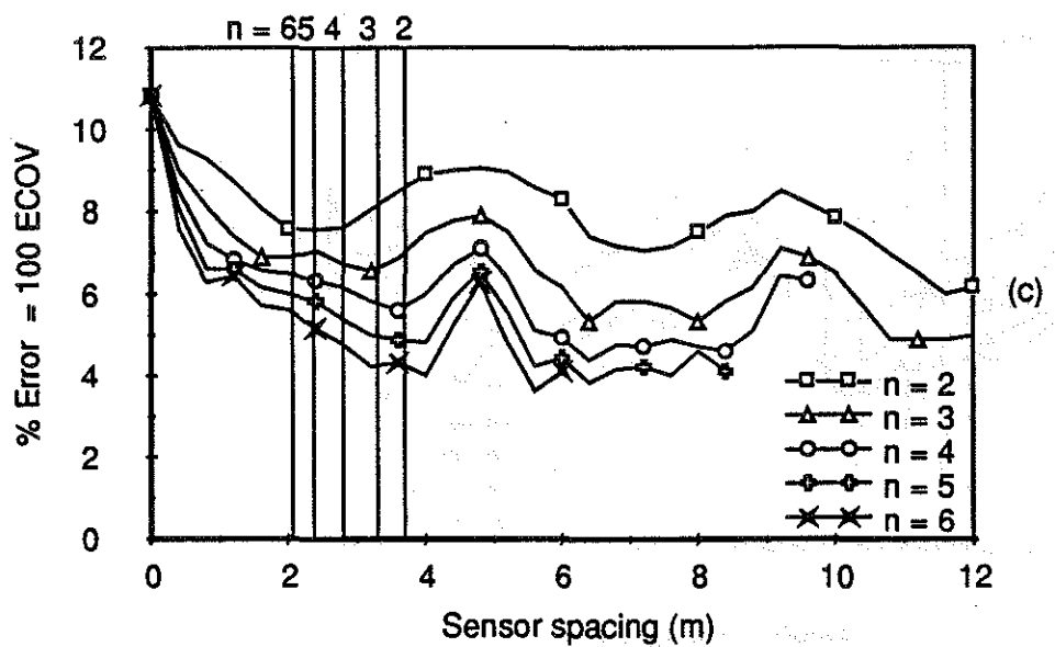
Fig. 5.34 WIM array error vs sensor spacing Vehicle S4, Speed = 18.6 m/s (67 km/h) (a) Axle 1 (b) Axle 3 (c) Axle 5
