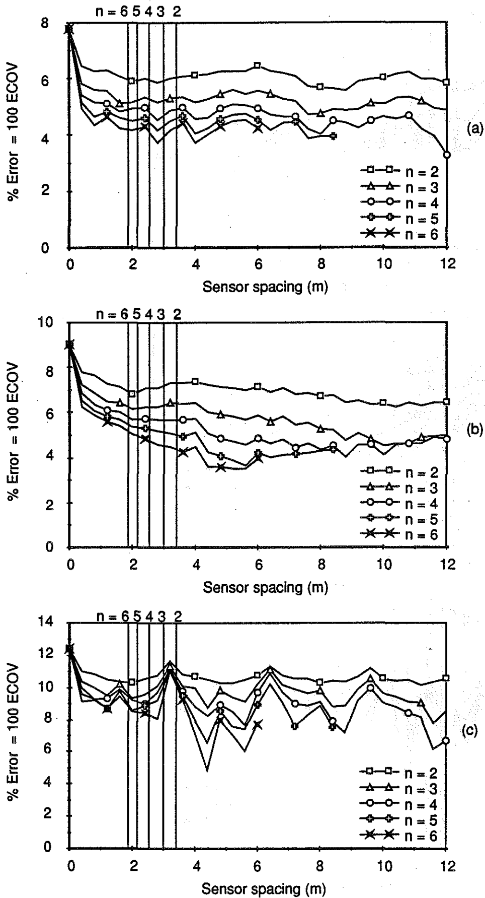
Fig. 5.16 WIM array error vs sensor spacing Vehicle S1, Speed = 16.9 m/s (61 km/h) (a) Axle 1 (b) Axle 3 (c) Axle 5
