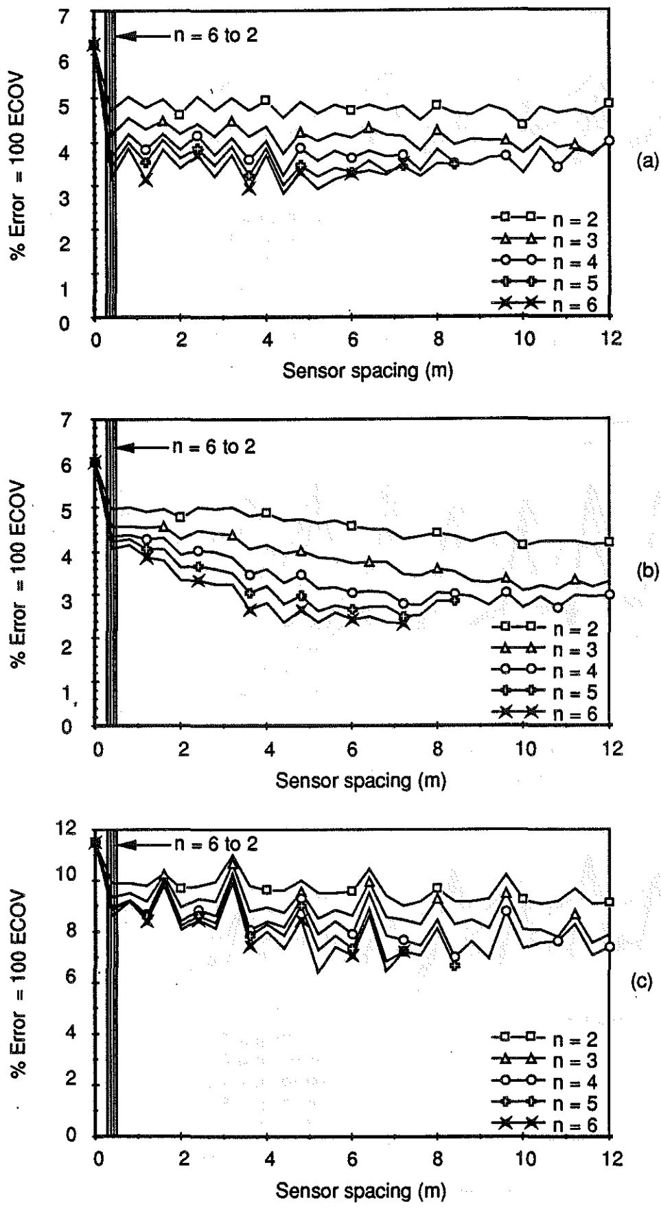
Fig. 5.18 WIM array error vs sensor spacing Vehicle S2, Speed = 2.4 m/s (8.7 km/h) (a) Axle 1 (b) Axle 3 (c) Axle 5
