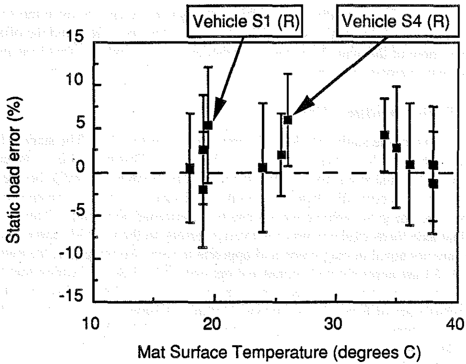
Fig 3.1 Static load errors, steering axles, Vehicles S1-S6. The error bars indicate one standard deviation either side of the mean
