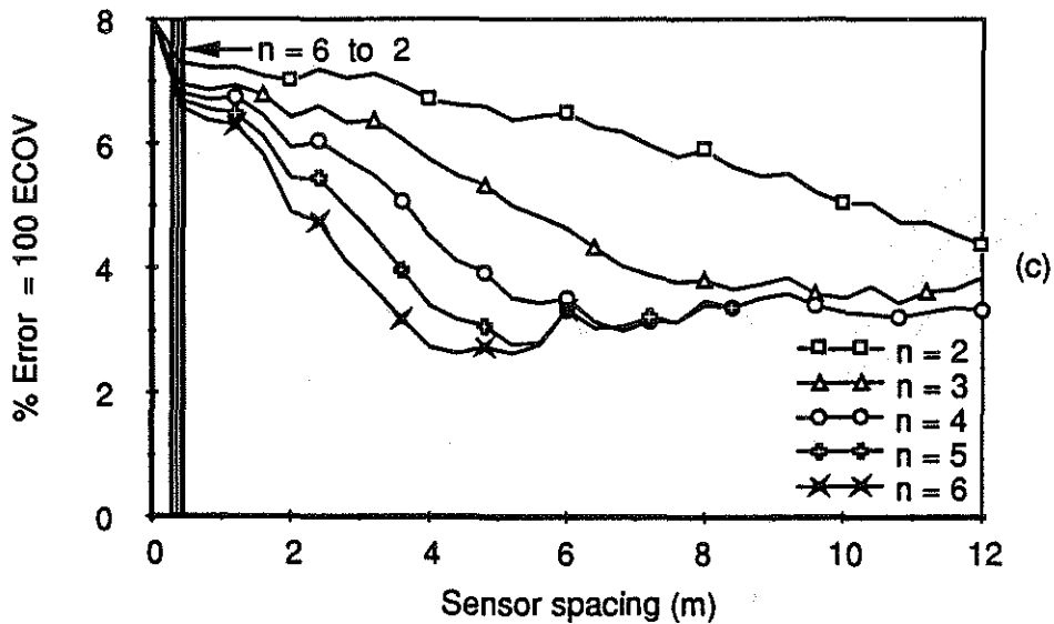
Fig. 5.42 WIM array error vs sensor spacing Vehicle S6, Speed = 2.4 m/s (8.6 km/h) (a) Axle 1 (b) Axle 3 (c) Axle 5
