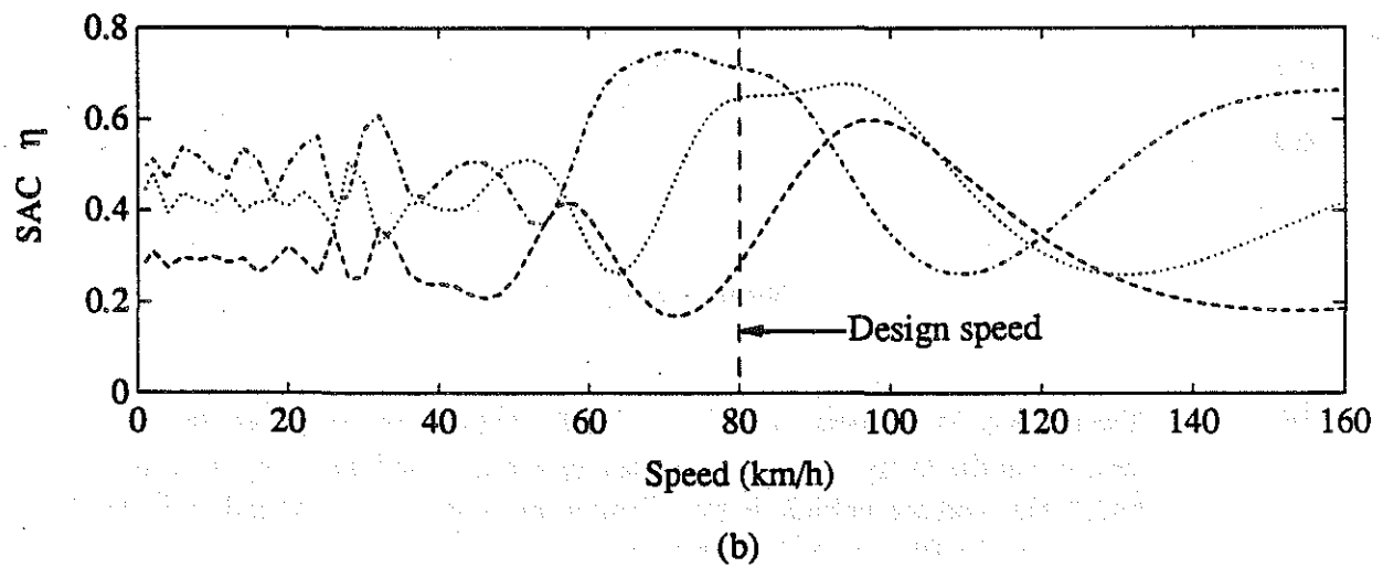
Fig 4.12 Influence of speed on the performance of 2-, 3- and 4-sensor WIM systems, designed for \bar{f} = 2.5 Hz and \bar{V} = 80 km/h, and trafficked by vehicle model 2. (a) Error Coefficient of Variation \rho , (b) Static Accuracy Coefficient \eta . ——— n=1 (DLC), - - - - - n=2 , ..... n=3 , - · - · - n=4 .
