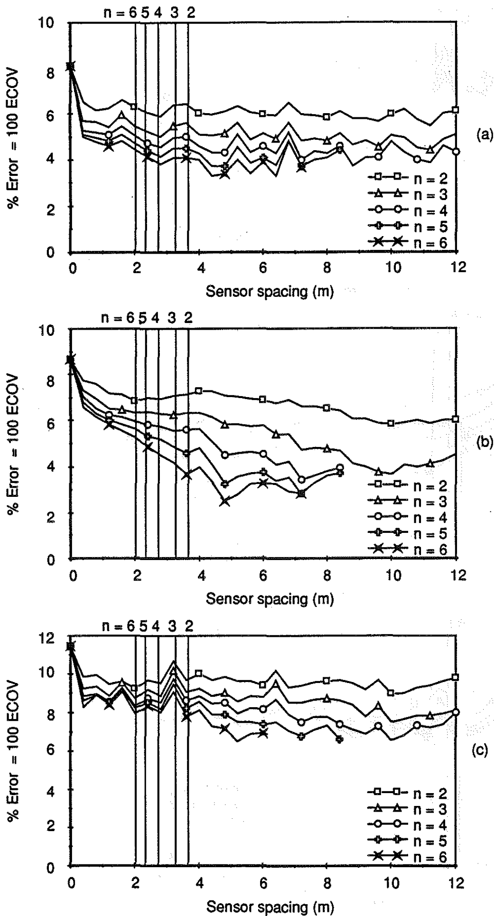
Fig. 5.22 WIM array error vs sensor spacing Vehicle S2, Speed = 18.3 m/s (66 km/h) (a) Axle 1 (b) Axle 3 (c) Axle 5
