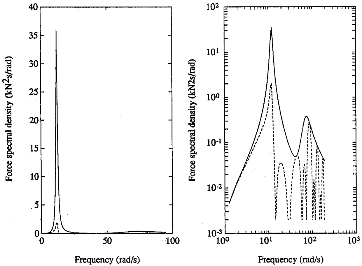
Fig. 4.6 Tyre force spectral density S_{pp}(\omega) and the WIM array error spectral density S_{cc}(\omega) for vehicle model 1 travelling at 100 km/h over a WIM array with n=3 and \Delta = 4 m.
