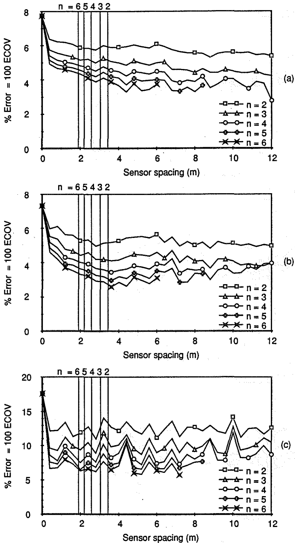
Fig. 5.28 WIM array error vs sensor spacing Vehicle S3, Speed = 17.1 m/s (62 km/h) (a) Axle 1 (b) Axle 3 (c) Axle 5
