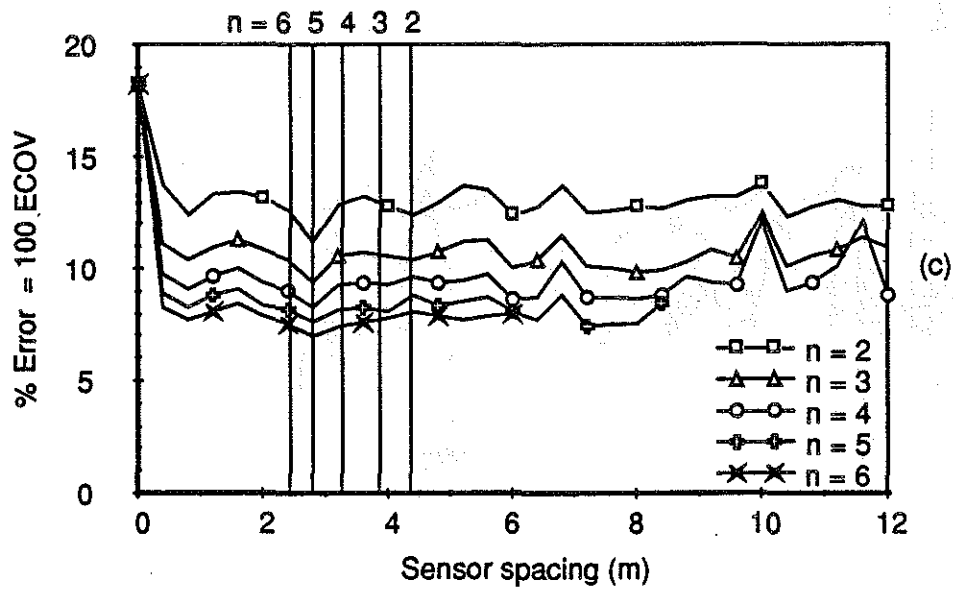
Fig. 5.29 WIM array error vs sensor spacing Vehicle S3, Speed = 21.8 m/s (78 km/h) (a) Axle 1 (b) Axle 3 (c) Axle 5
