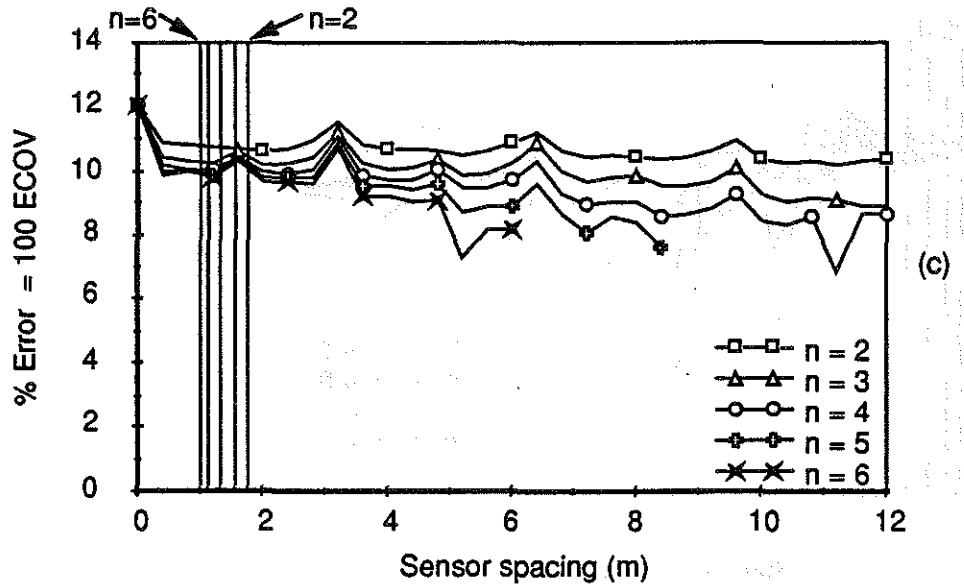
Fig. 5.14 WIM array error vs sensor spacing Vehicle S1, Speed = 8.9 m/s (32 km/h) (a) Axle 1 (b) Axle 3 (c) Axle 5
