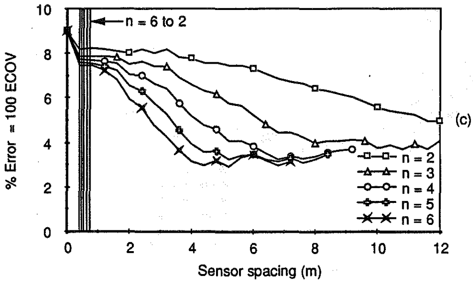
Fig. 5.36 WIM array error vs sensor spacing Vehicle S5, Speed = 3.6 m/s (13 km/h) (a) Axle 1 (b) Axle 3 (c) Axle 5
