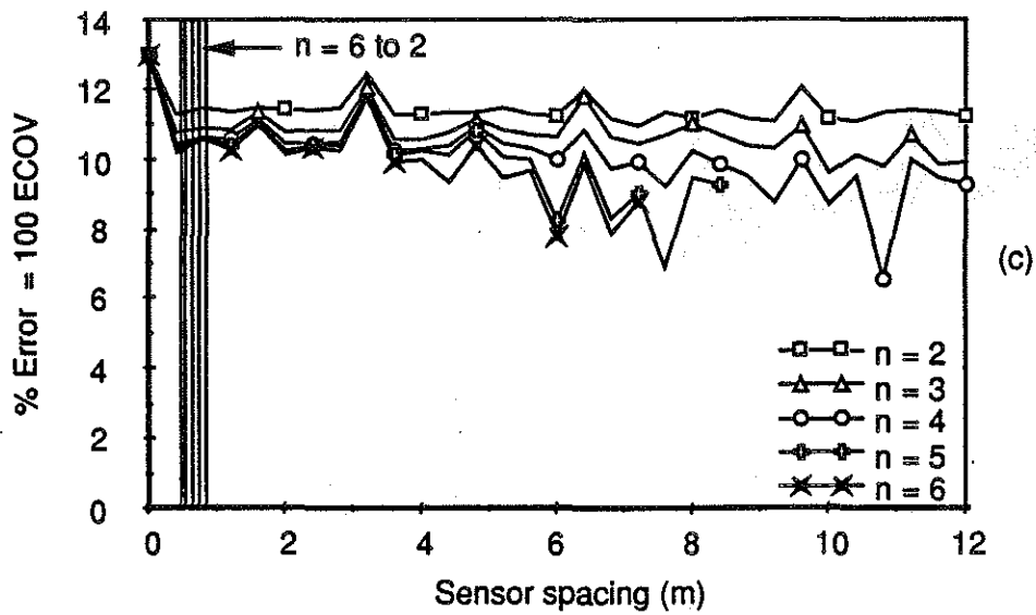
Fig. 5.13 WIM array error vs sensor spacing Vehicle S1, Speed = 4.1 m/s (15 km/h) (a) Axle 1 (b) Axle 3 (c) Axle 5
