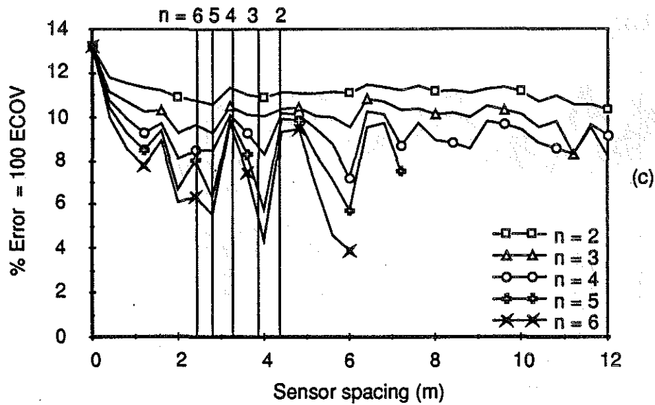
Fig. 5.17 WIM array error vs sensor spacing Vehicle S1, Speed = 21.8 m/s (79 km/h) (a) Axle 1 (b) Axle 3 (c) Axle 5
