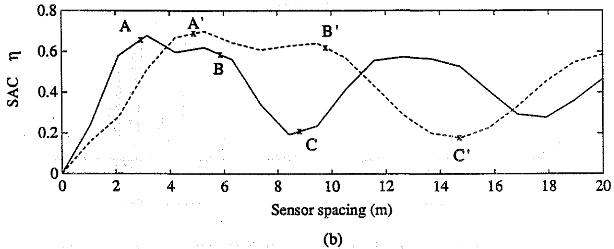
Fig. 4.7 WIM system performance versus sensor spacing \Delta for vehicle model 1. Points A, B, C etc. were calculated according to the theory for sinusoidal inputs. (a) Error Coefficient of Variation \rho . (b) Static Accuracy Coefficient \eta . — = 60 km/h, - - - = 100 km/h
