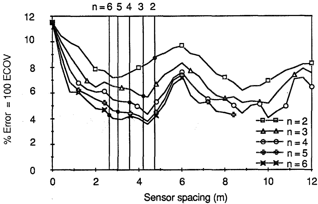
Fig. 5.7 Experimental WIM Error Coefficient of Variation \rho vs sensor spacing \Delta , Vehicle S4, speed 85 km/h, axle 5 (on trailer). Vertical lines denote design spacings according to eq 4.22.
