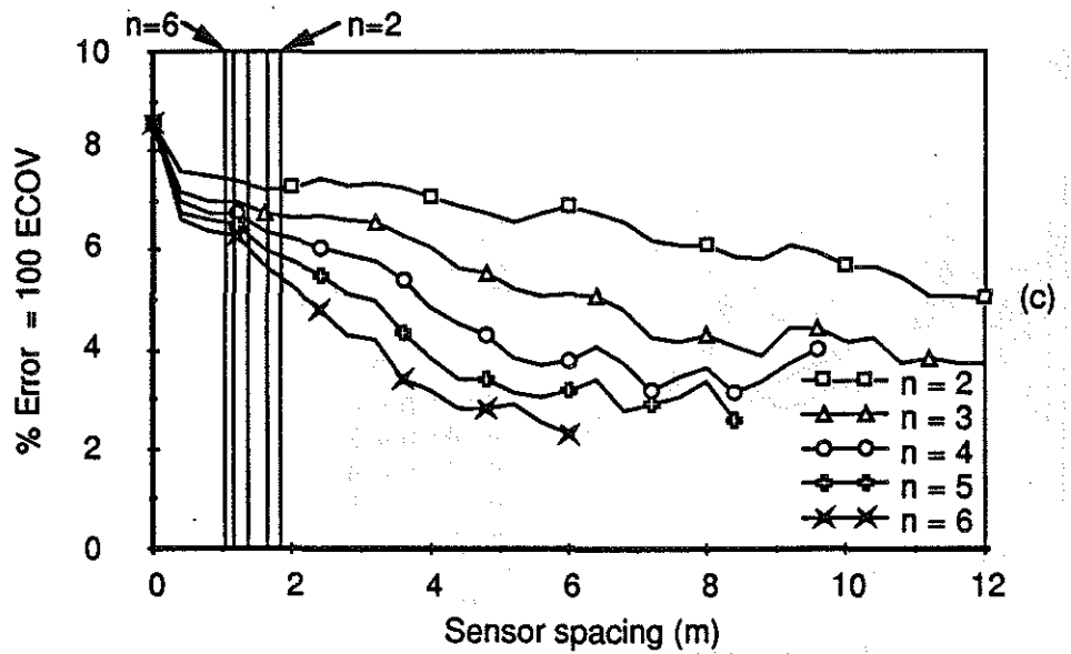
Fig. 5.44 WIM array error vs sensor spacing Vehicle S6, Speed = 9.1 m/s (33 km/h) (a) Axle 1 (b) Axle 3 (c) Axle 5
