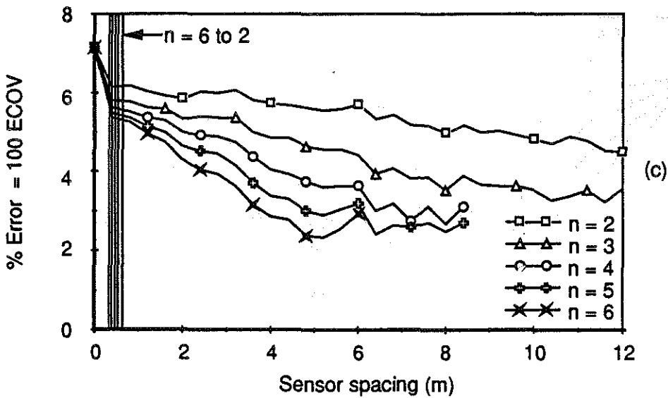
Fig. 5.30 WIM array error vs sensor spacing Vehicle S4, Speed = 3.1 m/s (11 km/h) (a) Axle 1 (b) Axle 3 (c) Axle 5
