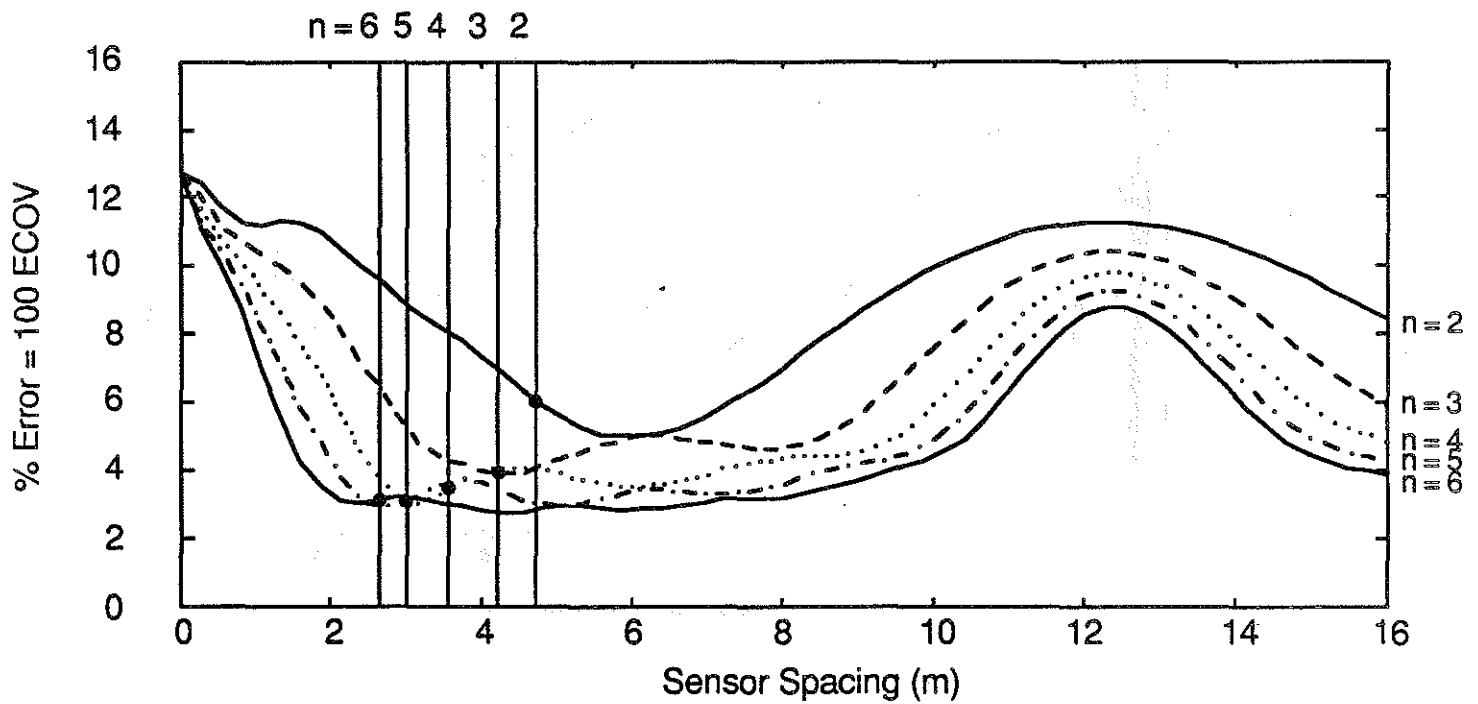
Fig. 5.8 Theoretical WIM array Error Coefficient of Variation \rho vs sensor spacing \Delta , 1/4-car model, speed = 85 km/h. Vertical lines denote design spacings according to eq 4.22.
