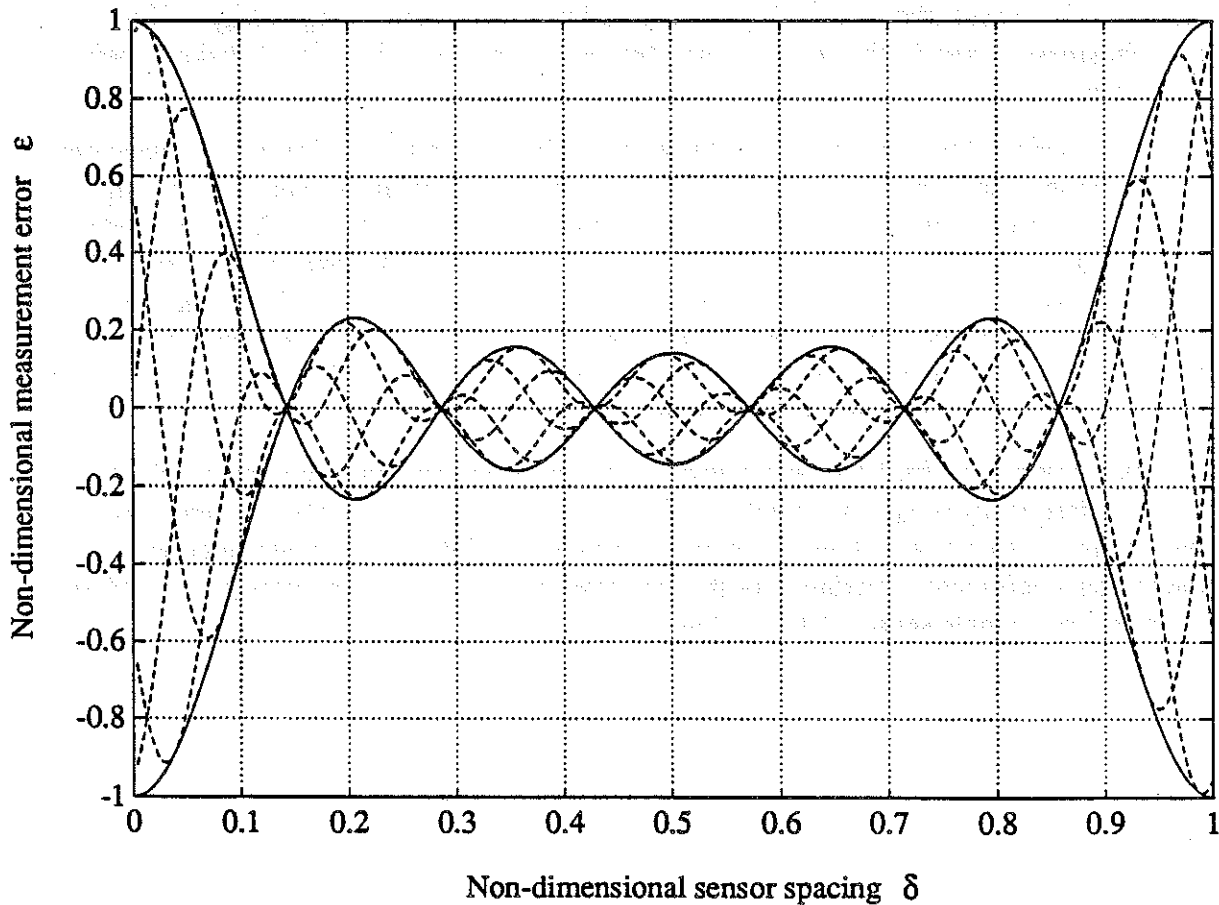
Fig. 4.2 Plot of equation 4.5 for n=7 with 5 different phase angles, \phi = 2\pi/5, 4\pi/5, \dots, 2\pi , (dashed lines) as well as the envelope error \hat{\epsilon} from eq. 4.7, (solid lines).
