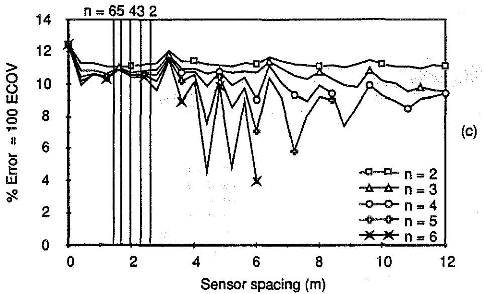
Fig. 5.15 WIM array error vs sensor spacing Vehicle S1, Speed = 13.0 m/s (47 km/h) (a) Axle 1 (b) Axle 3 (c) Axle 5
