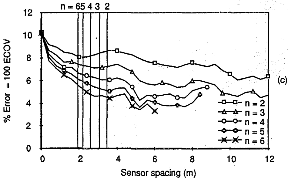
Fig. 5.46 WIM array error vs sensor spacing Vehicle S6, Speed = 17.3 m/s (62 km/h) (a) Axle 1 (b) Axle 3 (c) Axle 5
