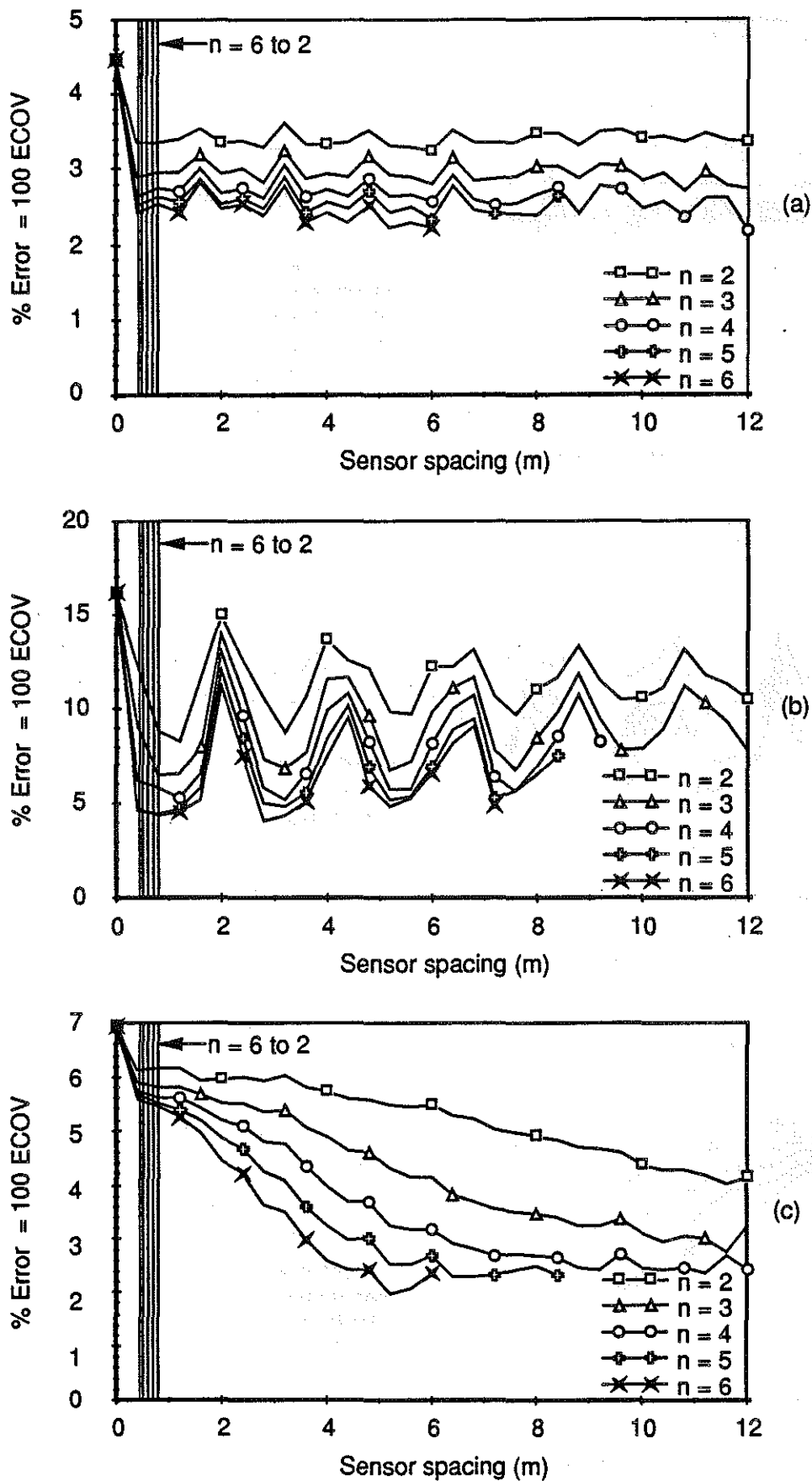
Fig. 5.31 WIM array error vs sensor spacing Vehicle S4, Speed = 4.0 m/s (14 km/h) (a) Axle 1 (b) Axle 3 (c) Axle 5
