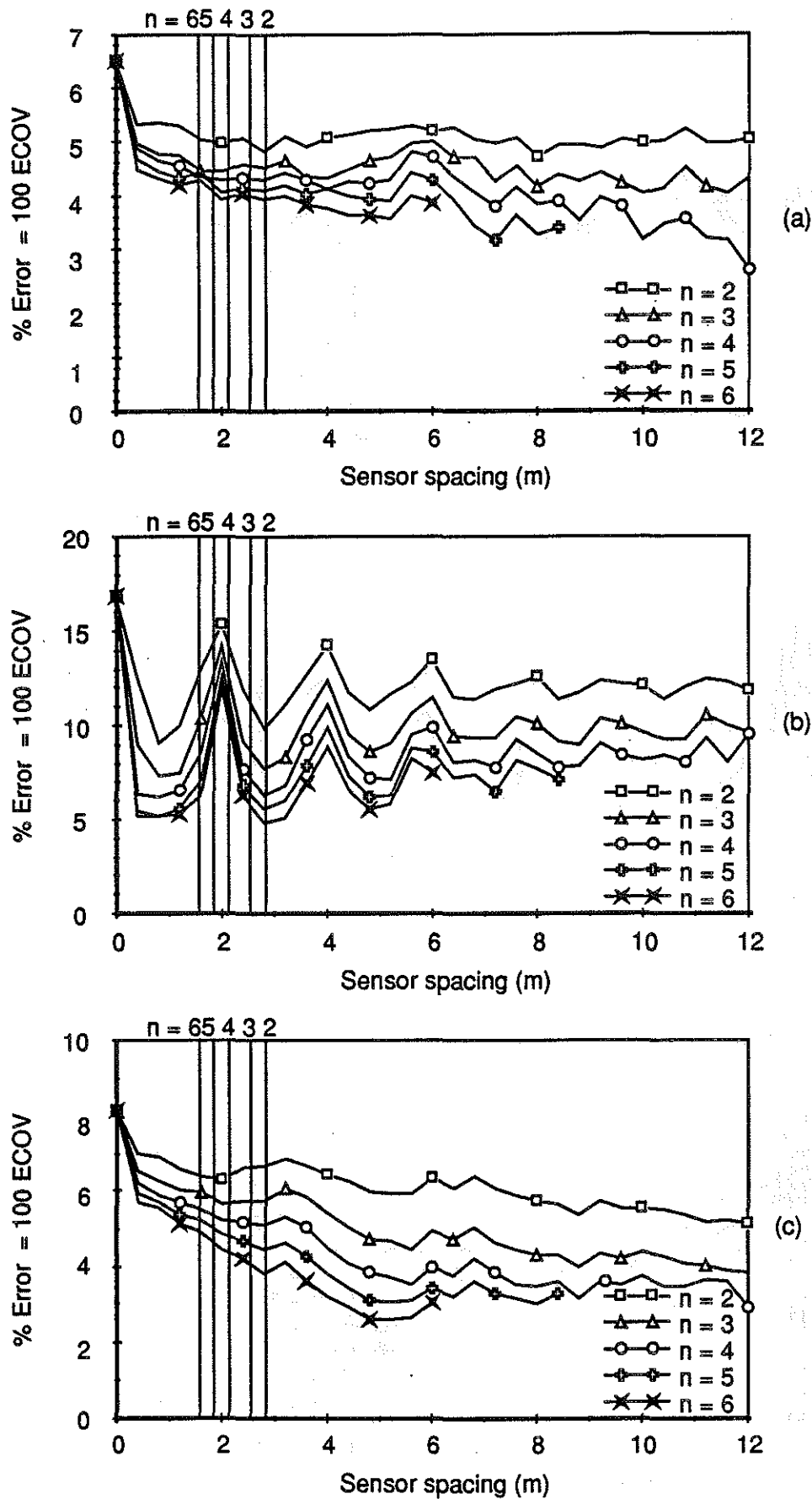
Fig. 5.33 WIM array error vs sensor spacing Vehicle S4, Speed = 14.2 m/s (51 km/h) (a) Axle 1 (b) Axle 3 (c) Axle 5
