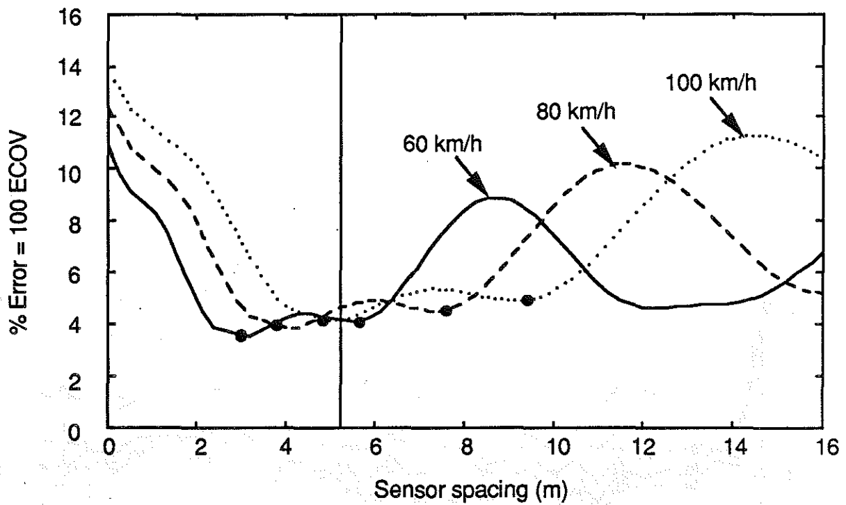
Fig. 5.9 Theoretical graph of \rho vs \Delta , for n = 3 and speeds of 60, 80 and 100 km/h. The design spacing was calculated using an average speed of 80 km/h and an average frequency of 1.9 Hz. The 'solid' circles on each curve correspond to \delta = 1/3 and \delta = 2/3 .
