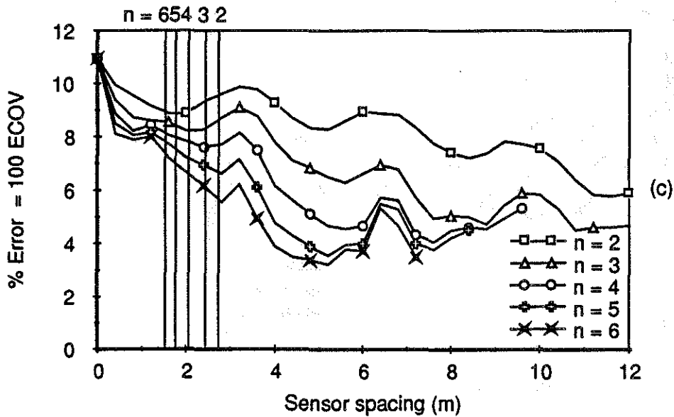
Fig. 5.39 WIM array error vs sensor spacing Vehicle S5, Speed = 13.7 m/s (49 km/h) (a) Axle 1 (b) Axle 3 (c) Axle 5
