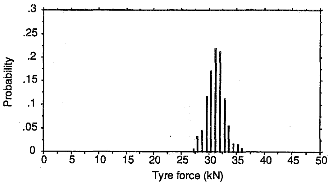
Fig. 5.2 Histograms of WIM average force, Vehicle S4, Axle 5, Speed = 23.7 m/s (85 km/h). (d) single sensor (e) 3 sensors, \Delta = 4.0 m (f) 6 sensors, \Delta = 2.4 m.
