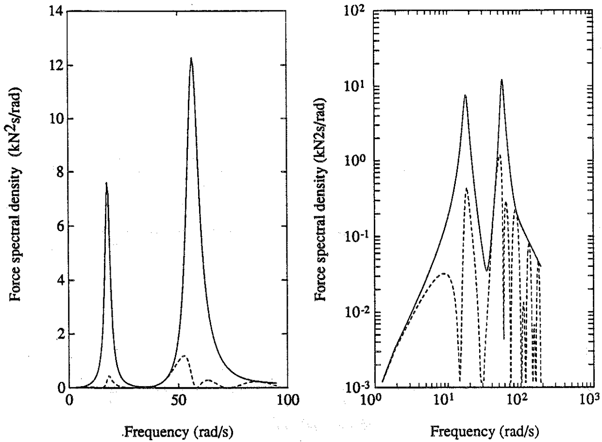
Fig 4.11 Leading tyre force and error spectral densities S_{pp}(\omega) and S_{ee}(\omega) for vehicle model 2 travelling at 100 km/h over a WIM array with n=3 and \Delta = 5 m. — = S_{pp}(\omega) , - - - = S_{ee}(\omega) .
