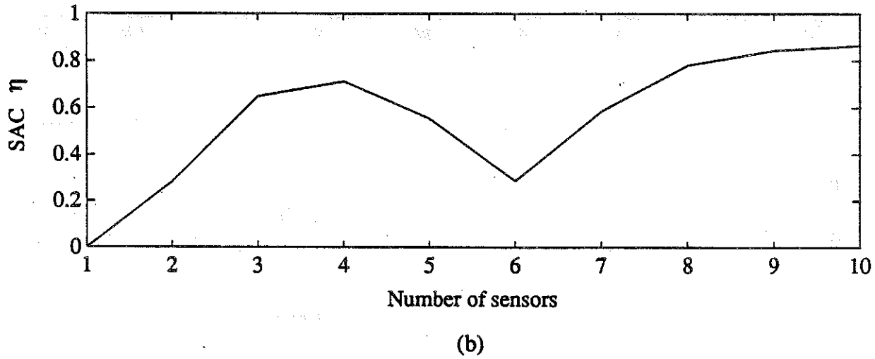
Fig 4.13 Variation of WIM system performance for vehicle model 2 with the number of sensors in the array. The sensors are spaced according to eq. 4.22 with \bar{f}=2.5 Hz and the vehicle is travelling at the array design speed of 80 km/h. (a) Error Coefficient of Variation \rho , (b) Static Accuracy Coefficient \eta .
