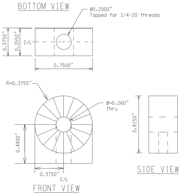
CENTER HINGE STAINLESS STEEL DETAIL "A"
