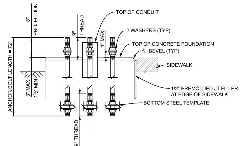
2 DETAIL - ANCHOR BOLTS
