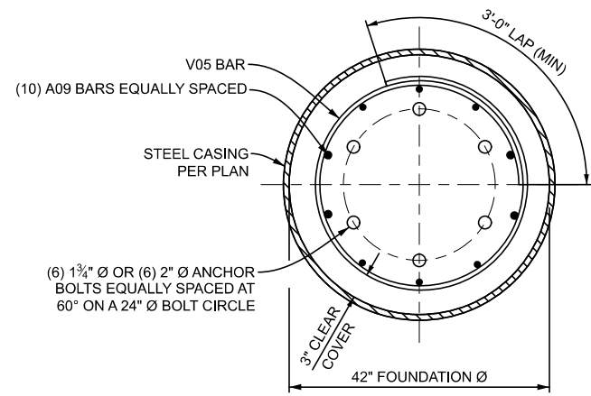
B SECTION - FOUNDATION PLAN
