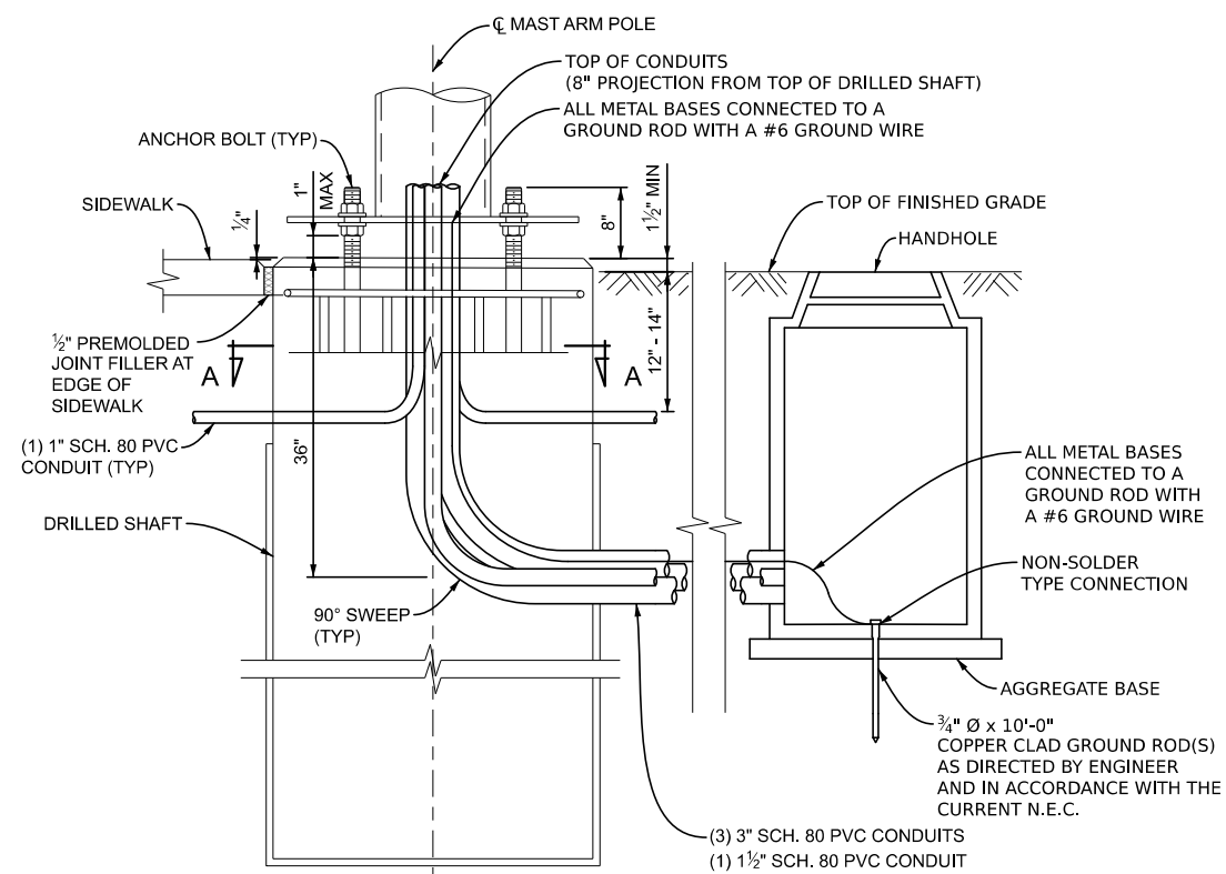
1 DETAIL - CONDUIT LAYOUT AND GROUNDING
