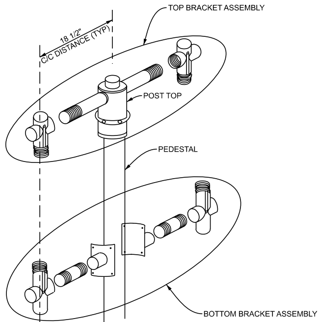
A DETAIL - SIGNAL MOUNTING HARDWARE FOR BACKSIDE BRACKET N.T.S.
