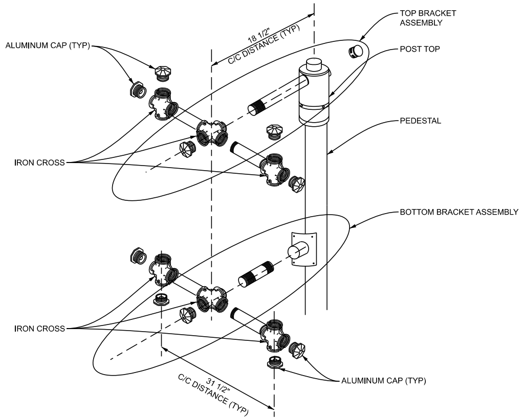
A DETAIL - SIGNAL MOUNTING HARDWARE FOR BACKSIDE BRACKET N.T.S.
