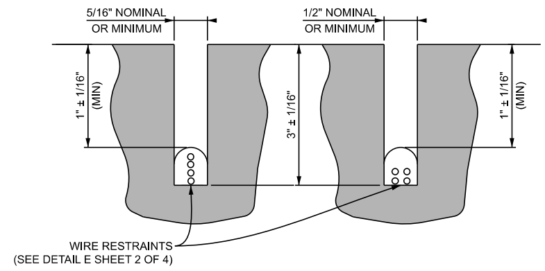
L SECTION A-A SECTION B-B LOOP SLOT LEAD-IN SLOT (BITUMINOUS PAVEMENT)
