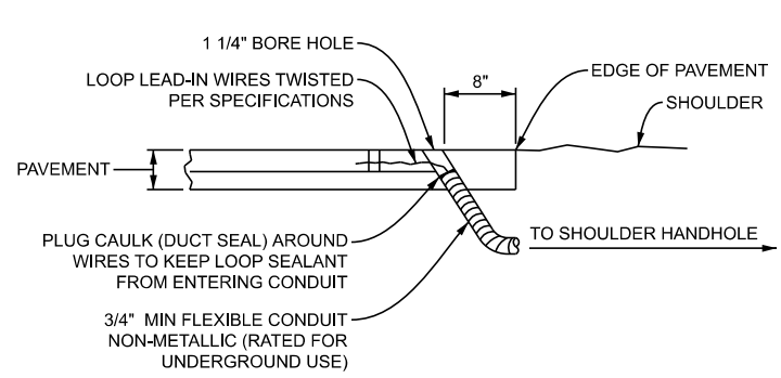
H BORE HOLE & LOOP WIRING SECTION F-F DETAIL - UNDER PAVEMENT INSTALLATION N.T.S.
