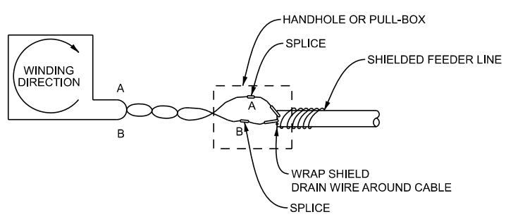
J DETAIL - SINGLE LOOP CONNECTION N.T.S.
