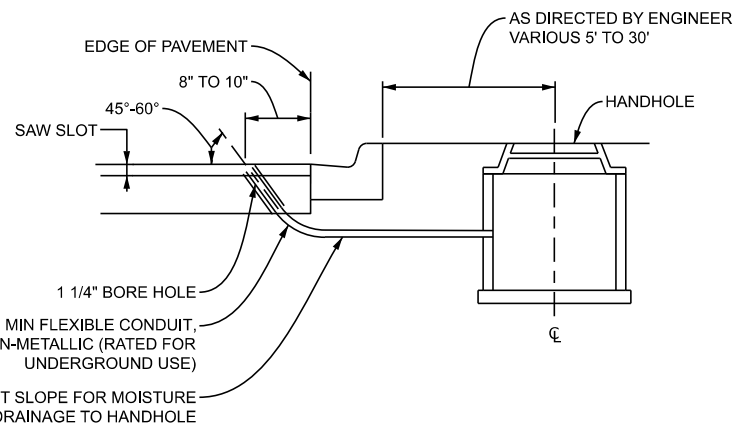
G TYPE II SECTION E-E DETAIL - UNDER CURB INSTALLATION N.T.S.
