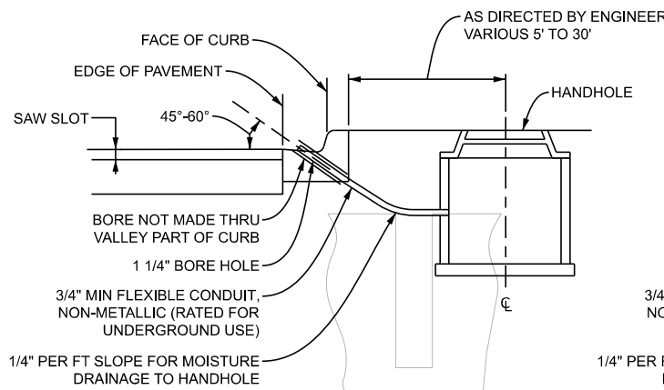
F TYPE I SECTION E-E DETAIL - UNDER CURB INSTALLATION N.T.S.
