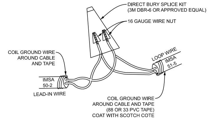
I DETAIL - HANDHOLE & PULL-BOX SPLICES (WATERPROOF) N.T.S.
