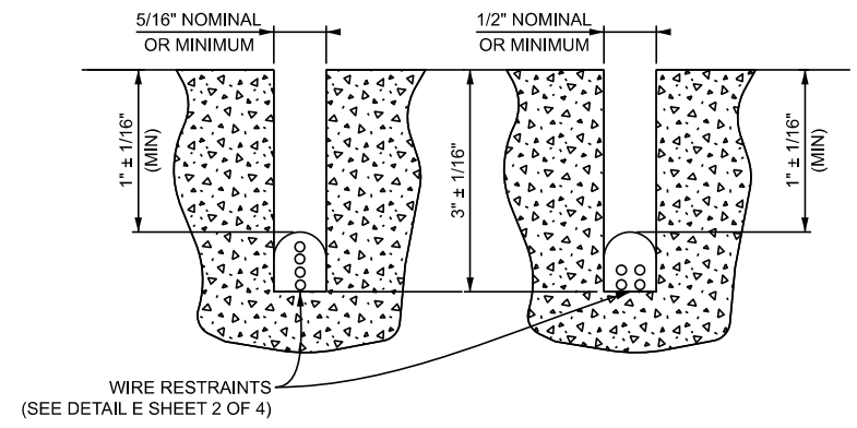
L SECTION A-A SECTION B-B LOOP SLOT LEAD-IN SLOT (CONCRETE PAVEMENT)
