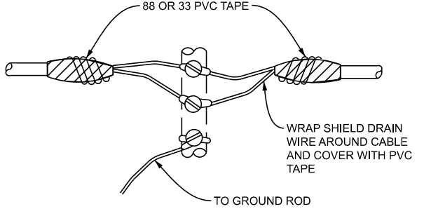
K DETAIL - CONTROLLER CABINET CONNECTION N.T.S.
