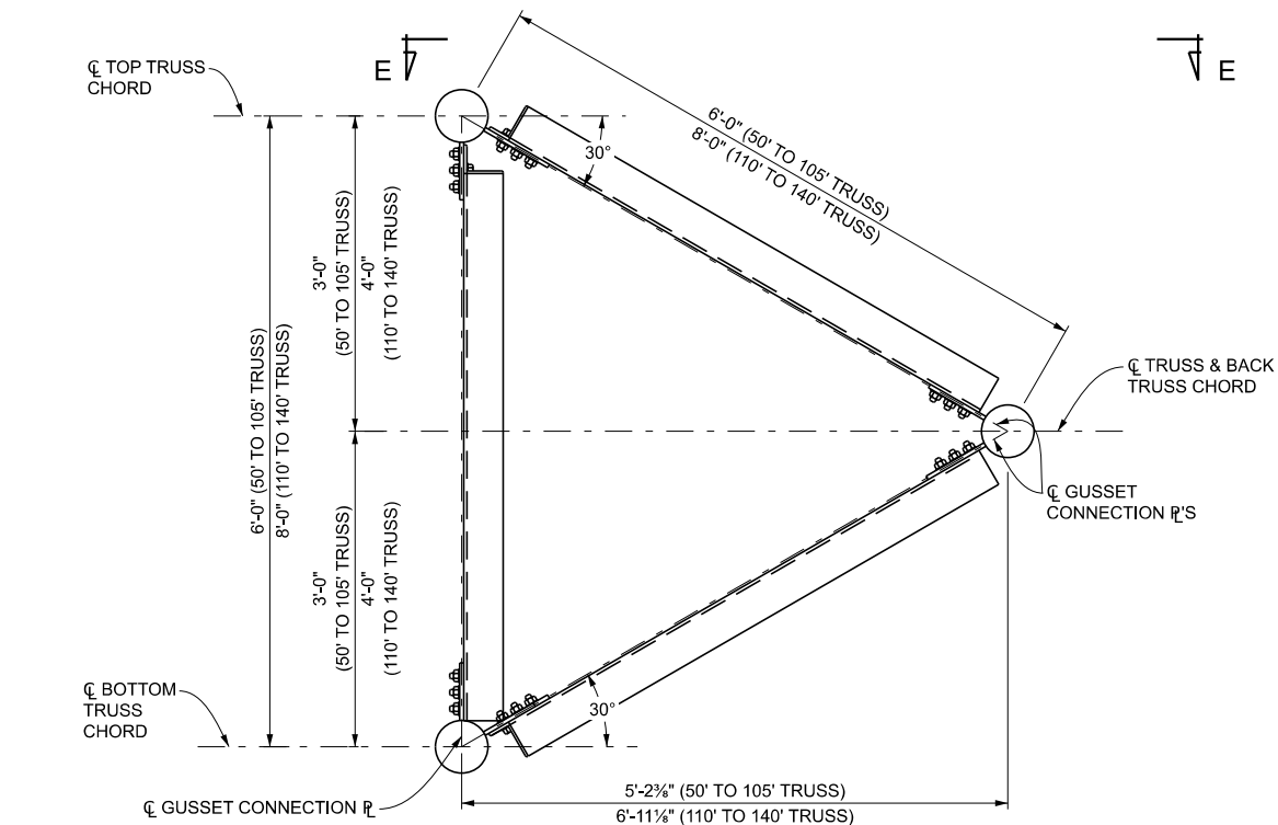
TYPICAL SECTION OF TRUSS
