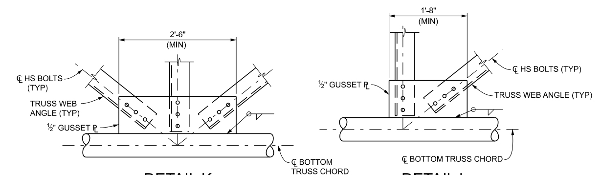
DETAIL K
