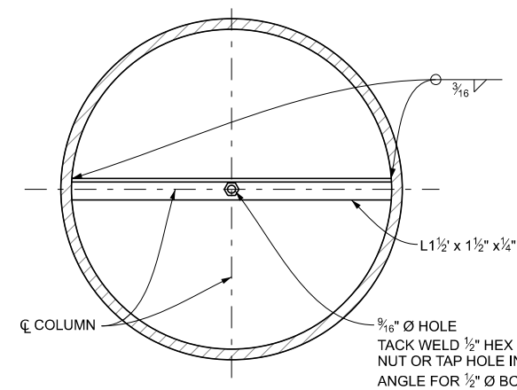
SECTION H-H
