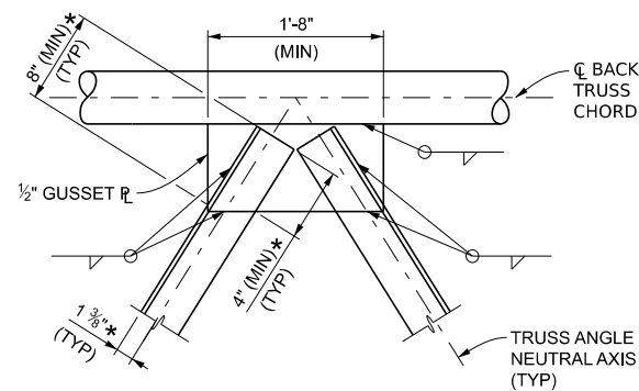
ALTERNATE DETAIL D
