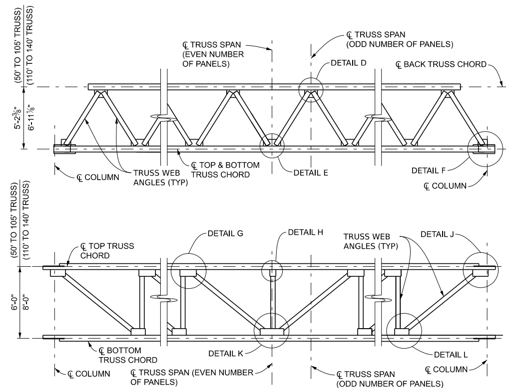
TYPICAL SECTION OF TRUSS
