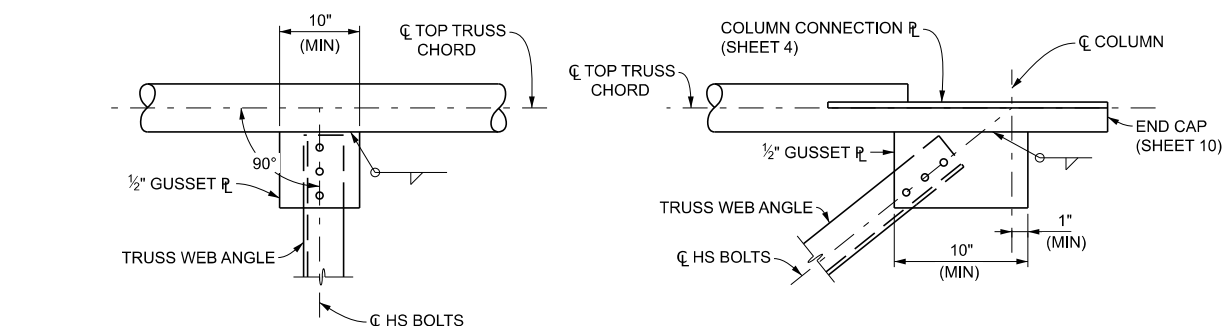
DETAIL H
