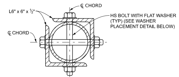
SECTION G-G
