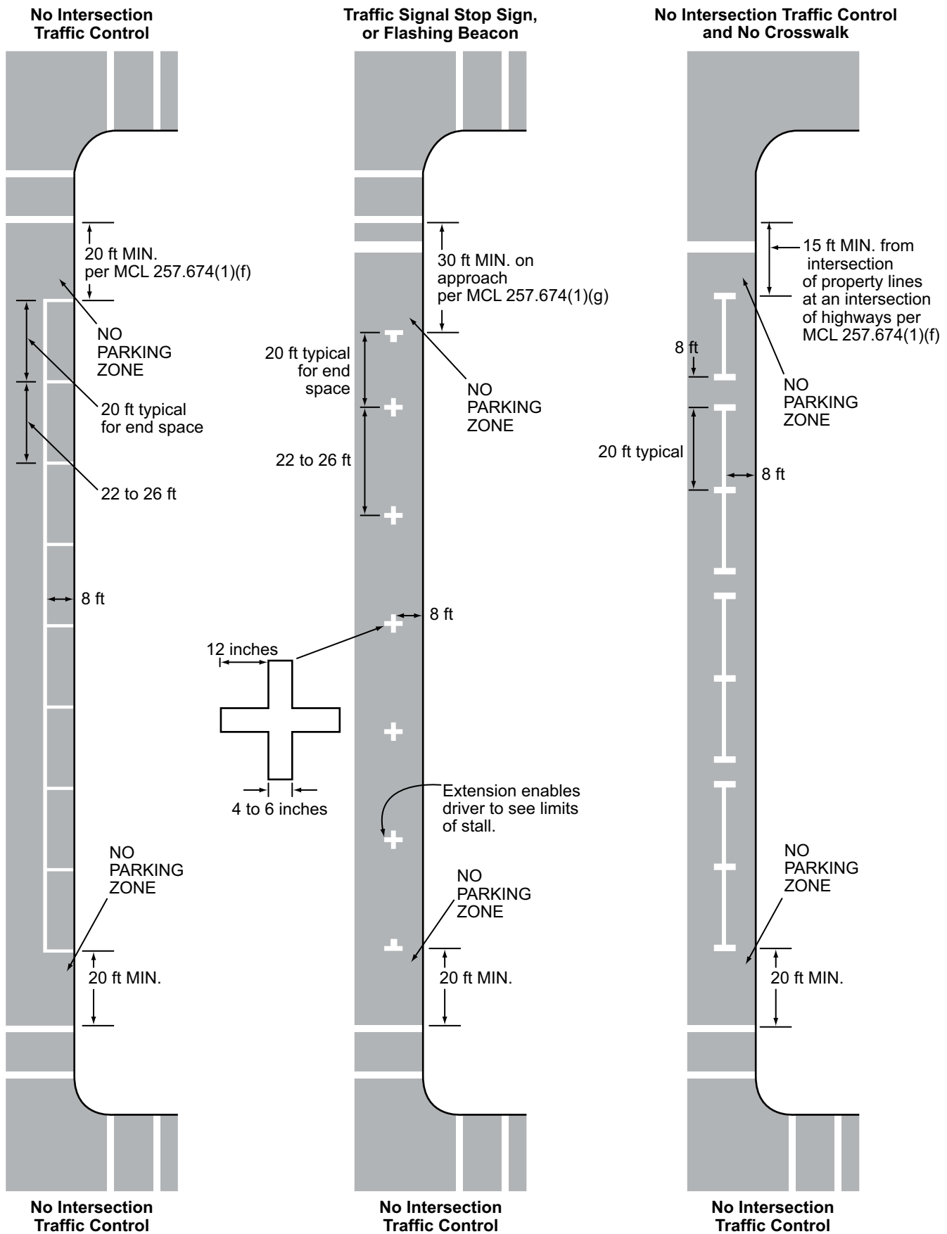
Figure 3B-21. Examples of Parking Space Markings
