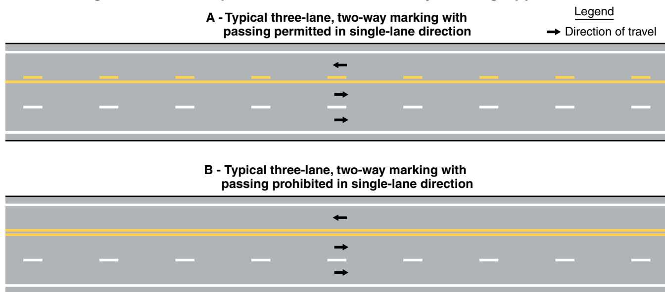
Figure 3B-3. Examples of Three-Lane, Two-Way Marking Applications
